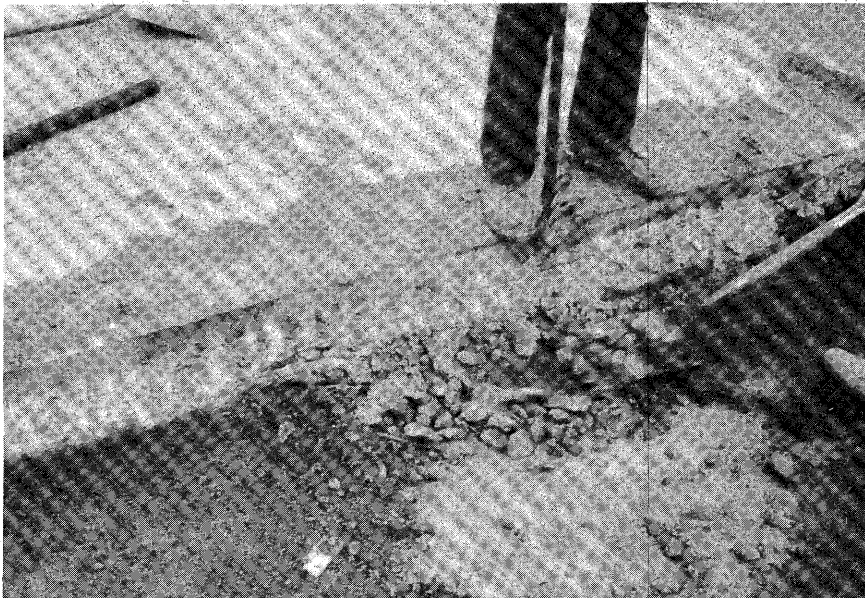
FIGURE 12 – CLEANING REPAIR AREA
