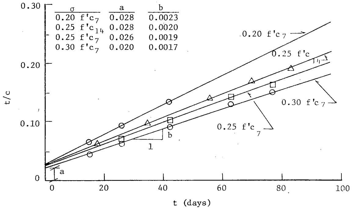
Figure A2--Creep constants according to Ross for group A specimens
