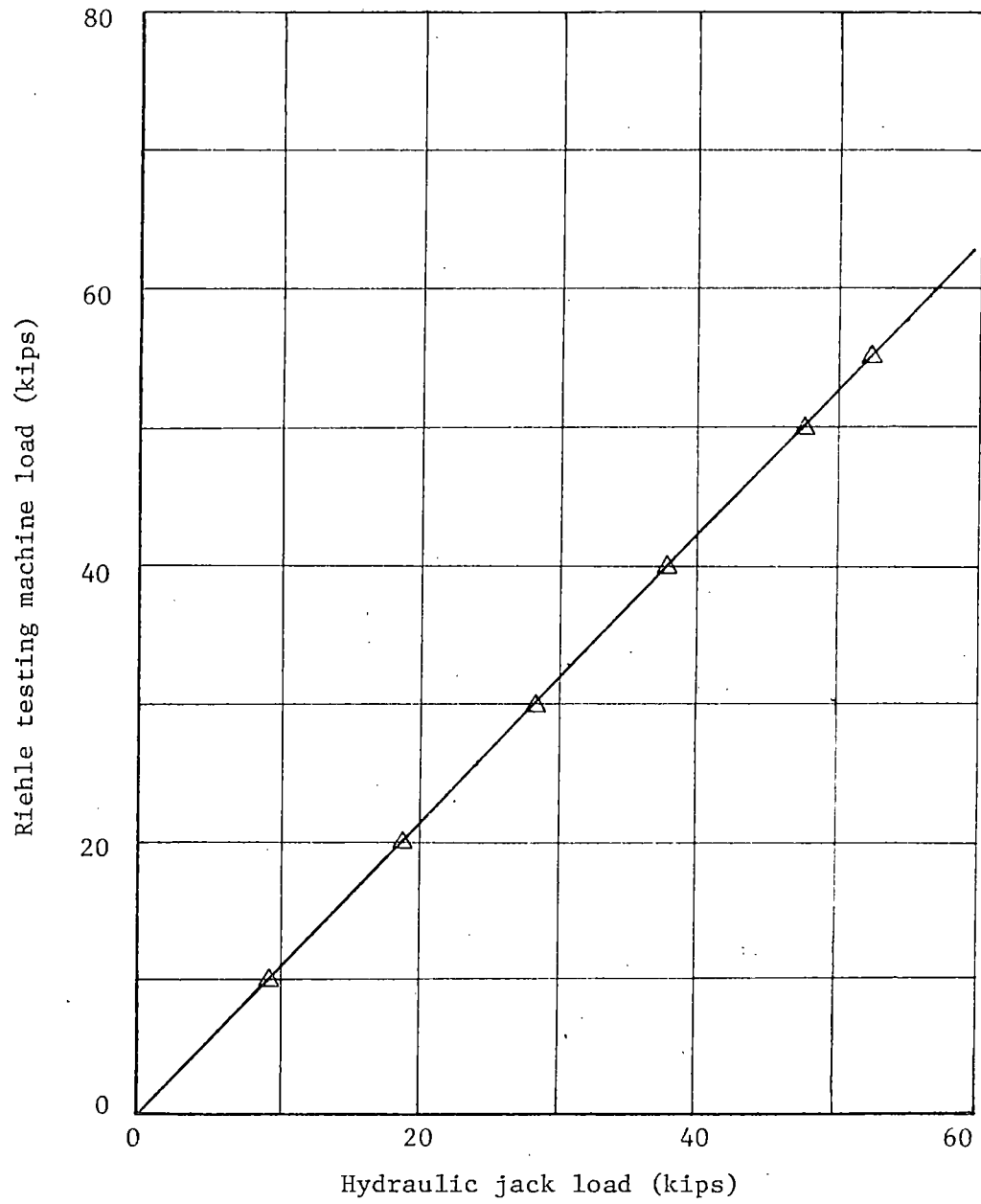
Figure 2--Calibration curve
