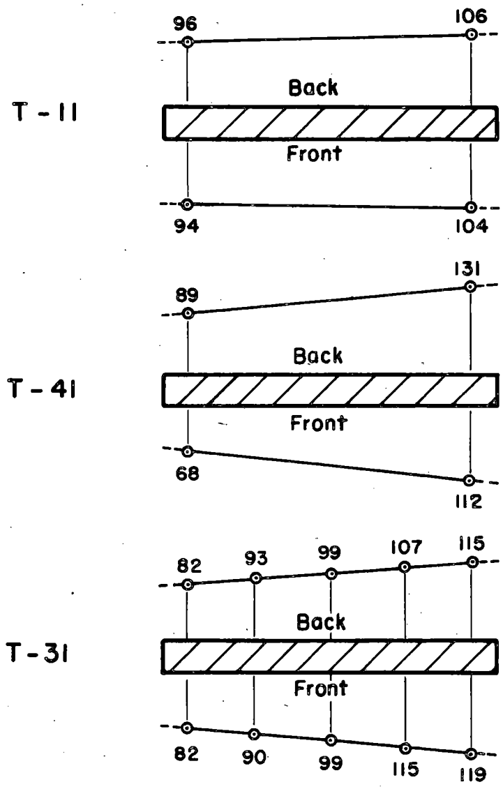
Fig. 34 Stress Distribution Patterns
