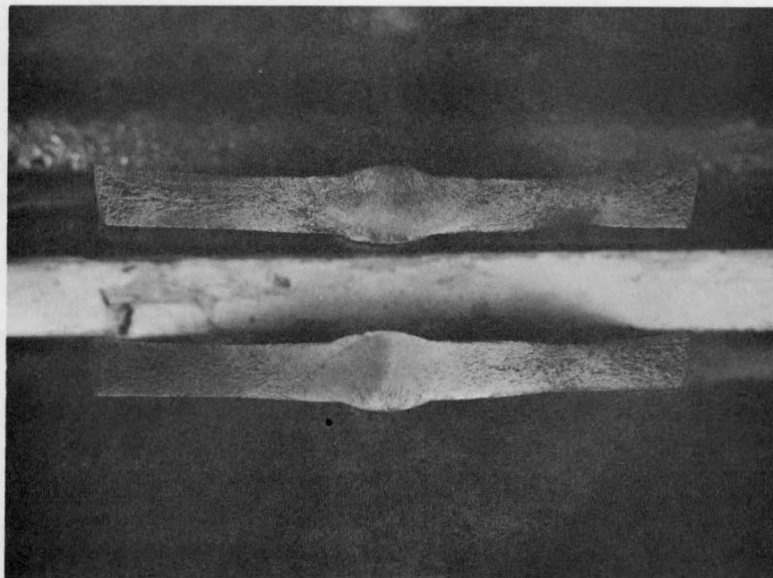
Fig. 38 Fracture Surfaces (T-32)
