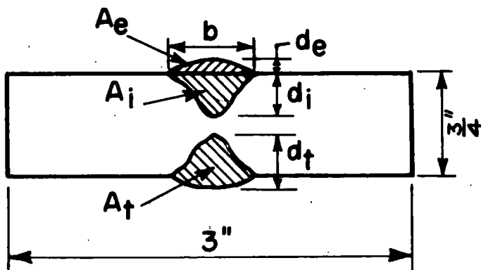
Fig. 5 Nomenclature for Weld Area Measurement
