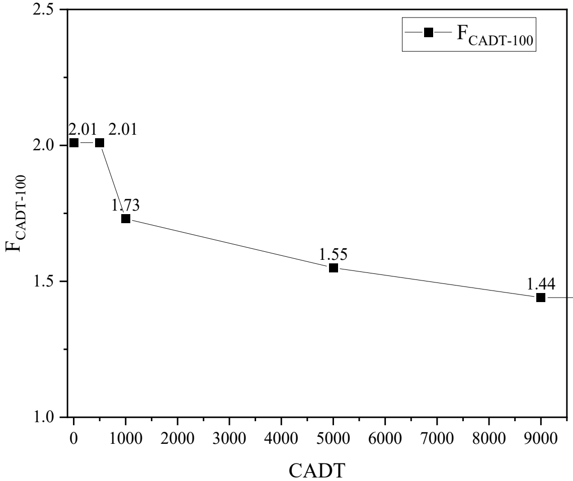
Figure 5.35. The adjustment factor for JPCP under different CADTs
