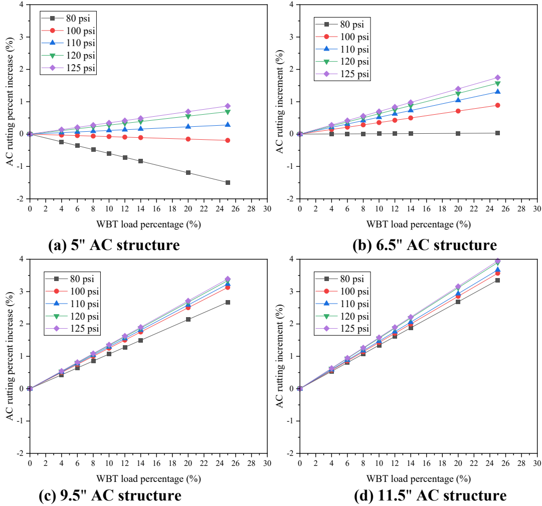
Figure 4.19. AC rutting increase at 95% reliability
