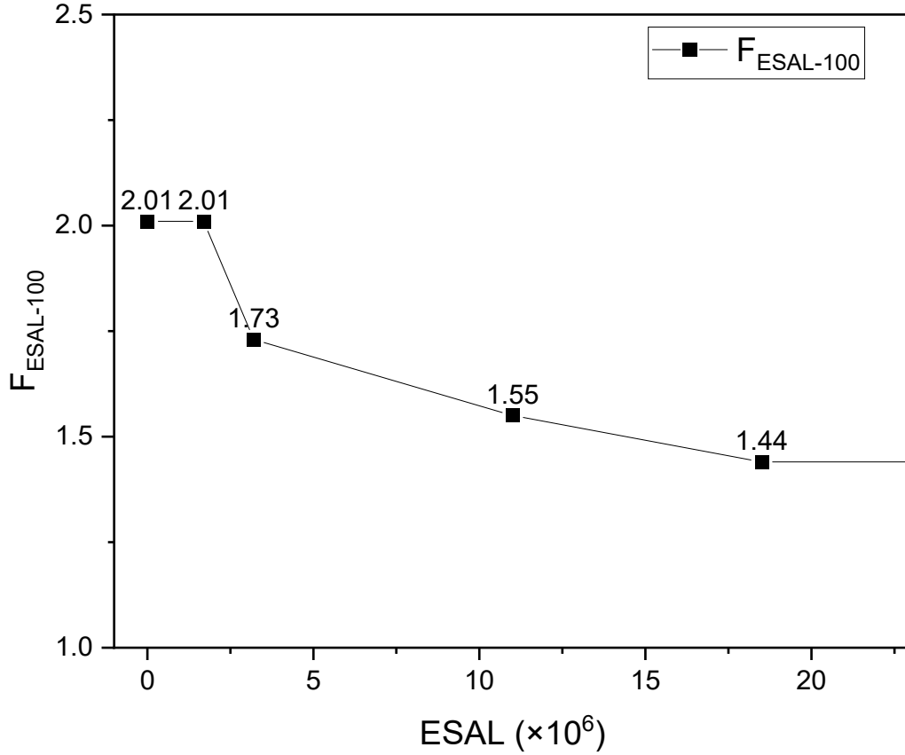
Figure 5.39. Adjust factor for JPCP under different ESALs
