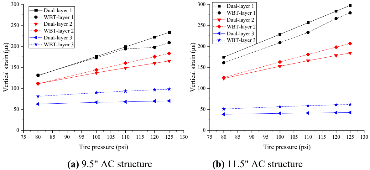
Figure 4.13. AC middle axial strain results
