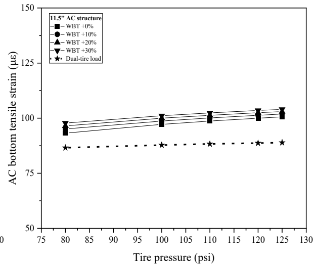
(e) 11.5" AC structure
