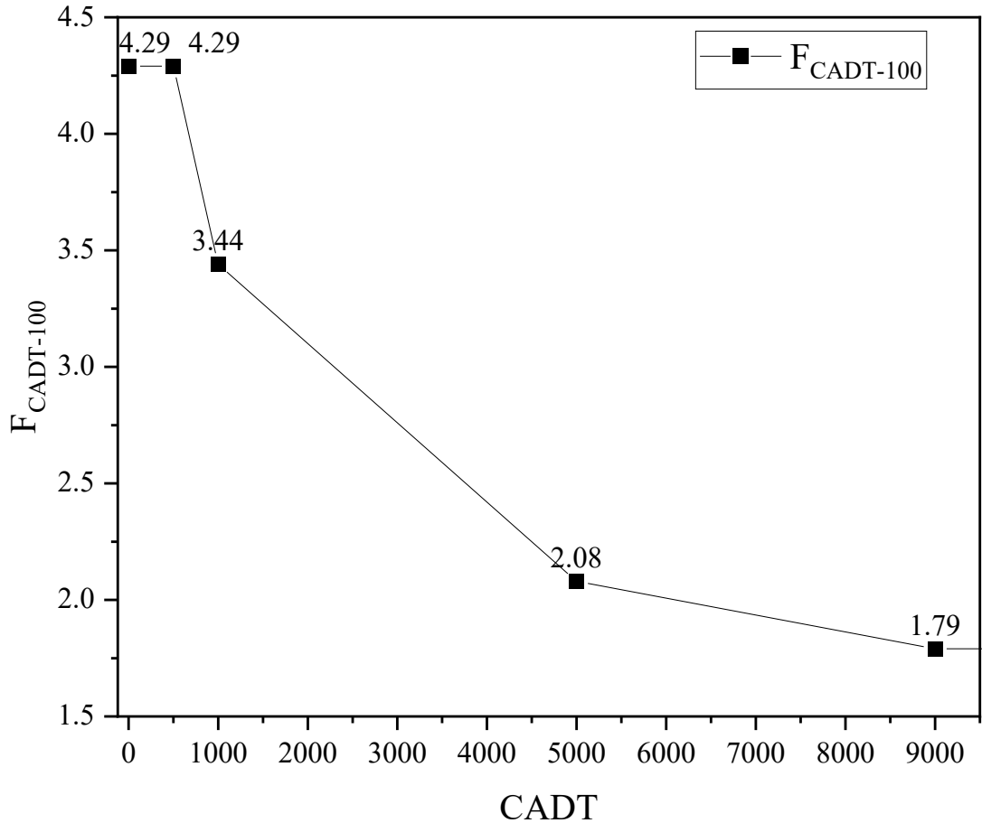
Figure 4.30. The adjustment factor for flexible pavement under different CADTs
