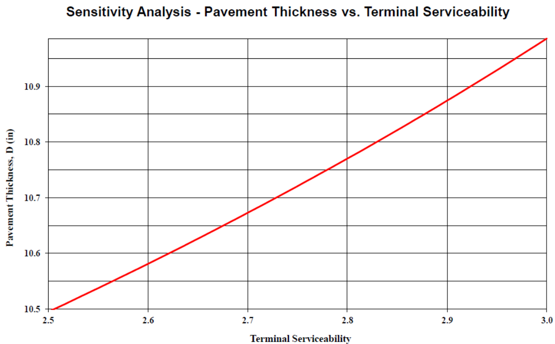
Figure 5.38. Sensitivity analysis of terminal PSI (ESALs: 1E7)
