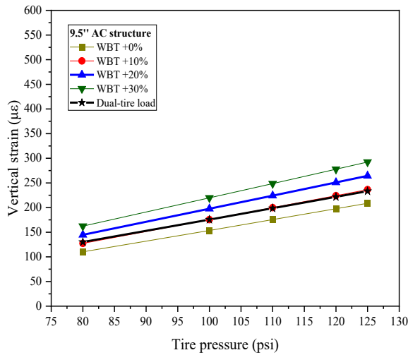
(a) 9.5" AC structure
