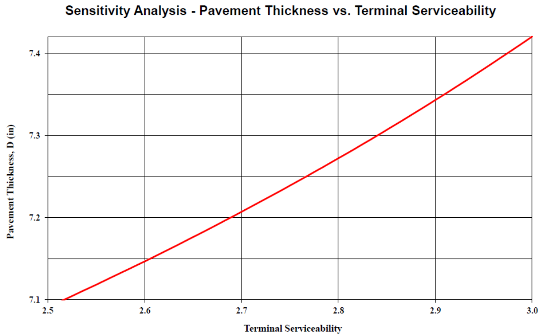
Figure 5.37. Sensitivity analysis of terminal PSI (ESALs: 1E6)
