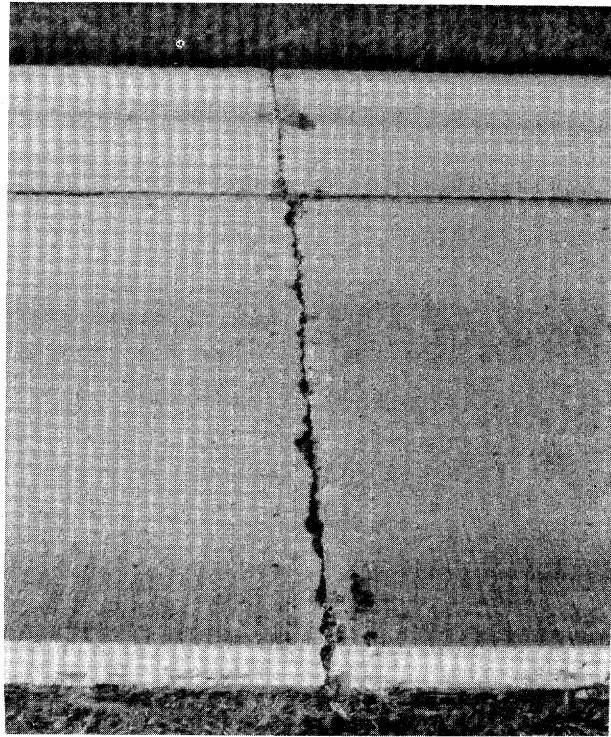
Figure 3.38. Low Severity Spalling (Transverse Joint).
