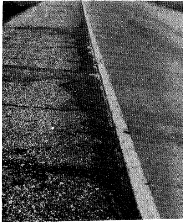
Figure 5.40. Low Severity Water Bleeding.
