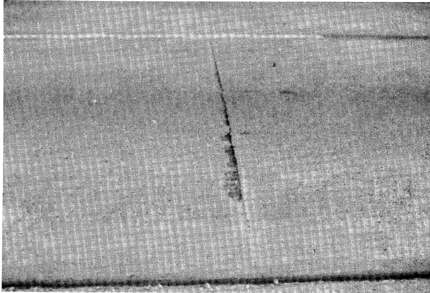
Figure 4.42. Low Severity Spalling (Fray).
