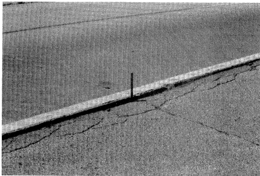
Figure 4.19. Lane/Shoulder Dropoff.
