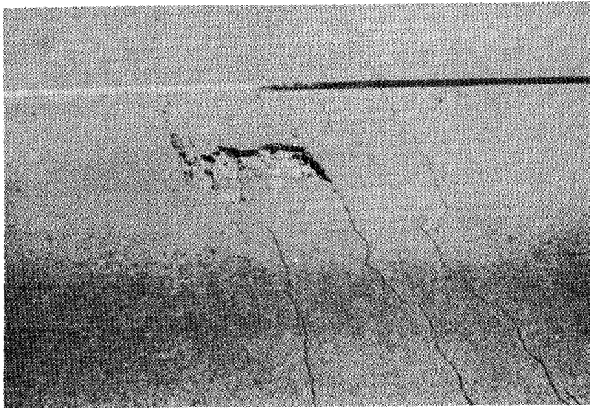
Figure 5.31. High Severity Localized Distress.
