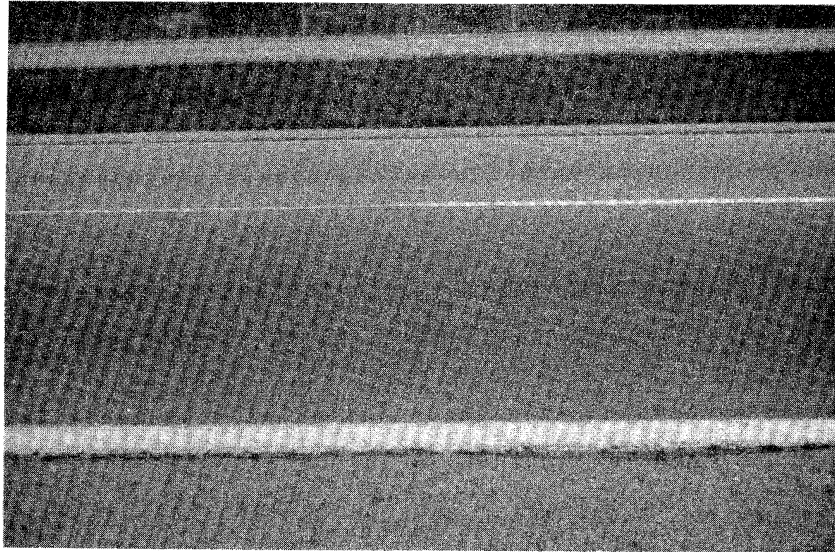
Figure 2.70. Low Severity Rutting.
