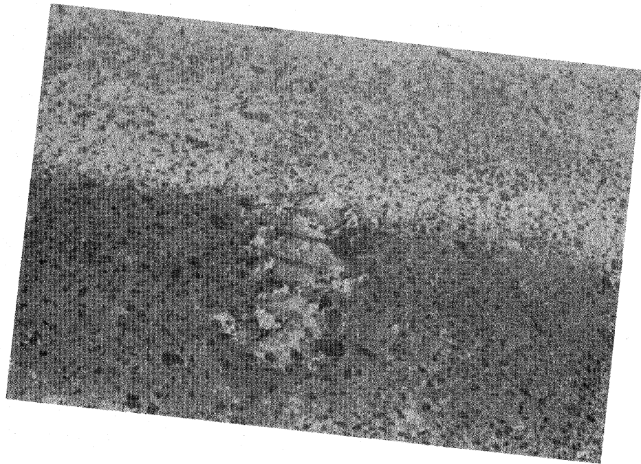
Figure 5.46. Medium Severity Scaling (steel close to surface).
