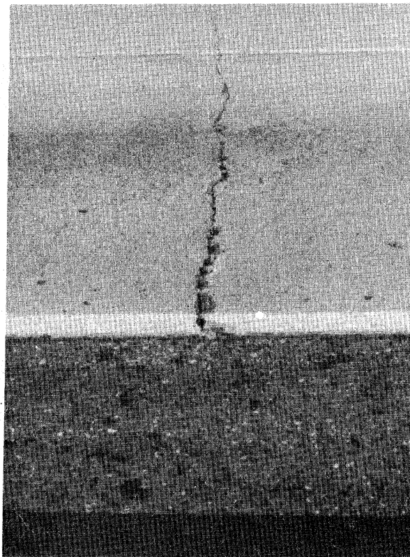
Figure 5.50. Medium Severity Spalling of Transverse Crack .
