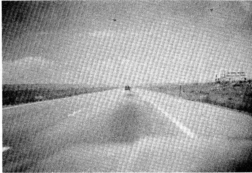
Figure 2.22. Low Severity Depression (identified by oil droppings on pavement surface).
