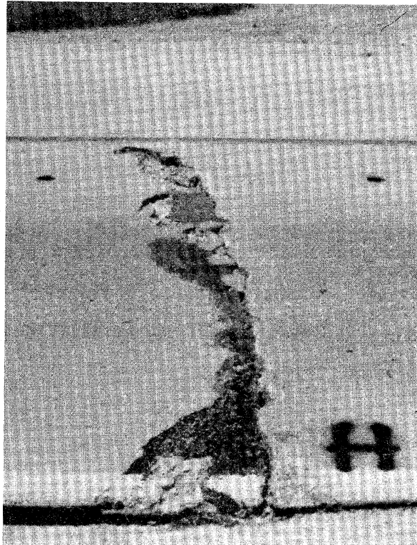
Figure 4.46. High Severity Spalling.
