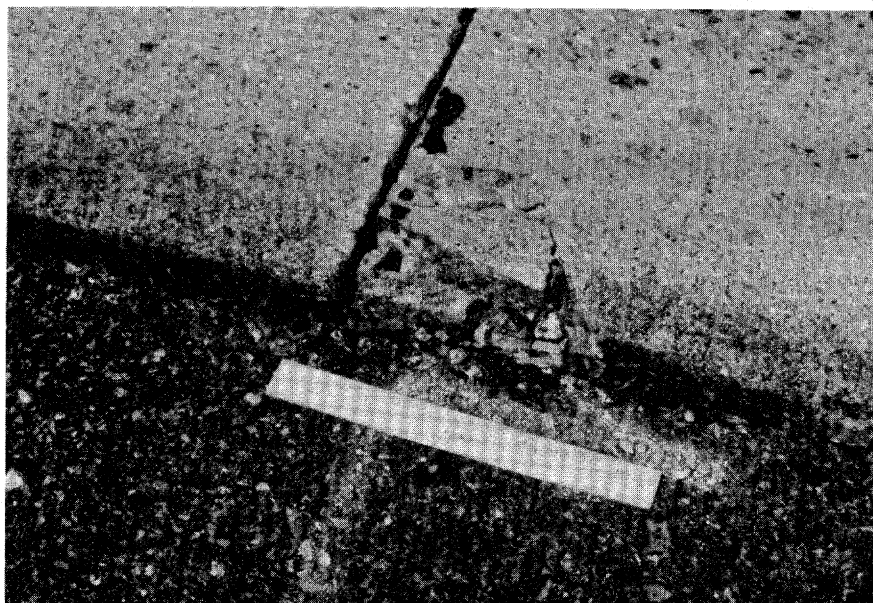
Figure 3.44. Low Severity Corner Spalling.
