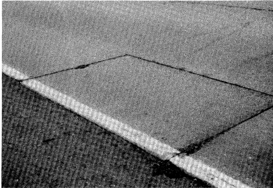
Figure 5.7. Medium Severity Concrete Patch Deterioration.
