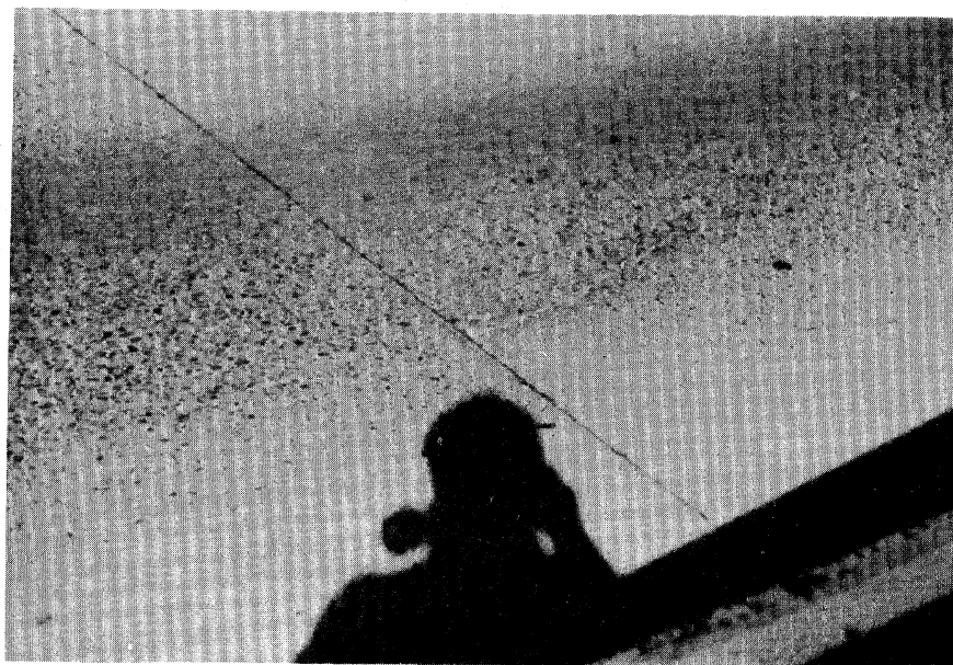
Figure 3.19. Low Severity Longitudinal Crack.
