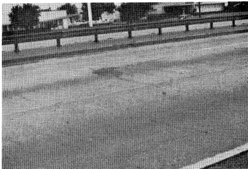
Figure 5.30. Medium Severity Localized Distress.
