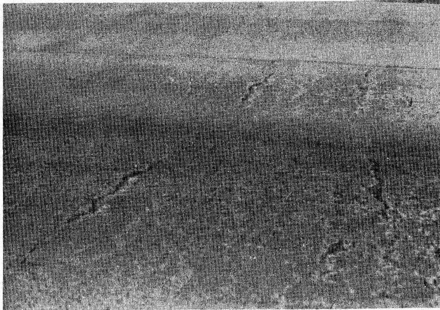
Figure 5.49. Low Severity Spalling of Transverse Cracks.
