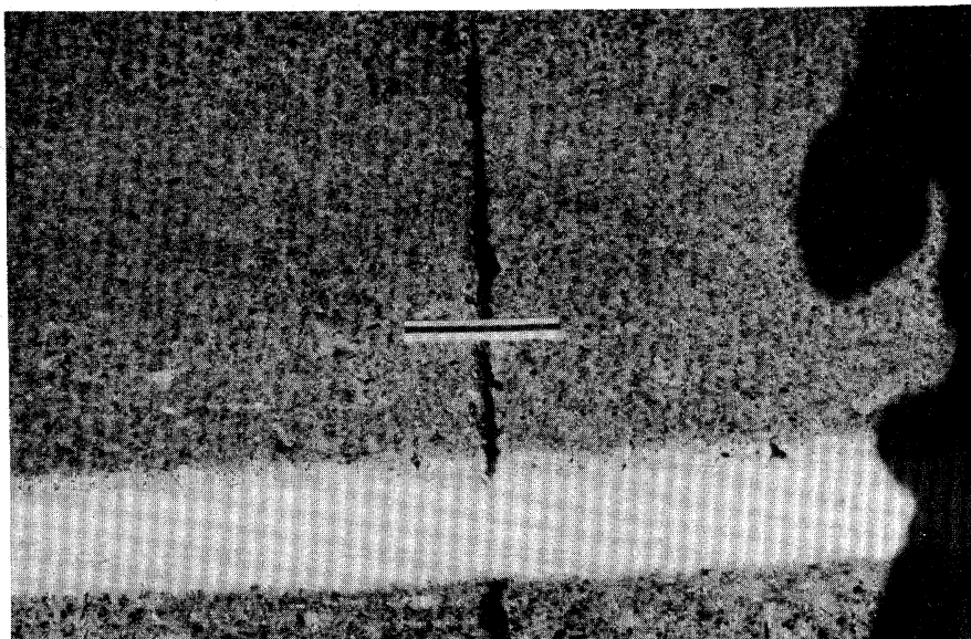
Figure 3.12. Medium Severity Joint Sealant Damage.
