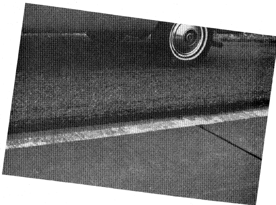
Figure 5.23. High Severity Lane/Shoulder Heave.
