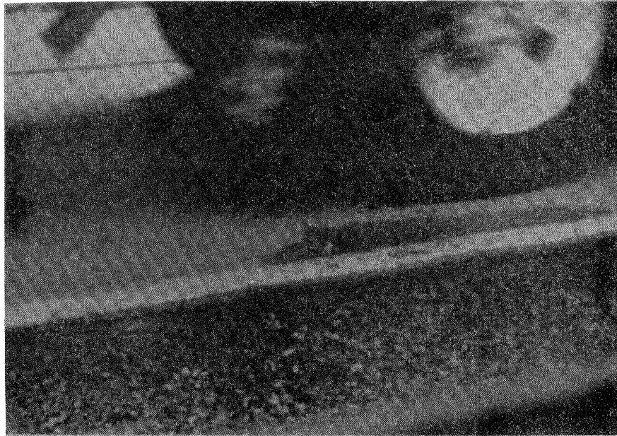
Figure 5.38. Low Severity Pumping (water ejected out of transverse crack under truck wheel).
