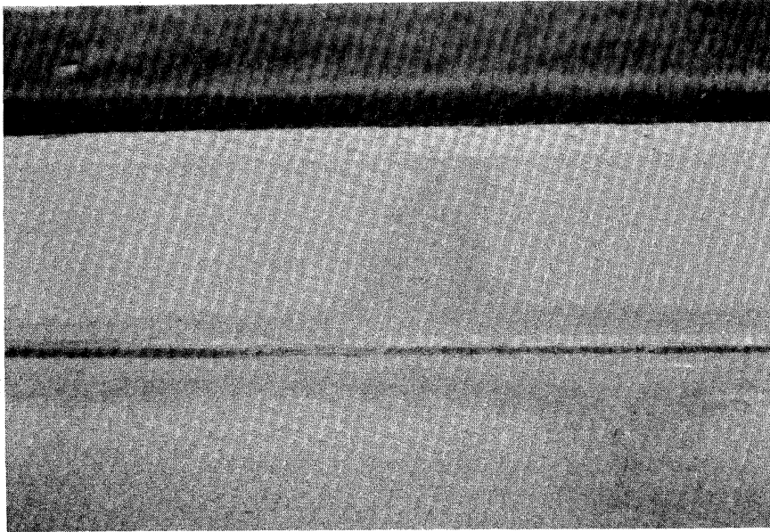
Figure 4.5. Low Severity "D" Cracking.
