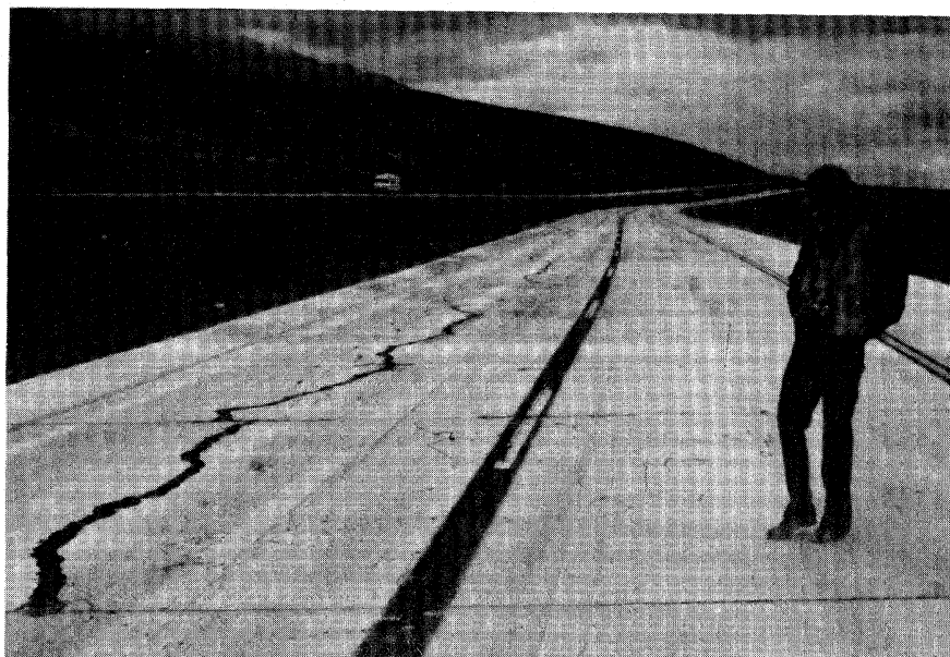
Figure 3.46. Swell Due to Frost Heave.
