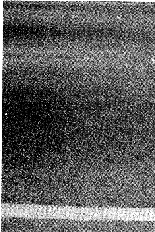
Figure 2.24. Low Severity Joint Reflection Cracking from Transverse Joint in PCC Slab.
