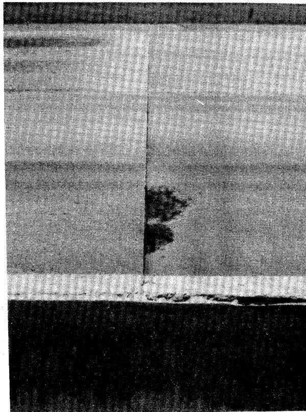
Figure 3.43. High Severity Spalling (Transverse Joint) (safety hazard).
