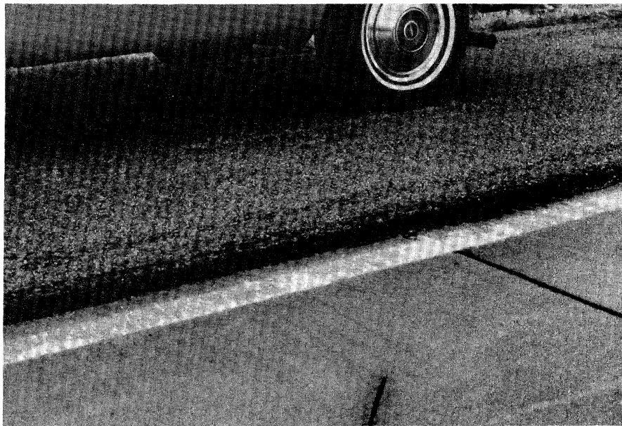
Figure 3.15. Lane/Shoulder Heave.
