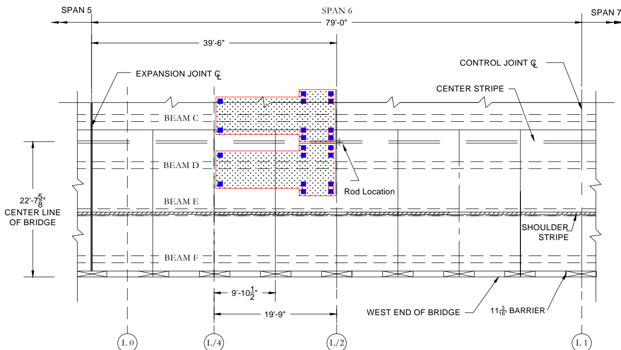
Figure 4.7 Truck Locations for Deflection Measurement of September, 2002
