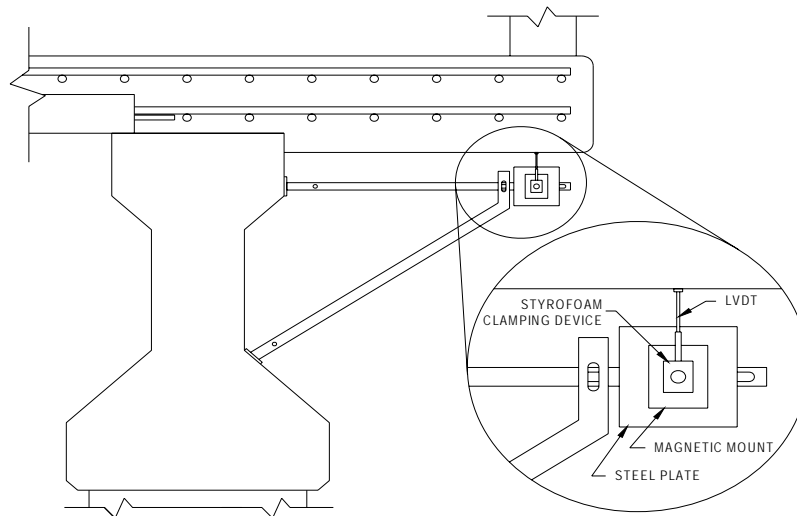
Figure 3.3 LVDT Mounted to Measure Overhang Displacements
