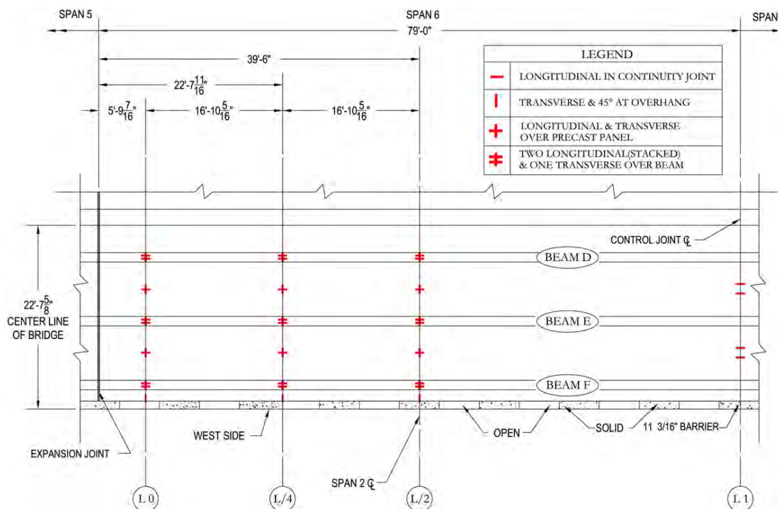
Figure 3.7 Embedded Strain Gauge Locations in Span 6
