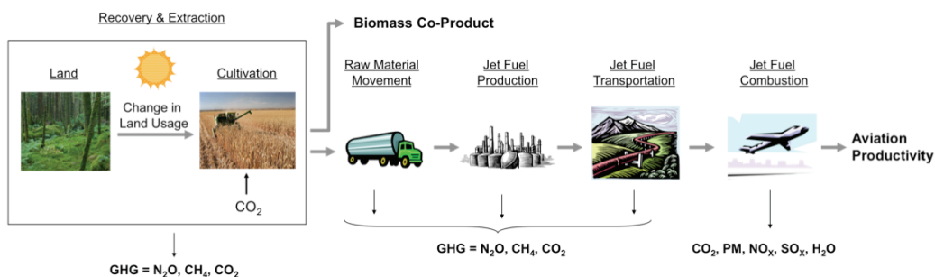
Figure B.2: Steps involved in the well-to-wake life-cycle analysis of bio-based alternative jet fuels.
