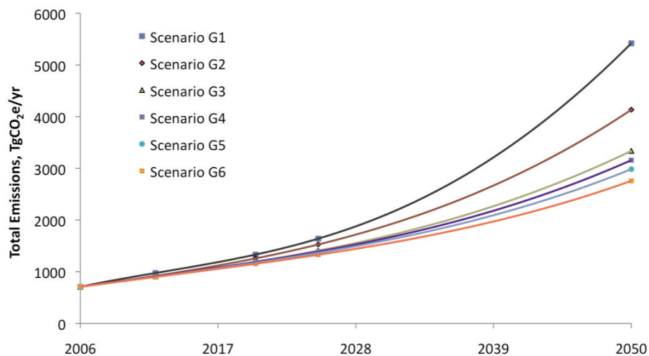
Figure B.20: Emissions from the projected fuel use cases developed for GIACC-4. The upper and lower extrema are taken as boundaries while Scenario 3 has been chosen to demonstrate the carbon mitigation potential if the fuels and the corresponding land requirements. The baseline jet fuel life cycle GHG emissions were used to estimate the total life cycle emissions.
