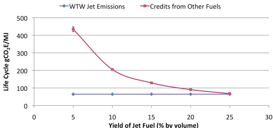
Figure B.5: The effects of product slate composition on life cycle emissions of F-T jet fuel
