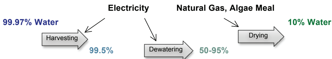
Figure B.10: Flow chart of dewatering and drying of algae
