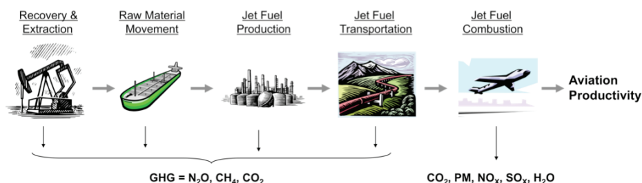
Figure B.1: Steps involved in the well-to-wake life-cycle analysis of jet fuel.
