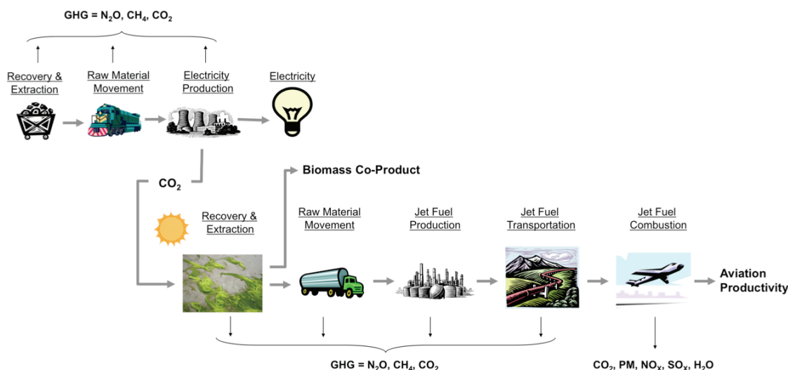
Figure B.3: Steps involved in the well-to-wake life-cycle analysis of bio-based fuels from algae.
