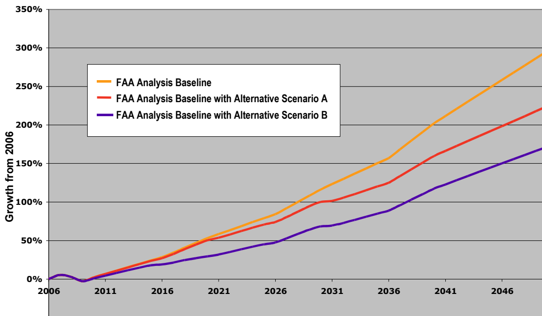
Figure 2: Global Fuel use Projected to 2050
