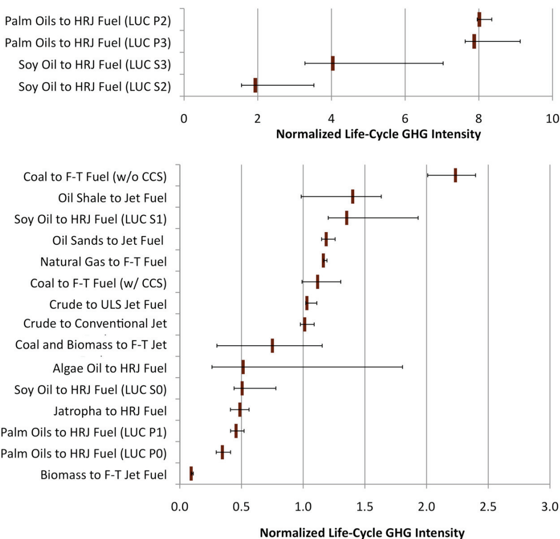
Figure B.18 Normalized life cycle GHG intensity for the alternative jet fuel pathways under consideration. Uncertainty bars represent the low emissions, baseline, and high emissions scenarios. Please note the different scales for the top and bottom portions of the figure. This is not an all-encompassing list of alternative jet fuel options; it merely represents those examined by the authors as part of their ongoing research. Note: CCS denotes Carbon Capture and Storage and Land Use Change (LUC) scenarios are defined in Table B.2.
