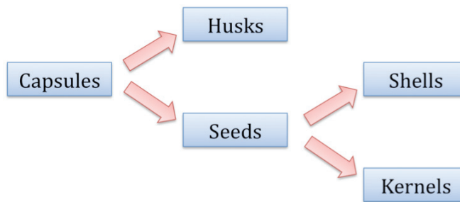
Figure B.13: Parts of the Jatropha fruit: husks, seeds, shells and kernels
