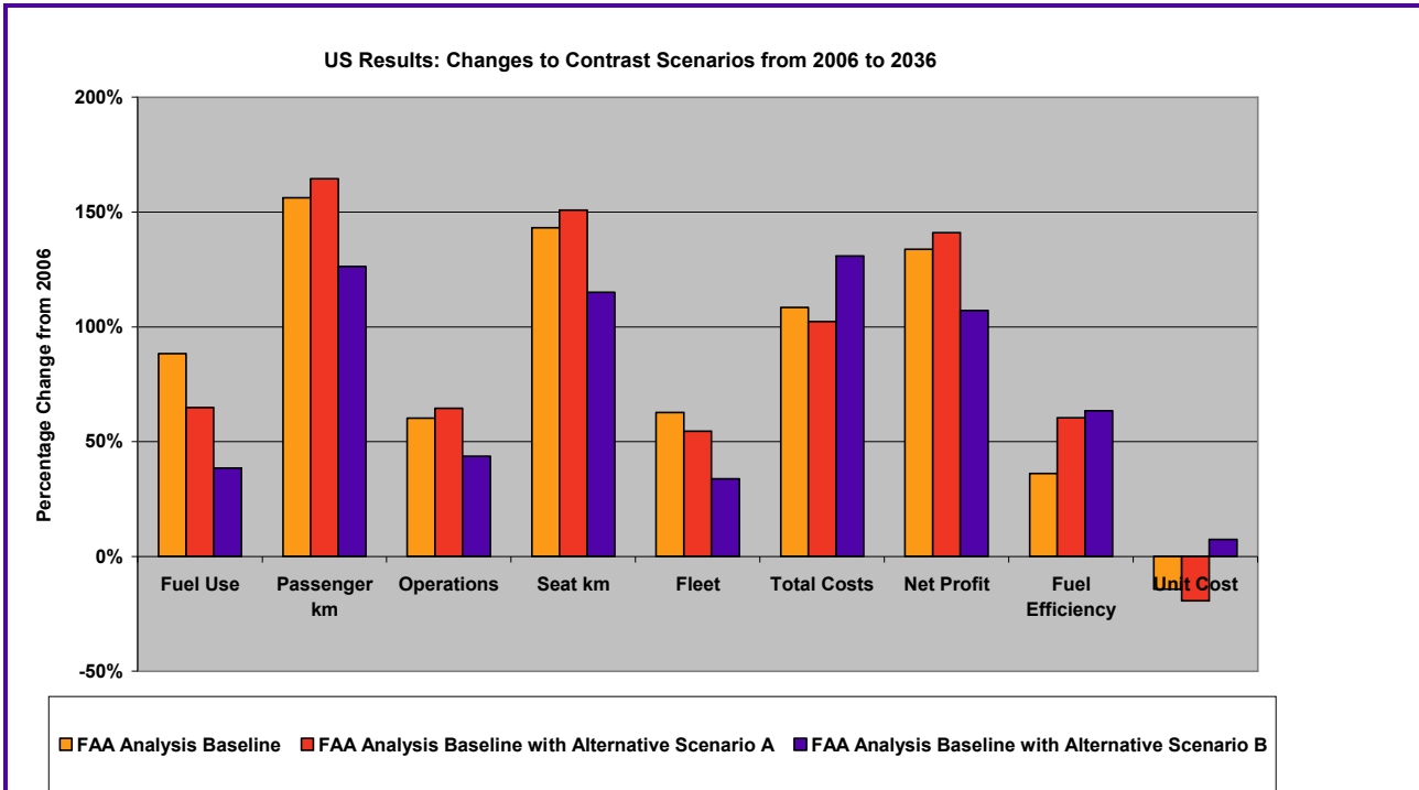
Figure 4.4 Comparison of Scenario Outputs at 2036 Relative to 2006 – U.S.
