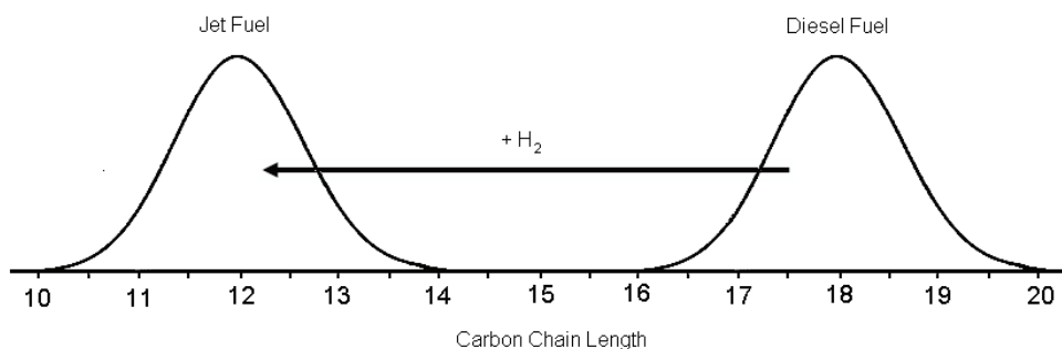
Figure B.4: Schematic showing the change in hydrocarbon composition between HRD and HRJ fuels that results from additional hydroprocessing.
