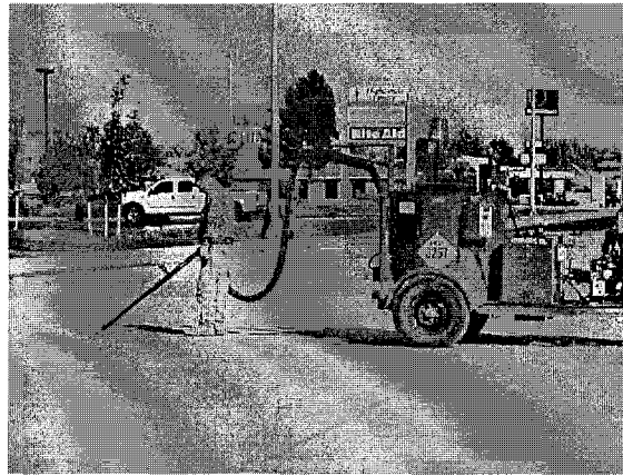
Figure 53 – Joint sealing of sawed construction joint
