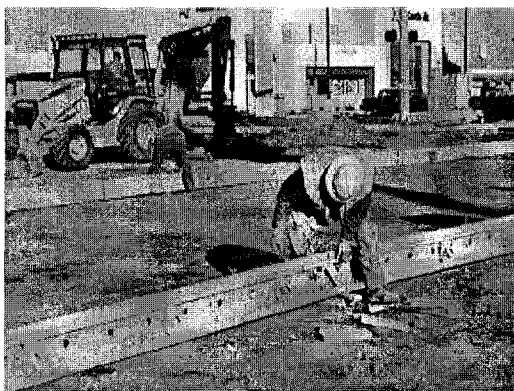
Figure 26 – Setting forms
