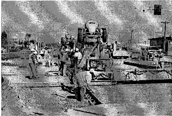
Figure 42 – Finishing concrete
