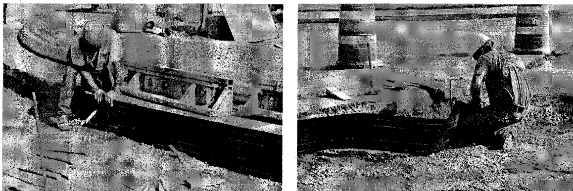
Figure 57 – Placement of roofing paper sheet as a bond breaker between existing curbing and new concrete slab
