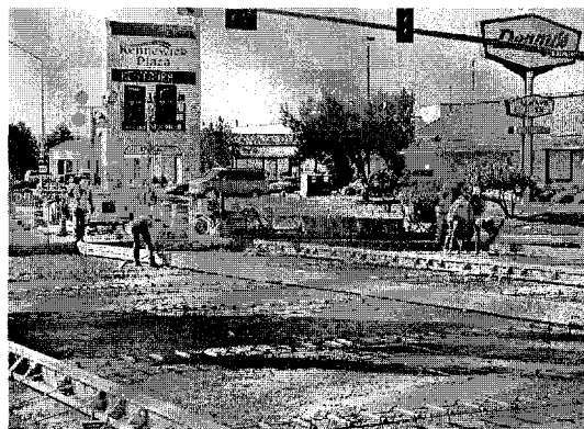
Figure 27 – Installation of dowel bar baskets
