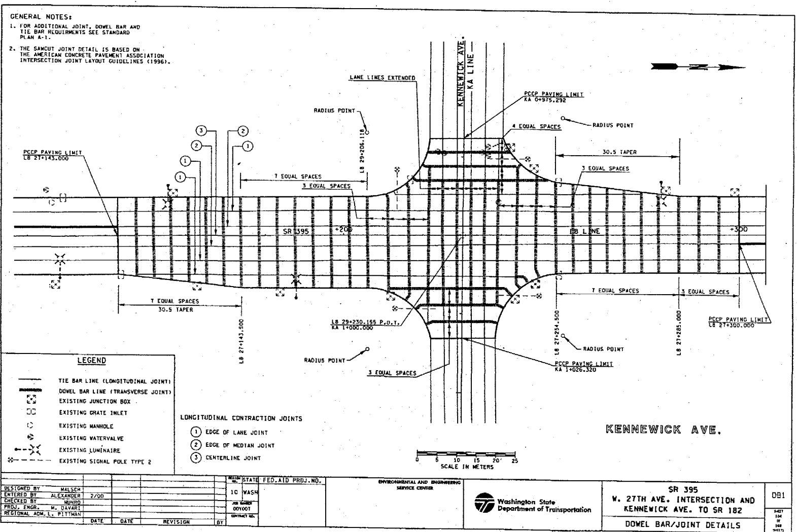
Figure 28 – Design criteria for installation of dowel bars and joint details
