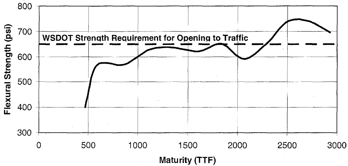
Figure 40 – Maturity vs. concrete flexural strength
