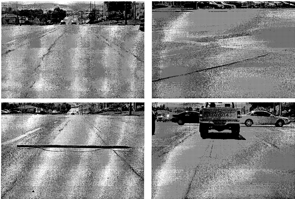
Figure 2 – Severity of pavement rutting at the intersection of W. Kennewick Avenue and SR 395
