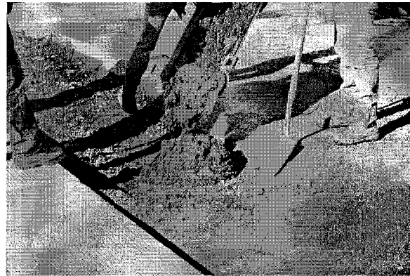
Figure 63 – Placing concrete at pourback area
