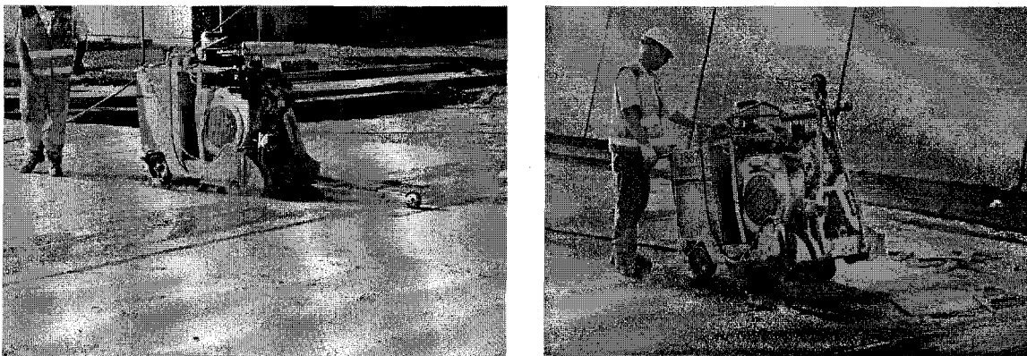
Figure 49 – Sawcutting freshly placed PCCP
