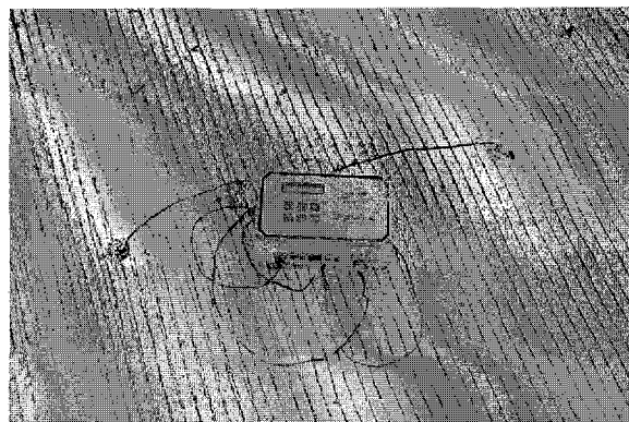
Figure 38 – Maturity meter sensors imbedded in concrete
