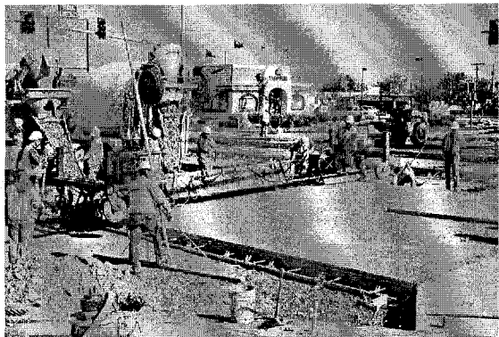
Figure 31 – Two Trucks delivering concrete
