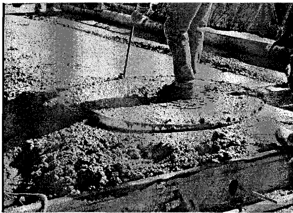
Figure 60 – Placing concrete inside and out side of the box out
