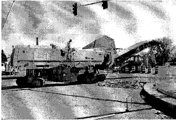
Figure 20 – Wirtgen W2200 Rotomill
