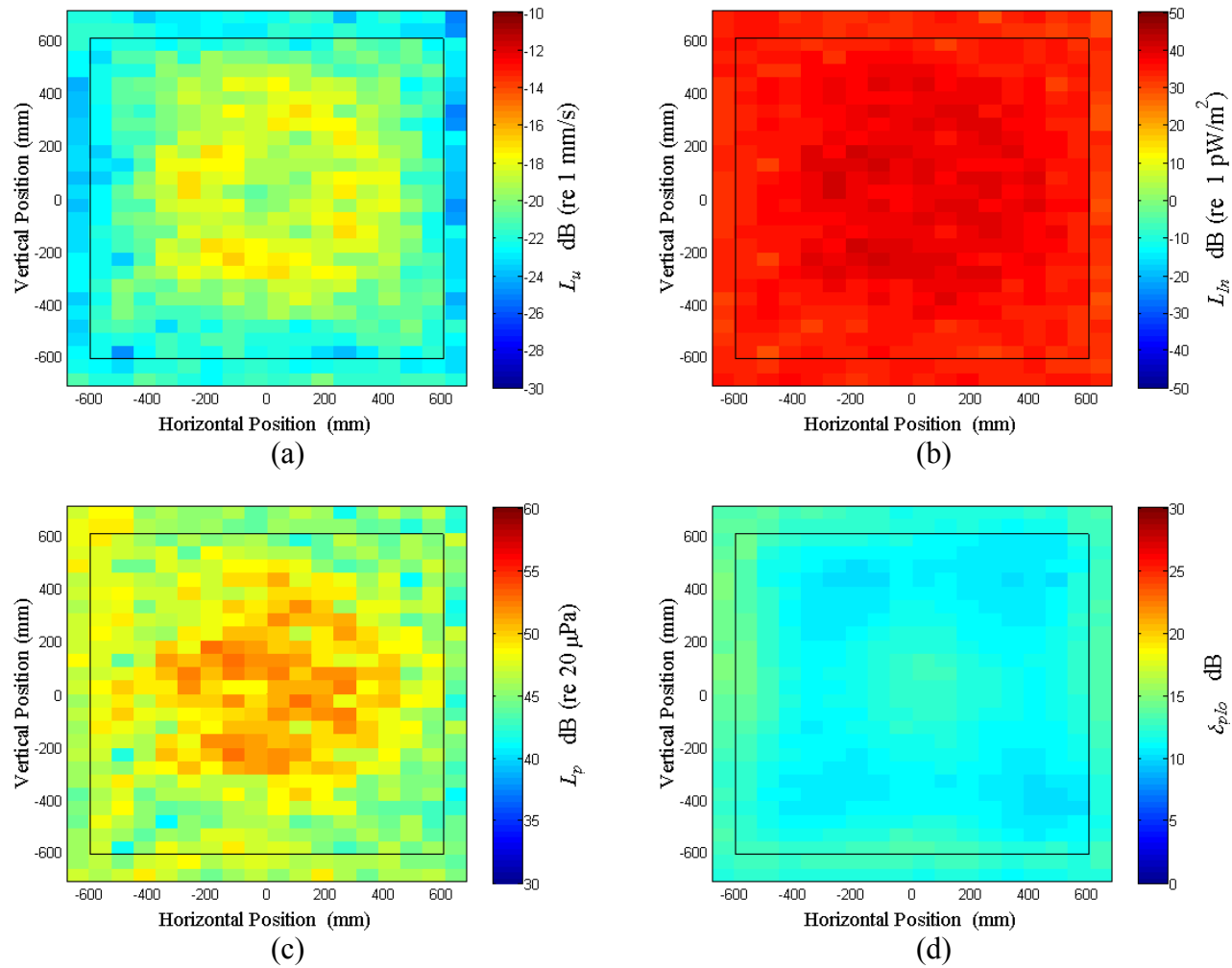
Figure E.39: Surface scan of Window E at 190 Hz (a) particle velocity level, L_u (b) normal signed sound intensity level, L_{In} (c) sound pressure level, L_p (d) pressure-residual intensity index, \delta_{plo} .
