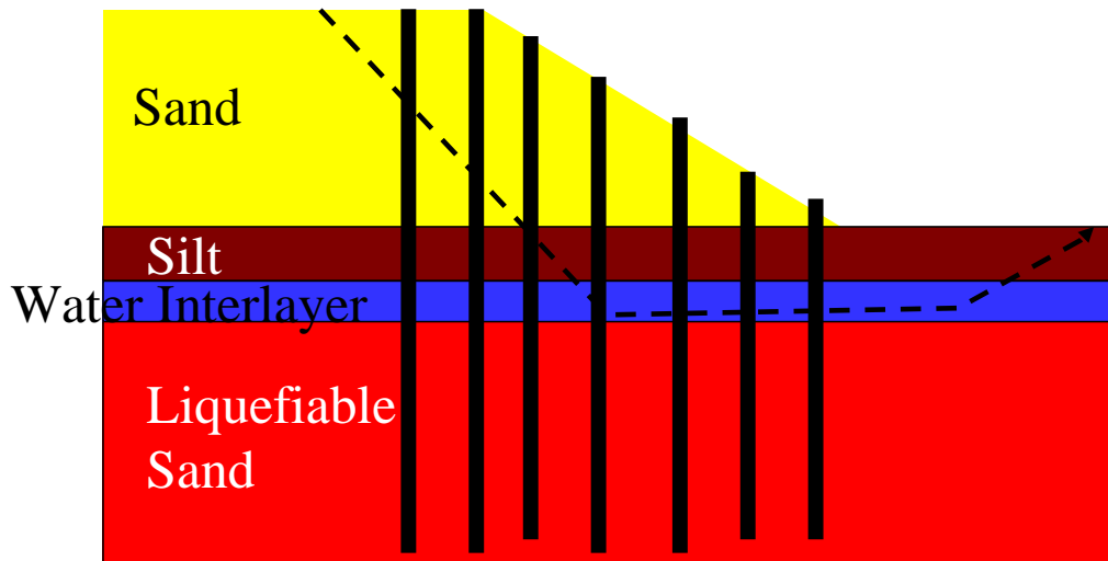
Figure 1 Schematic Drawing Showing the Potential for Vertical Drains to Relieve Pore Pressures and Intercept Water Interlayers Which May Form Below a Low Permeability Silt Layer
