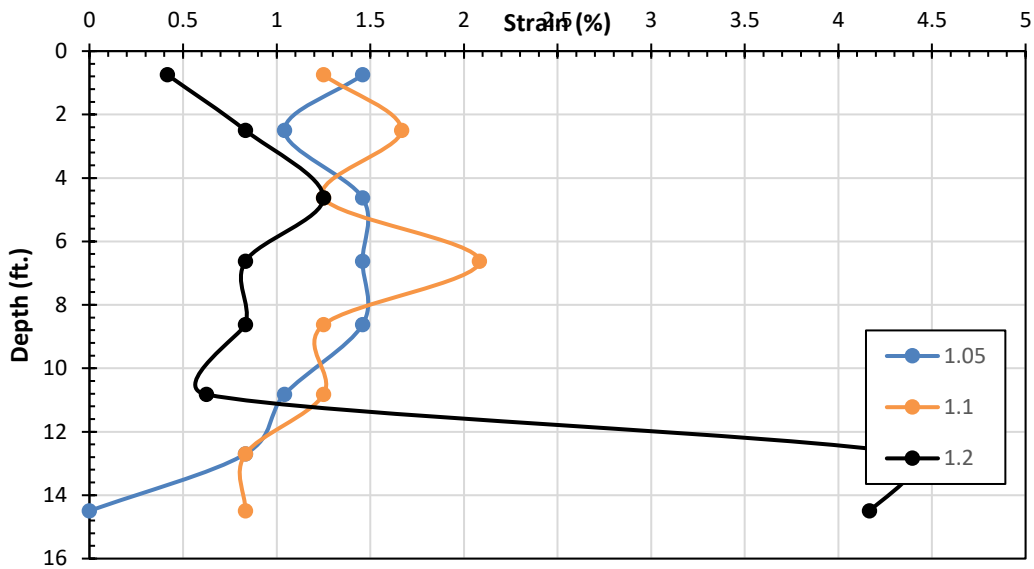
Figure 101 Profiles of Strain Versus Depth Using Smoothed Sondex Measurements for Round 1
