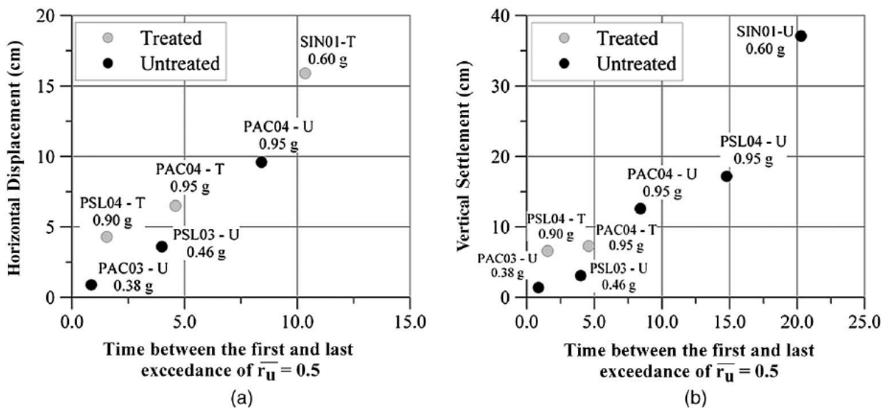
Figure 13 Horizontal and Vertical Deformations at Midslope in the Untreated and Treated Areas: (A) Horizontal Displacement, (B) Vertical Displacements as a Function of Time (in seconds) Between The First And Last Exceedance Of R_u=0.5 . (Howell et al. 2012).
