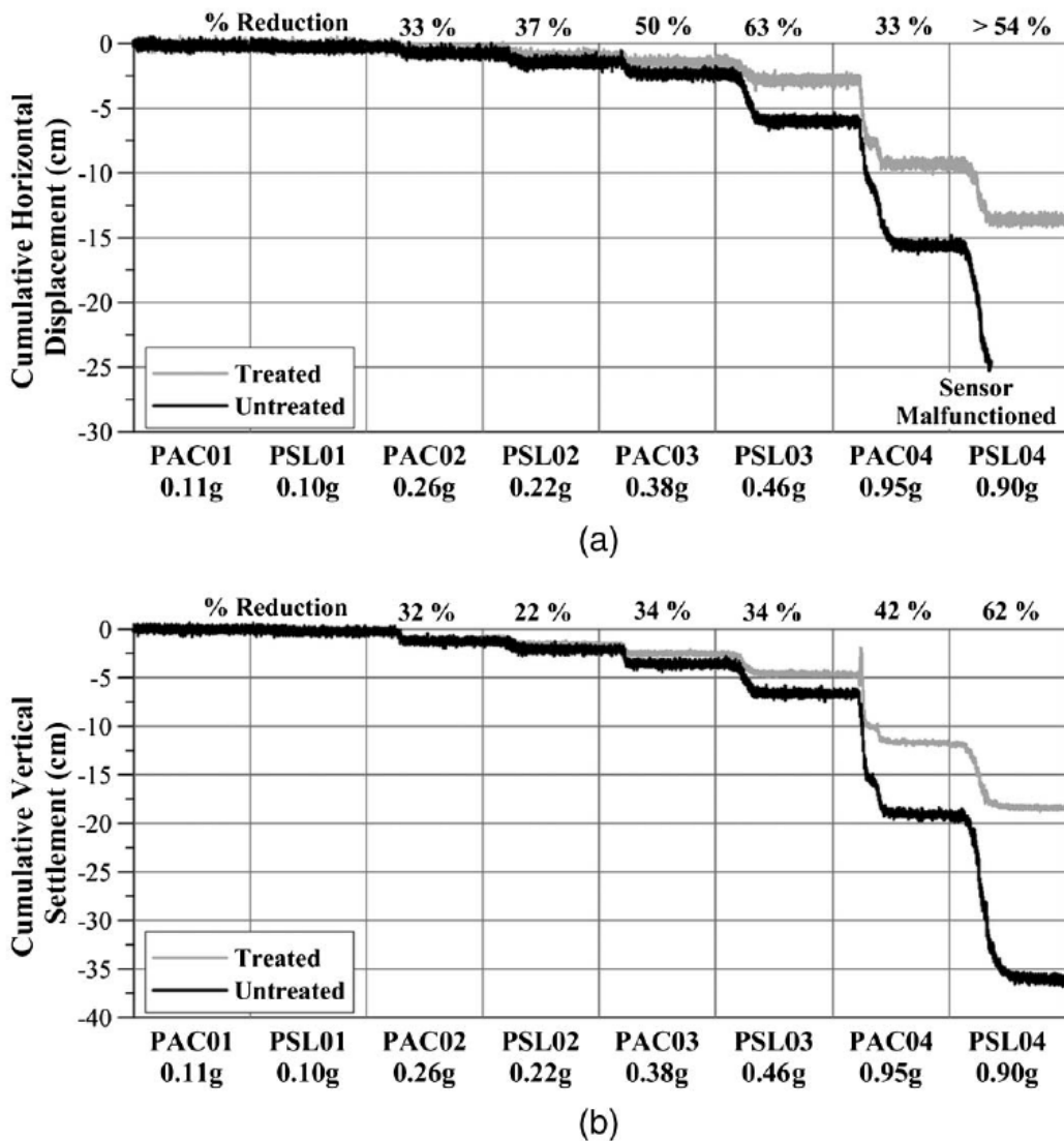
Figure 12 Cumulative (A) Horizontal and (B) Vertical Displacements at Mid-Slope in the Untreated and Treated Areas for All Shaking Events. (After Howell et al, 2012).
