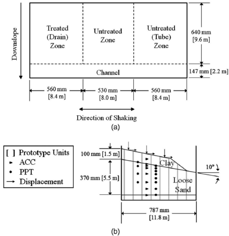
Figure 11 Layout for Centrifuge Test Comparing Behavior of Slopes in Liquefiable Sand with and Without Vertical Drains to Mitigate Liquefaction Hazard: (A) Plan; (B) Cross Section (Howell et al. 2012).
