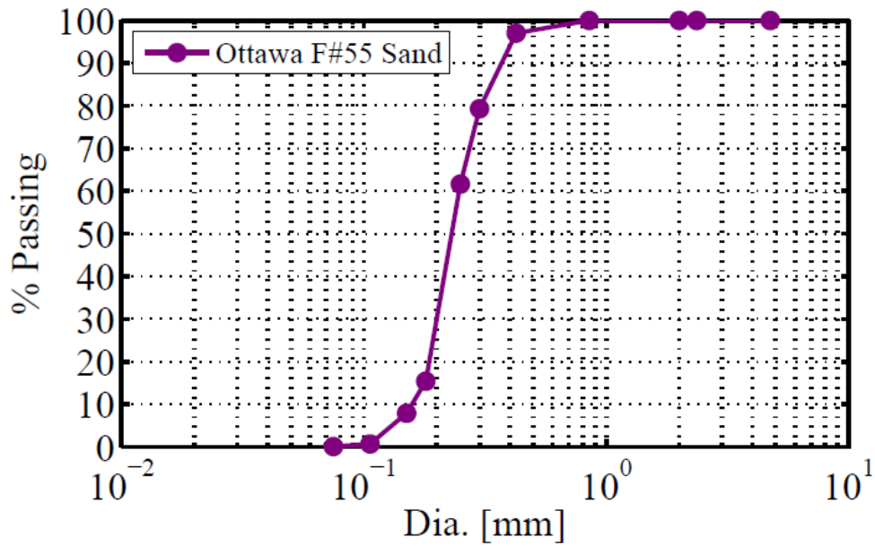
Figure 32 Grain Size Distribution for Ottawa F55 Sand
