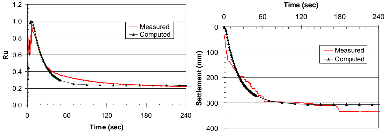
Figure 15 Comparison of (a) Measured and Computed Excess Pore Pressure Ratio ( r_u ) Versus Time at a Depth of 11.8 m and (b) Measured and Computed Settlement Versus Time Curves for the Vancouver Test Site. (Rollins et al, 2004).
