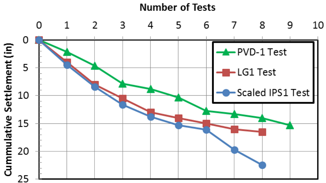
Figure 69 Comparison of Cumulative Settlement from PVD-1 with Other Tests
