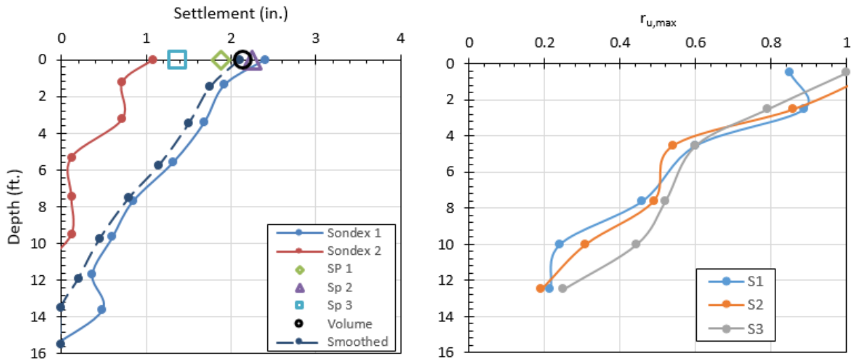
Figure 92 Profiles of Liquefaction Induced Settlement and Maximum Excess Pore Pressure Ratio ( r_{u,max} ) for Round 1 with a_{max} = 0.05 g.
