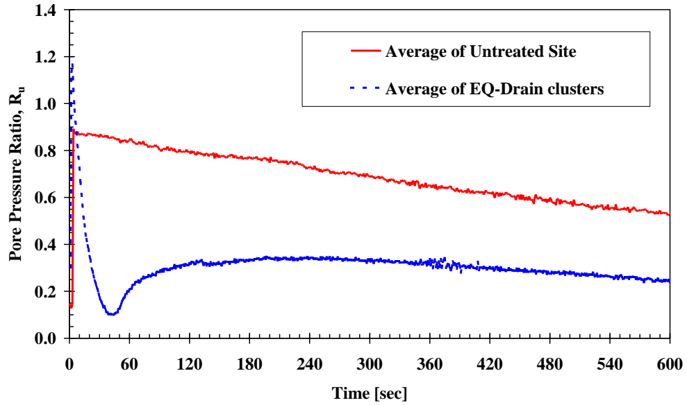
Figure 3 Comparison of Excess Pore Pressure Ratio as a Function of Time at Sites Treated with EQ Drains Relative to an Untreated Test Site (Rollins et al. 2003).
