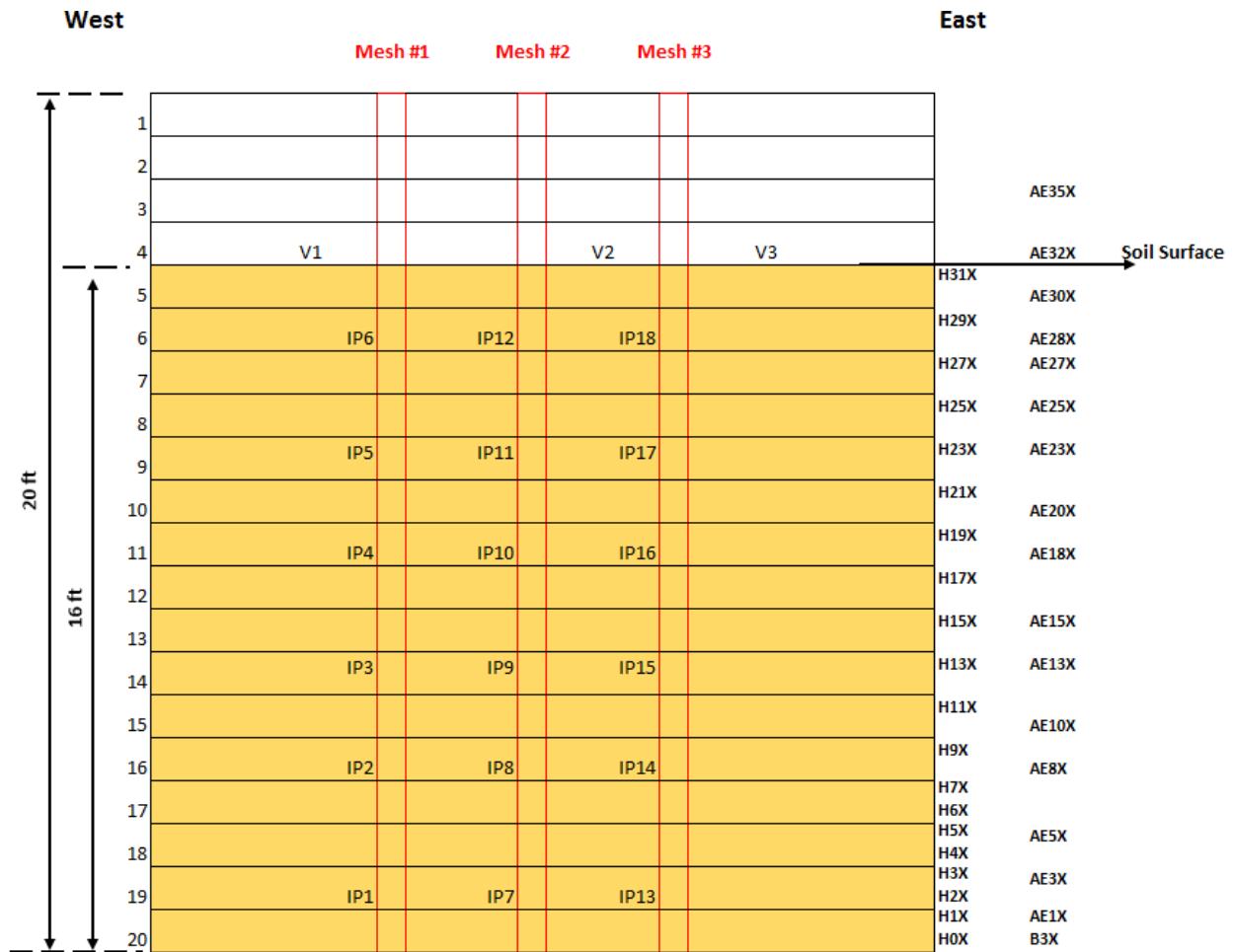
Figure 74 Profile View of Sensors Installed for PVD-2. Numbers on the right side of the figure indicate the LVDTs (H—X) or the accelerometers (AE—X)
