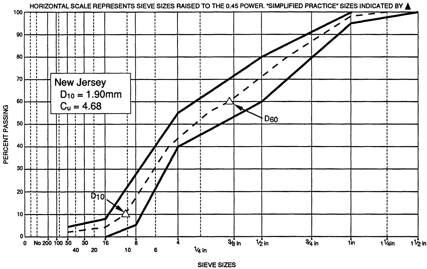
Figure 28. Plot of New Jersey Gradation
