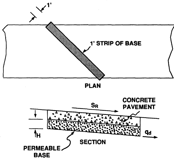
Figure 16. Sketch of Permeable Base Capacity
