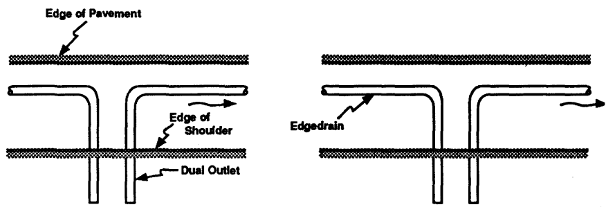
Figure 43. Edgedrain Design for Maintenance
