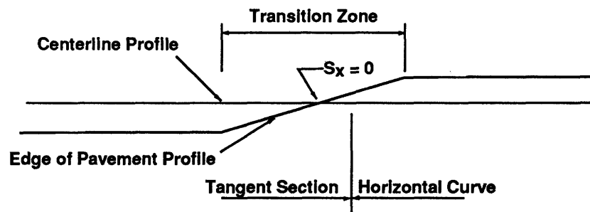
Figure 6. Horizontal Curve Transition
