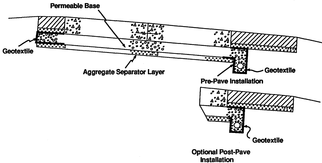
Figure 26. Edgedrain Location for Concrete Pavement with Asphalt Concrete Shoulders
