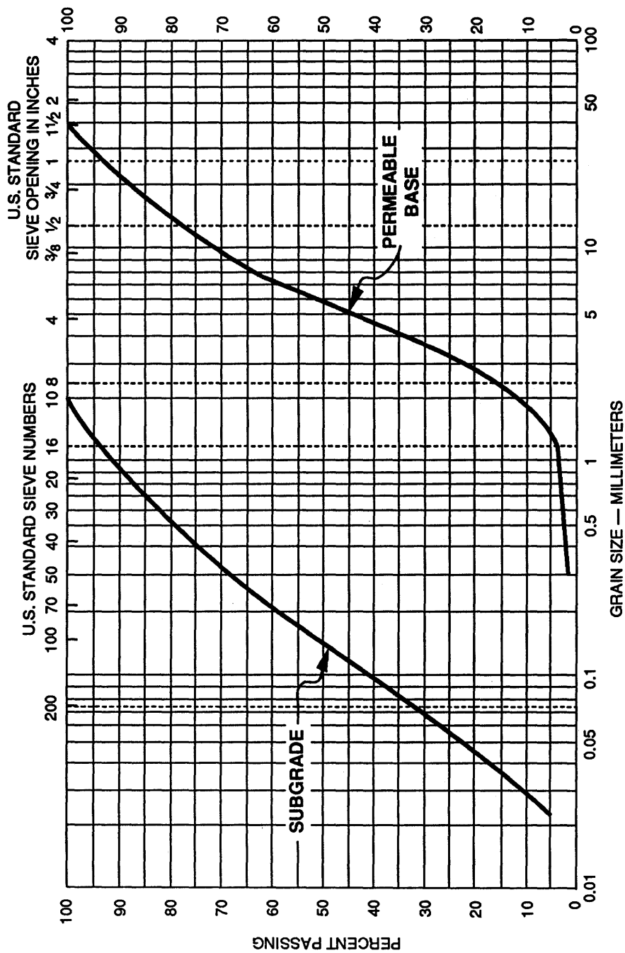
Figure 34. Plot of Subgrade and Permeable Base Gradations
