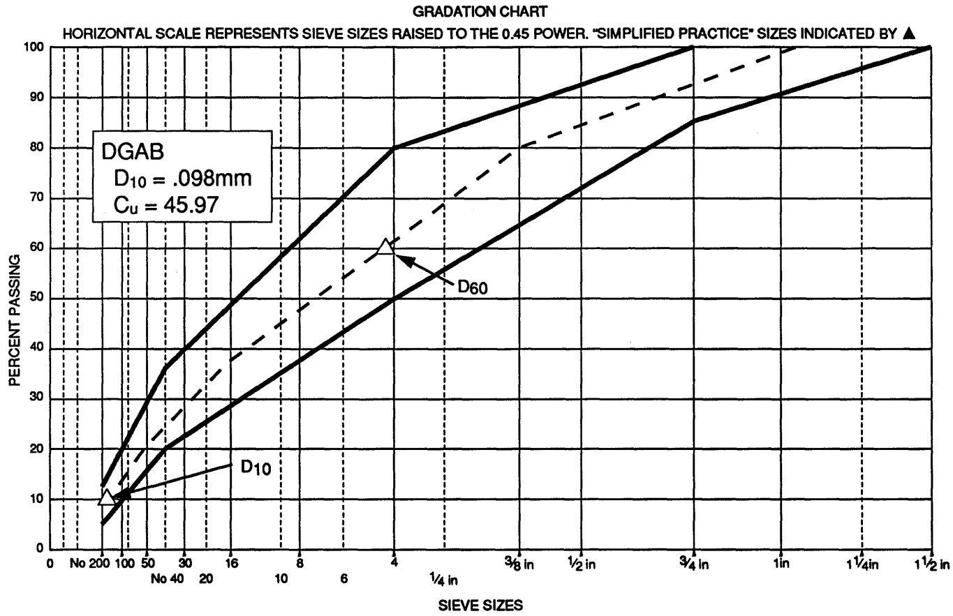
Figure 33. Plot of DGAB Gradation
