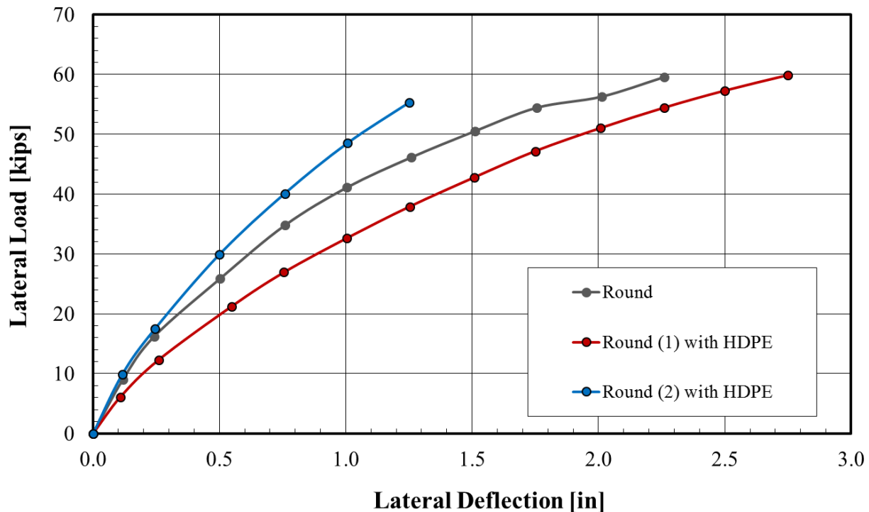
Figure 5-4: Load Test Results for Round Piles with HDPE Sheeting
