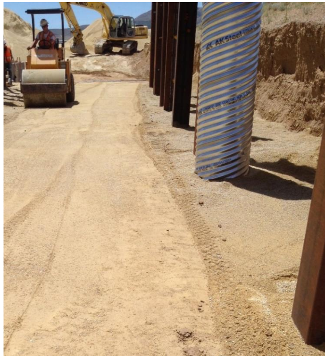
Figure 3-6: Phase 1 compaction
