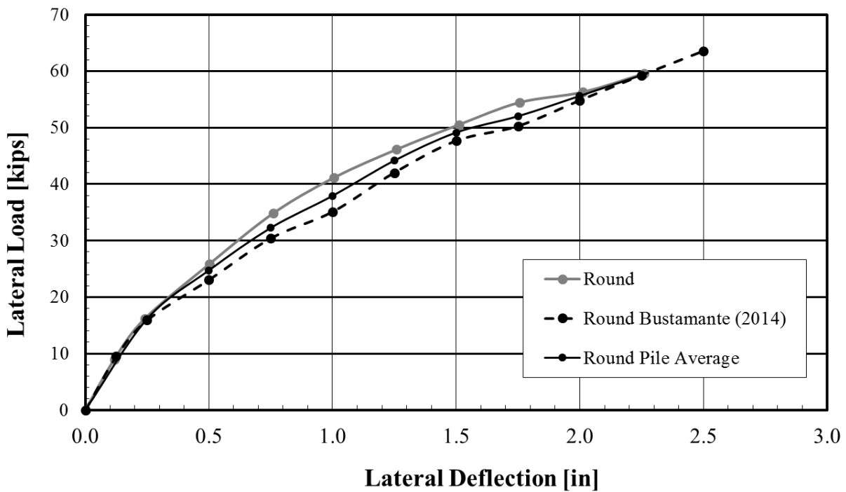
Figure 5-3: Lateral Load versus Deflection Curves for Round Piles
