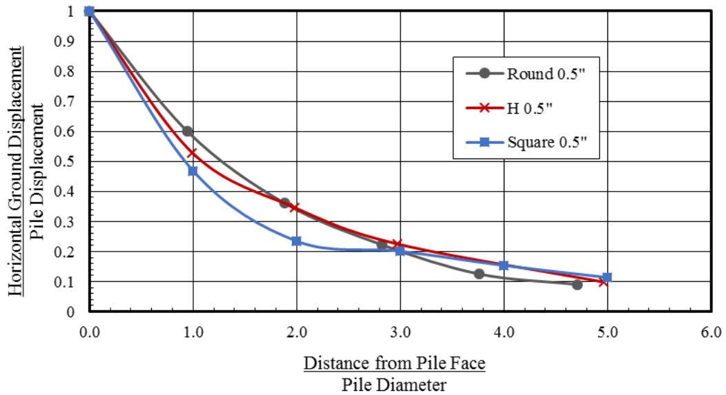
Figure 5-23: Normalized Deflection vs. Normalized Distance at 0.50" Equivalent Load
