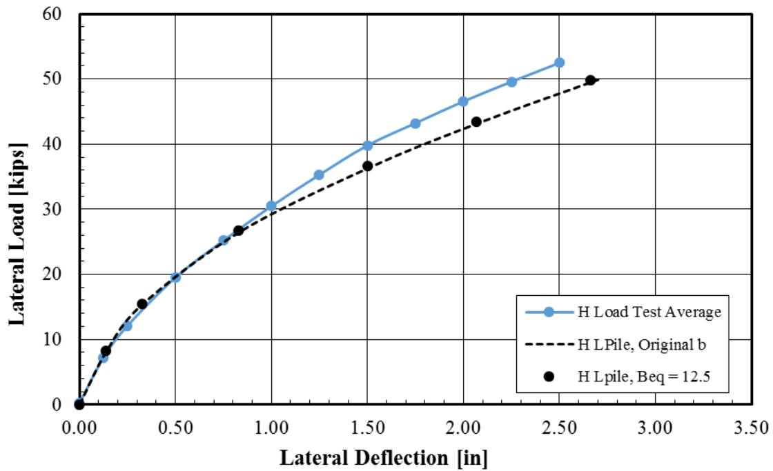
Figure 6-6: Load vs. Deflection Curve for Equivalent Diameter Approach for an H Pile
