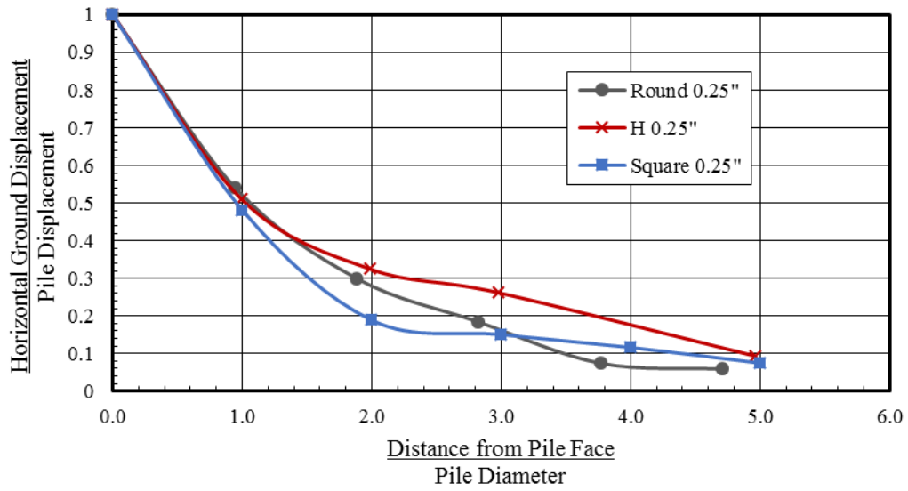
Figure 5-22: Normalized Deflection vs. Normalized Distance at 0.25" Equivalent Load
