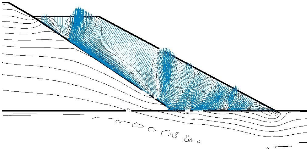
Figure 4-19 Convective Airflow Pattern in the Ventiladed Shoulder on January 1 for Case 4
