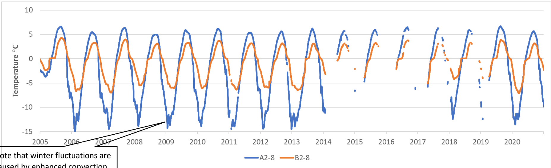
Figure 3-16 Temperature Time Series for Test Section #2 Below Horizontal ACE layer
