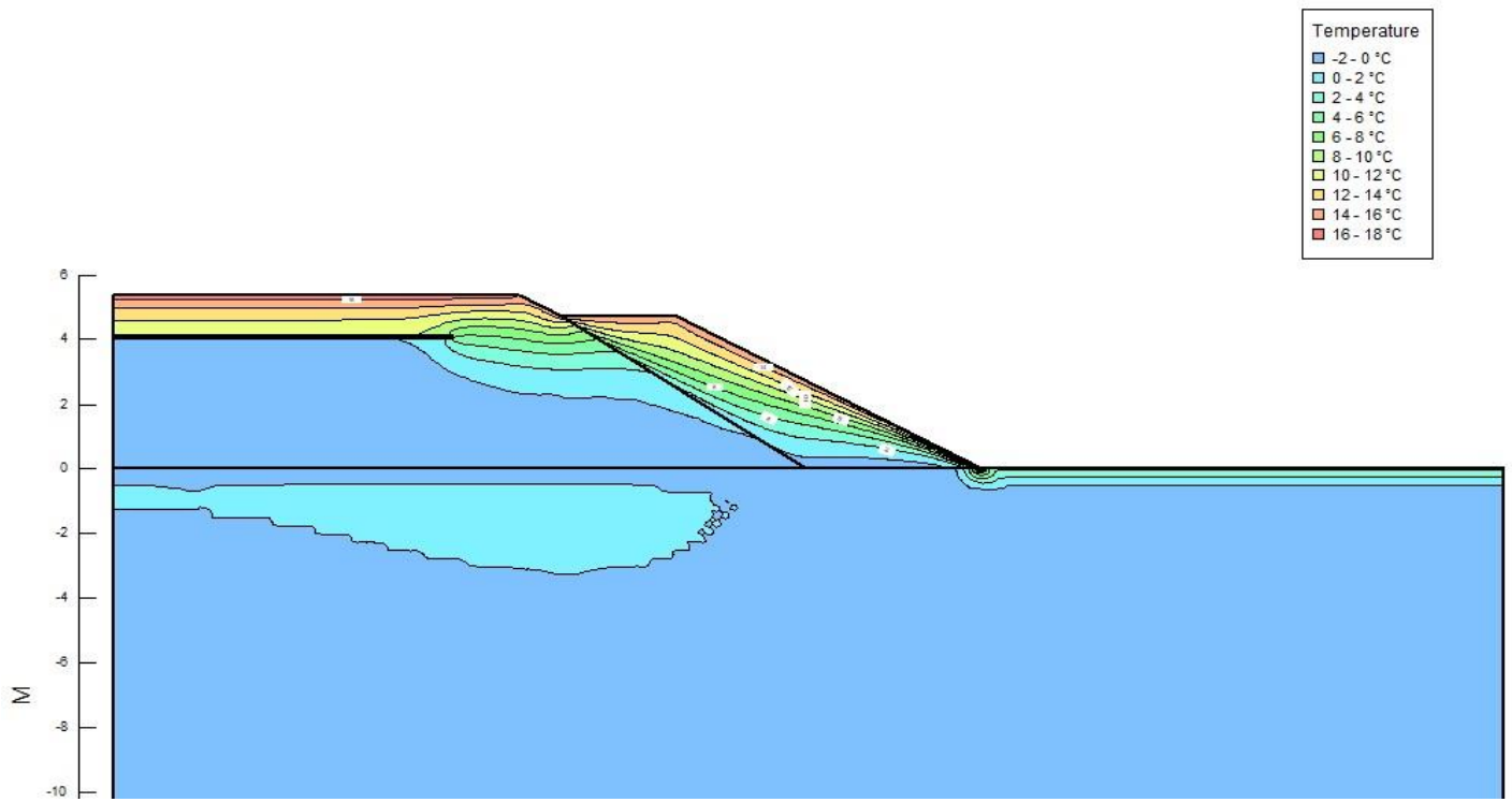
Figure 4-17 Simulation Results for Case 3 for May 15 of Year 12
