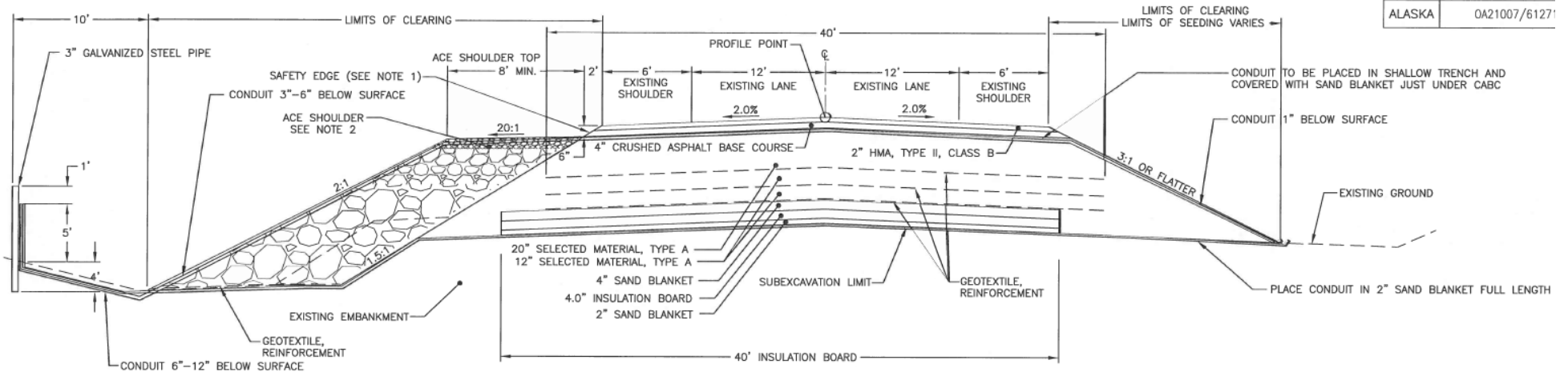
MODIFIED TYPICAL VI - HIGHWAY REHABILITATION STATIONS: 4125+00-4133+00
