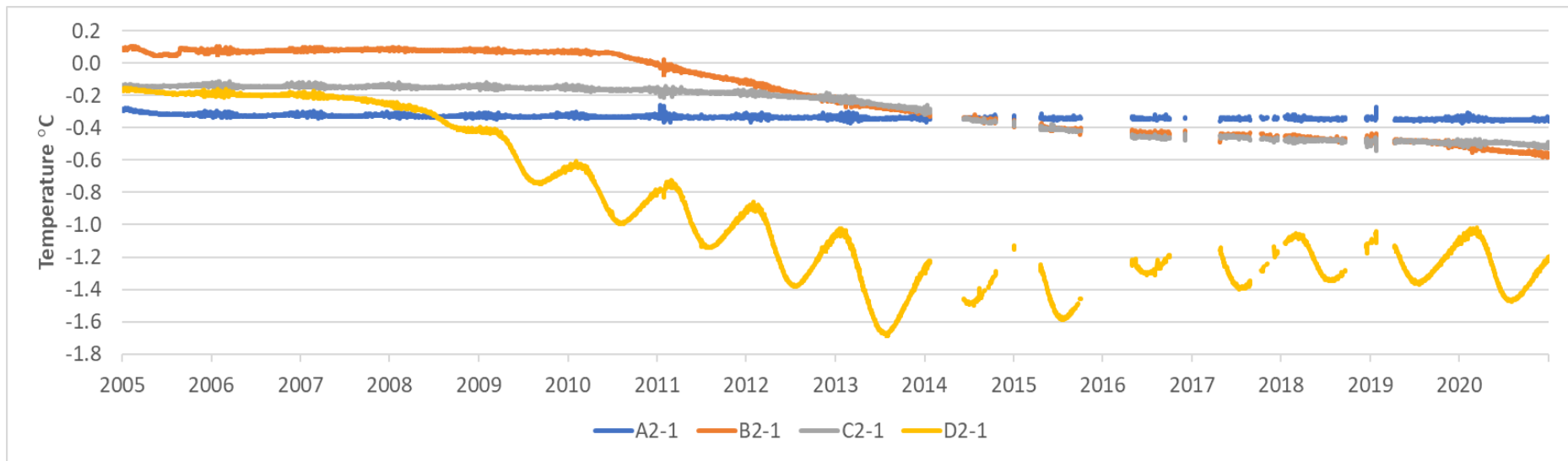
Figure 3-19 Temperature Time Series for Test Section #2 at 8 m Below Original Grade
