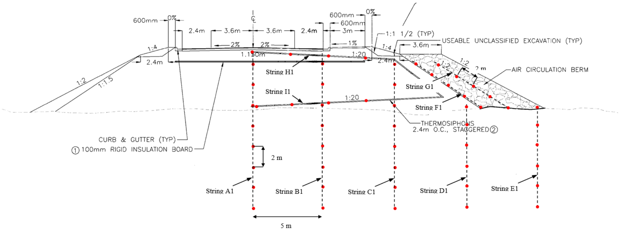
Figure 3-6 Instrumentation for test section #1 consisting of 9 thermistor strings with a total of 62 thermistor temperature sensors
