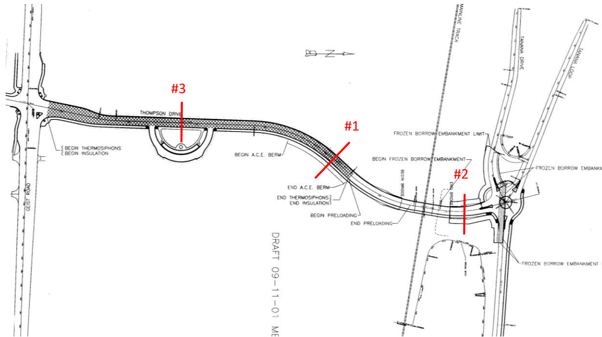
Figure 3-1 Thompson Drive test section locations
