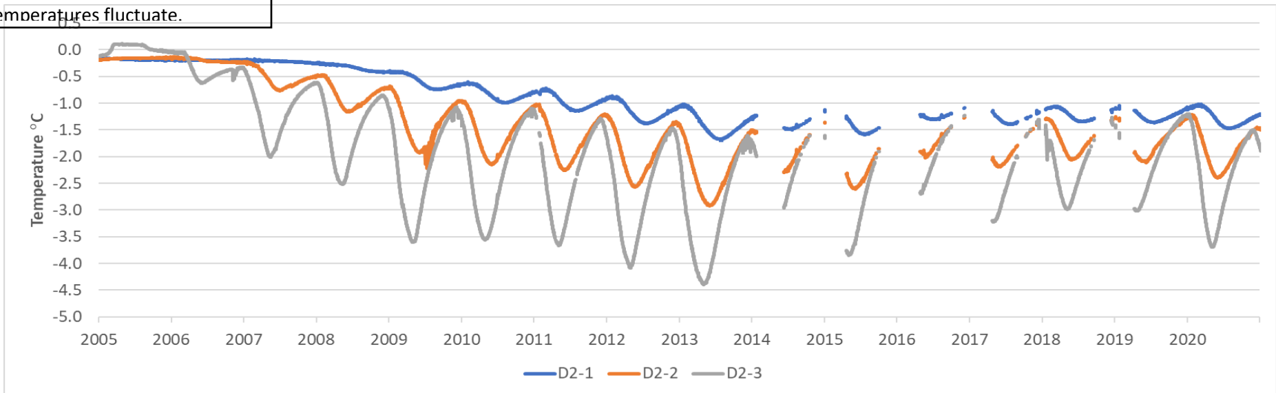
Figure 3-17 Temperature Time Series for Test Section #2 Below Ventilated Shoulder
