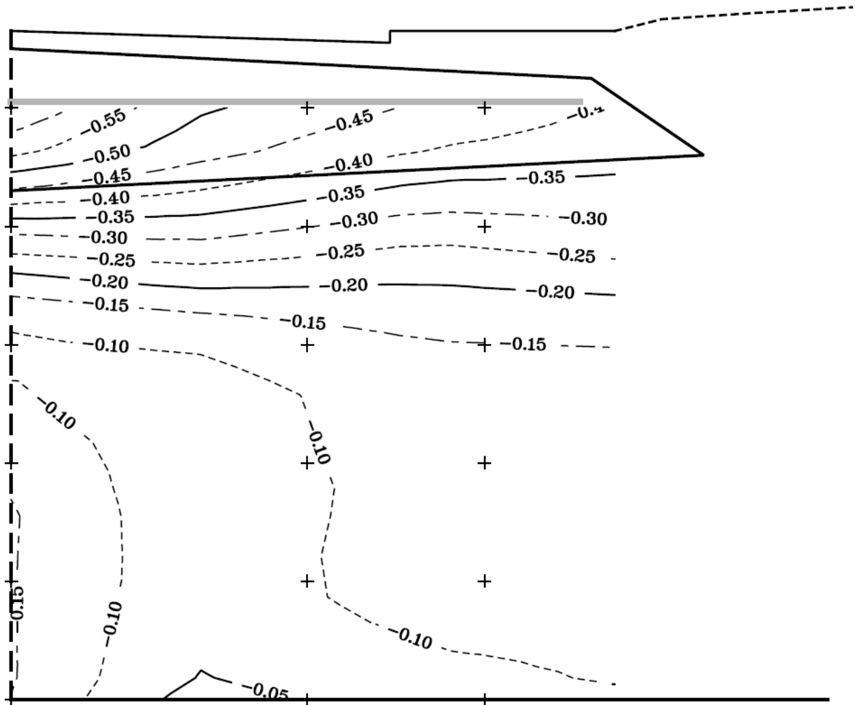
Figure C-8 Mean annual temperature contours for test section 3 in 2012
