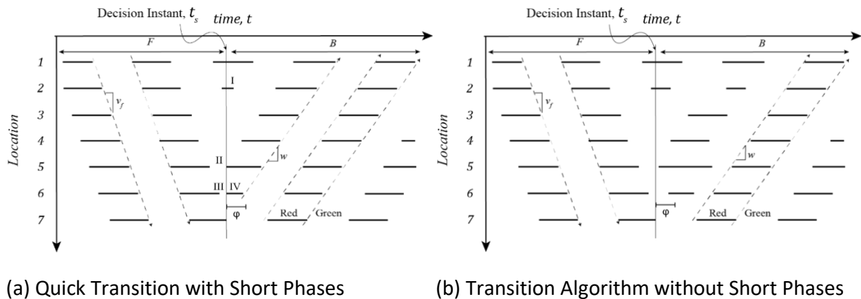
Figure. 2: Switching Between Coordination Strategies
