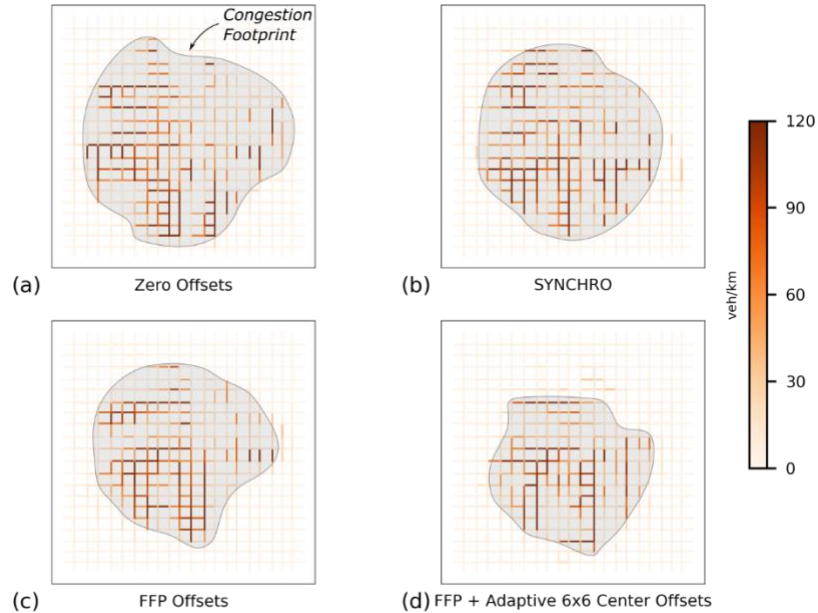
Figure. 6: Link Density Plots at t = 120 min: (a) Zero Offsets, (b) SYNCHRO, (c) FFP Offsets, (d) FFP + Adaptive 6x6 Center Offsets
