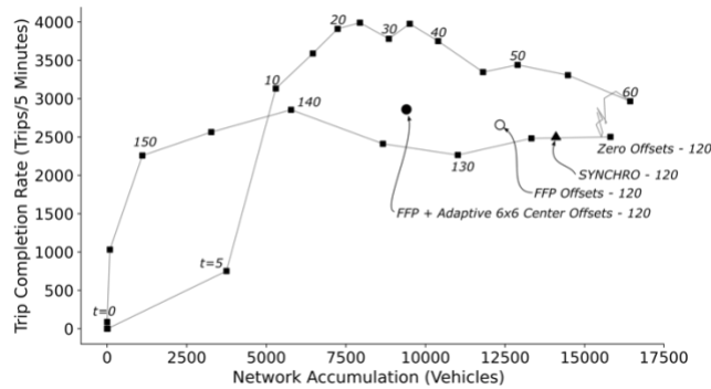
Figure. 5: Sample Path for Zero Offsets; and data points at 120 min for alternative strategies
