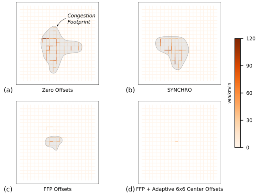
Figure. 7: Link Density Plots at t = 150 min: (a) Zero Offsets, (b) SYNCHRO, (c) FFP Offsets, (d) FFP + Adaptive 6x6 Center Offsets
