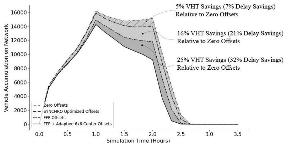
Figure. 8: Vehicle Accumulation on the Network for Different Coordination Strategies
