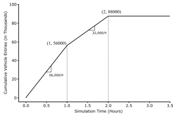
Figure. 4: Cumulative Vehicle Entries into the Network
