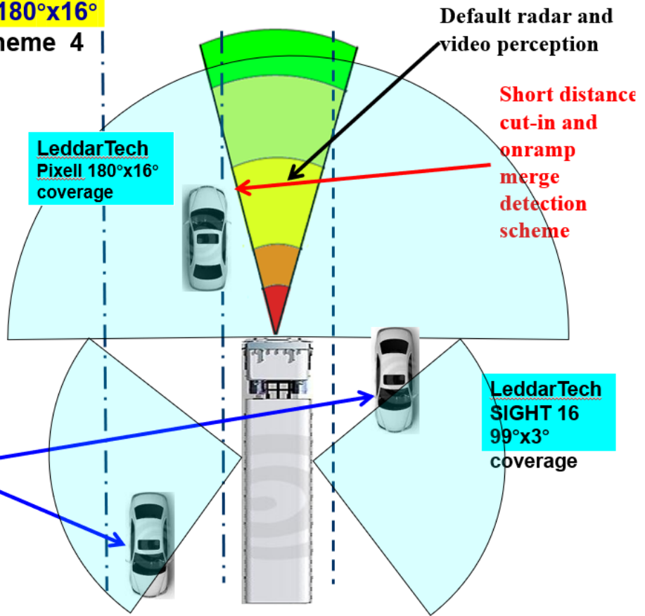
Figure 9. Three fixed beam lidar coverage scheme, mounted on the tractor only
