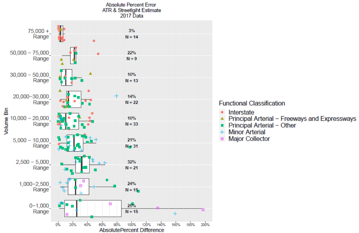
Figure 2.6: Absolute percent error comparing ODOT ATR AADT estimates and streetlight AADT
