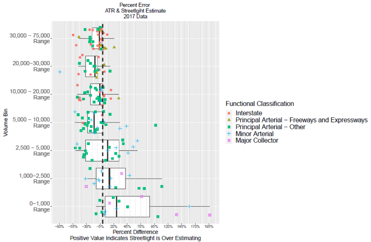
Figure 2.5: Percent error comparing ODOT ATR AADT estimates and streetlight AADT
