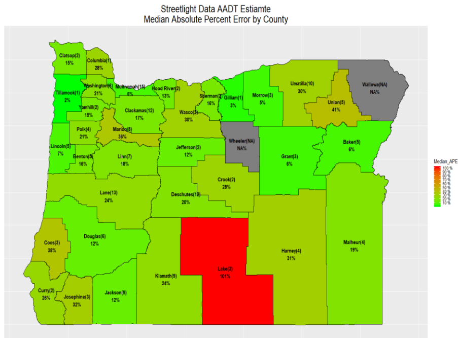
Figure 2.4: Median absolute percent error by county
