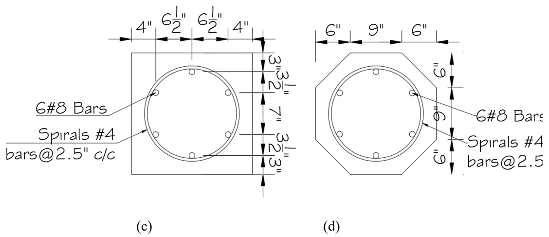
Figure 2.1 Column Details: (a) Test 1 column; (b) Test 2 column; (c) cross-section of column at B-B, and (d) cross-section of column at C-C
