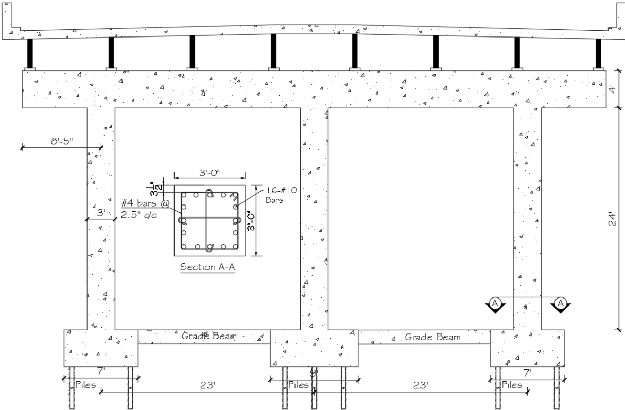
Figure 5.4 Three-column bridge bent with new seismic details
