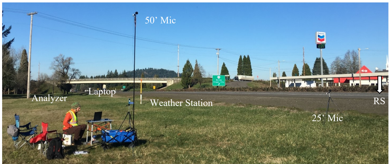
Figure 4.8: Exterior sound measurement setup
