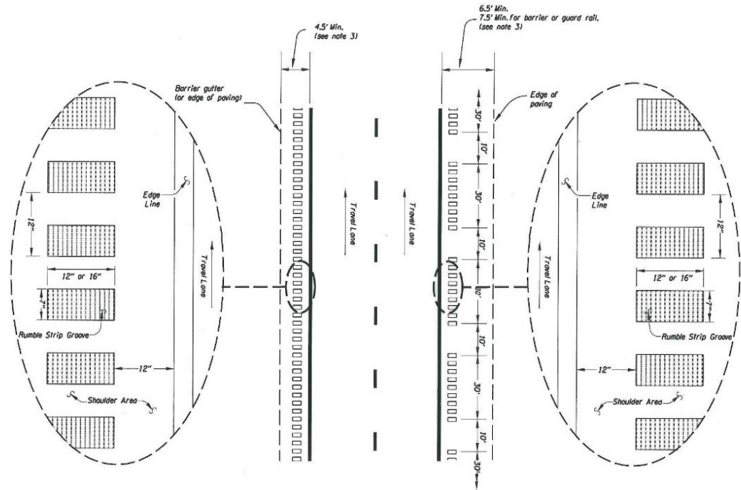
LEFT SHOULDER CONTINUOUS PATTERN
