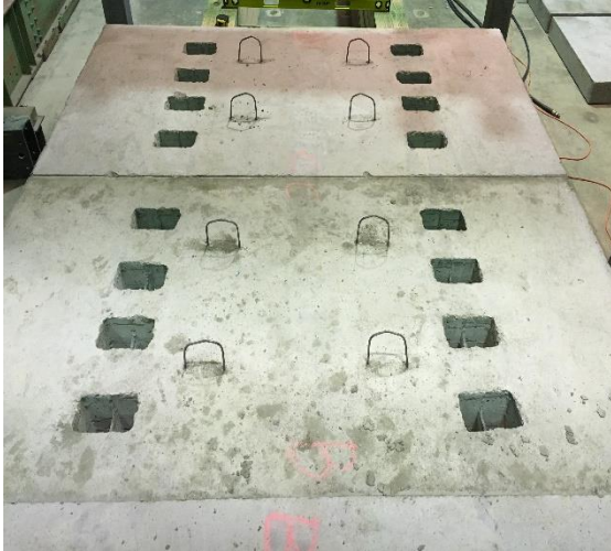
(a) Precast panels with grout pockets
