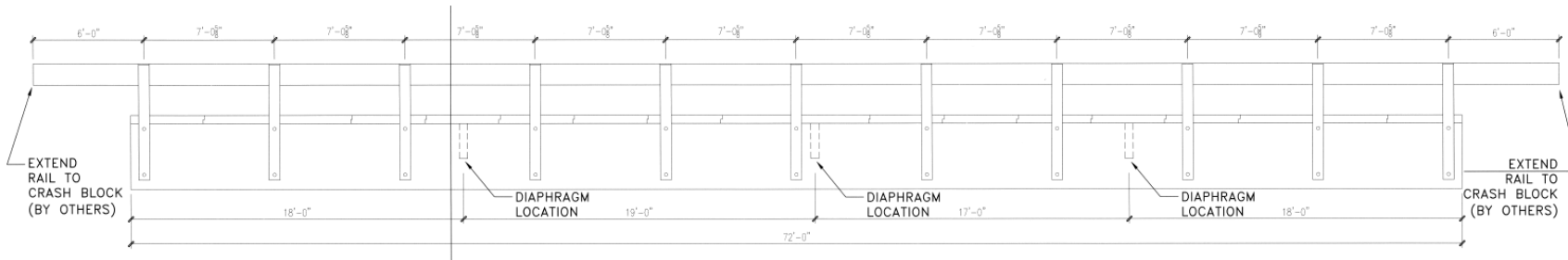
Figure 9. Elevation view of composite timber bridge, page 1/3 in Appendix A
