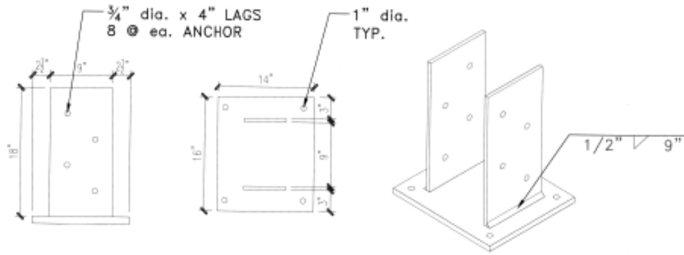
ANCHOR ASSEMBLY SCALE 1 1/2" = 1' - 0"
