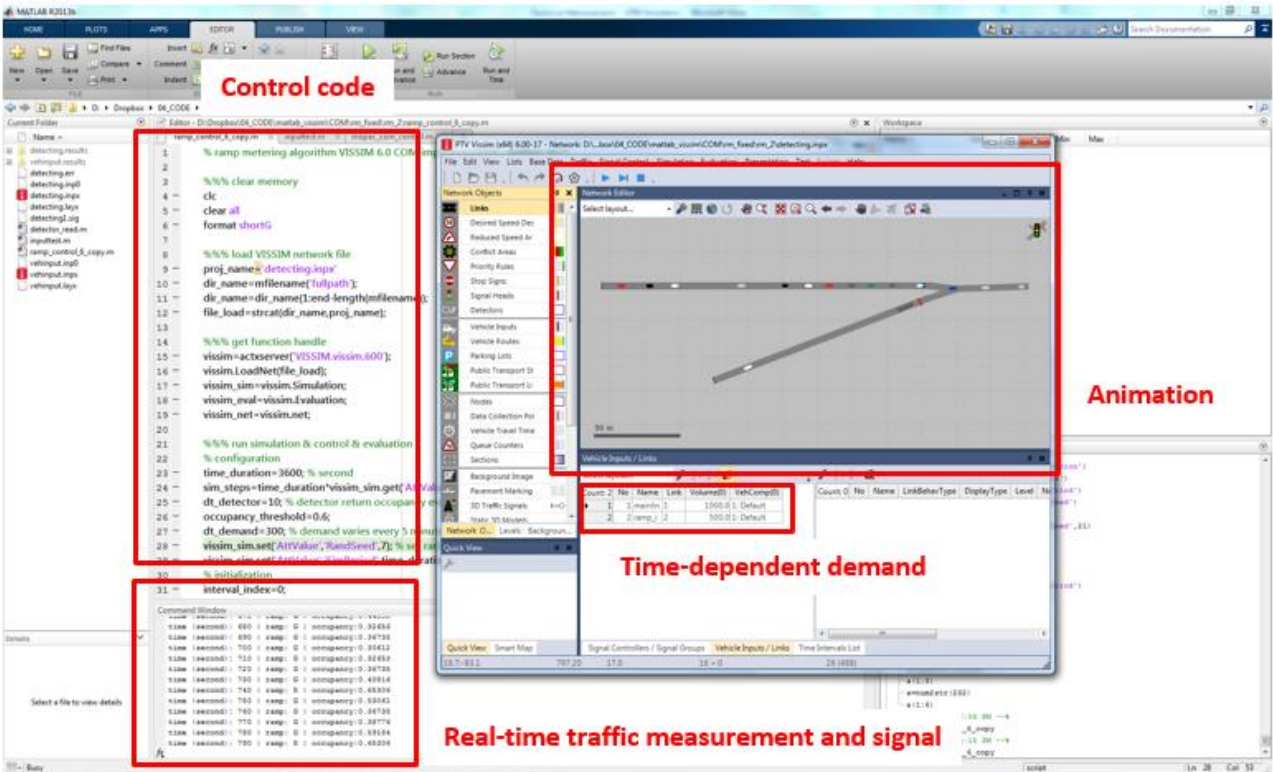
Figure 4.2 Example of graphical user interface of VISSIM-MATLAB integration
