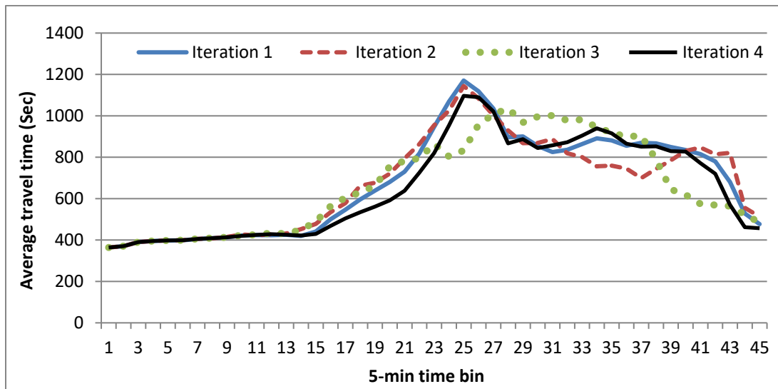
Figure 6.6 Average travel time in VISSIM for the HSR case
