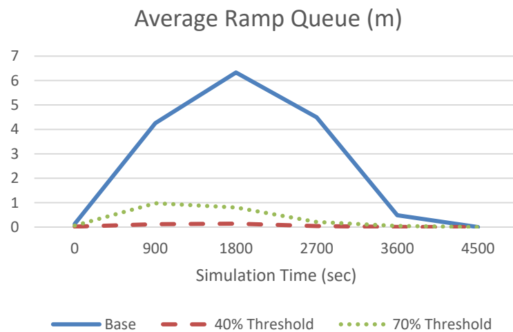
Figure 4.17 Average ramp queue length: ramp-based dynamic merge control
