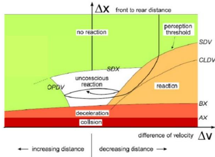
Figure 4.3 Car-following in Wiedemann's model
