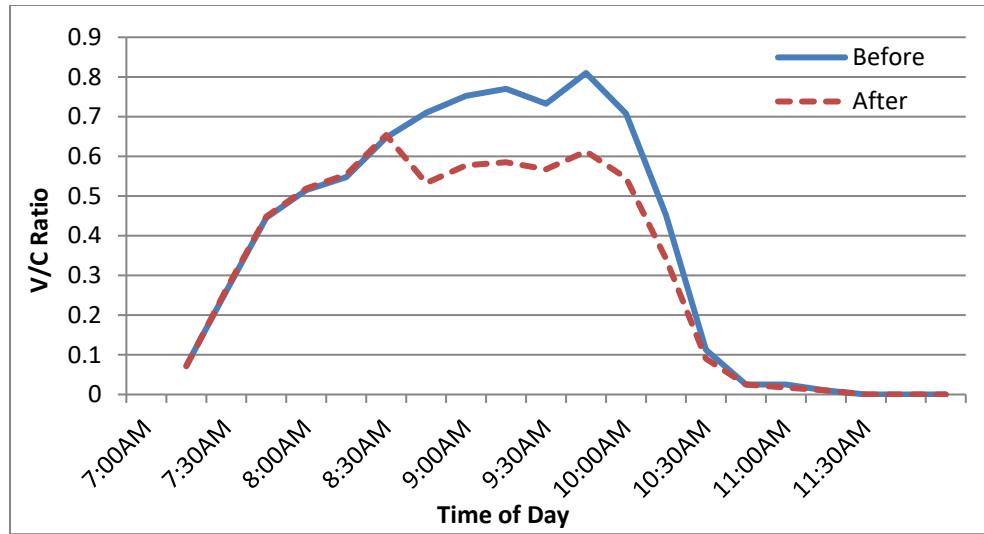
Figure 5.17 Change in volume-to-capacity ratio of the section after installing HSR
