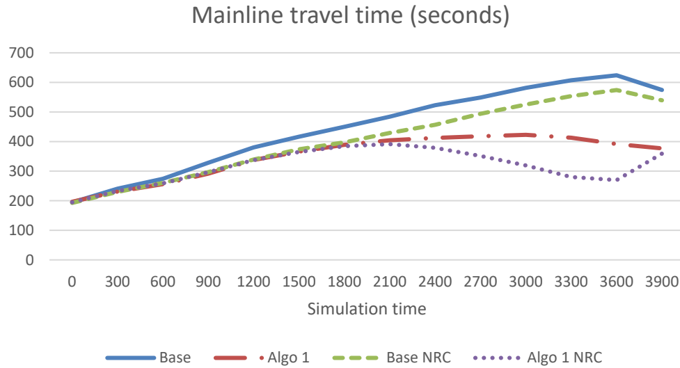
Figure 4.25 Mainline travel time: ramp metering non-recurring congestion
