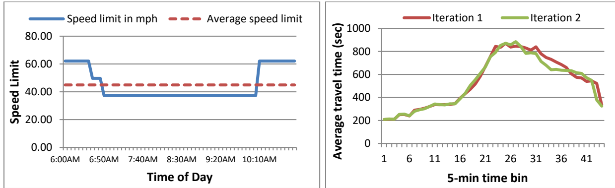
Figure 6.4 Speed limit variation and the travel time variation in VISSIM: (a) speed control output obtained from VISSIM, which is for the same for both iterations, (left) and (b) average travel time variation over the corridor (right)
