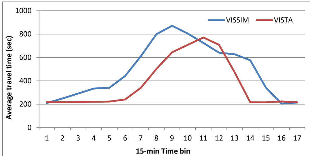
Figure 6.5 Main lane travel time in VISTA and VISSIM
