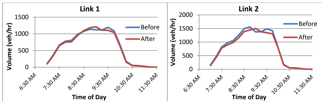
Figure 5.18 Time-dependent volumes on links with VSLs
