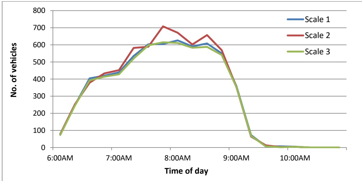
Figure 7.6 OD demand variation after ramp metering for each of the three scales
