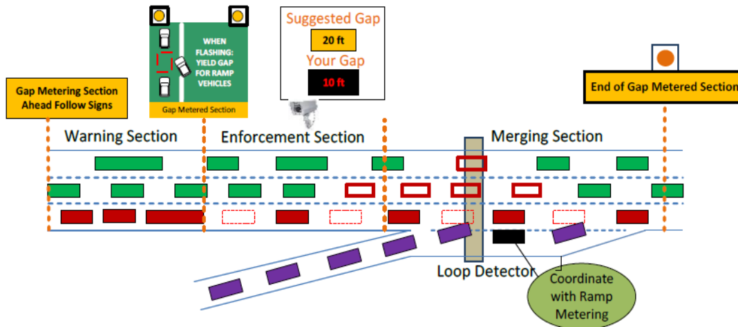
Figure 2.6 Gap metering design
