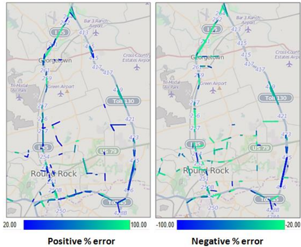
Figure 5.4 Percentage link errors after fine-tuning calibration
