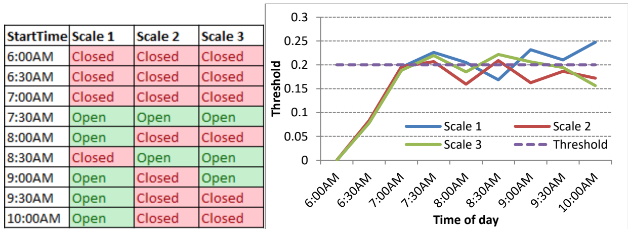
Figure 7.4 Control strategy output: (a) control strategy output obtained after convergence; (b) occupancy reading for the HSR control detector for each of the three scales
