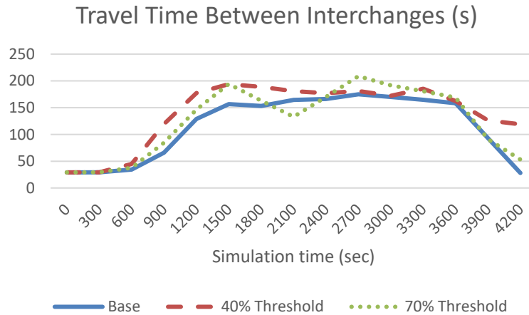
Figure 4.16 Mainline travel time measured between first two interchanges: ramp-based dynamic merge control
