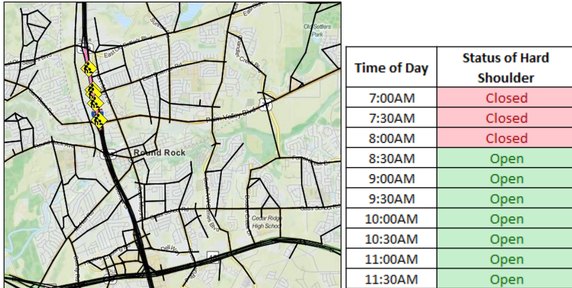
Figure 5.16 Selected segment for the analysis: (a) hard shoulder implementation location in VISTA modeled as lane closure; (b) output of the VISSIM implementation of HSR
