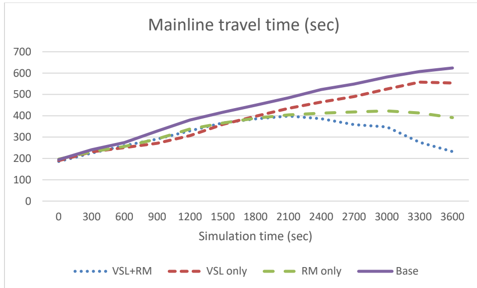
Figure 4.23 Mainline travel time with and without VSL+RM
