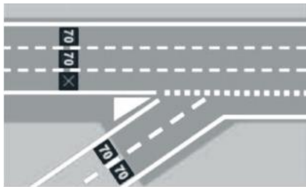
Figure 4.14 Dynamic lane use: ramp merge control (Jones, et al., 2011)
