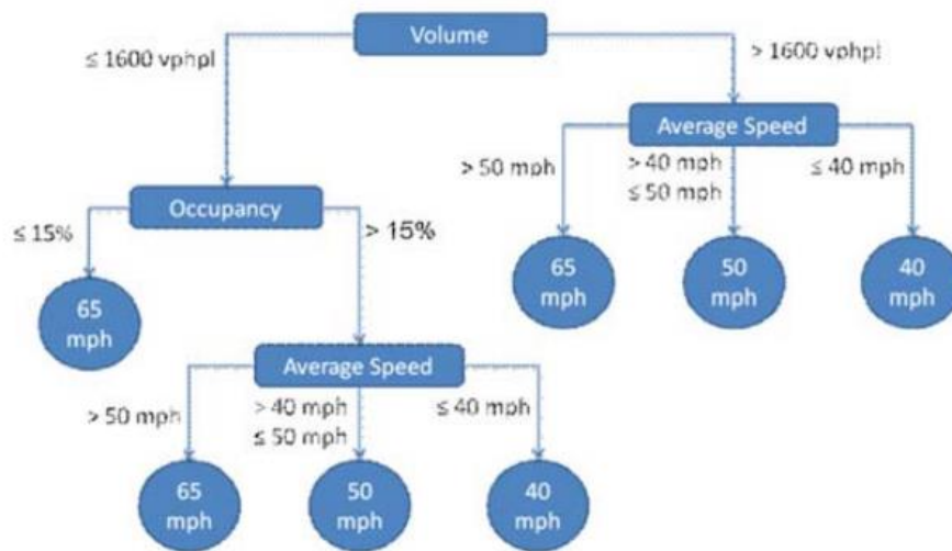
Figure 4.12 VSL control algorithm architecture (Allaby et al., 2007)
