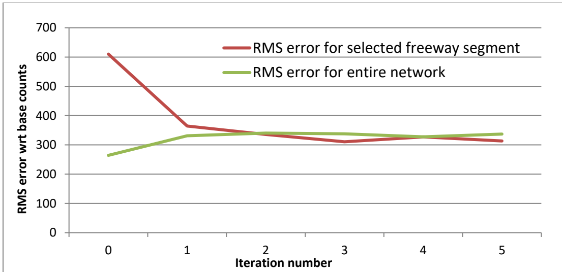
Figure 5.3 RMS error changes with fine-tuning calibration performed on the base network
