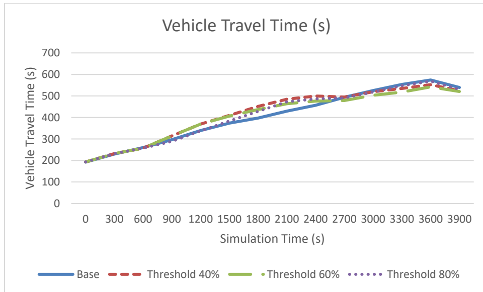
Figure 4.28 Mainline travel time: HSR with non-recurring congestion
