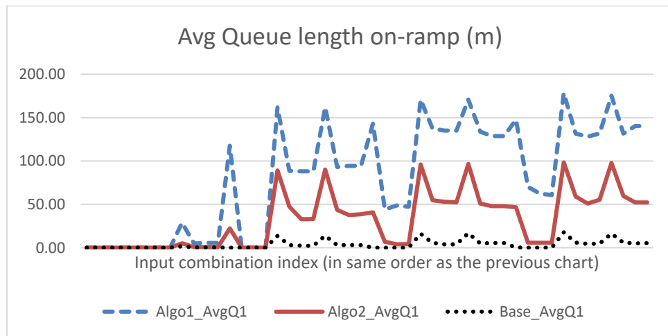
Figure 8.4 Average on-ramp queue length compared to base case for ramp metering algorithms
