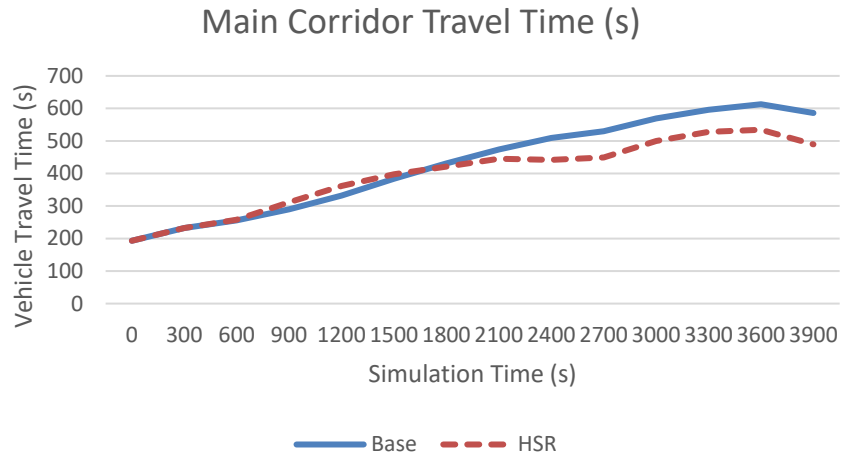
Figure 4.30 Mainline travel time: HSR non-recurring congestion increased duration
