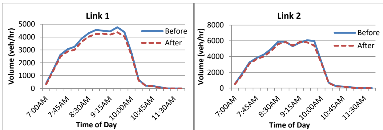
Figure 5.13 Changes in link volumes for the sections where VSL is installed
