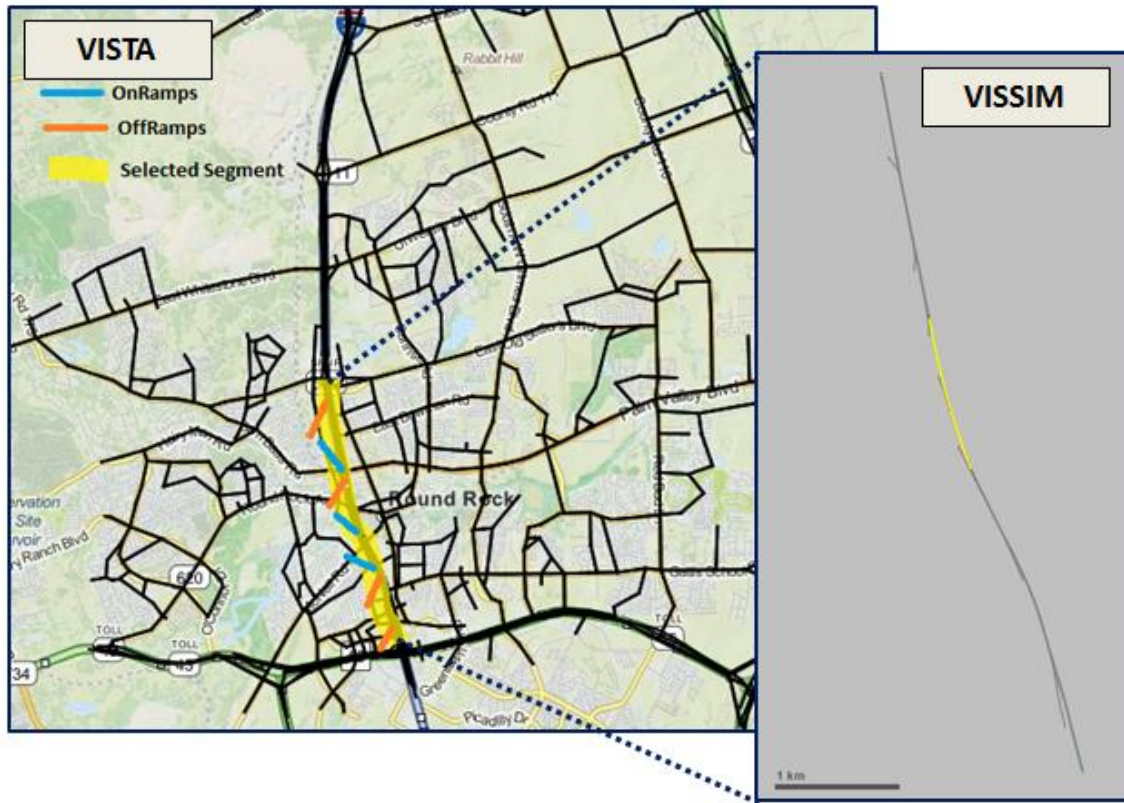
Figure 6.2 Multi-resolution network modeling in VISTA and VISSIM
