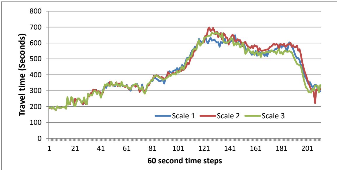
Figure 7.7 Average travel time (in sec) along the main lanes for each of the three scales
