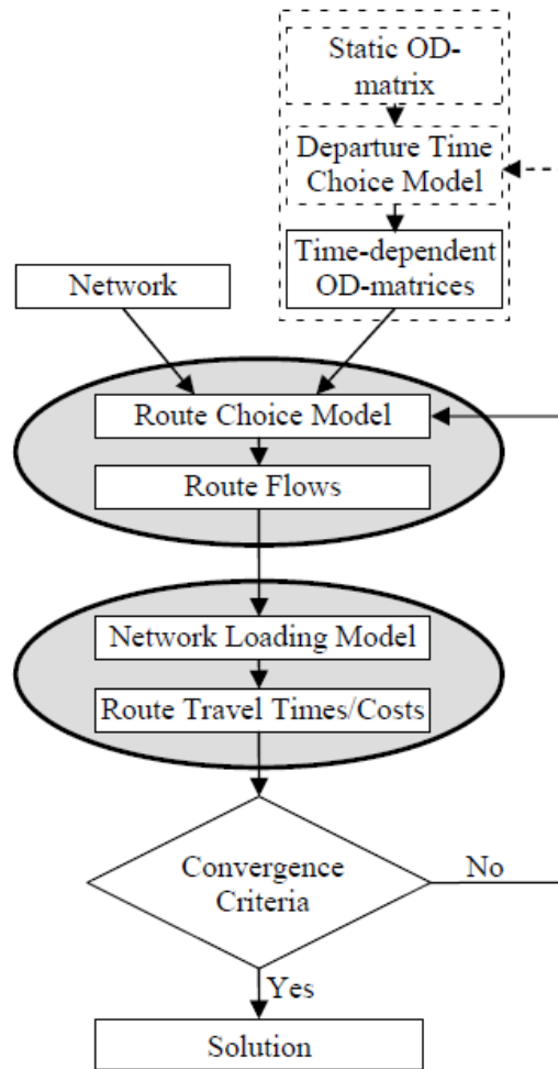
Figure 5.1 Overview of DTA procedure
