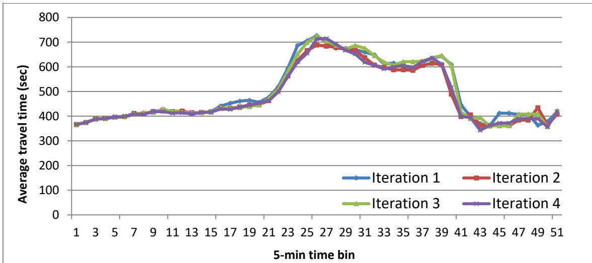
Figure 6.3 Average travel time on corridor in VISSIM
