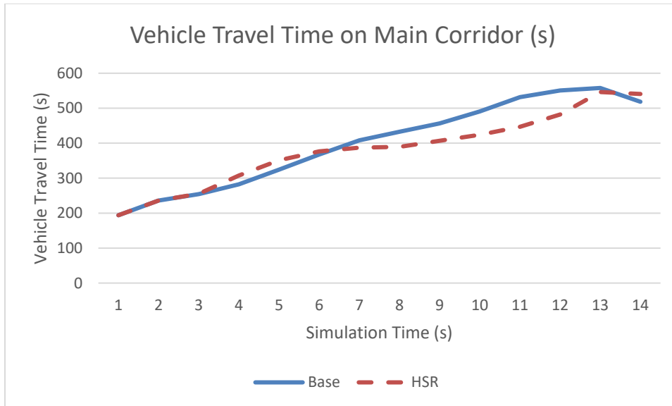
Figure 4.31 Mainline travel time: HSR non-recurring congestion, upstream bottleneck
