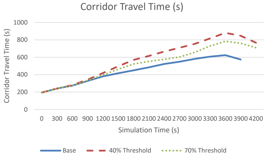
Figure 4.15 Mainline travel time: ramp-based dynamic merge control
