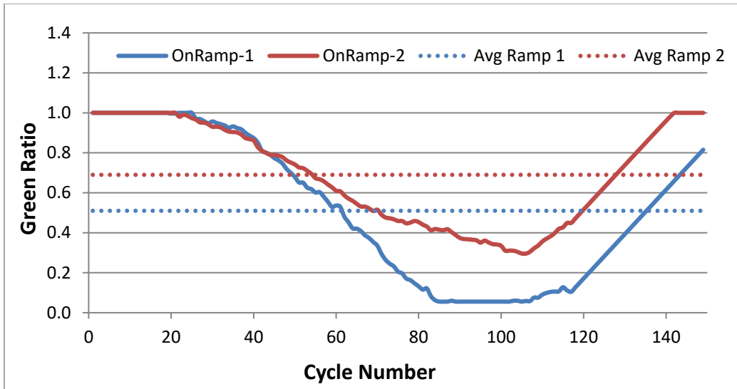
Figure 5.7 Variation of green ratios observed in VISSIM and the average value used in VISTA
