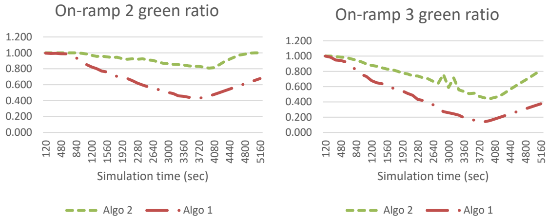
Figure 4.11 Plot of the green ratio on the on-ramps: ramp metering
