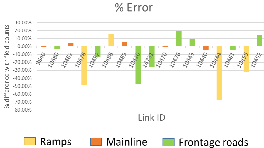
Figure 4.6 Plot of calibration errors in link flows for selected link IDs
