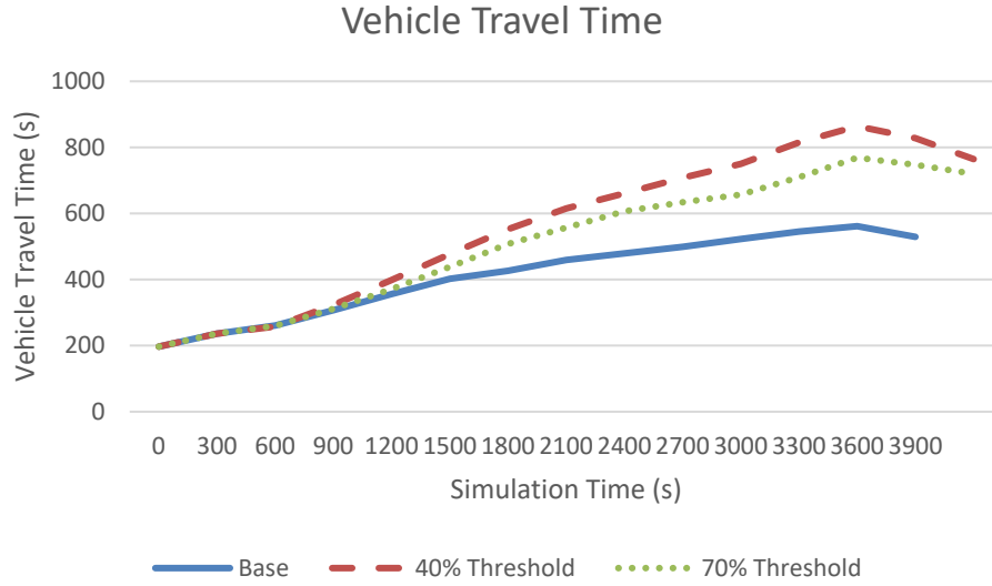
Figure 4.27 Mainline travel time: DLUC near ramp merge with non-recurring congestion
