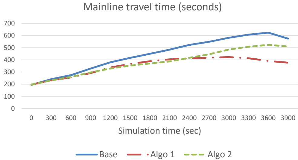
Figure 4.9 Plot of mainline travel time: ramp metering
