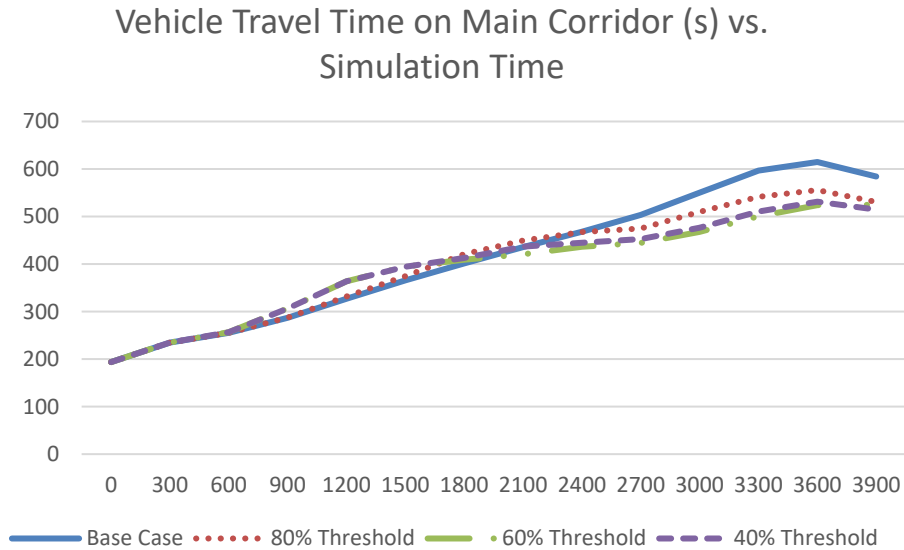
Figure 4.19 Mainline travel time: HSR
