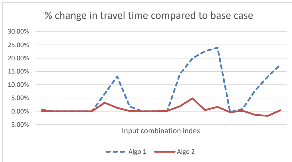
Figure 8.5 Percent change in corridor travel time compared to base case for VSL algorithms
