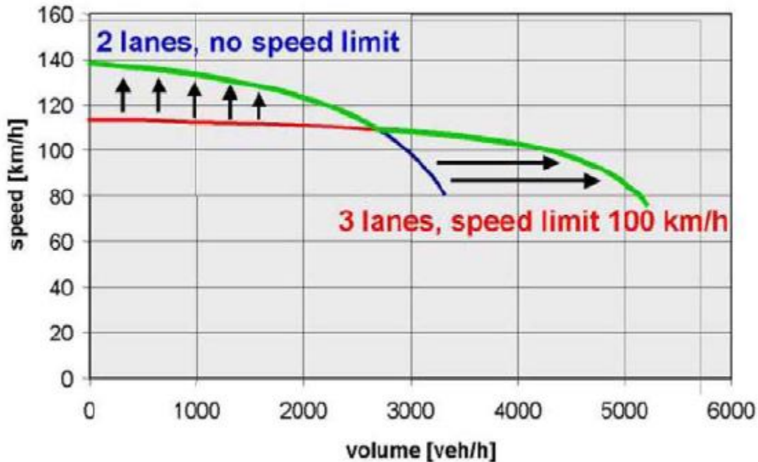
Figure 2.3 Increased throughput for temporary shoulder use in Germany (Mirshahi et al., 2007)
