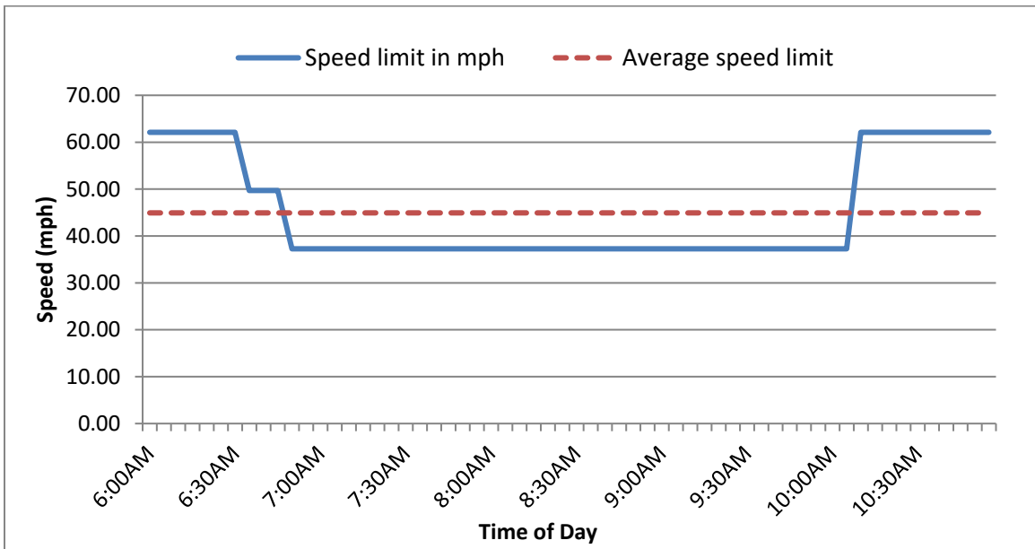
(b) Speed Limit variation as observed in VISSIM and the approximation average used in VISTA
