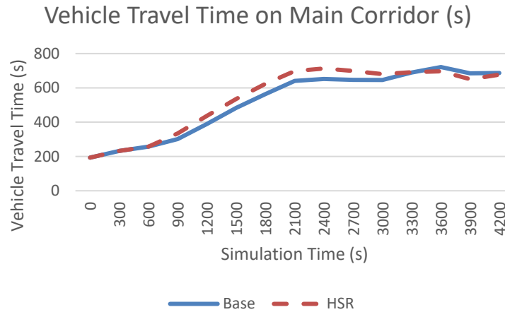
Figure 4.29 Mainline travel time: HSR non-recurring congestion with increased severity
