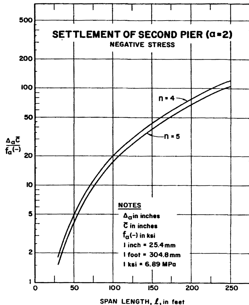
Figure 31. Design aid for determining the maximum negative stress increase caused by differential settlement of the second interior support.
