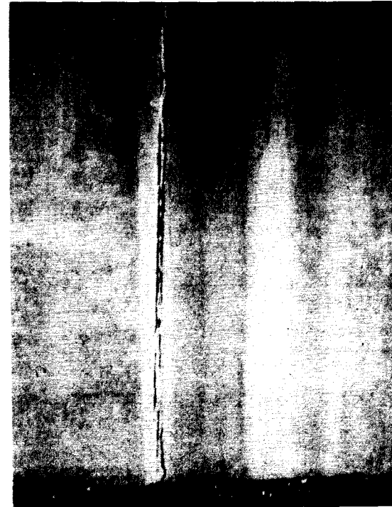
Figure 6. Opening of construction joint in abutment as result of differential settlement.
