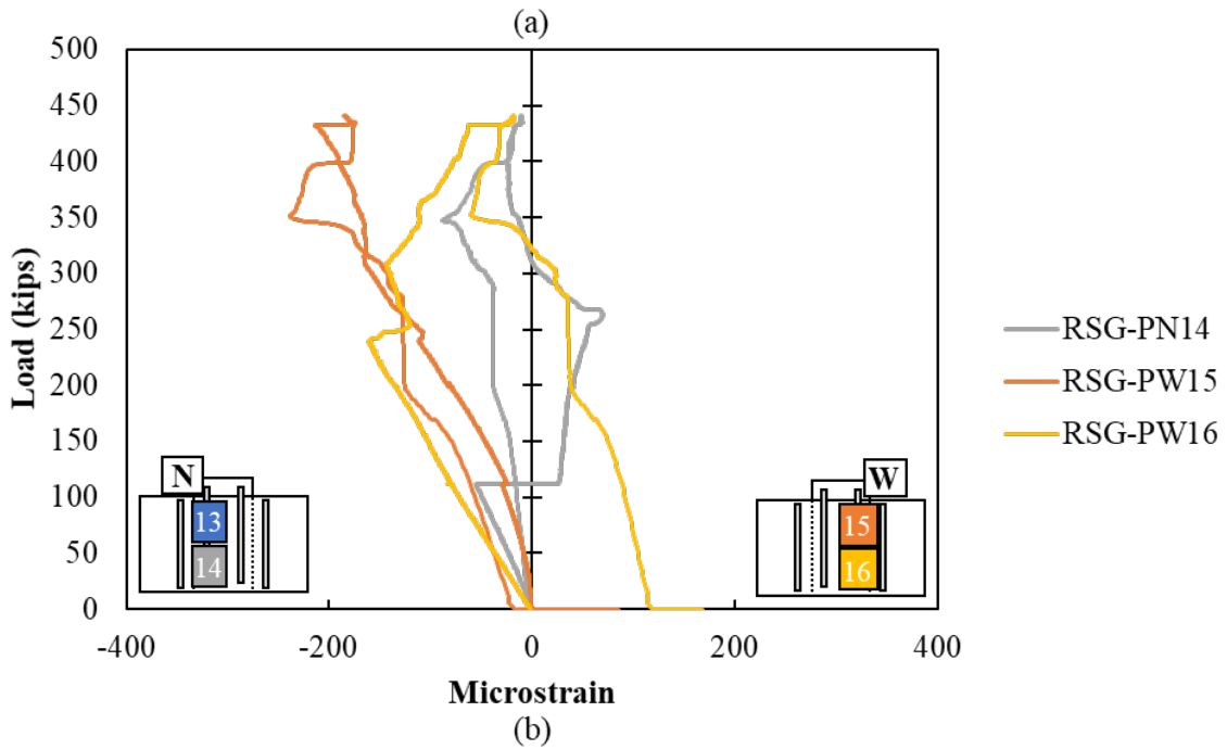
Figure A.158: Rebar strain gauges in vertical reinforcement on (a) cap and (b) plug of Specimen S3-3
