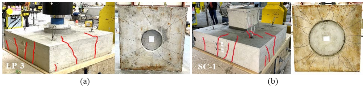
Figure 4.40: Crack patterns at failure for LP and SC specimens with corrugated interface (a) LP-3 and (b) SC-1
