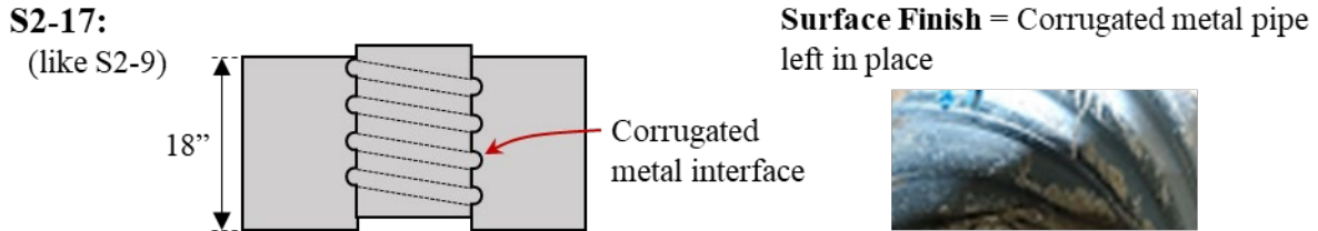
Figure A.123: Details for S2-17
