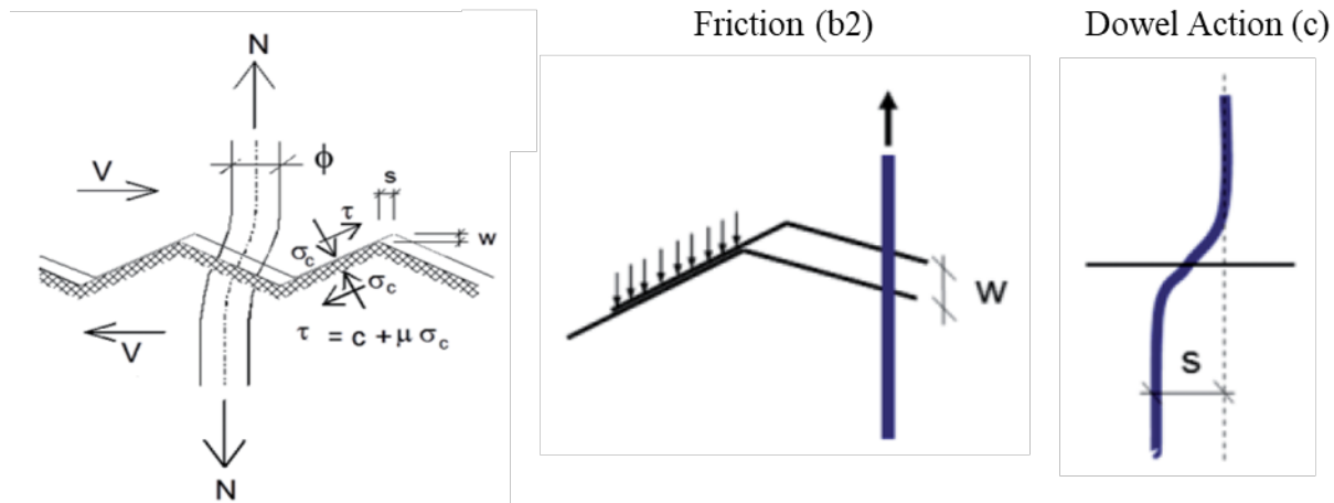
Figure 2.18: Shear resistance mechanisms when reinforcement is crossing interface [10]
