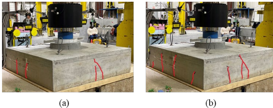
Figure B.10: Crack progression during testing at (a) 200 kips and (b) 300 kips
