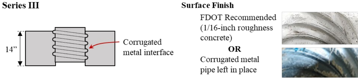
Figure A.139: Details for Series III specimens
