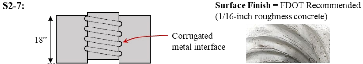
Figure A.62: Details for S2-7
