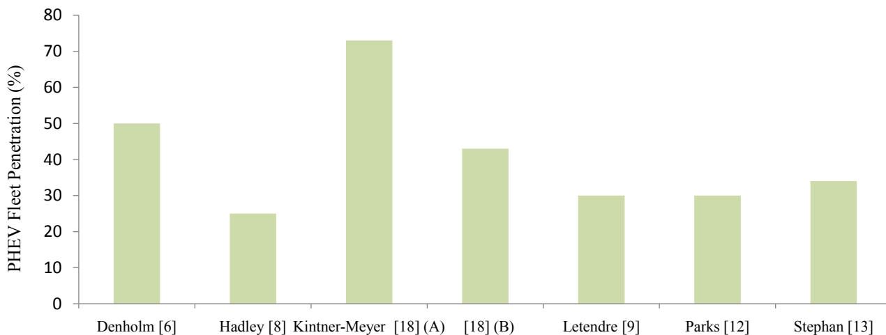
Figure 1-3. Currently supportable PHEV fleet penetration assuming optimal charging patterns. [18] (A) assumed optimized day and night charging. [18] (B) assumed optimized night charging only.
