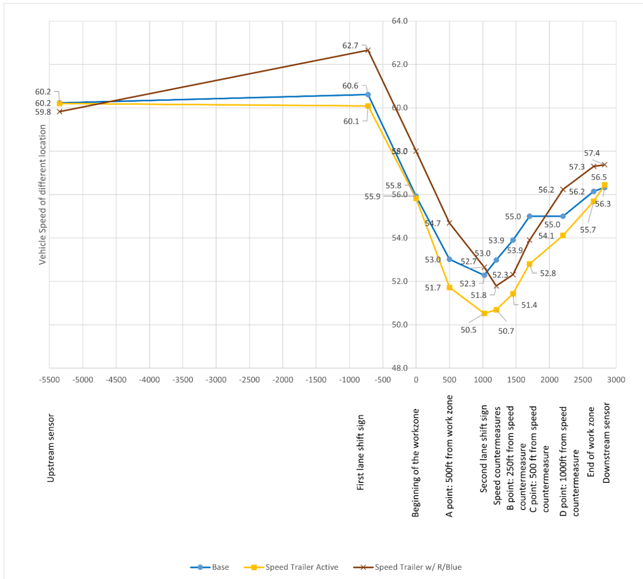
Figure 4-18. Speed profiles for speed trailer related countermeasures during nighttime
