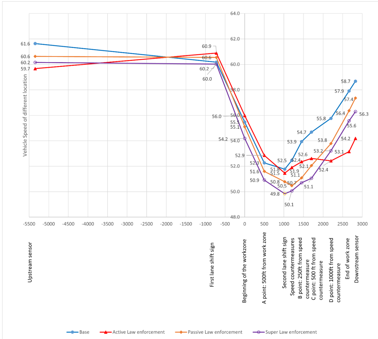
Figure 4-16. Speed profiles for law enforcement during daytime
