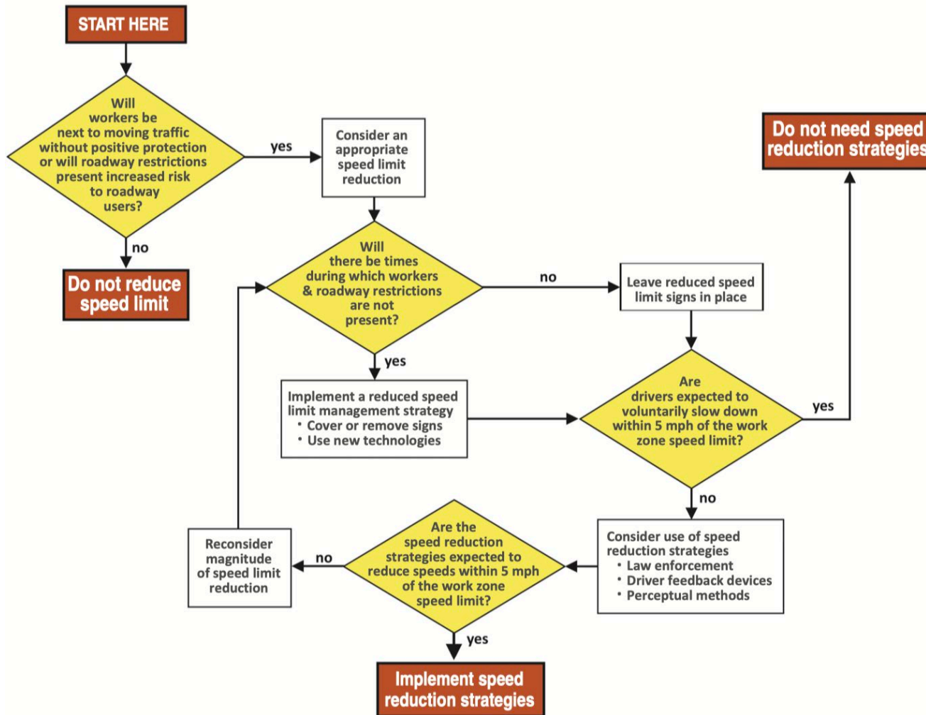
Figure B-1. Decision tree for implementation of work zone speed countermeasures
