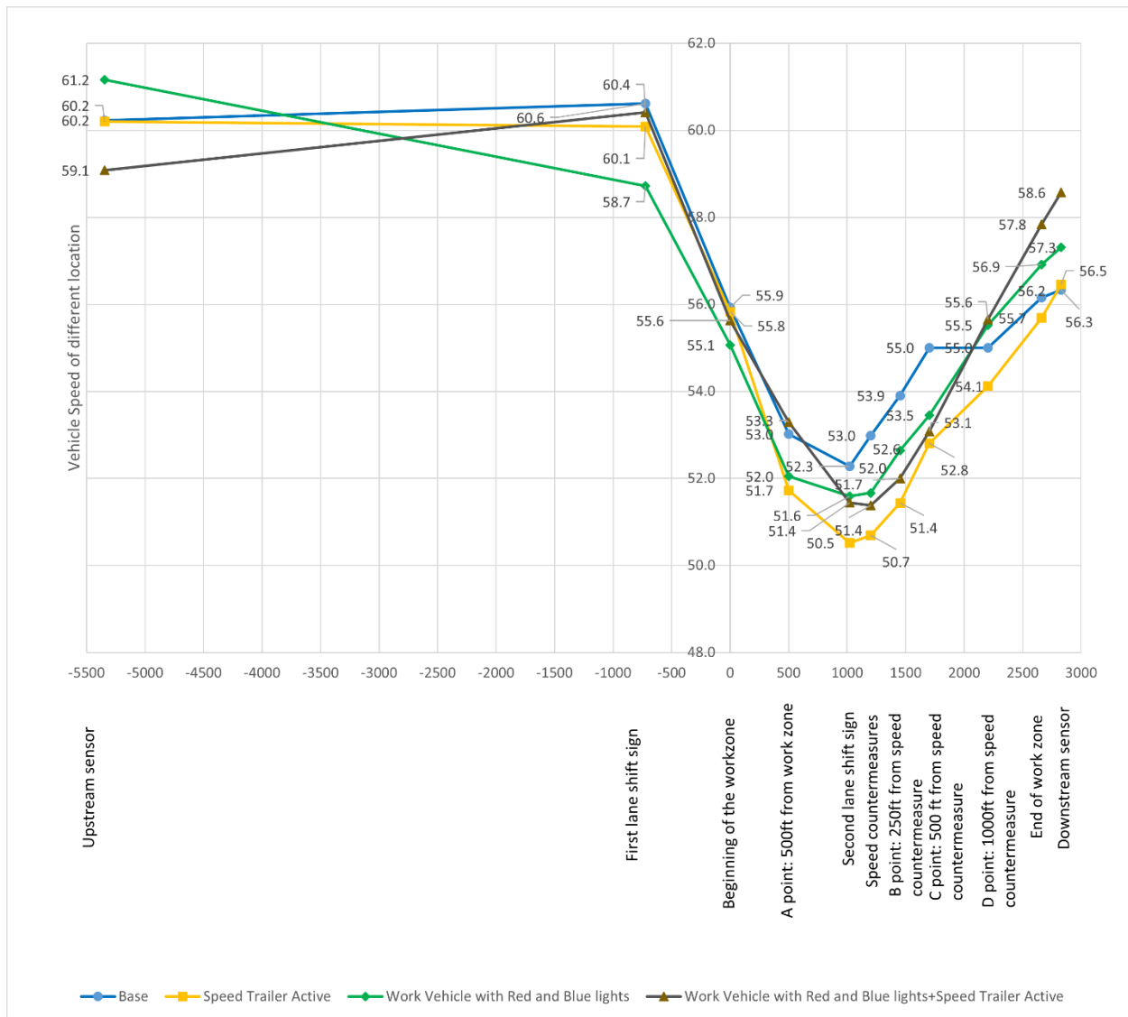
Figure 4-19. Speed profiles for work vehicle with red and blue lights and speed trailer active during nighttime
