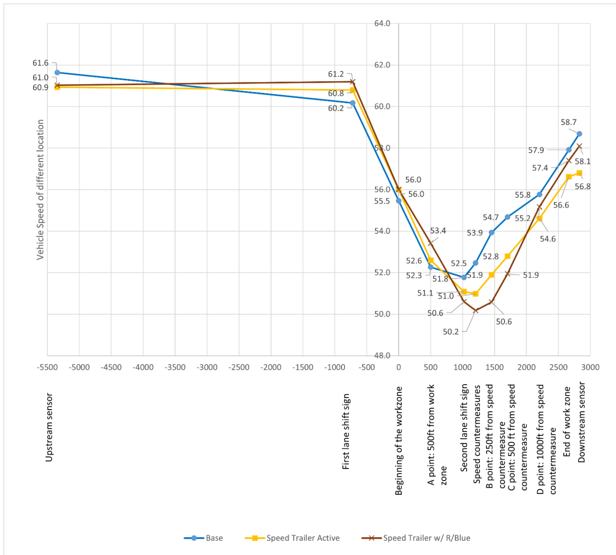
Figure 4-15. Speed profiles for speed trailers during daytime
