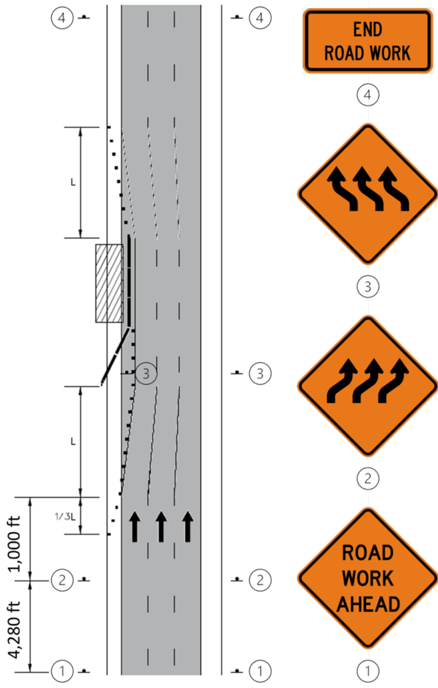
Figure 4-2. Work zone plan for driving simulator study
