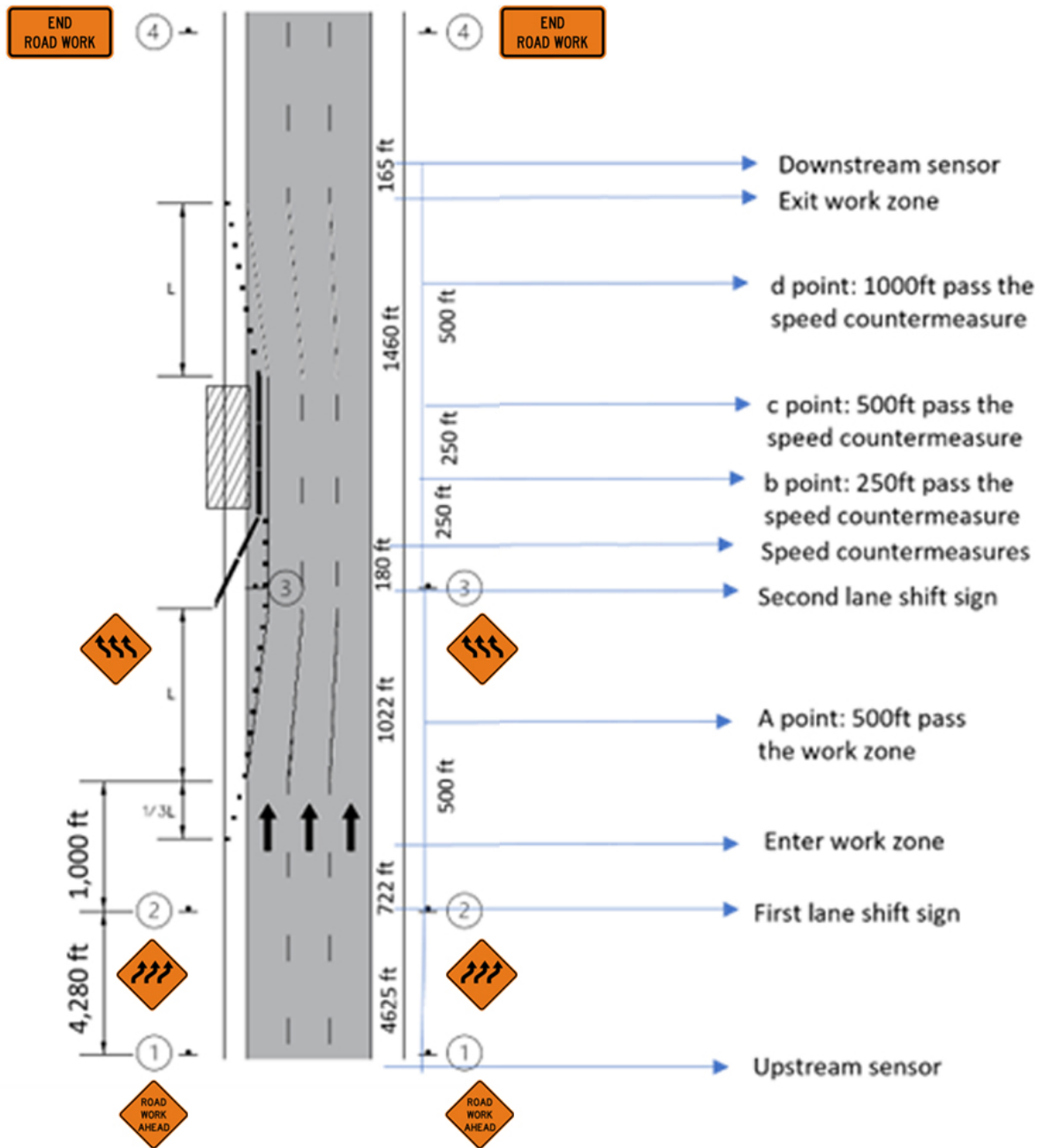
Figure 4-14. Diagram of unity.log location of collecting speed in simulator study
