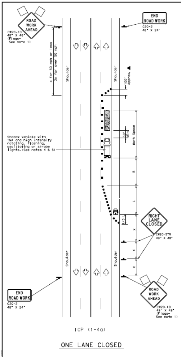
Figure 10. TxDOT TCP (1-4)-18 for Lane Closures on Multilane Conventional Roads (84).
