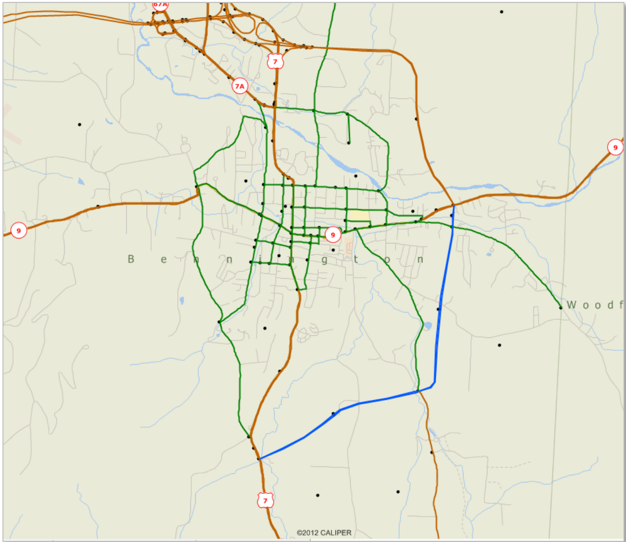
Figure 18 Roads that are not part of the state-maintained network (in green) are bypassed by the new project (in blue)
