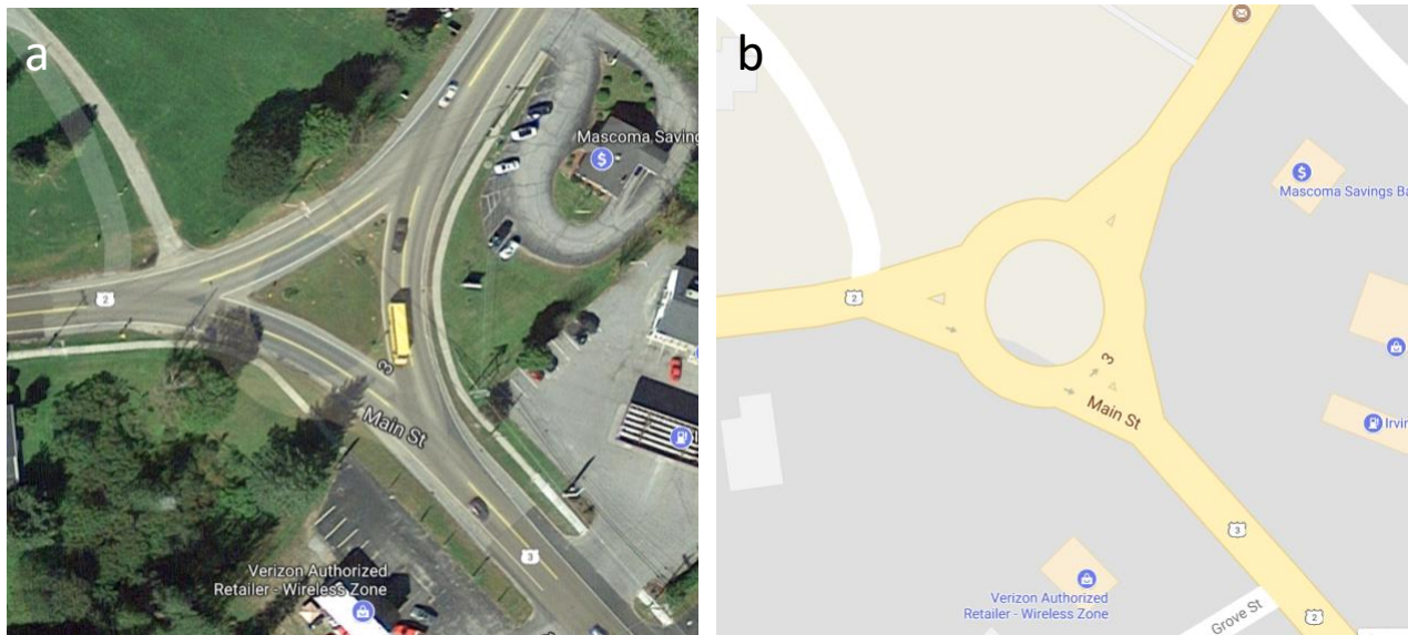
Figure 8 The intersection of US 2 and US 3 in Lancaster, New Hampshire as a stop- and yield-controlled intersection (a) and as a roundabout (b)
