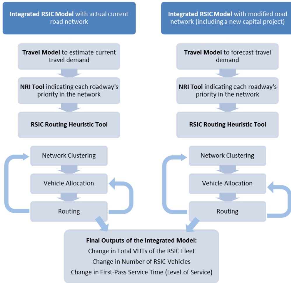
Figure 12 Integrated RSIC Model capital project evaluation flowchart
