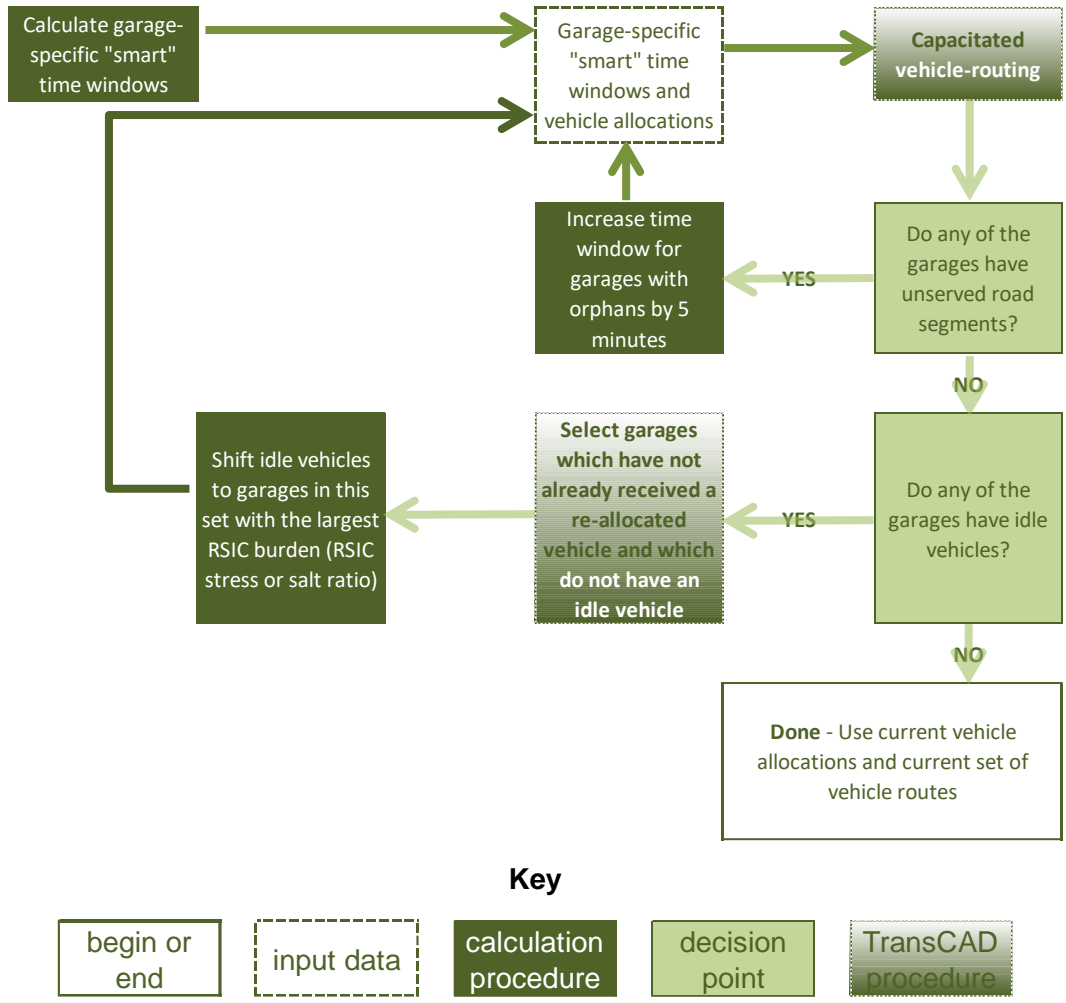
Figure 3 Iterative Procedure for RSIC Allocation & Routing
