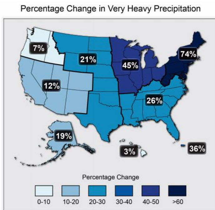
Figure 1 Percentage Change in Very Heavy Precipitation (from the Third National Climate Assessment Report, 2014)
