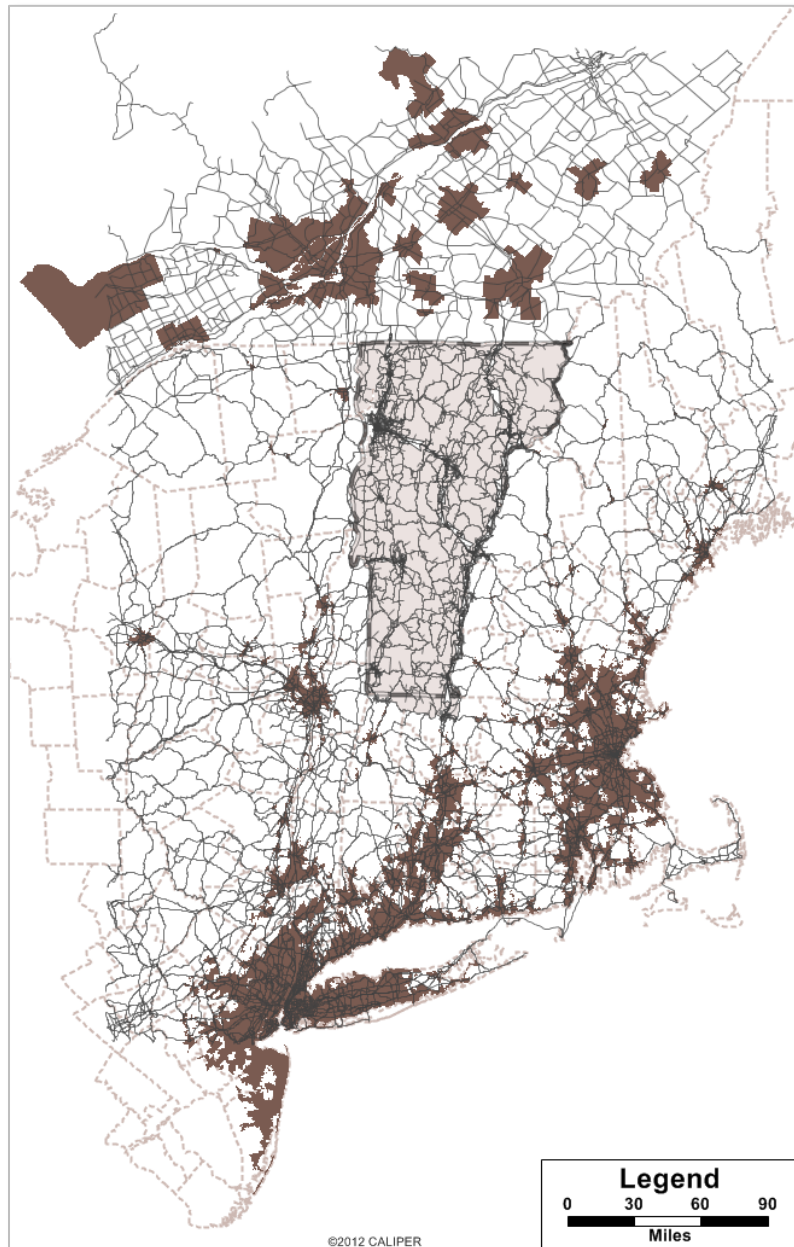
Figure 2 Zones and Road Network in the Vermont Travel Model
