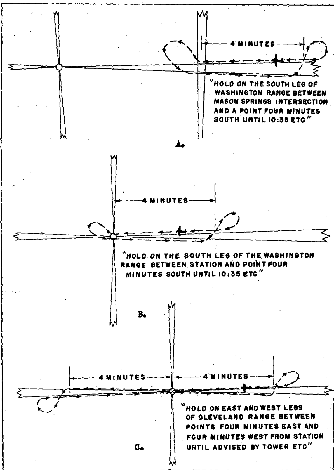
Figure 22. Aircraft holding
