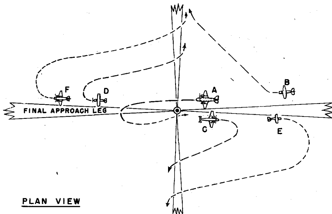
Figure 20. Emergency descent
