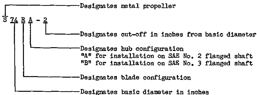
Figure 2. Sample Propeller Specification for Metal Fixed-Pitch Propellers.
