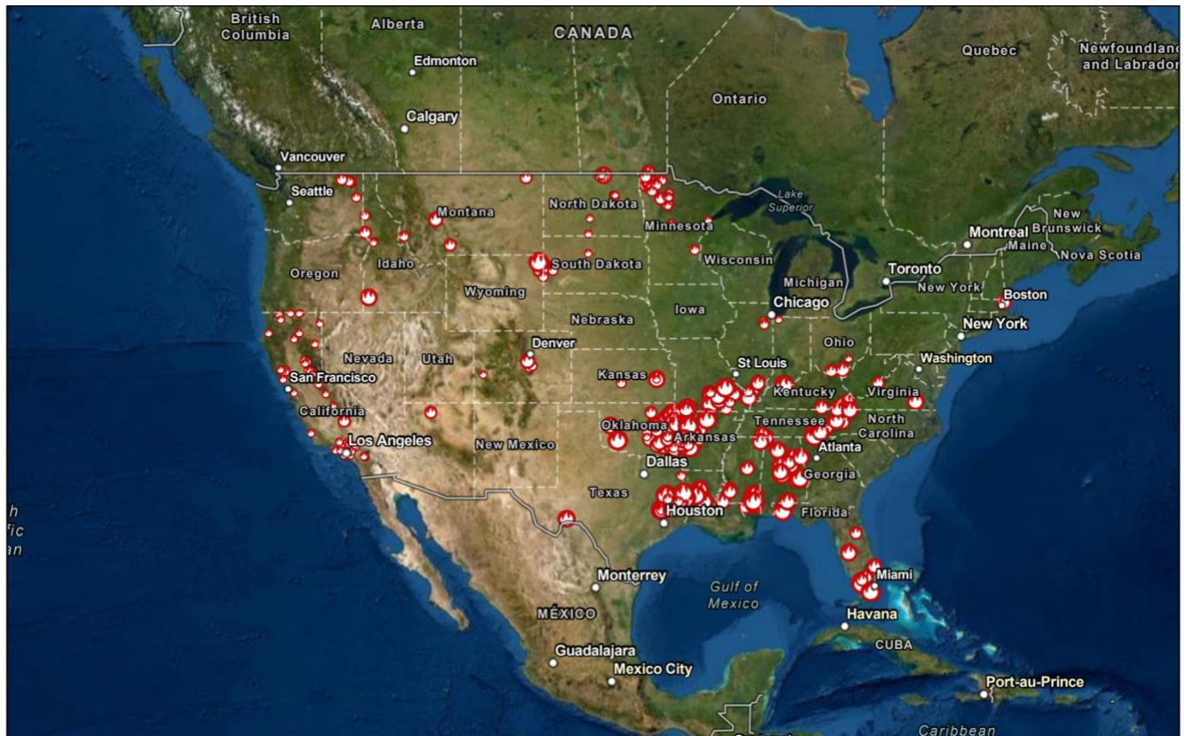
Figure 2. Wildfire incidents in the US as of March 28, 2021 (Image obtained courtesy of US Wildfire reports by Esri Disaster Response Program).
