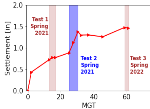
Figure 5. Settlement during surfacing cycle from Spring 2021 to Spring 2022
