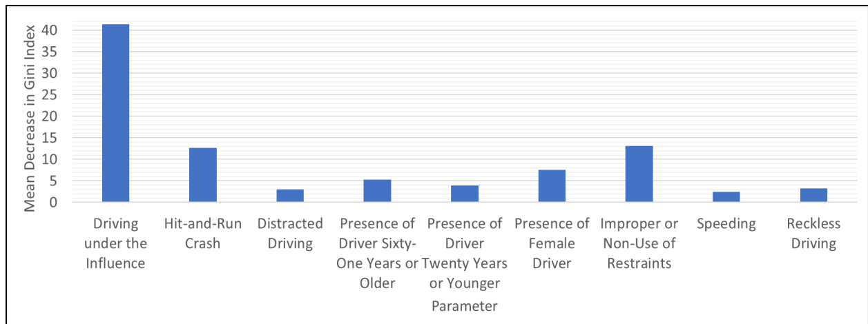
Figure 4.1 Random forest model’s variable importance chart
