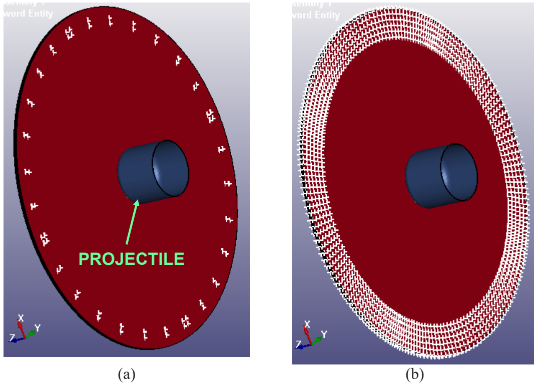
Figure 36. Nodes which have Translational Restraints: (a) In-Plane Displacement (b) Out-Of-Plane Displacement
