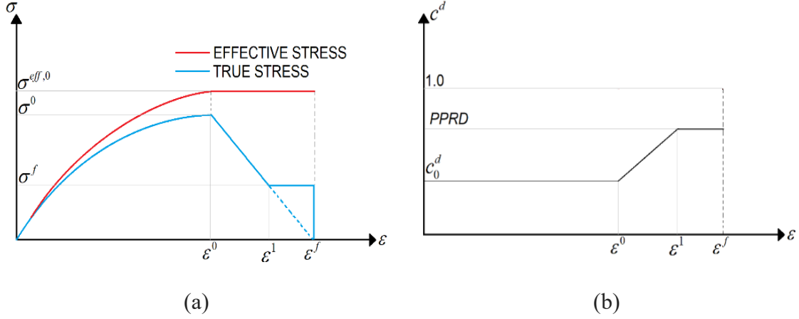
Figure 8. (a) Stress vs Strain Response using PFC (note \sigma^{\max} = \sigma^0 ) (b) Effective Damage
