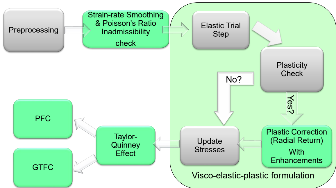
Figure 3. Algorithm Used in the New Implementation
