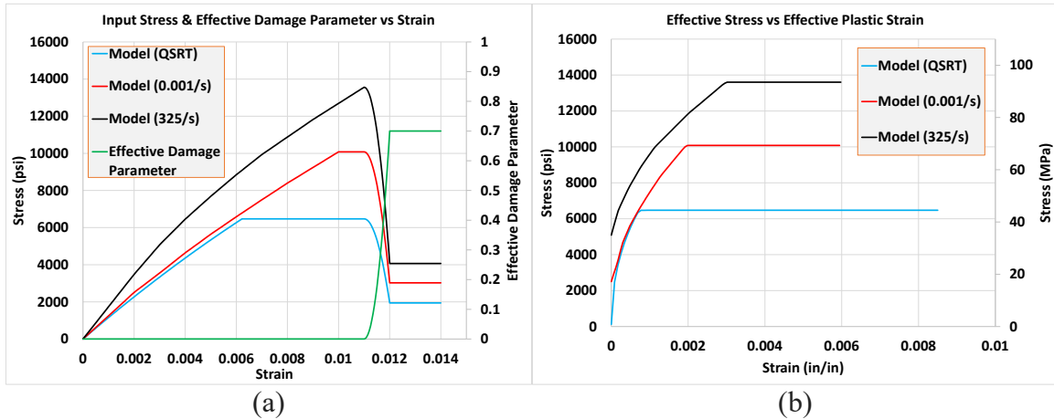
Figure 35. 2-Direction Tension Data for T800/F3900 Composite: (a) Input Stress and Effective Damage Parameter vs Strain Curves (b) Effective Stress vs Effective Plastic Strain Curves Constructed from Data in (a)
