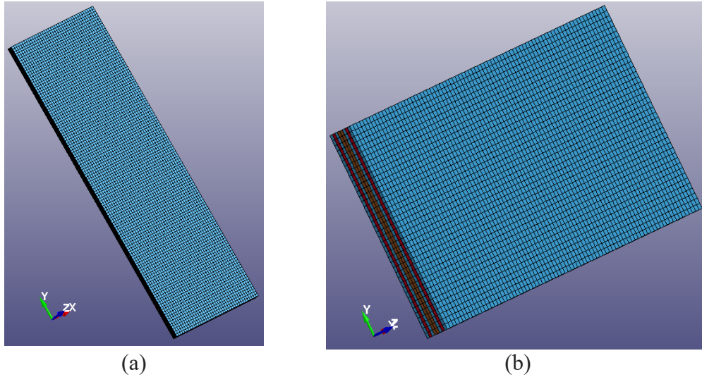
Figure 22. FE Model Used for (a) Stacked-Ply Tension Test (SPVT) (b) Stacked-Ply Compression Test (SPVC).
