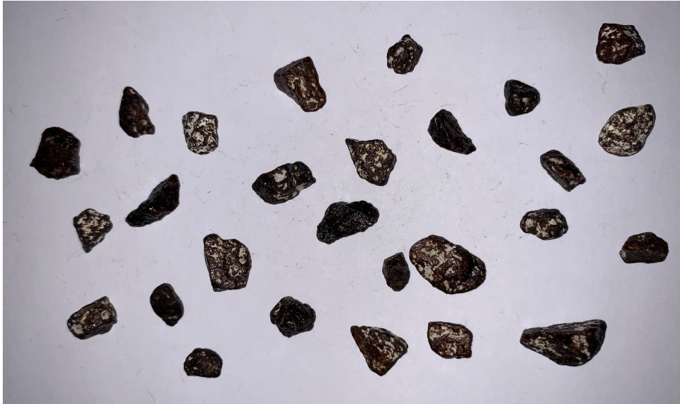
Figure 4.15. Limestone aggregate at 85.6% precoat (0.6% binder by weight)
