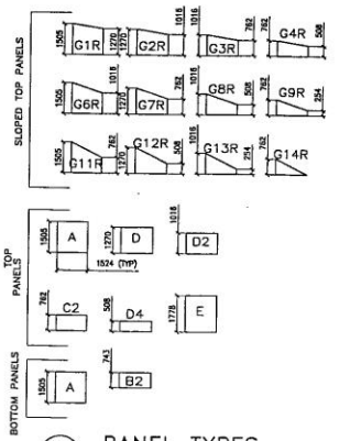
4 PANEL TYPES ALL DIMENSIONS ARE IN MILLIMETERS
