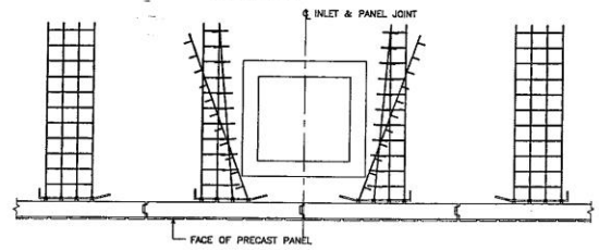
101 INLET OBSTRUCTION DETAIL
