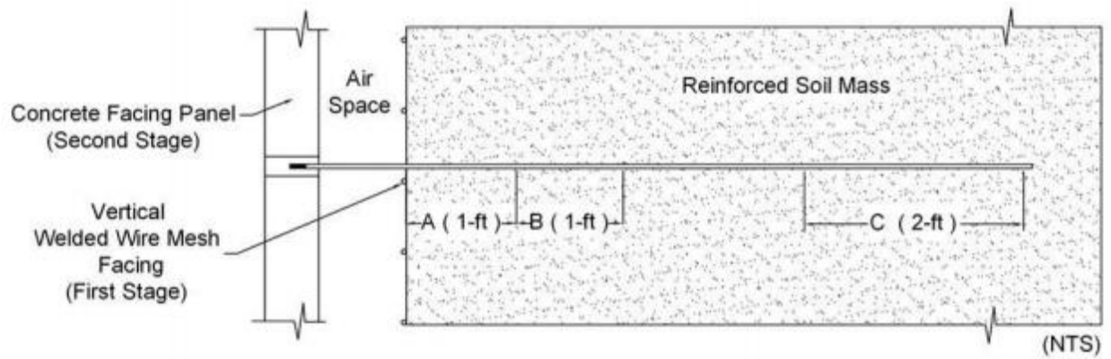
Figure 3-9: Coupon Segmentation
