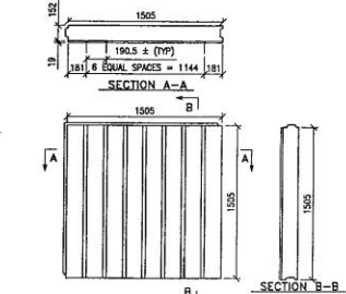
6 ARCHITECTURAL PANEL FINISH (PANEL FRONT FACE SHOWN)
