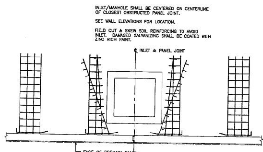
100 INLET OBSTRUCTION DETAIL FACE OF PRECAST PANEL
