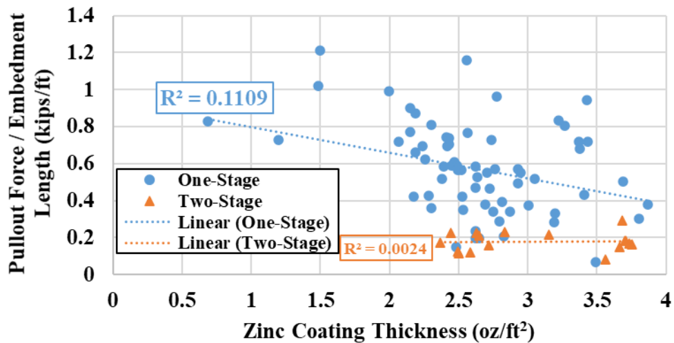
Figure 5-6: Pullout Force / Embedment Length vs. Zinc Coating Thickness
