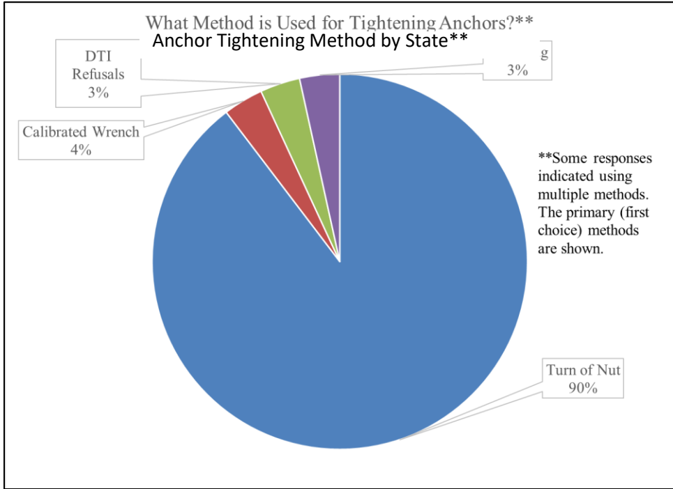
Figure 3-2 - Preferred Anchor Tightening Procedure Per State Survey
