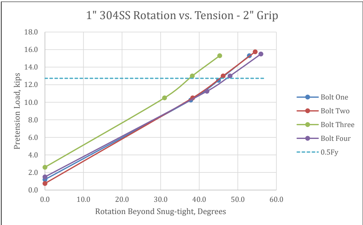
Figure 4-21 - 1" 304 Stainless Steel Rotation vs. Tension
