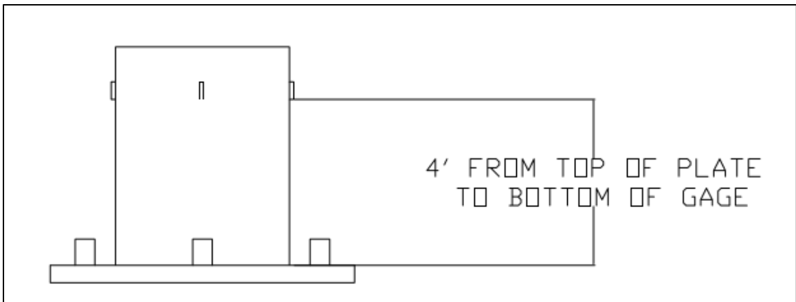
Figure 5-3 - Elevation View of Strain Gages
