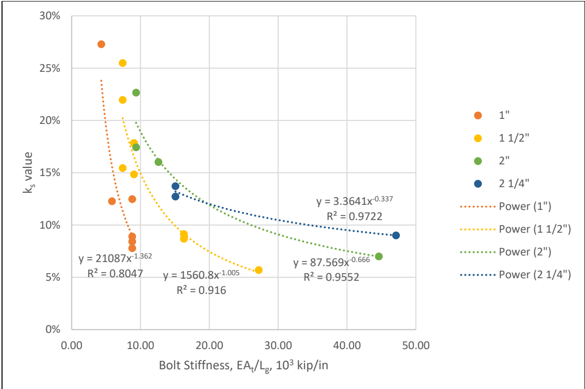
Figure 7-2 - k_s Values vs. Bolt Stiffness and Diameter
