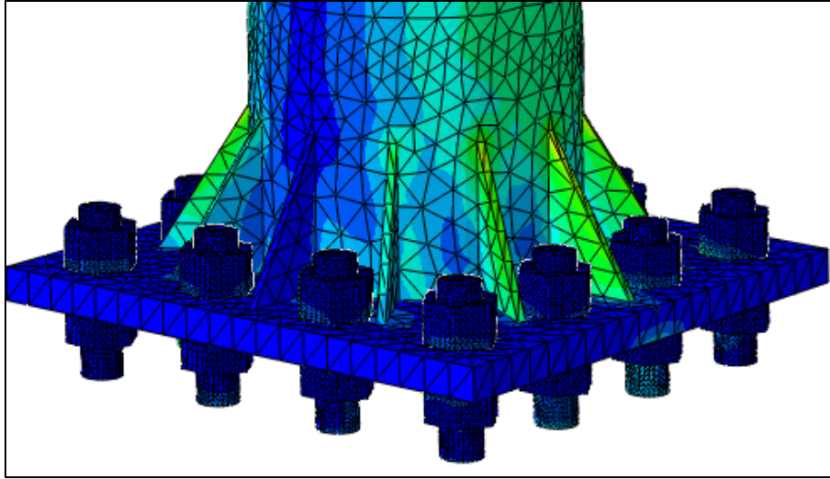
Figure 6-14 - Stresses on Top Nuts
