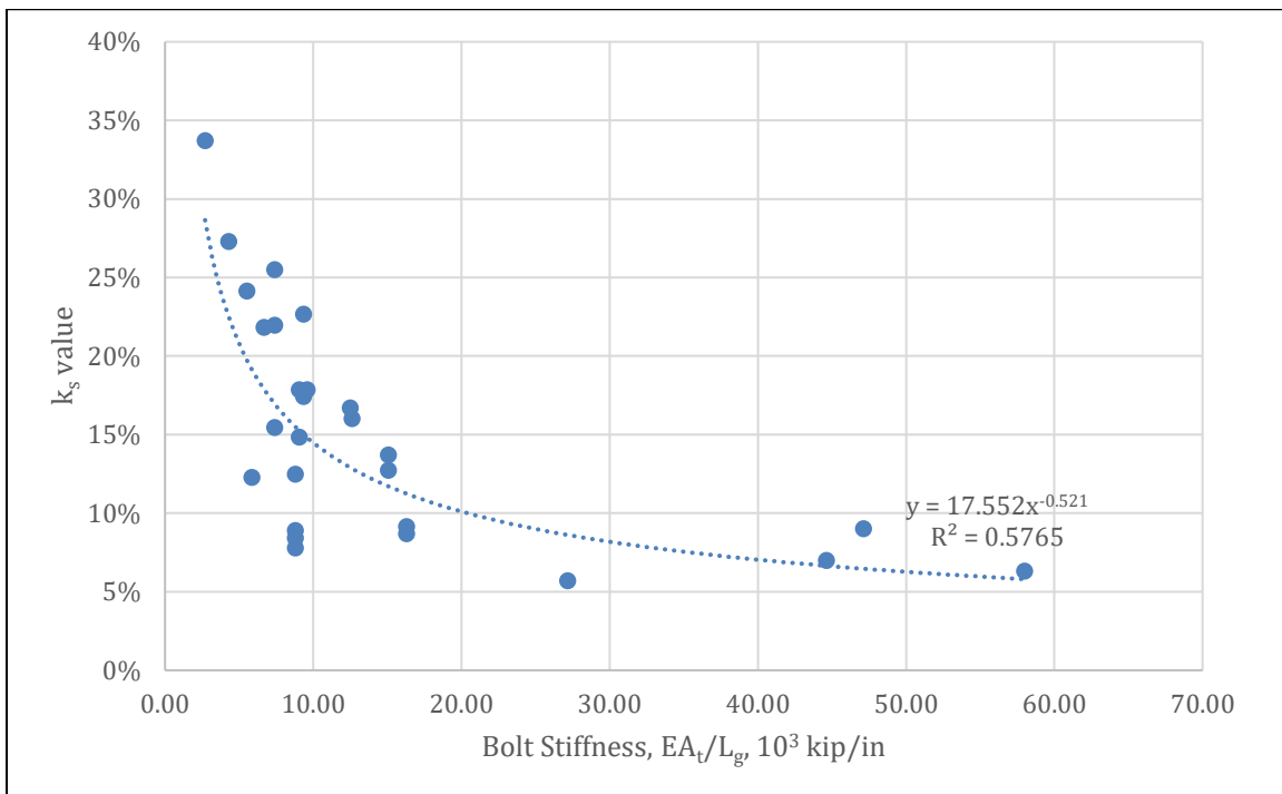
Figure 7-1 - k_s Value vs. Bolt Stiffness
