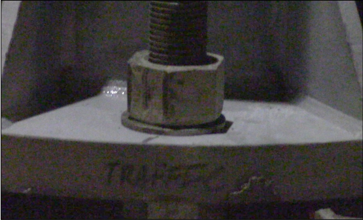
Figure 3-26 - Post Tightening with Reference Marks Shown
