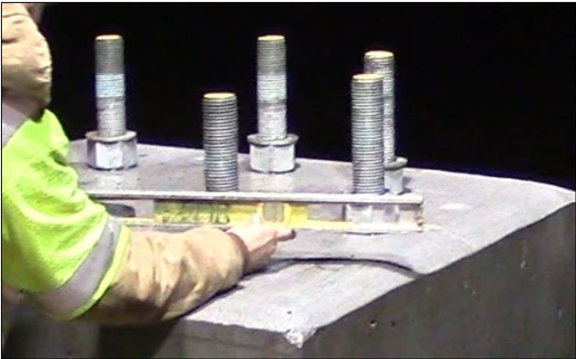
Figure 3-21 - Preparing for Pole Installation
