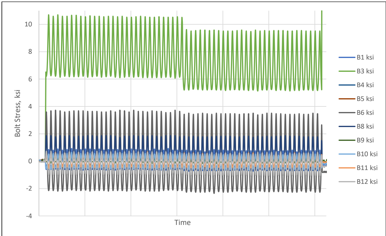
Figure 5-50 - Bolt Stress vs. Time
