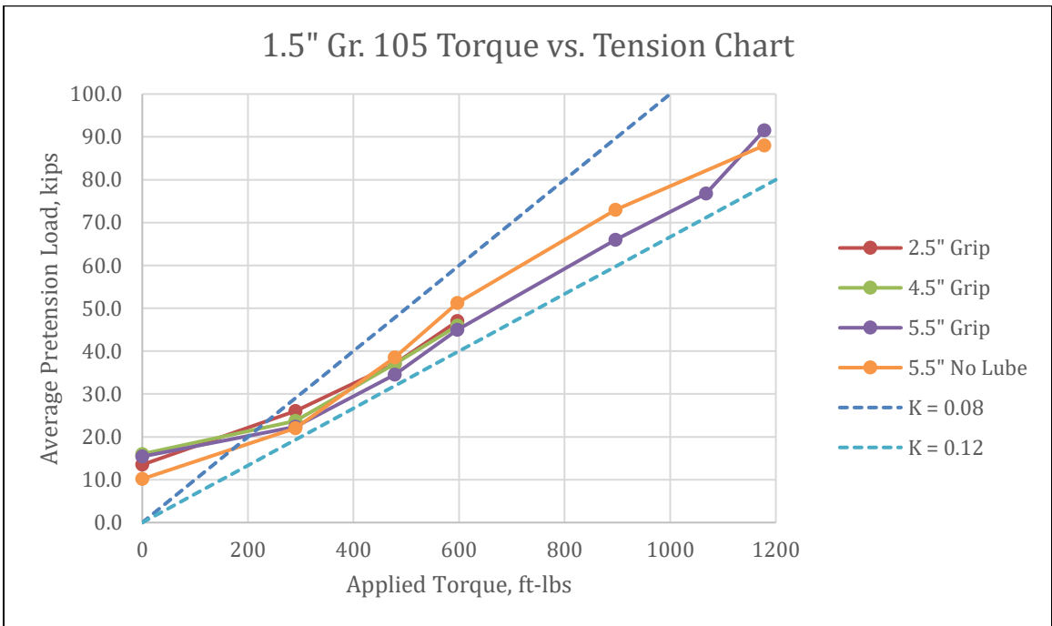
Figure 4-11 – 1.5" Torque vs. Tension
