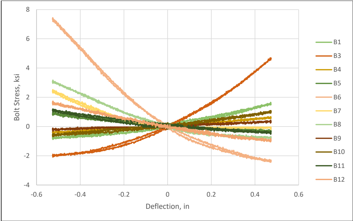
Figure 5-41 - Deflection vs. Bolt Stress
