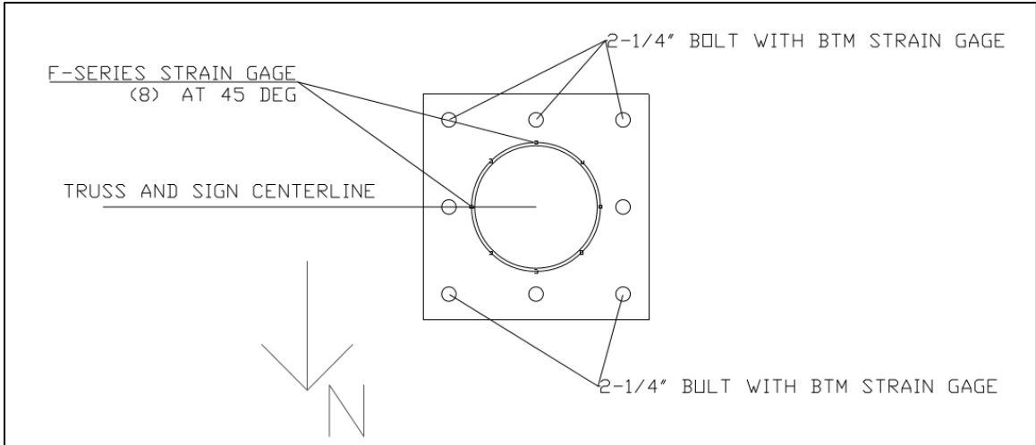
Figure 5-2 - Strain Gage Layout
