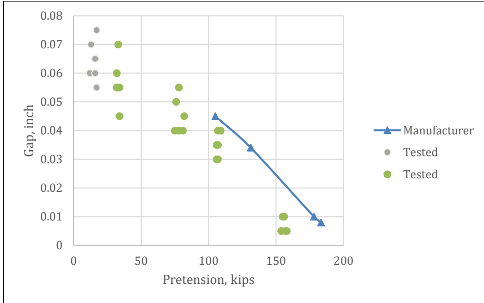
Figure 4-43 - 2" Gr. 105 DTI
