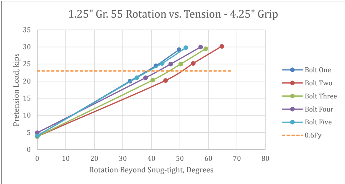
Figure 4-24 - 1.25" Gr. 55 Rotation vs. Tension
