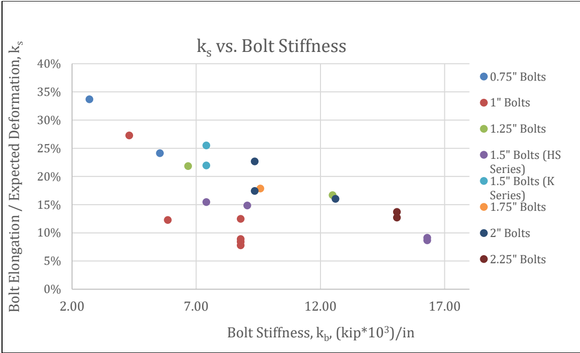
Figure 4-36 - Bolt Stiffness vs. k s
