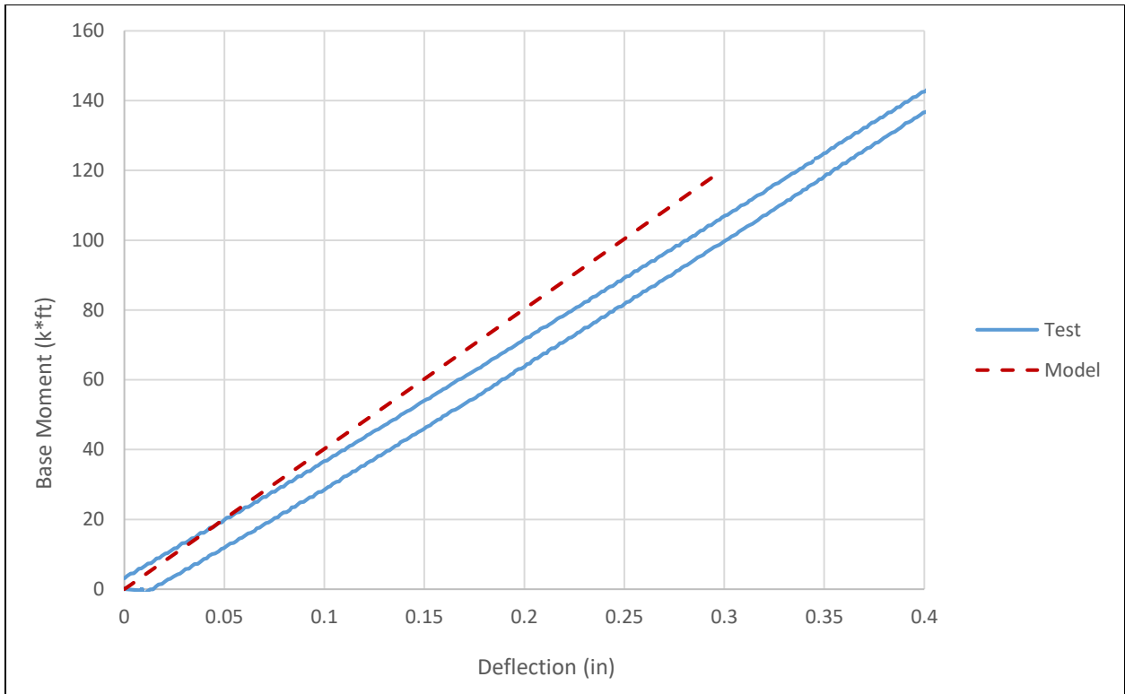
Figure 6-9 - Deflection vs. Base Moment
