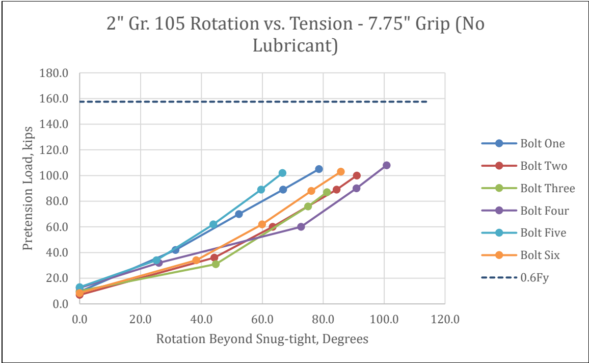
Figure 4-32 - 2" Gr. 105 with 7.75" Grip (No Lubricant) Rotation vs. Tension
