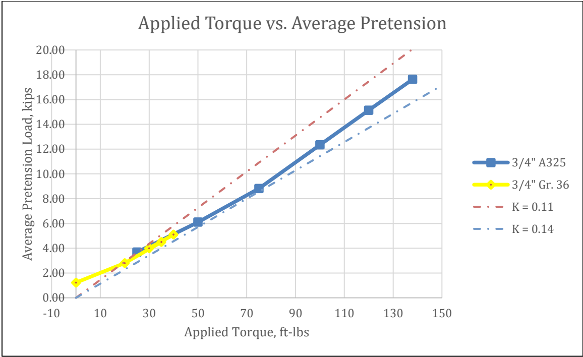
Figure 4-8 – 0.75" Bolts Torque vs. Tension
