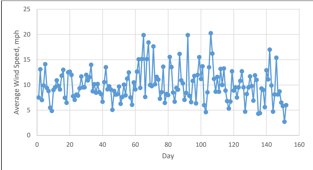
Figure 5-18 - Average Wind Speeds During Monitoring
