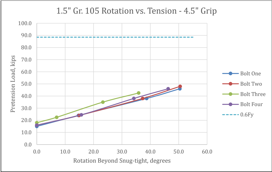
Figure 4-26 - 1.5" Gr. 105 with 4.5" Grip Rotation vs. Tension
