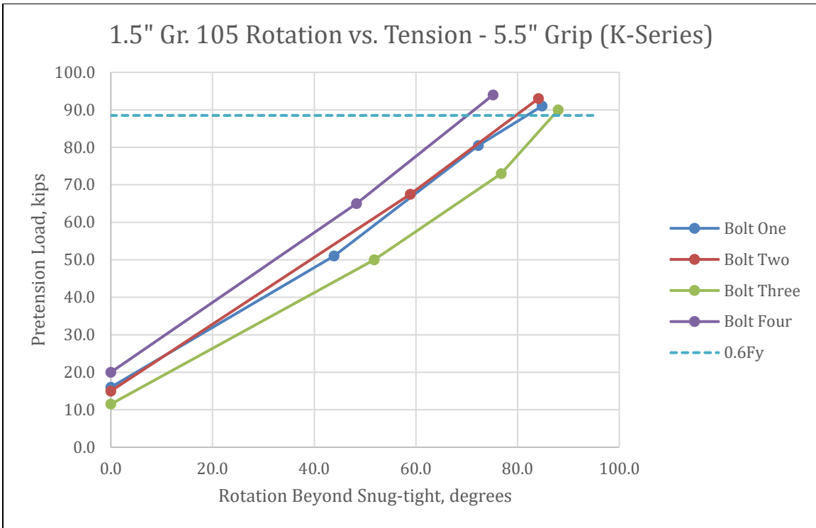
Figure 4-28 - 1.5" Gr. 105 with 5.5" Grip (K-Series) Rotation vs. Tension
