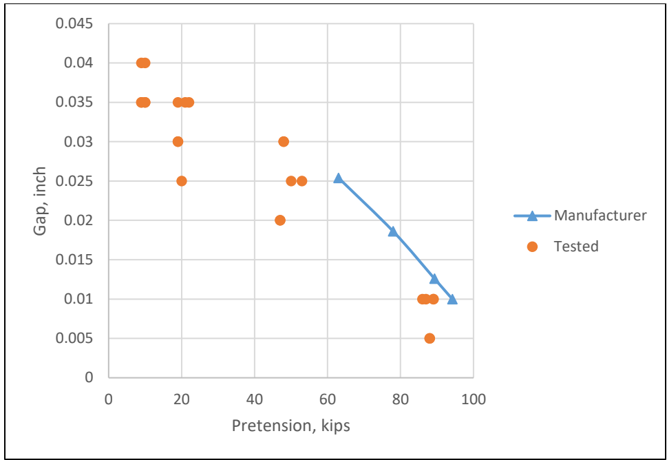
Figure 4-41 - 1.5" Gr. 105 DTI
