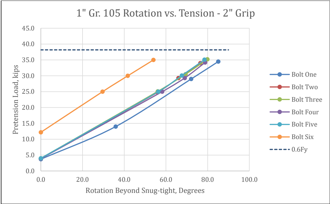
Figure 4-18 - 1" Gr. 105 Rotation vs. Tension
