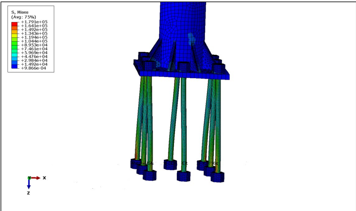
Figure 6-2 - Stress in Bolts Under 20 PSF Wind
