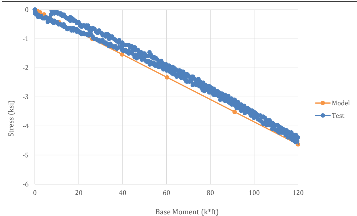
Figure 6-11 - Base Moment vs. Stress in Bolt 6
