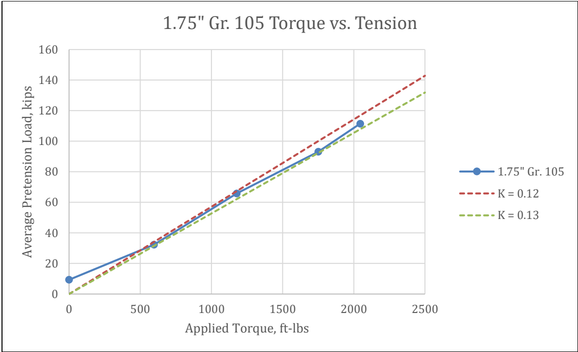
Figure 4-12 – 1.75" Torque vs. Tension
