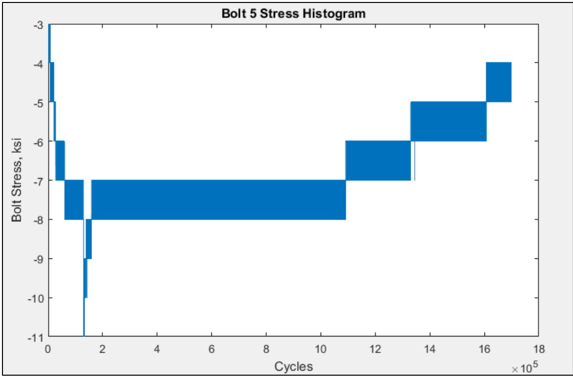
Figure 5-16 - Bolt 5 Stress Histogram
