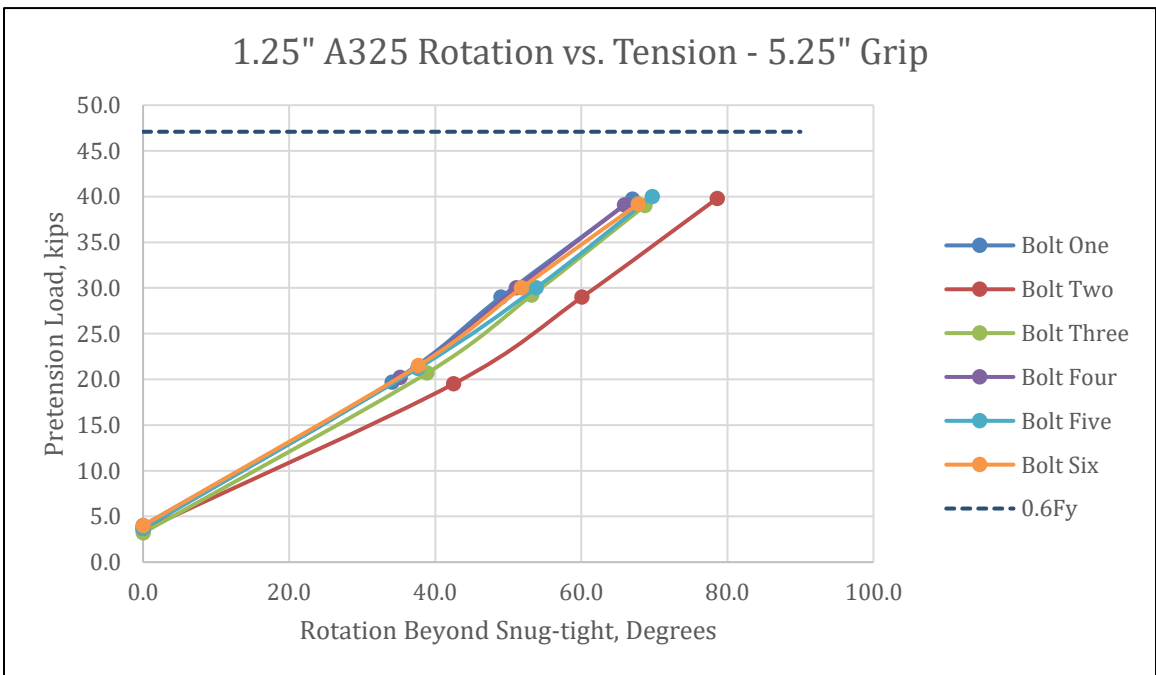
Figure 4-23 - 1.25" A325 Rotation vs. Tension
