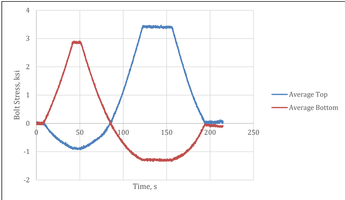
Figure 5-45 - Average Stresses vs. Time
