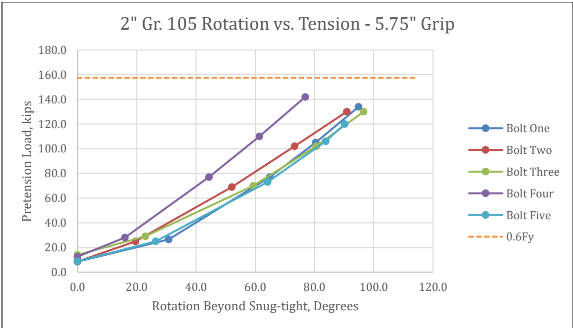
Figure 4-31 - 2" Gr. 105 with 5.75" Grip Rotation vs. Tension
