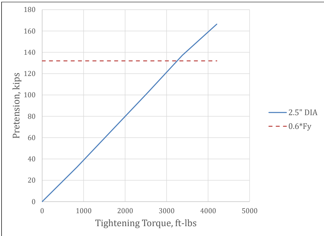
Figure 5-38 - Torque vs. Tension for 2-1/2" Diameter Bolts
