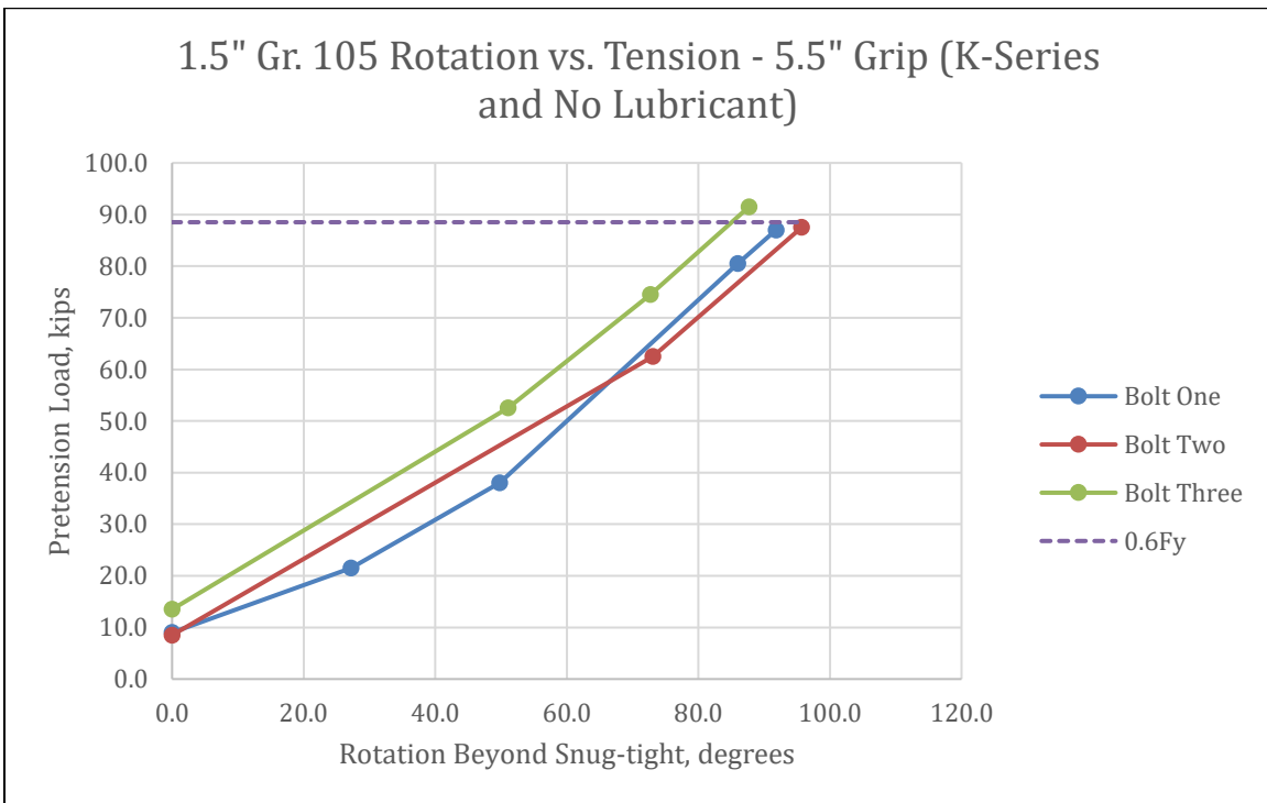
Figure 4-29 - 1.5" Gr. 105 with 5.5" Grip (K-Series & No Lubricant) Rotation vs. Tension
