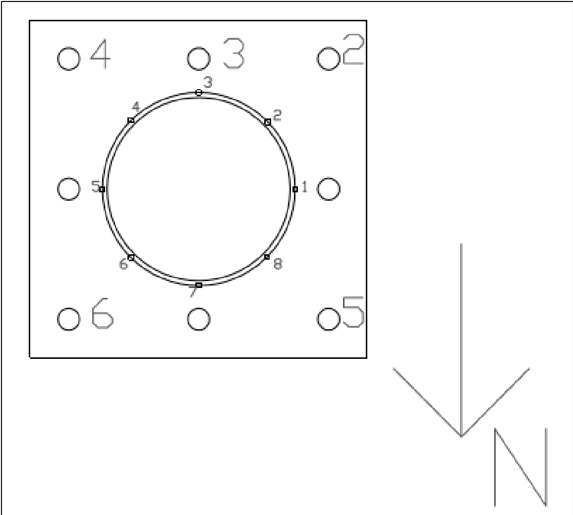
Figure 5-4 - Labeling for Strain Gages
