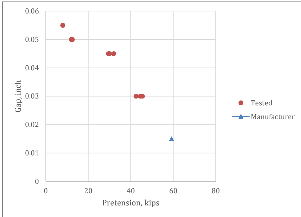
Figure 4-40 - 1.25" A325 DTI
