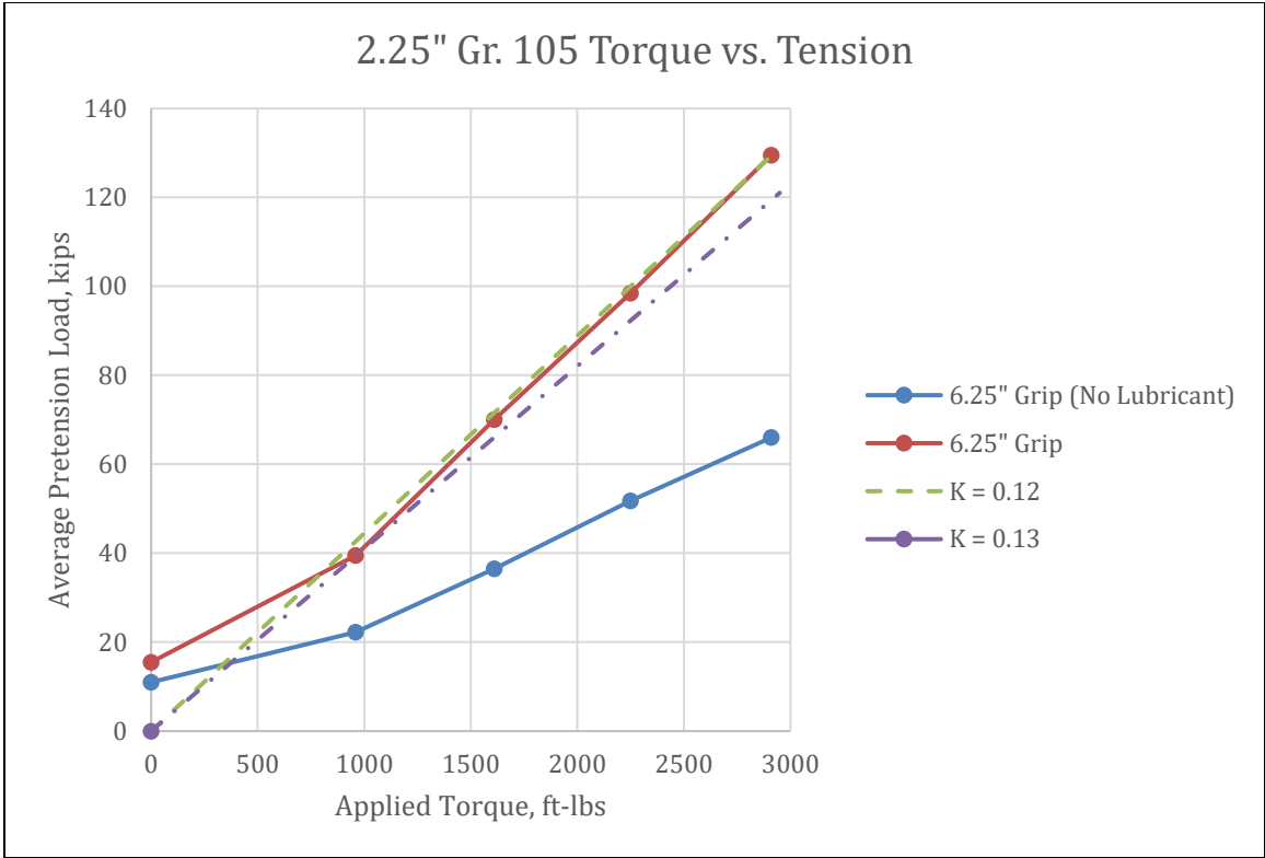
Figure 4-14 – 2.25" Torque vs. Tension
