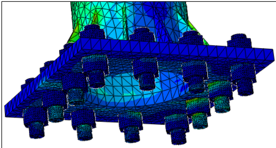
Figure 6-13 - Stresses on Bottom Nuts
