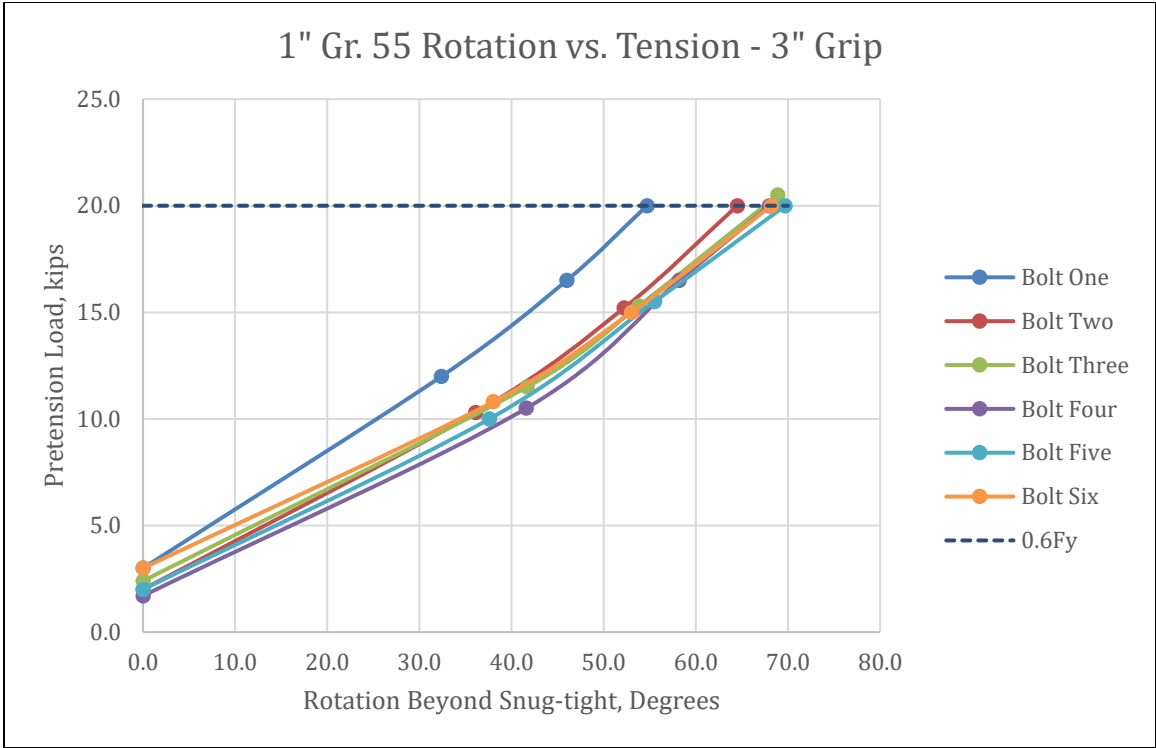
Figure 4-20 - 1" Gr. 55 with 3" Grip Rotation vs. Tension
