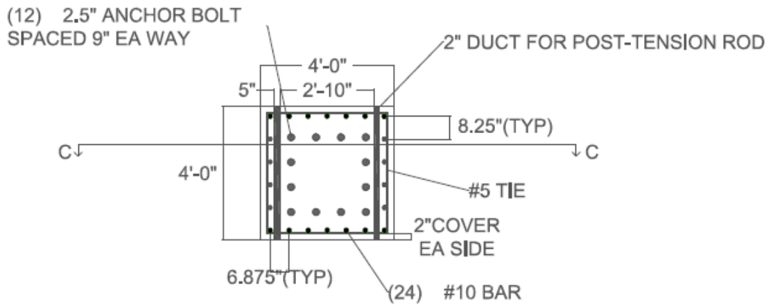
Figure 5-21 - Cross Section of Concrete Block (A-A)
