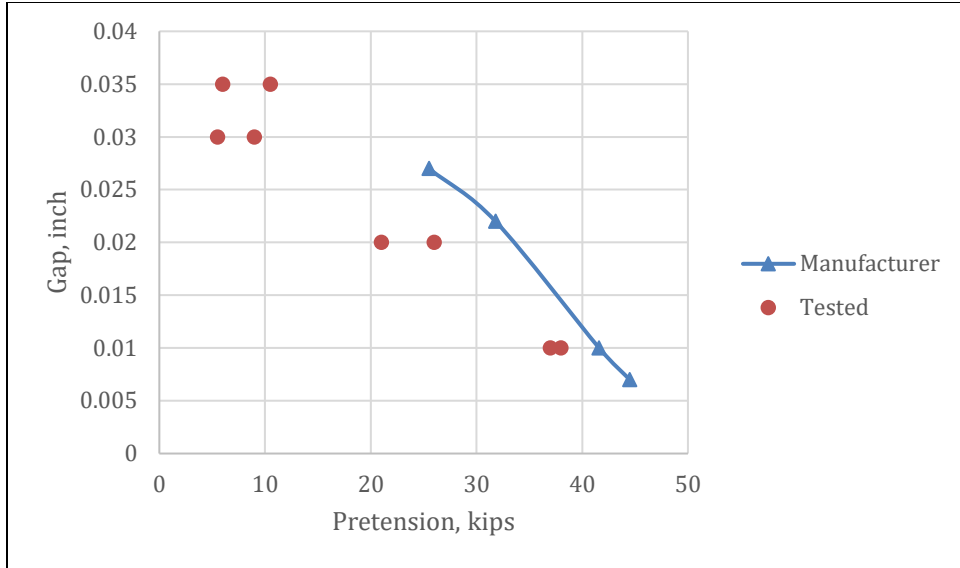
Figure 4-39 - 1.0" Gr. 105 DTI
