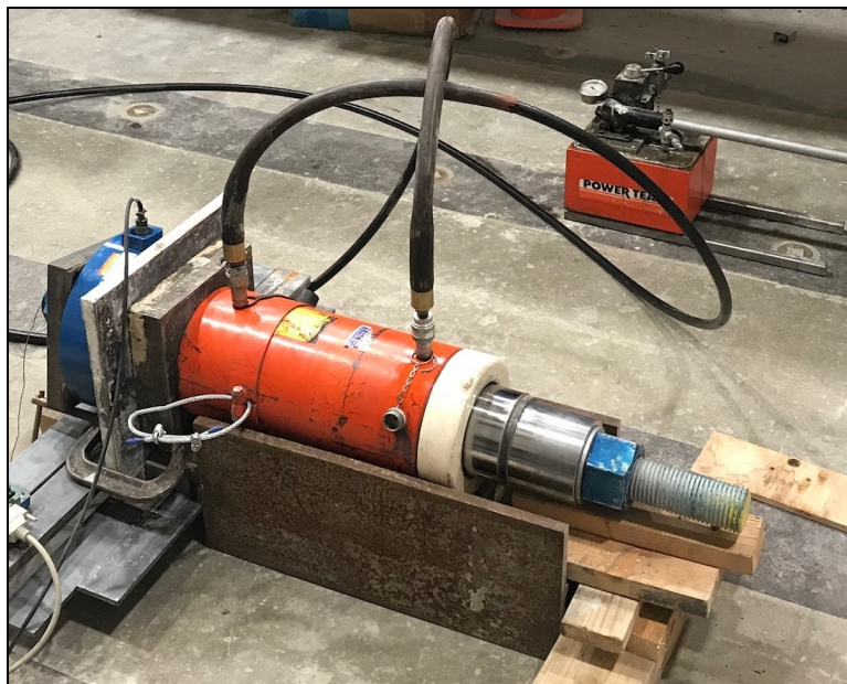
Figure 5-27 - Individual Calibration of Anchor Bolts
