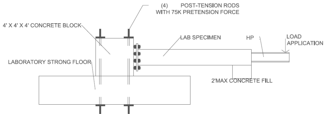
Figure 5-23 - Side View of Lab Specimen
