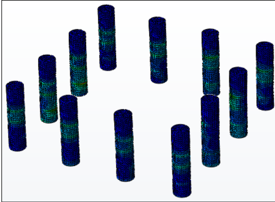
Figure 6-12 - Anchor Bolt Stresses
