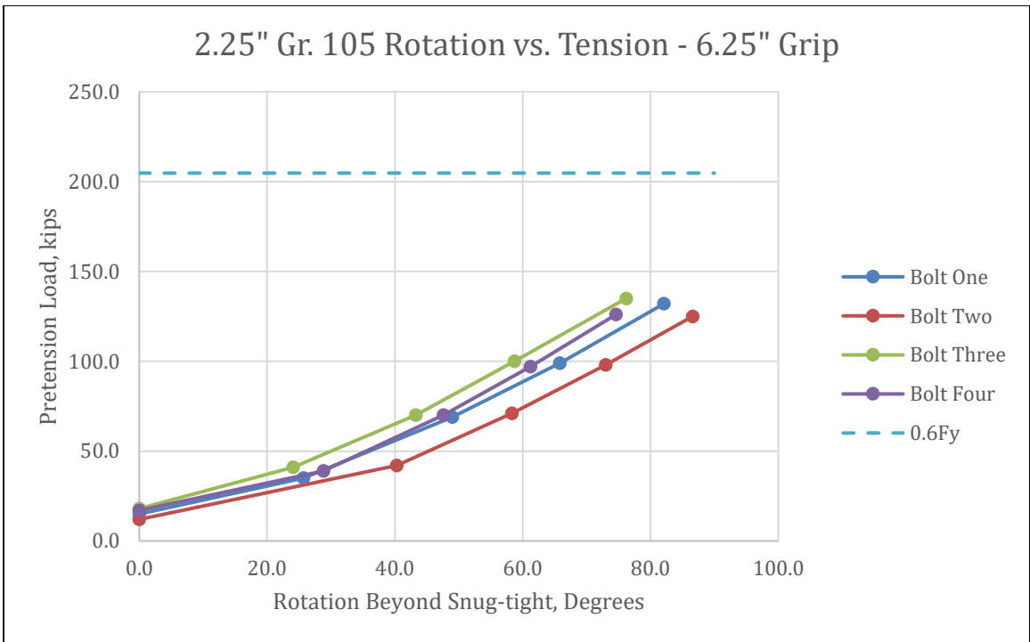
Figure 4-35 - 2.25" Gr. 105 Rotation vs. Tension
