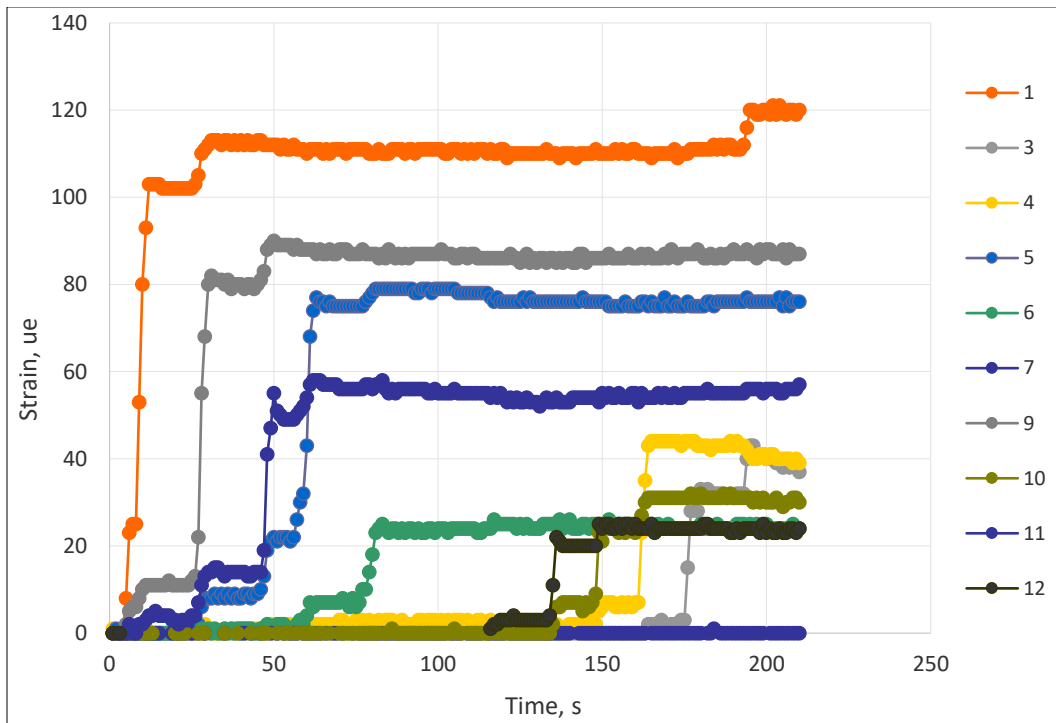
Figure 5-39 – Circle Pattern Data
