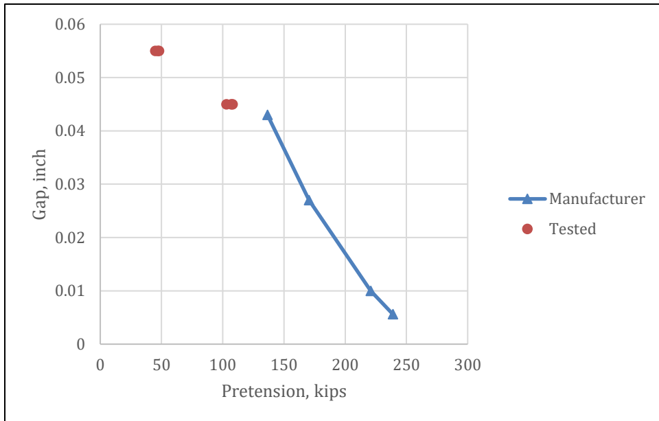
Figure 4-44 - 2.25" Gr. 105 DTI
