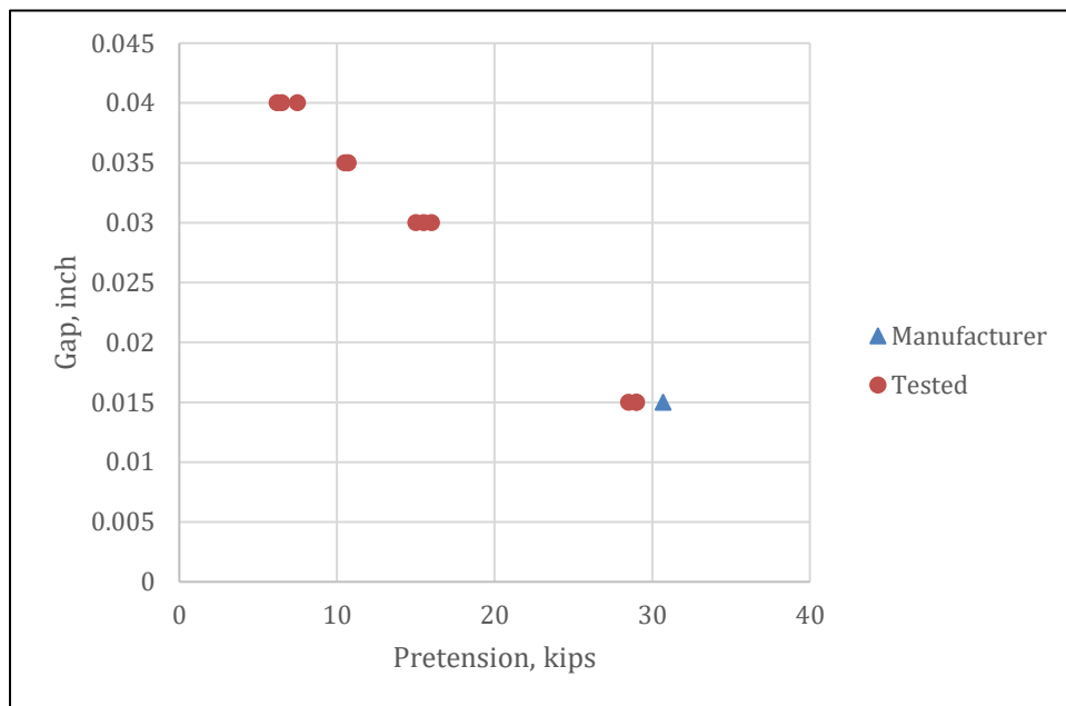
Figure 4-38 - 0.75" A325 DTI
