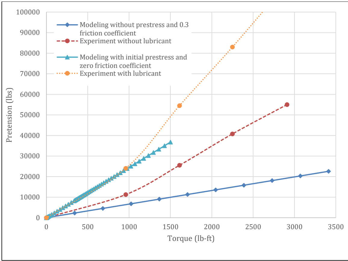
Figure 6-8 - Comparison of Experiment and Modeling
