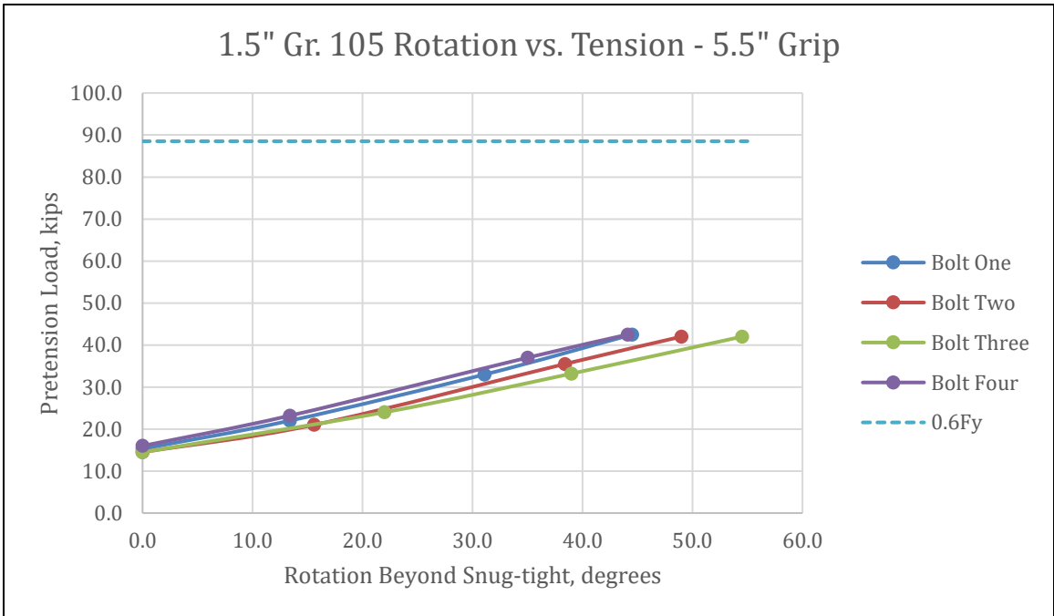
Figure 4-27 - 1.5" Gr. 105 with 5.5" Grip Rotation vs. Tension
