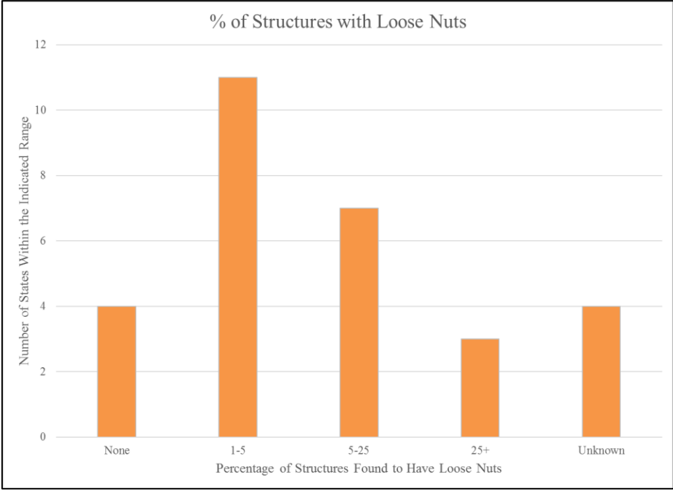
Figure 3-5 - Percentage of Structures with Loose Nuts Per State Survey
