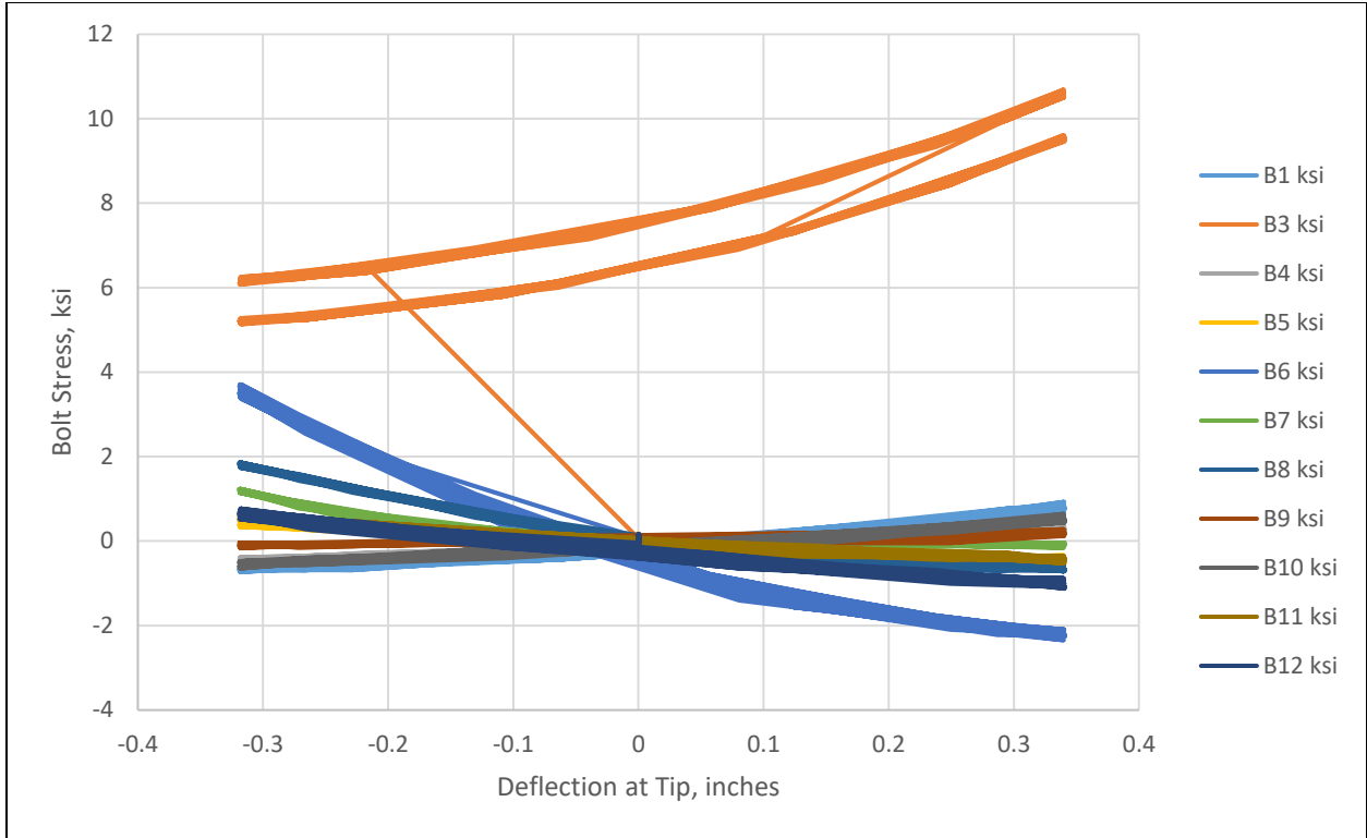
Figure 5-47 - Bolt Stress vs. Deflection
