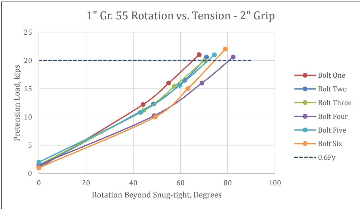
Figure 4-19 - 1" Gr. 55 with 2" Grip Rotation vs. Tension
