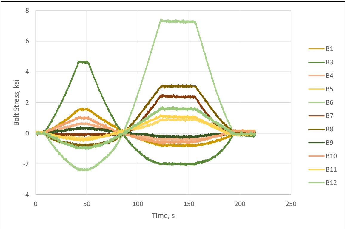
Figure 5-44 - Time vs. Bolt Stress
