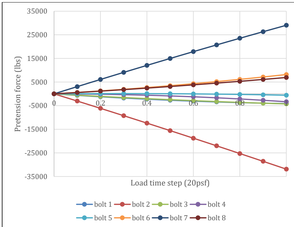
Figure 6-4 - Reaction Force in 8 Anchors Using Predefined Prestress Option
