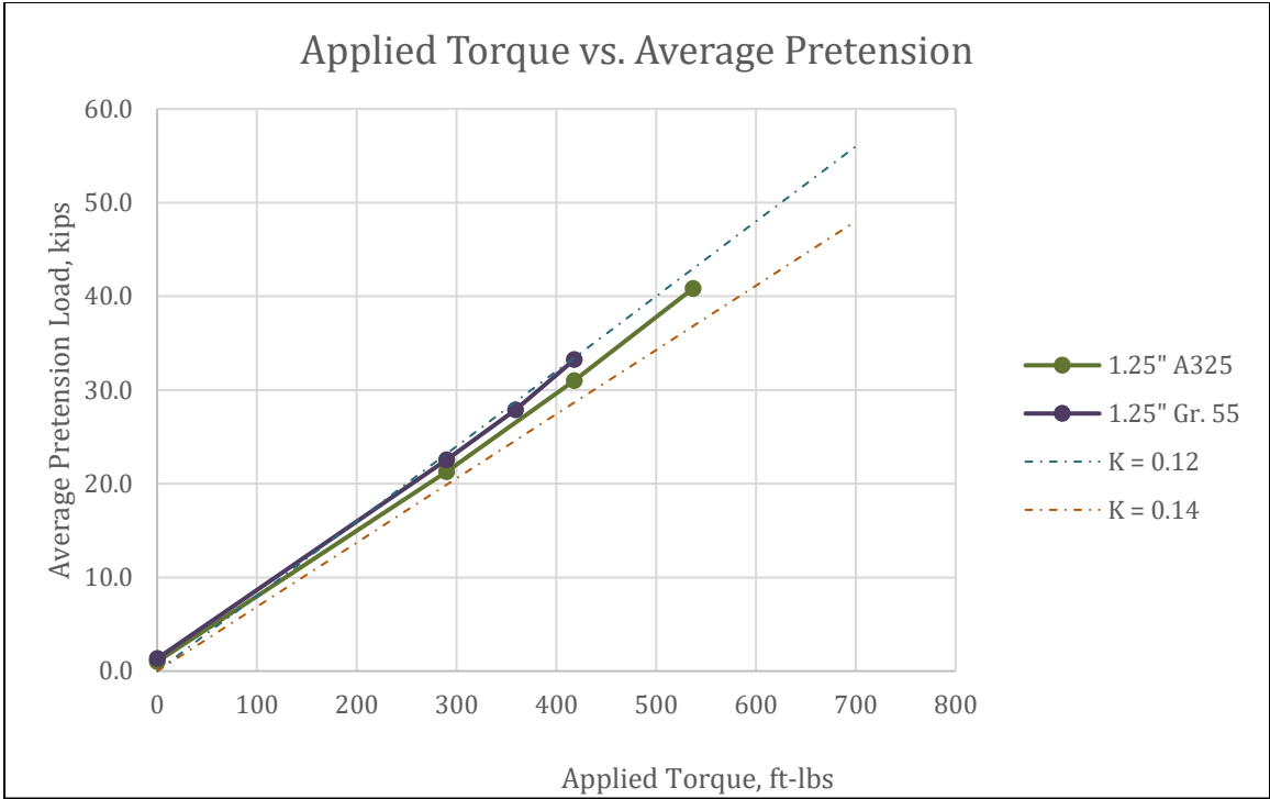
Figure 4-10 – 1.25" Torque vs. Tension
