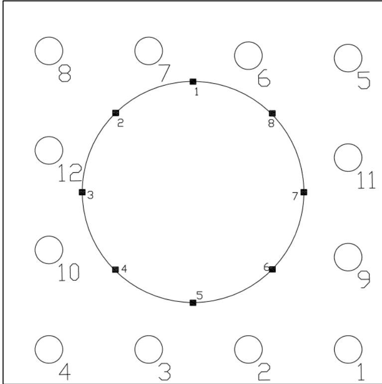
Figure 5-24 - Strain Gage Numbering for Lab Specimen
