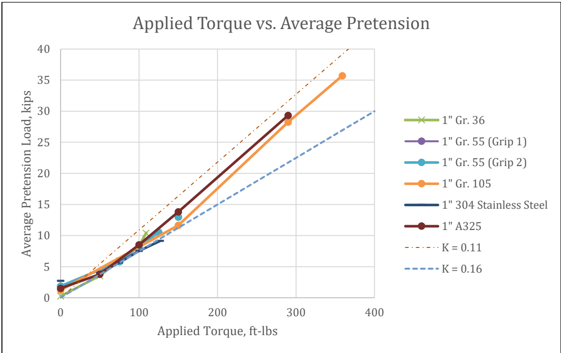
Figure 4-9 - 1" Torque vs. Tension
