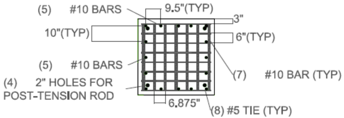
Figure 5-22 - Top View of Concrete Block Reinforcement (C-C)
