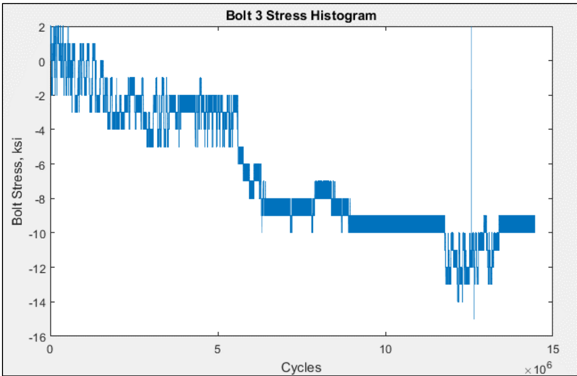
Figure 5-15 - Bolt 3 Stress Histogram
