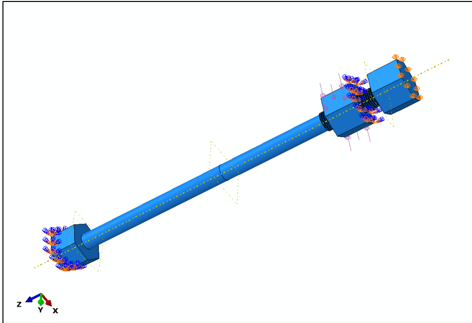
Figure 6-6 - Single Bolt Model with Boundary Conditions
