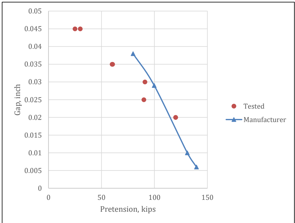
Figure 4-42 - 1.75" Gr. 105 DTI
