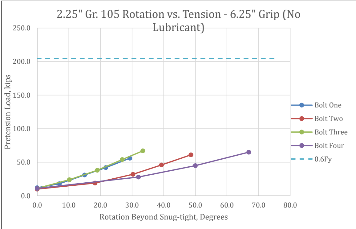
Figure 4-34 - 2.25" Gr. 105 Rotation vs. Tension (No Lubricant)
