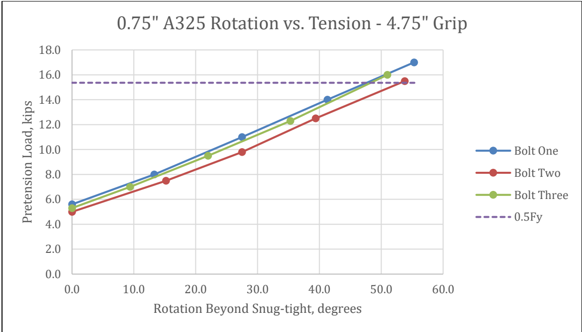
Figure 4-16 - 0.75" A325 Rotation vs. Tension
