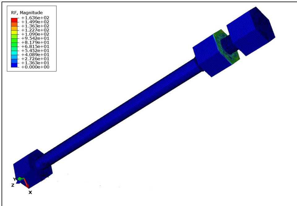
Figure 6-7 - Reaction Force on the Top Surface of Leveling Nut
