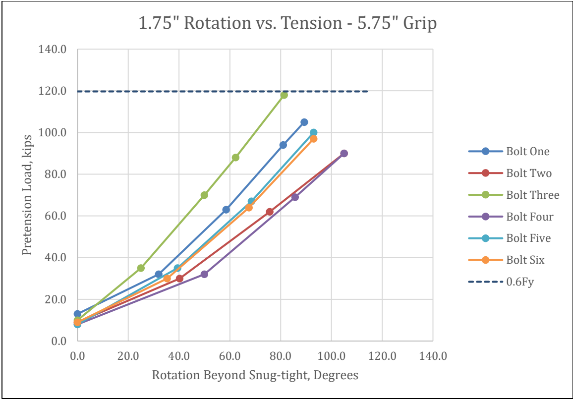
Figure 4-30 - 1.75" Gr. 105 Rotation vs. Tension
