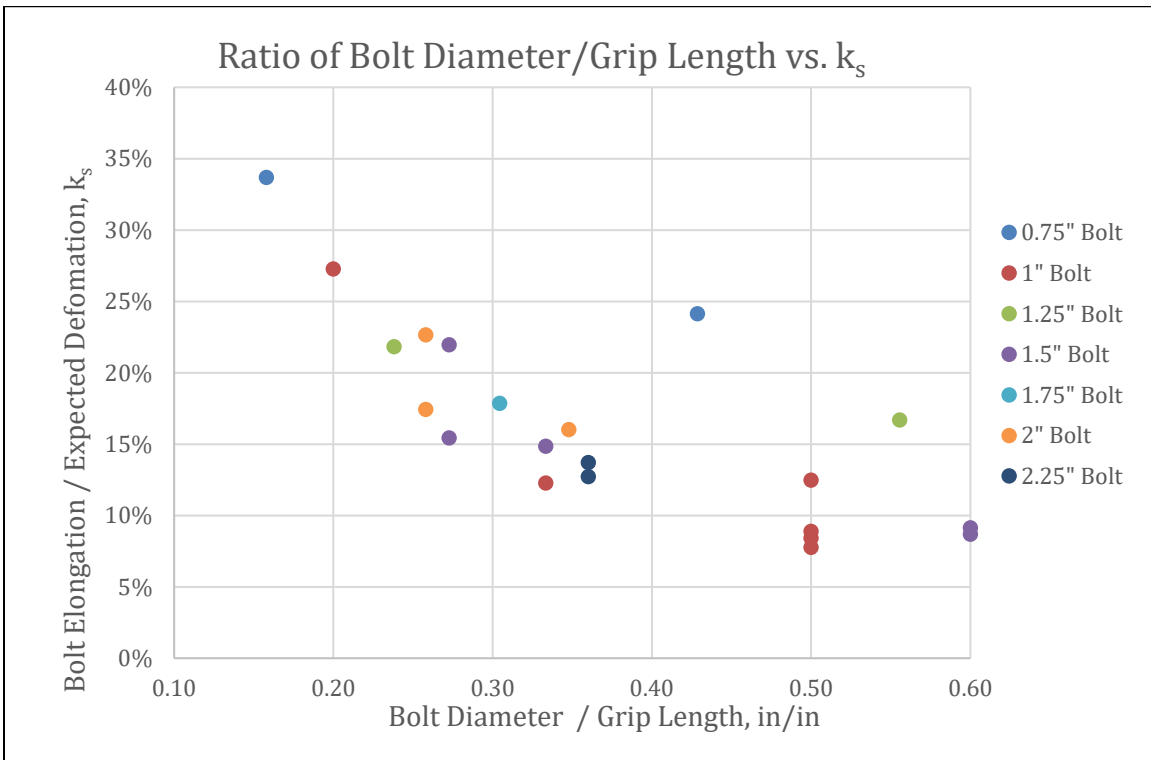
Figure 4-37 - Bolt Diameter / Grip Length vs. k s
