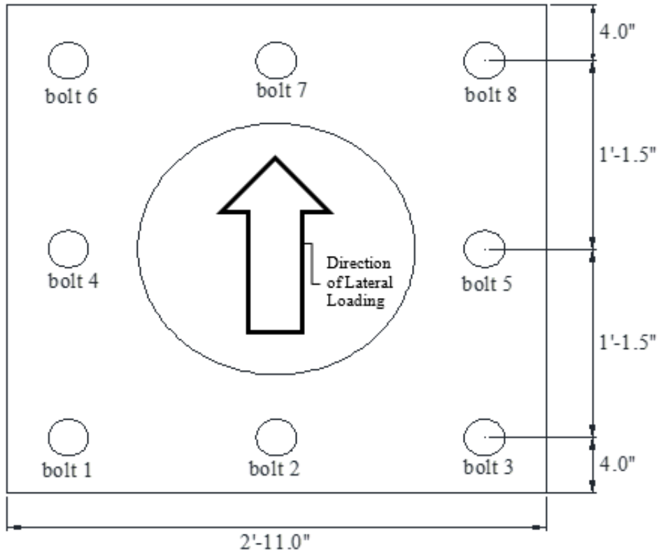
Figure 6-3 - Bolt Numbering Plan
