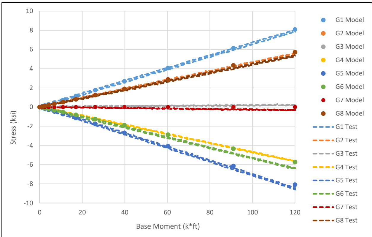
Figure 6-10 - Base Moment vs. Stresses in the Pole
