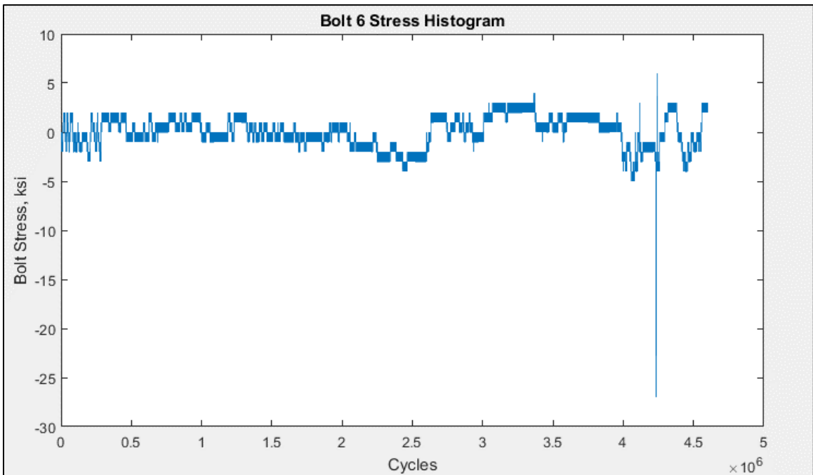
Figure 5-17 - Bolt 6 Stress Histogram
