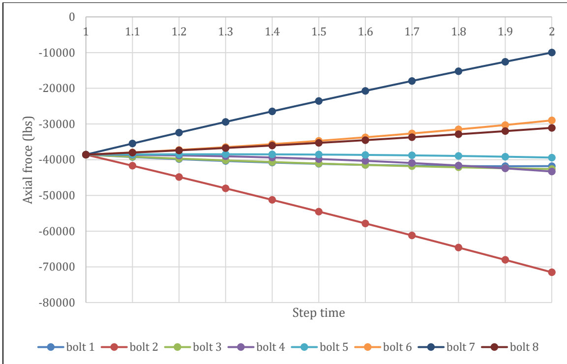
Figure 6-5 - Reaction Force in Anchor Bolts Using Predefined Preload Step
