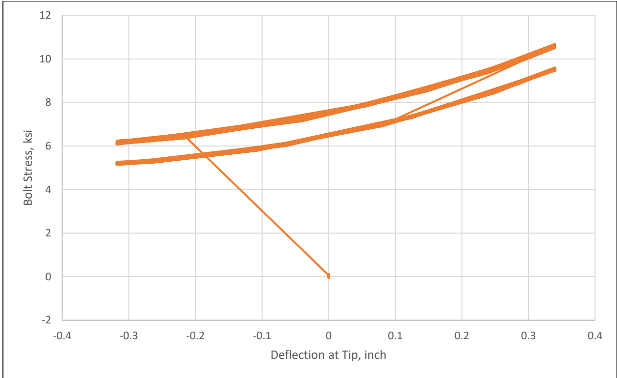
Figure 5-49 - Bolt 3 Stress vs. Deflection
