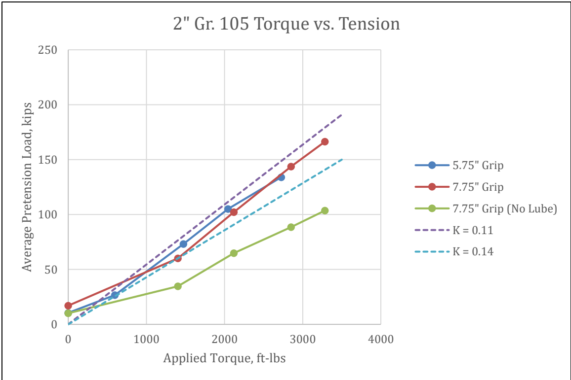
Figure 4-13 - 2" Torque vs. Tension
