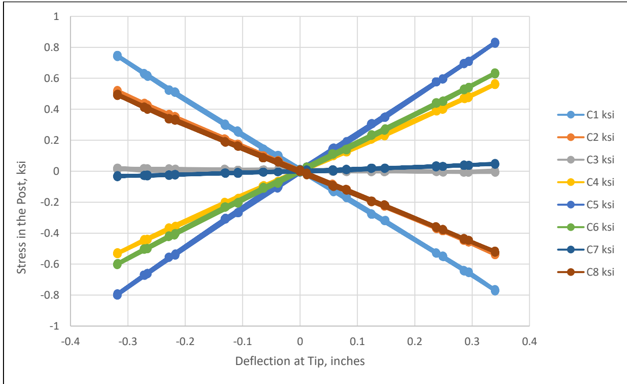
Figure 5-46 - Post Stress vs. Deflection
