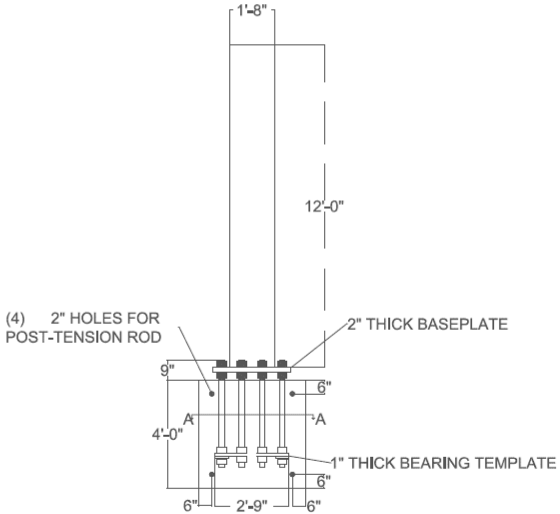
Figure 5-20 - Top View of Lab Specimen
