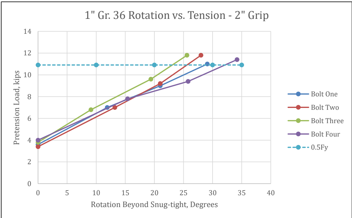
Figure 4-17 - 1" Gr. 36 Rotation vs. Tension
