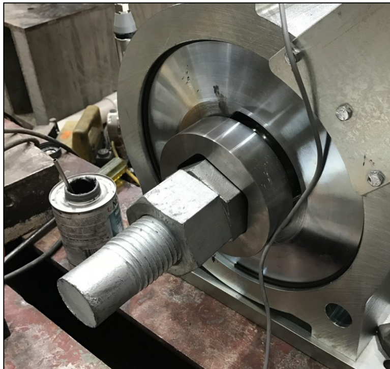
Figure 4-7 - Double Nut to Prevent Bolt Rotation
