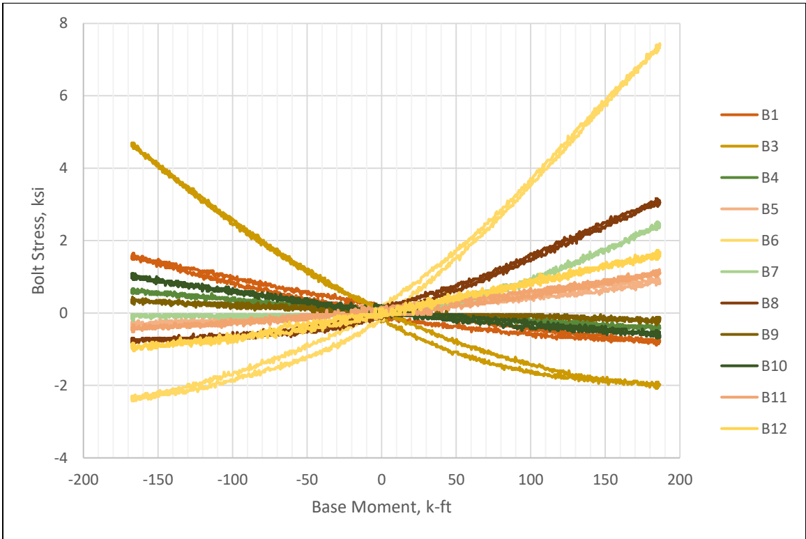
Figure 5-42 - Base Moment vs. Bolt Stress
