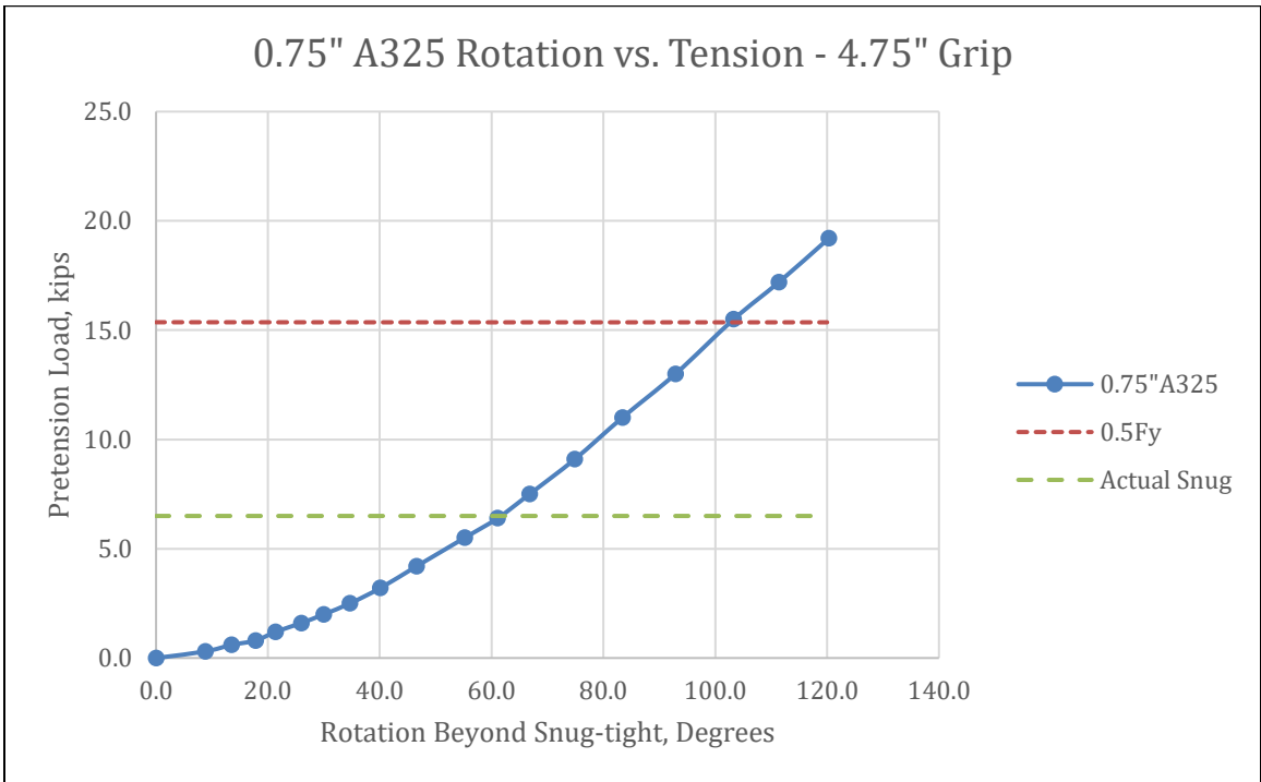
Figure 4-15 - Pre-Snug & Rotation Beyond Snug Curve
