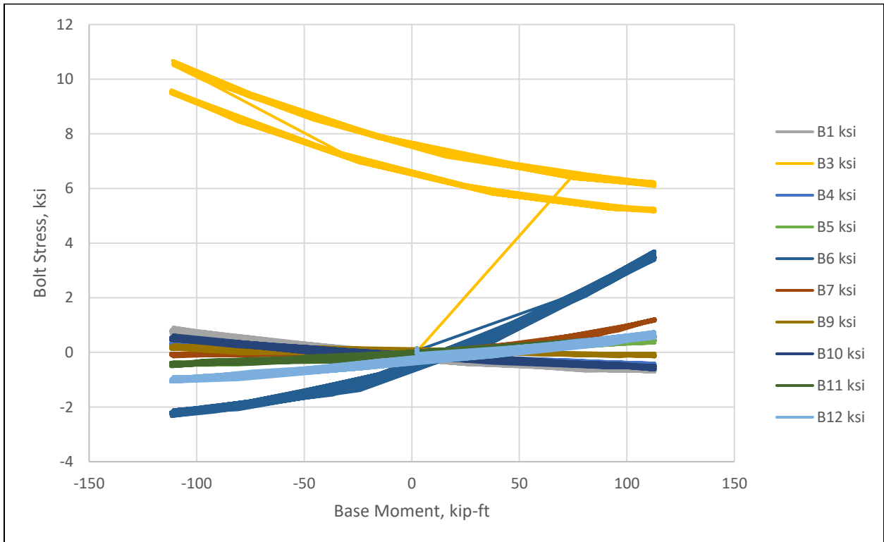
Figure 5-48 - Bolt Stress vs. Base Moment
