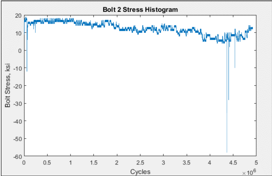
Figure 5-14 - Bolt 2 Stress Histogram
