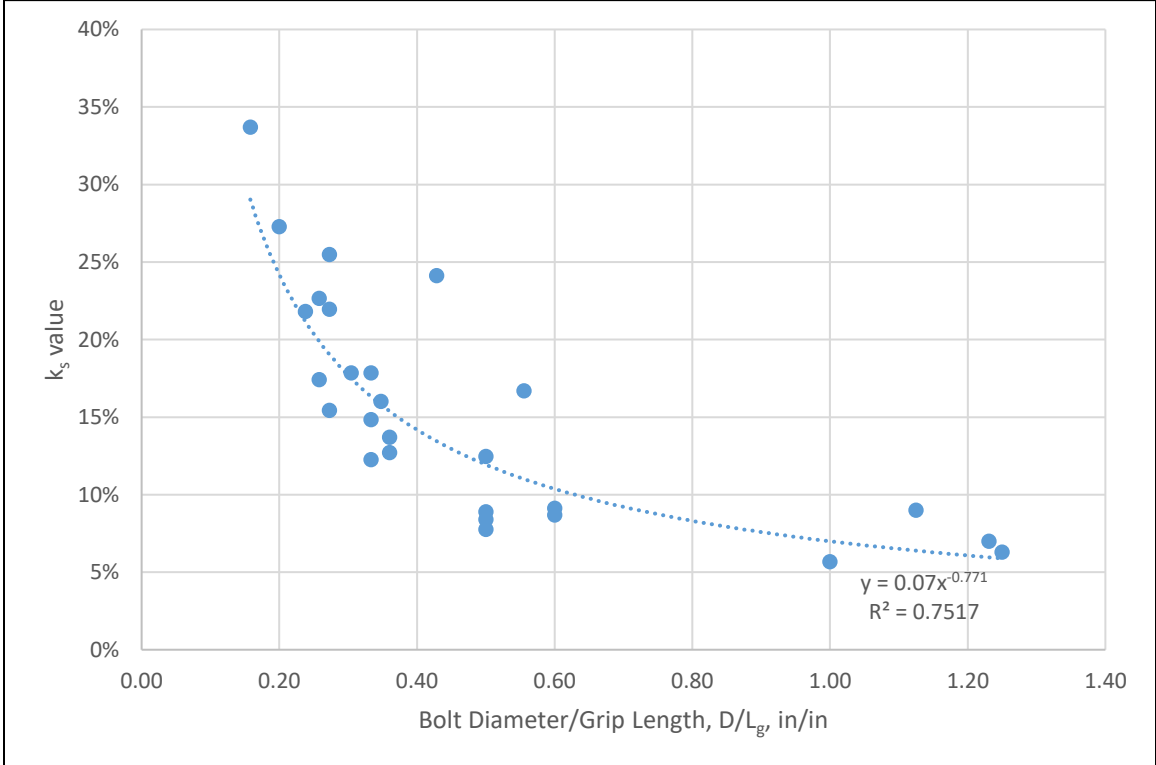
Figure 7-3 - k_s Values vs. Ratio of Bolt Diameter to Grip Length
