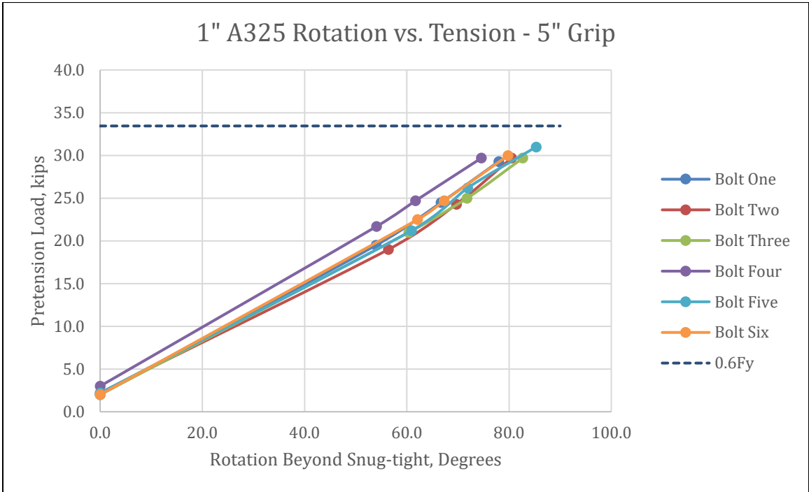
Figure 4-22 - 1" A325 Rotation vs. Tension
