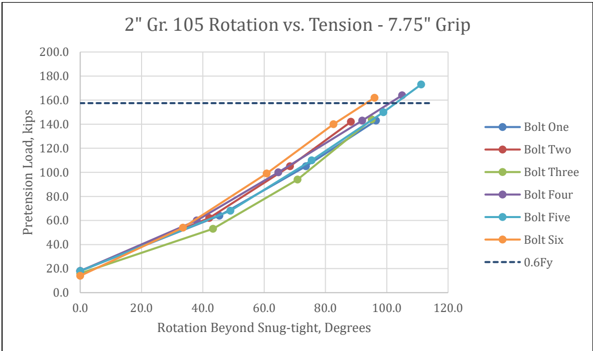
Figure 4-33 - 2" Gr. 105 with 7.75" Grip Rotation vs. Tension
