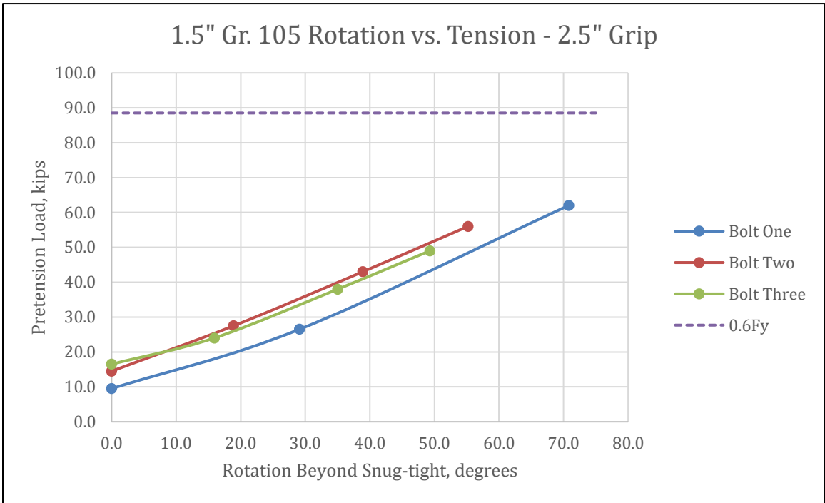
Figure 4-25 - 1.5" Gr. 105 with 2.5" Grip Rotation vs. Tension
