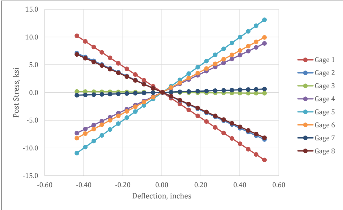
Figure 5-43 - Deflection vs. Stress in the Post
