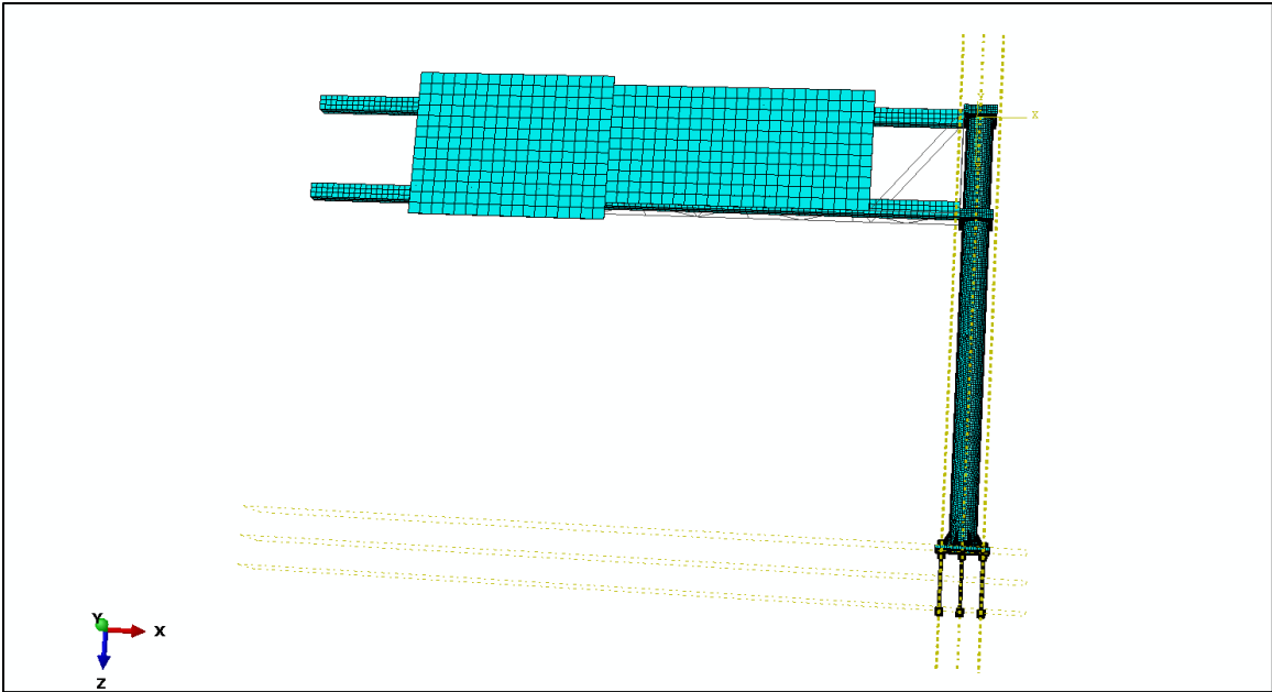
Figure 6-1 - Mesh Generation for Sign Structure
