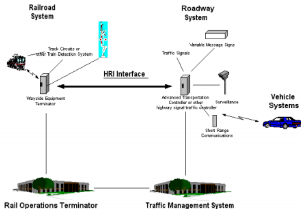
Figure 2. Highway Rail Intersection Interface Overview, IEEE Std 1570-2002 [Error! Bookmark not defined.] .
