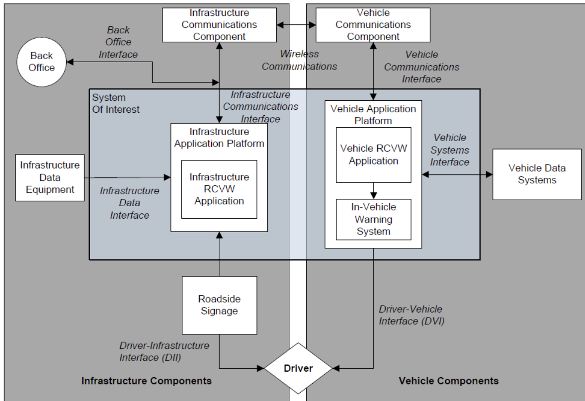
Figure 3. Railroad Crossing Violation Warning Application Diagram [9]
