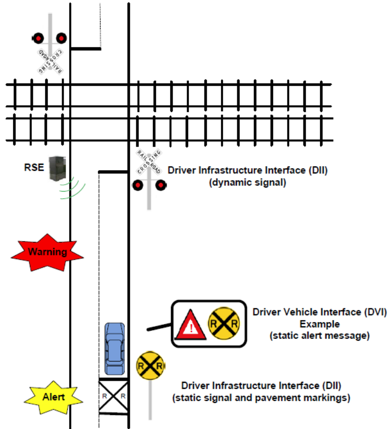
Figure 4. Prior CV Railroad Crossing Violation Warning Layout [9]
