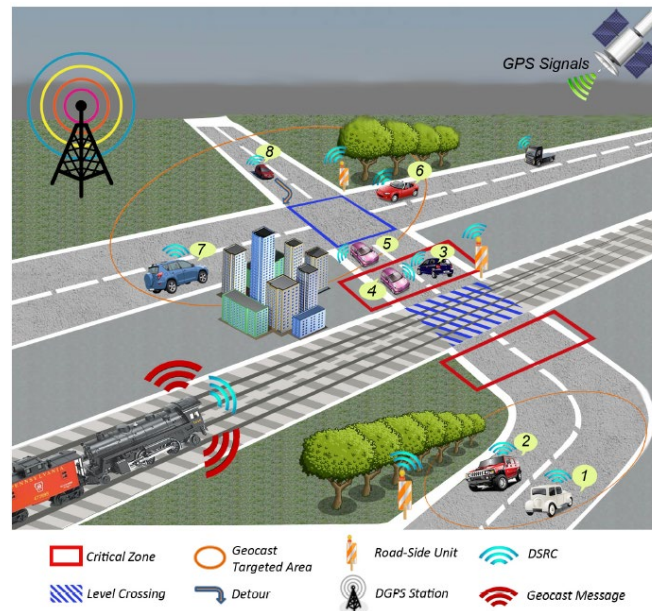
Figure 1. Various Potential Safety Situations at an At-Grade HRGC [4].
