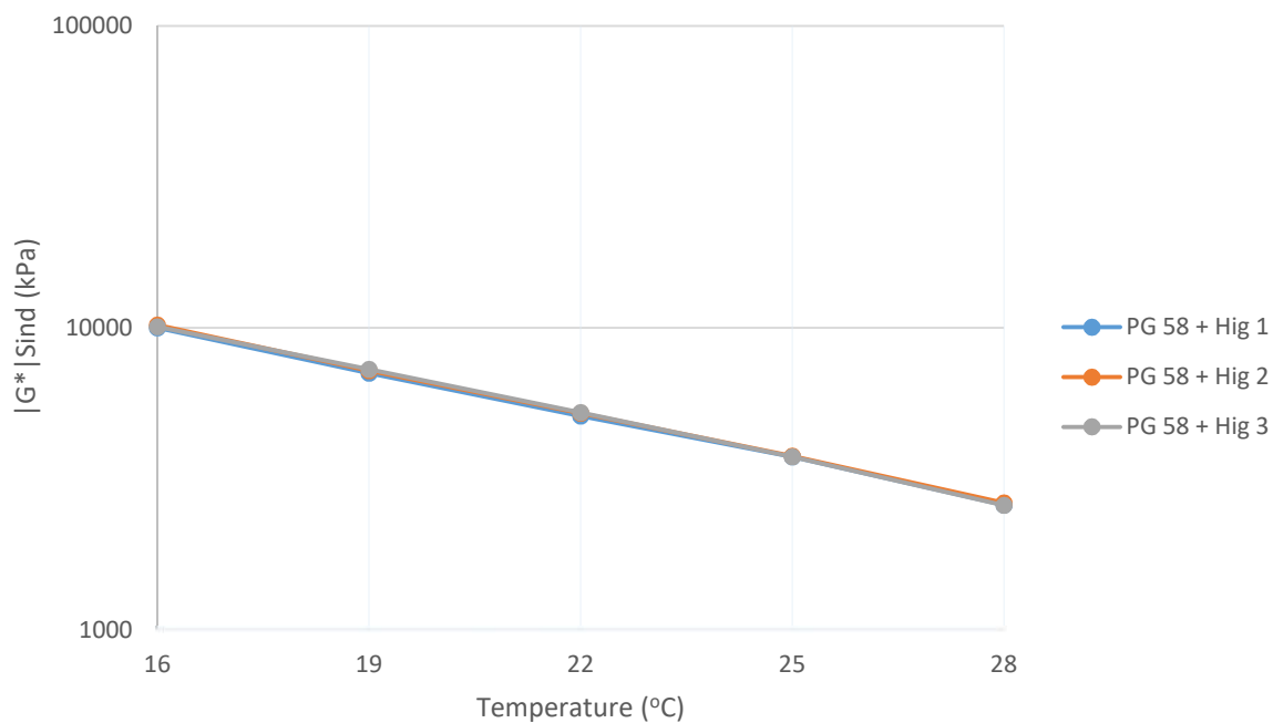
Figure 6-17: DSR Results of PG 58-28 and Highland RAP Binder Blends (PAV Aged)
