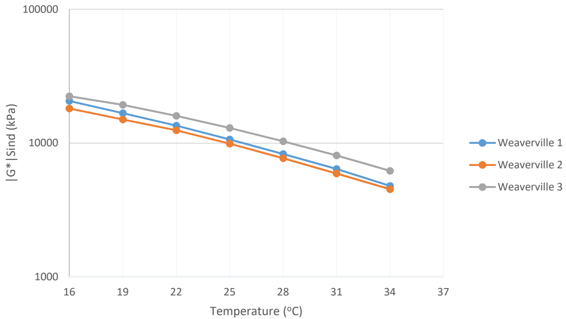
Figure 4-24: DSR Results for the Weaverville RAP Binders (PAV Aged) at Various Temperatures
