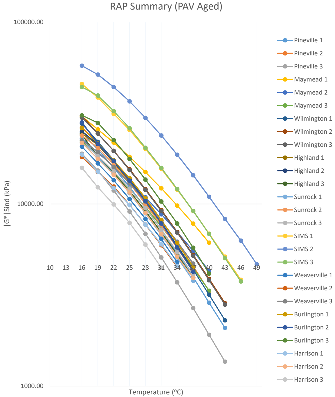
Figure 4-30: DSR Test Results of All RAP Binders in PAV Aged Conditions
