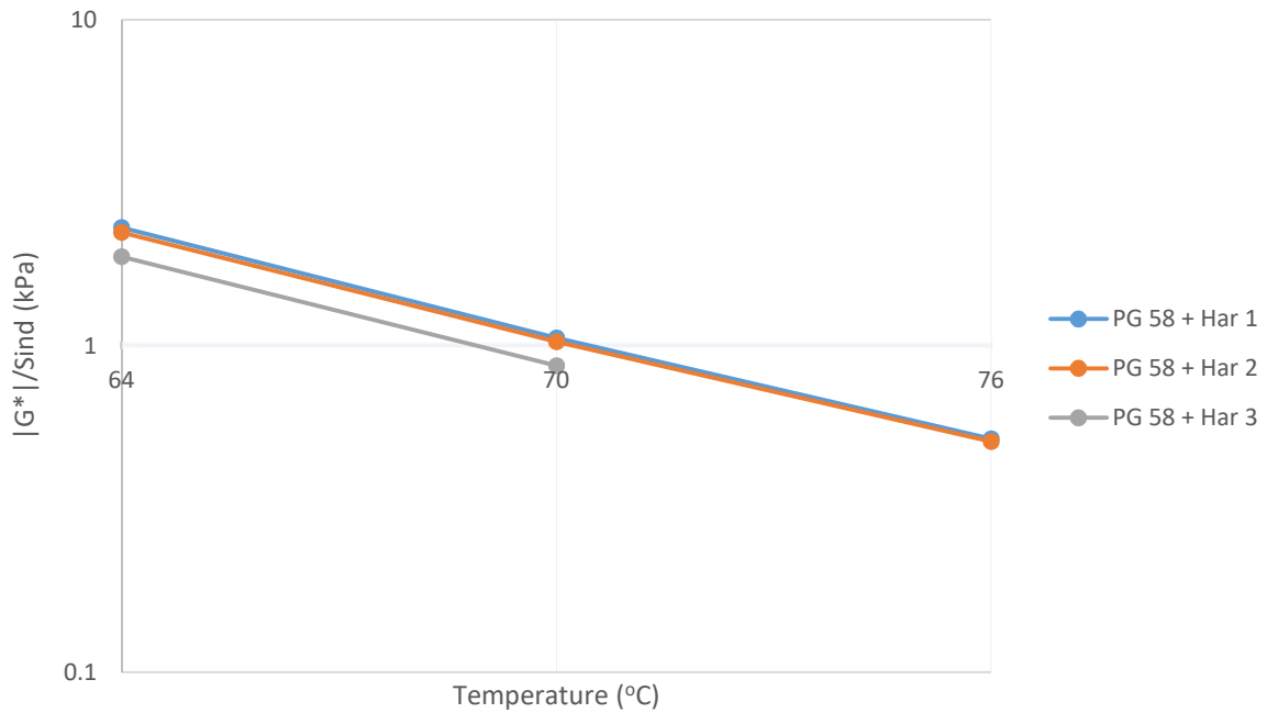
Figure 6-4: DSR Results of PG 58-28 and Harrison RAP Binder Blends (Unaged)
