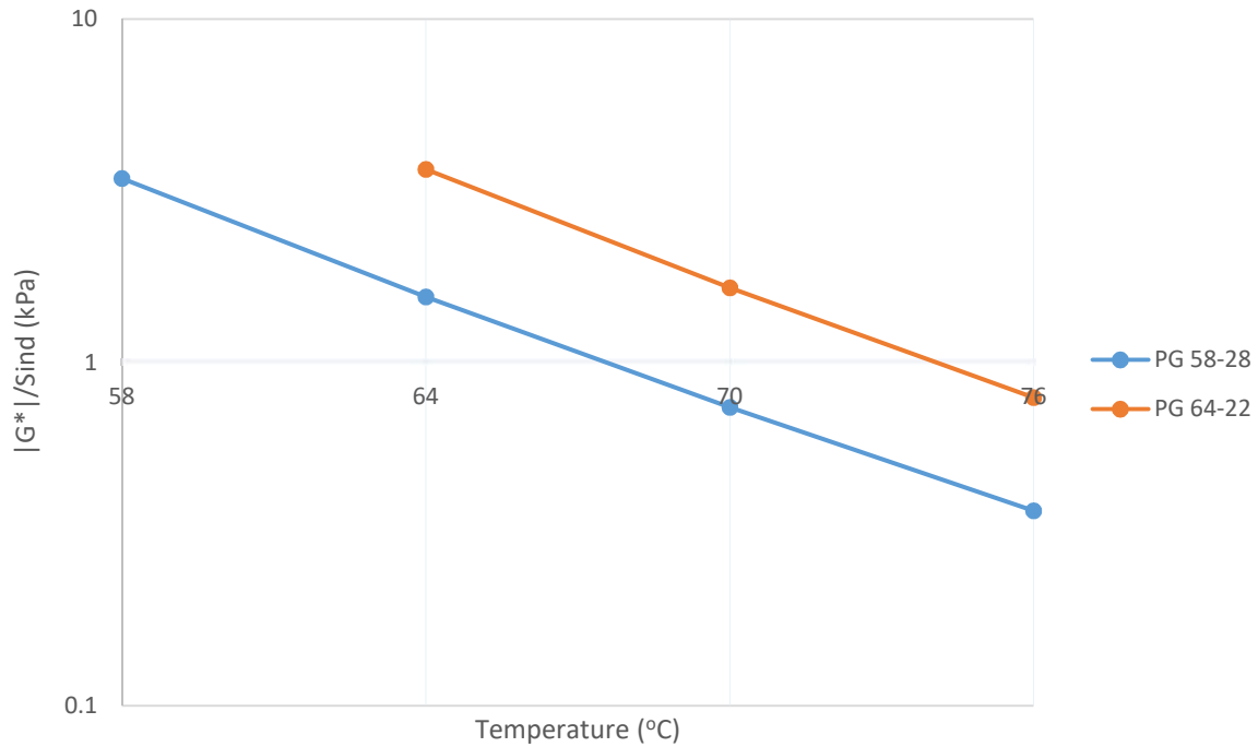
Figure 6-2: DSR Results of Virgin Binders (RTFO Aged)
