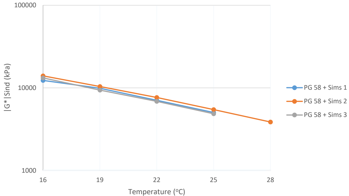
Figure 6-18: DSR Results of PG 58-28 and Sims RAP Binder Blends (PAV Aged)
