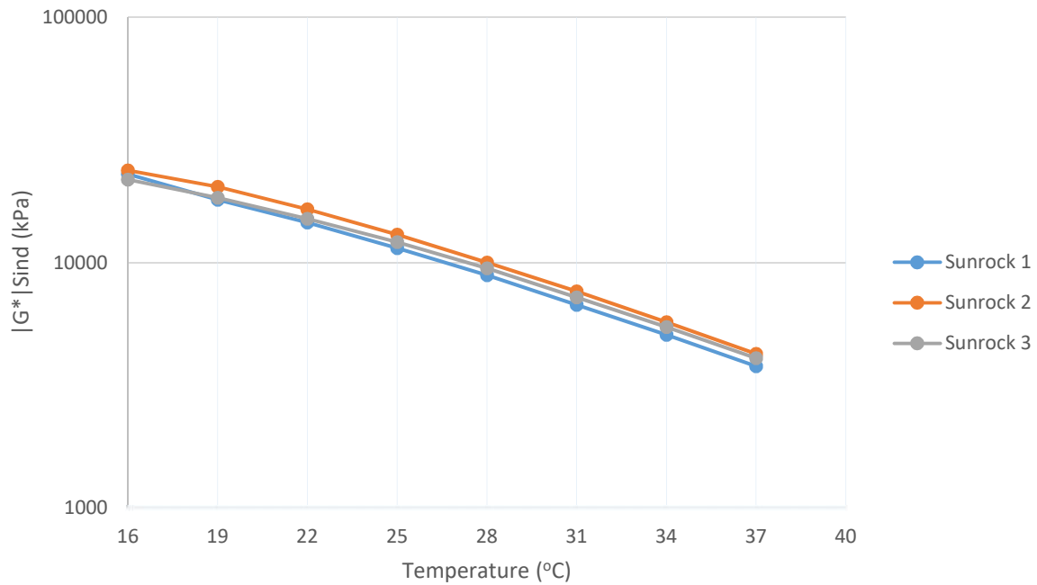
Figure 4-22: DSR Results for the Sunrock RAP Binders (PAV Aged) at Various Temperatures
