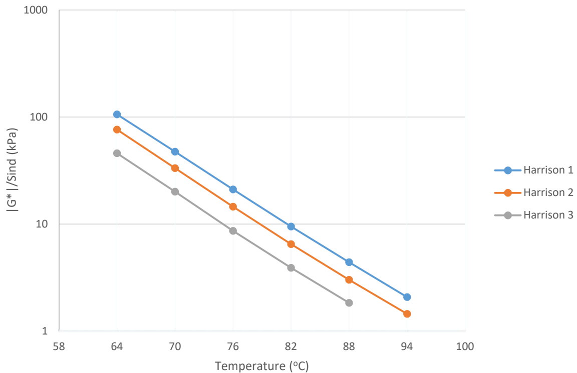
Figure 4-17: DSR Results for the Harrison RAP Binders (RTFO Aged) at Various Temperatures
