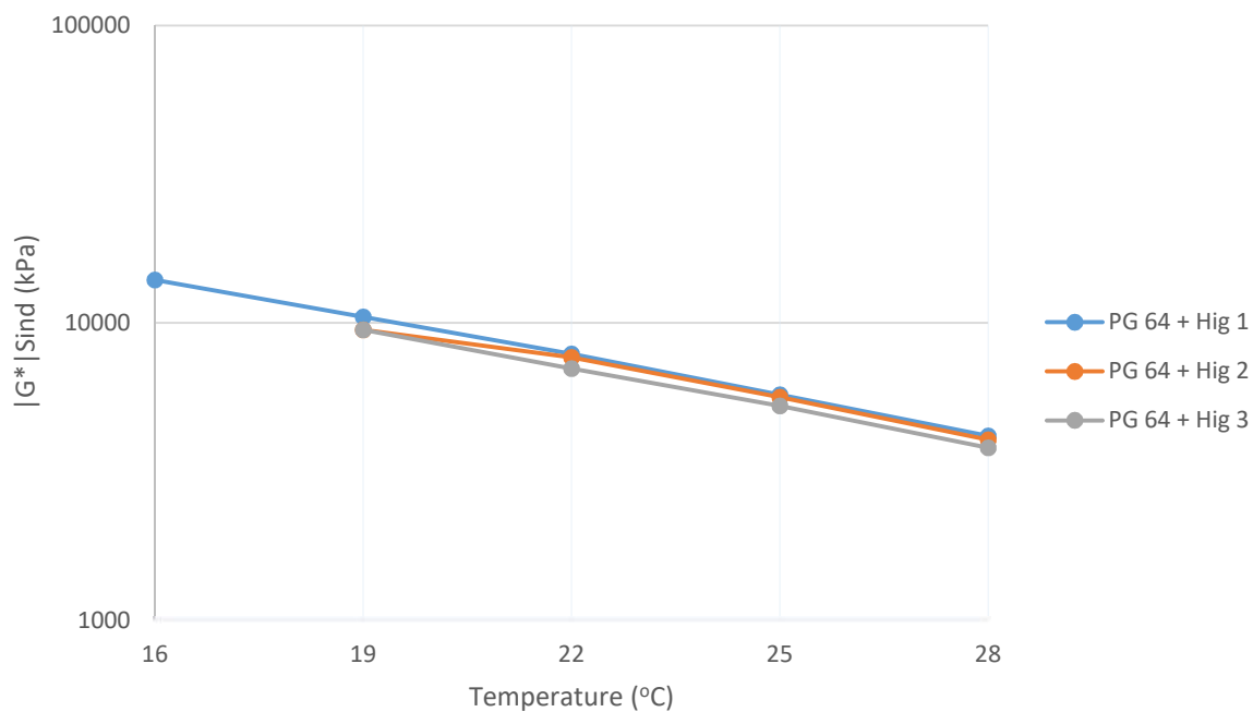
Figure 6-20: DSR Results of PG 64-22 and Highland RAP Binder Blends (PAV Aged)
