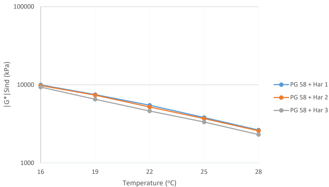
Figure 6-16: DSR Results of PG 58-28 and Harrison RAP Binder Blends (PAV Aged)
