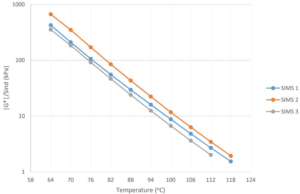
Figure 4-14: DSR Results for the Sims RAP Binders (RTFO Aged) at Various Temperatures
