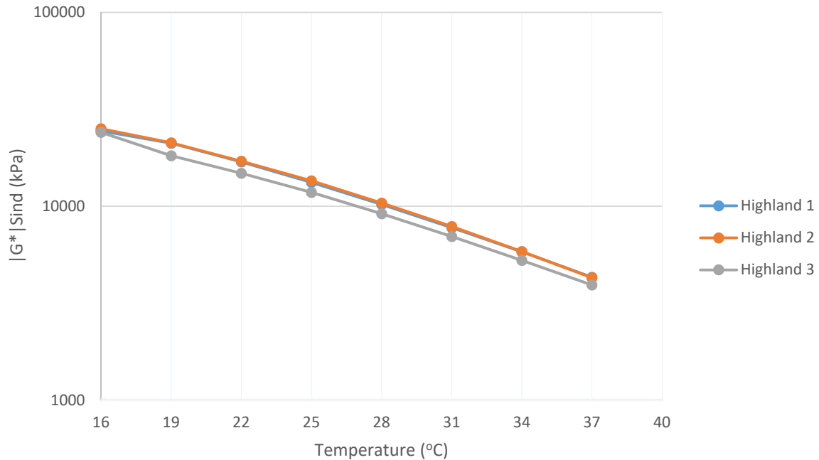
Figure 4-25: DSR Results for the Highland RAP Binders (PAV Aged) at Various Temperatures
