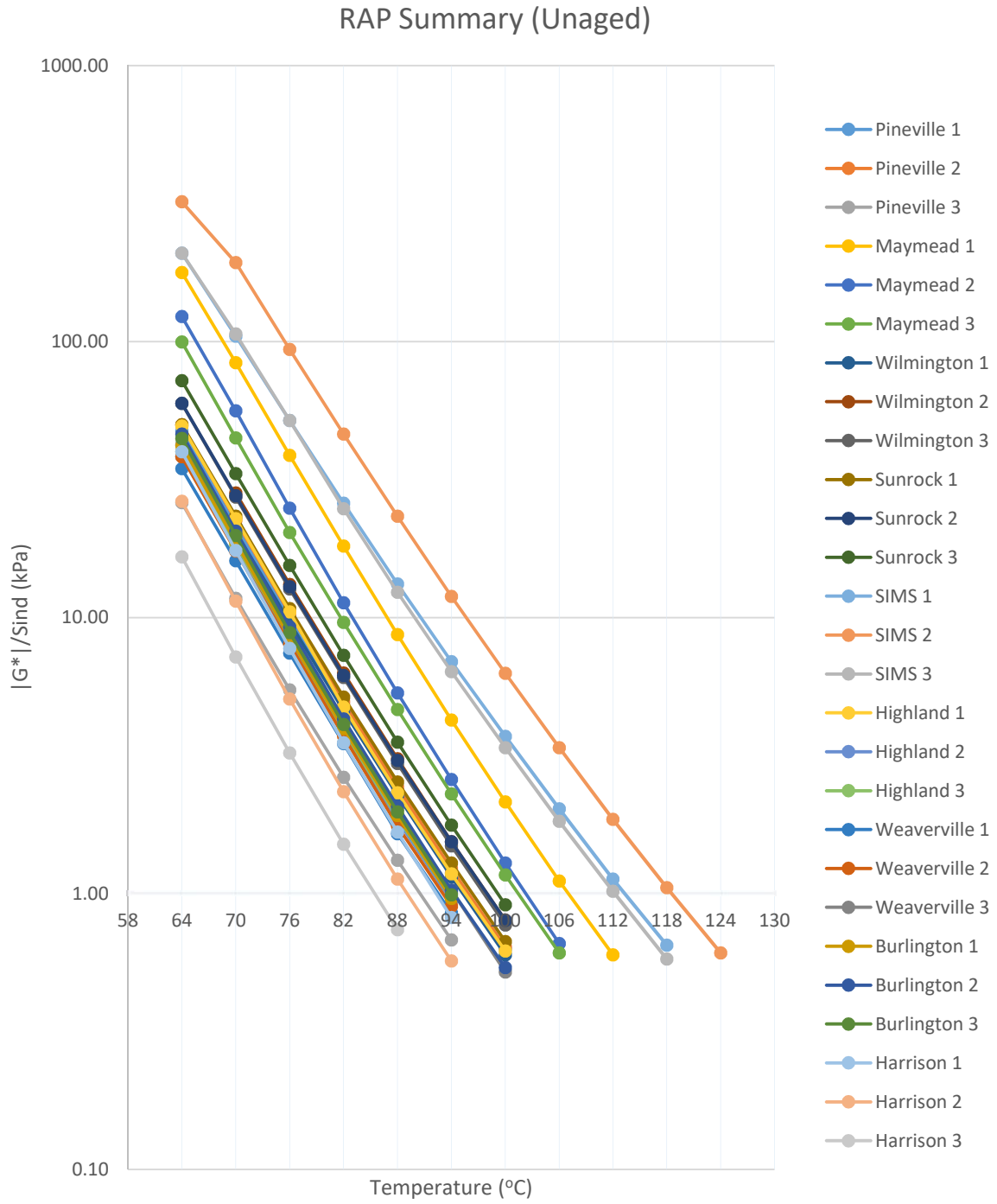
Figure 4-28: DSR Test Results of All RAP Binders in Unaged Conditions
