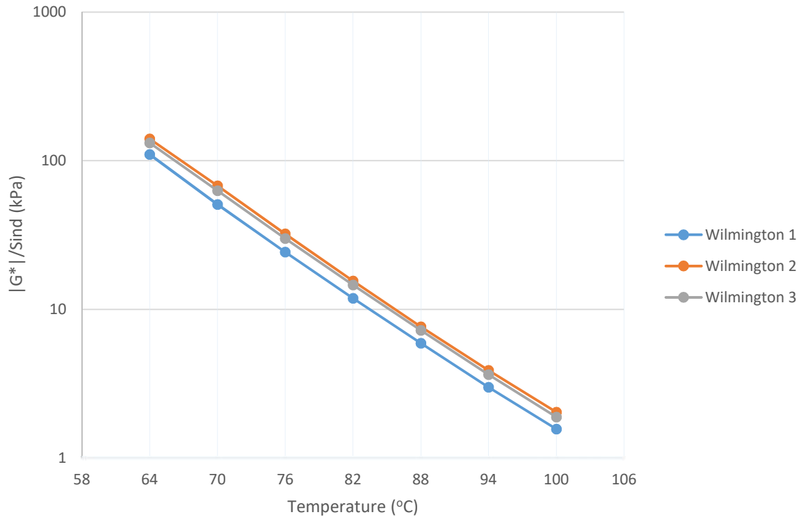
Figure 4-10: DSR Results for the Wilmington RAP Binders (RTFO Aged) at Various Temperatures
