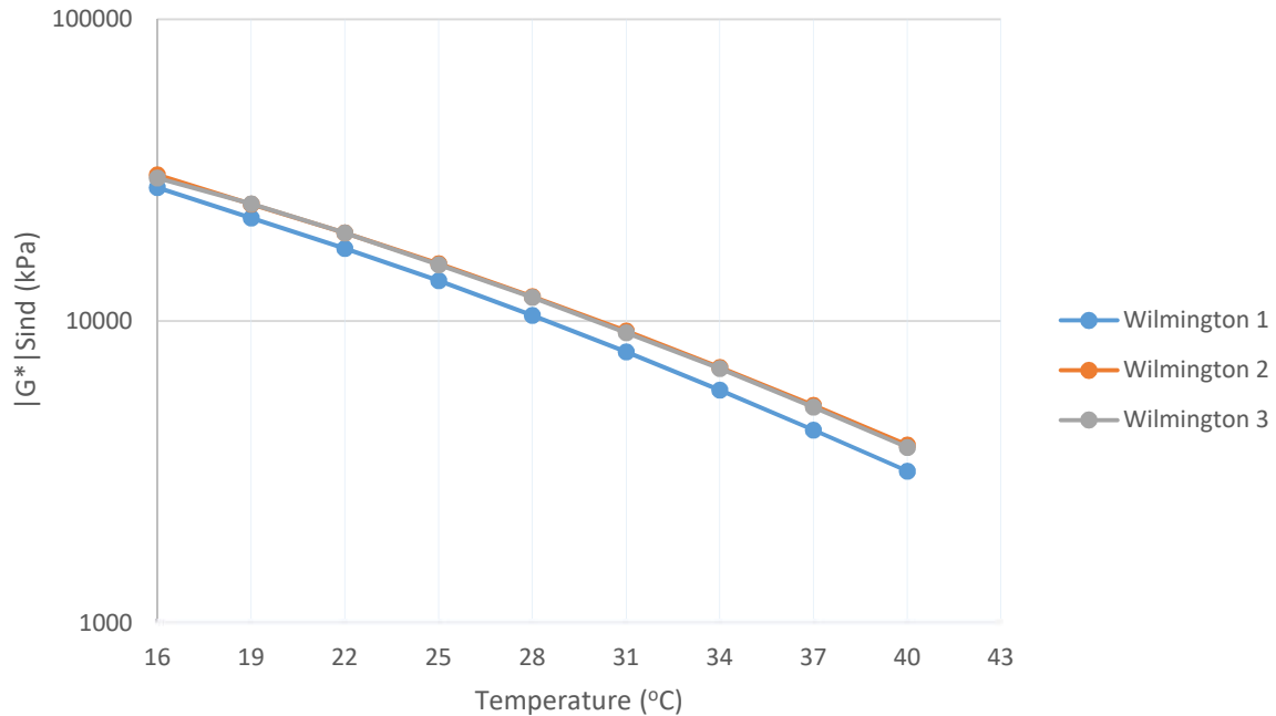
Figure 4-19: DSR Results for the Wilmington RAP Binders (PAV Aged) at Various Temperatures
