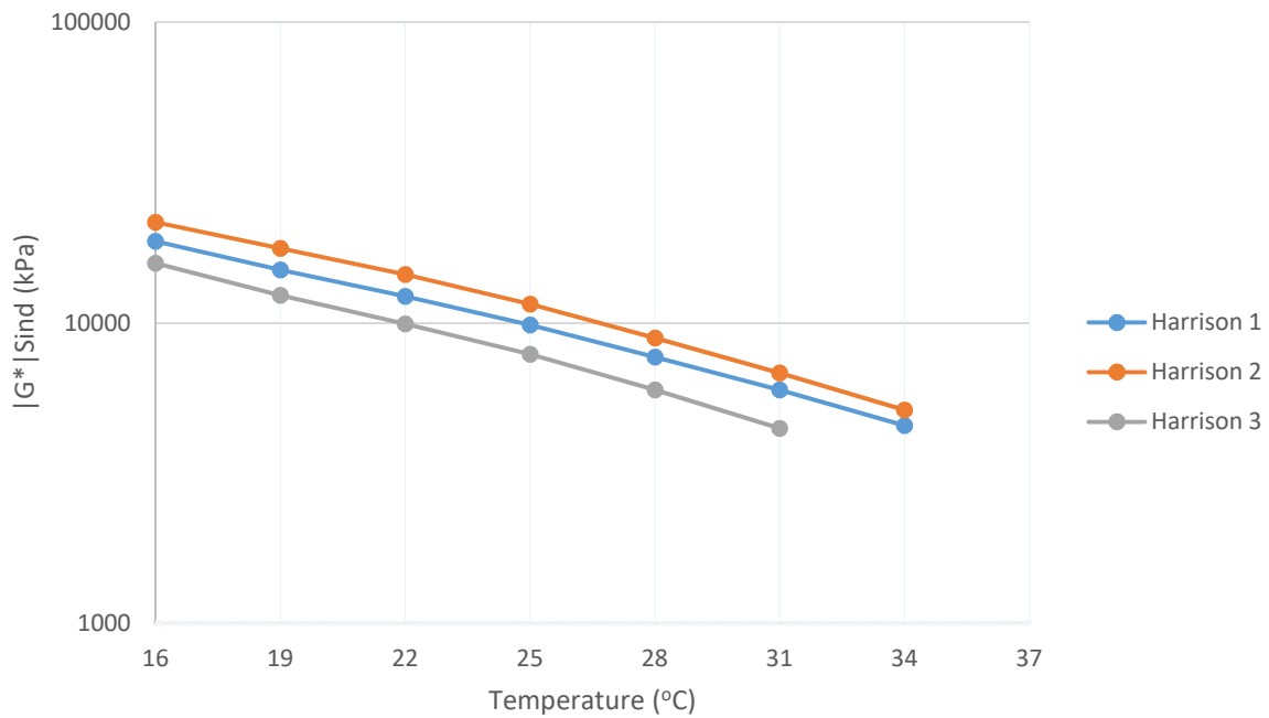
Figure 4-26: DSR Results for the Harrison RAP Binders (PAV Aged) at Various Temperatures
