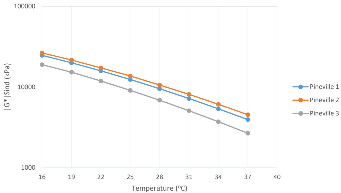
Figure 4-20: DSR Results for the Pineville RAP Binders (PAV Aged) at Various Temperatures
