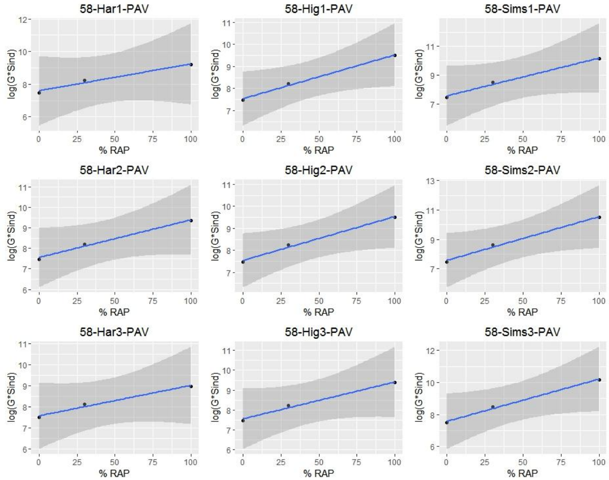
Figure 7-3: Blending Charts for PG 58-28 at 25°C (PAV Aged)
