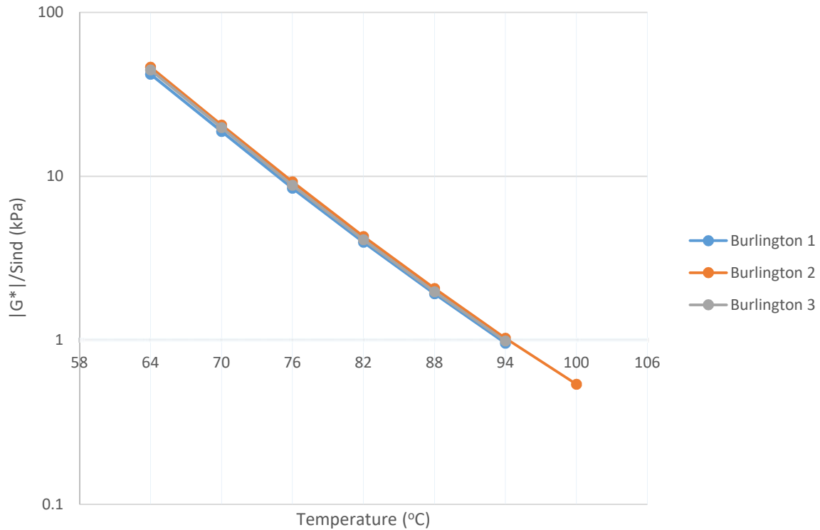
Figure 4-9: DSR Results for the Burlington RAP Binders (Unaged) at Various Temperatures
