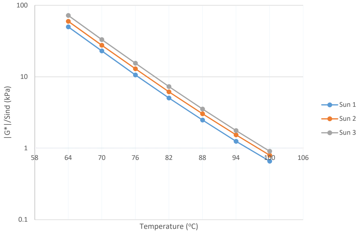
Figure 4-4: DSR Results for the Sunrock RAP Binders (Unaged) at Various Temperatures
