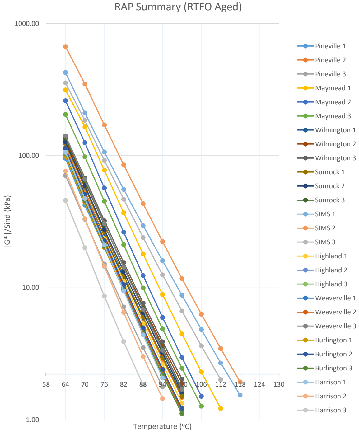
Figure 4-29: DSR Test Results of All RAP Binders in RTFO Aged Conditions
