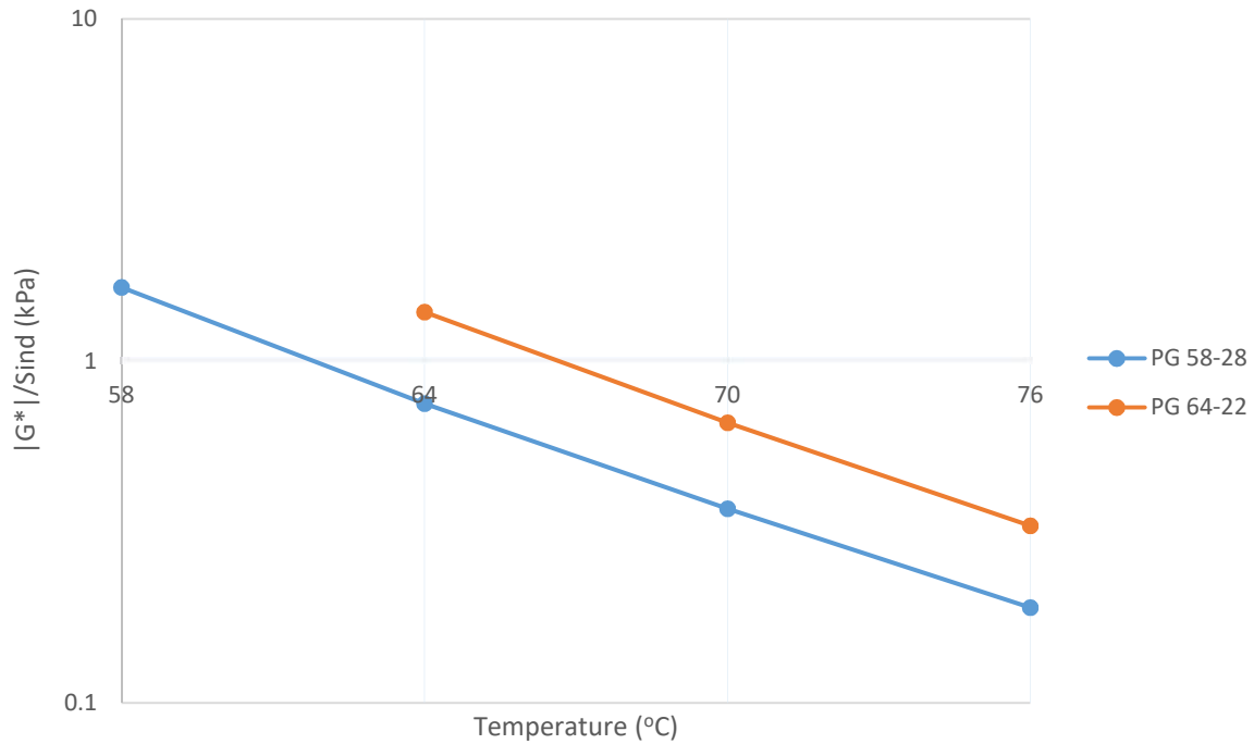
Figure 6-1: DSR Results of Virgin Binders (Unaged)
