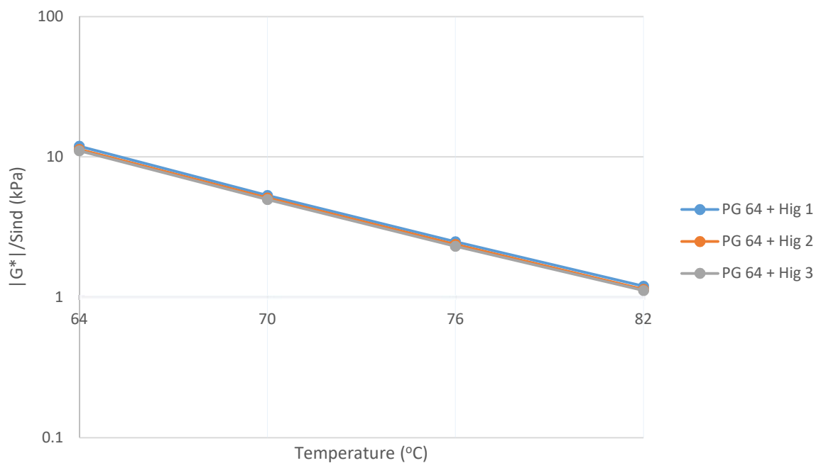
Figure 6-14: DSR Results of PG 64-22 and Highland RAP Binder Blends (RTFO Aged)
