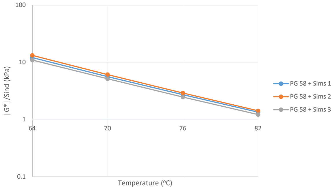
Figure 6-12: DSR Results of PG 58-28 and Sims RAP Binder Blends (RTFO Aged)
