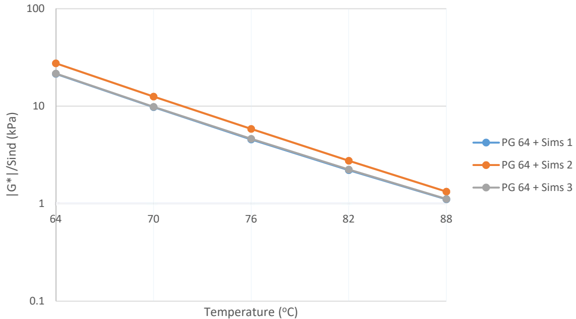
Figure 6-15: DSR Results of PG 64-22 and Sims RAP Binder Blends (RTFO Aged)
