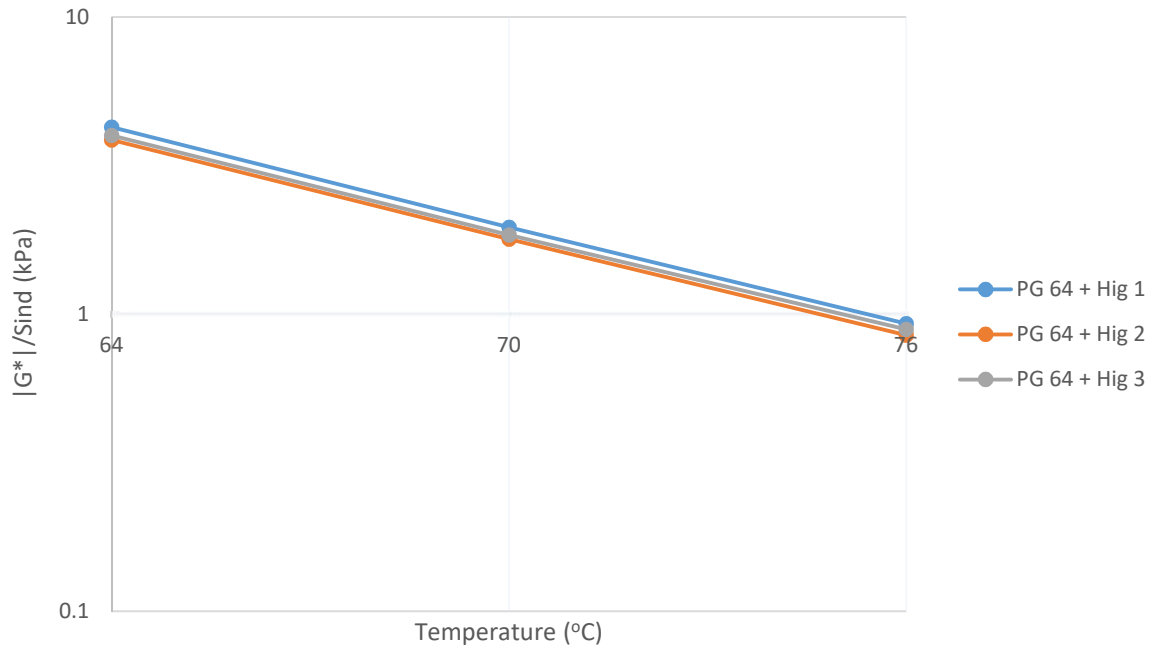
Figure 6-8: DSR Results of PG 64-22 and Highland RAP Binder Blends (Unaged)
