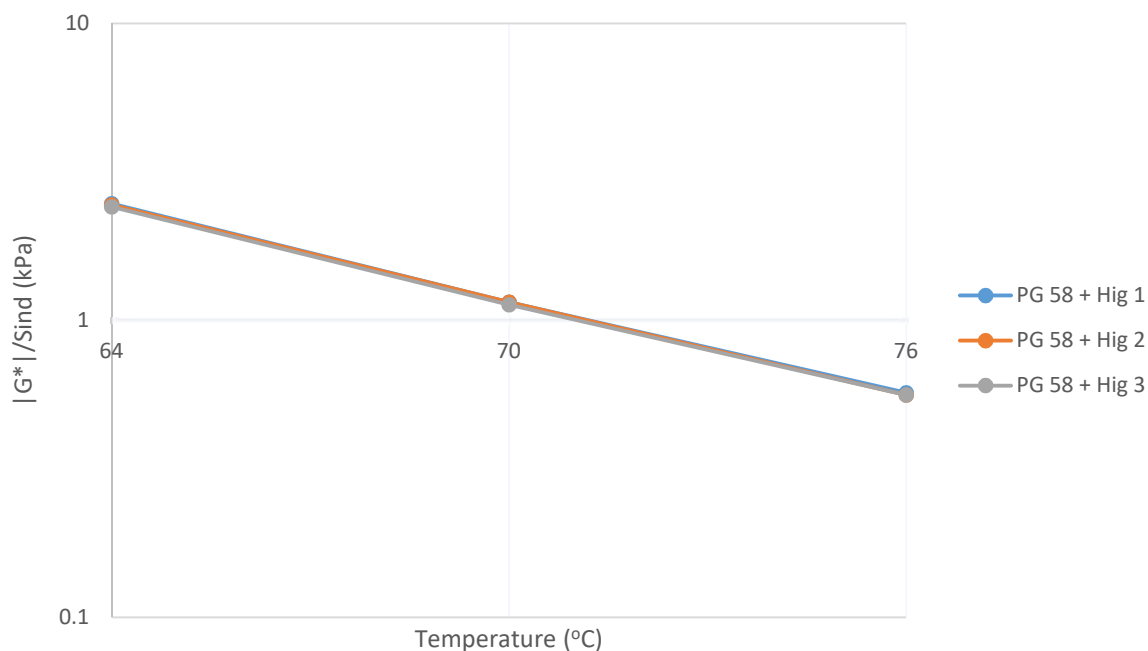
Figure 6-5: DSR Results of PG 58-28 and Highland RAP Binder Blends (Unaged)
