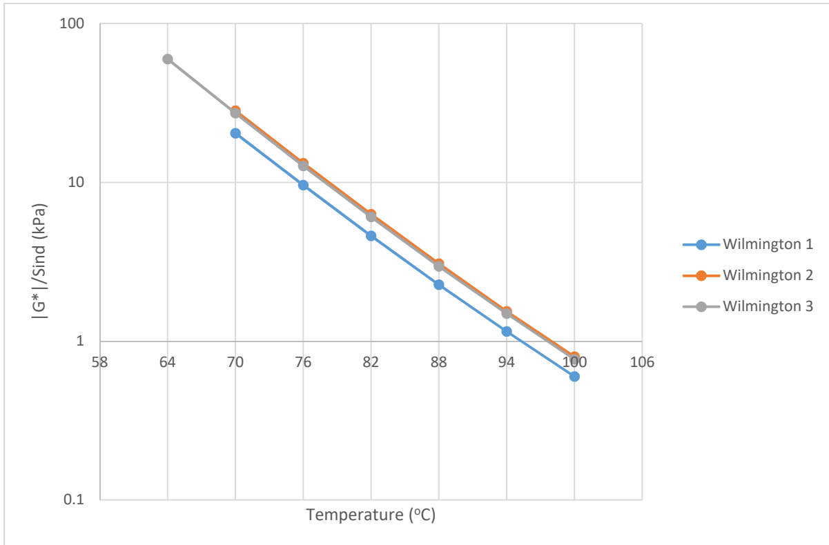
Figure 4-1: DSR Results for the Wilmington RAP Binders (Unaged) at Various Temperatures
