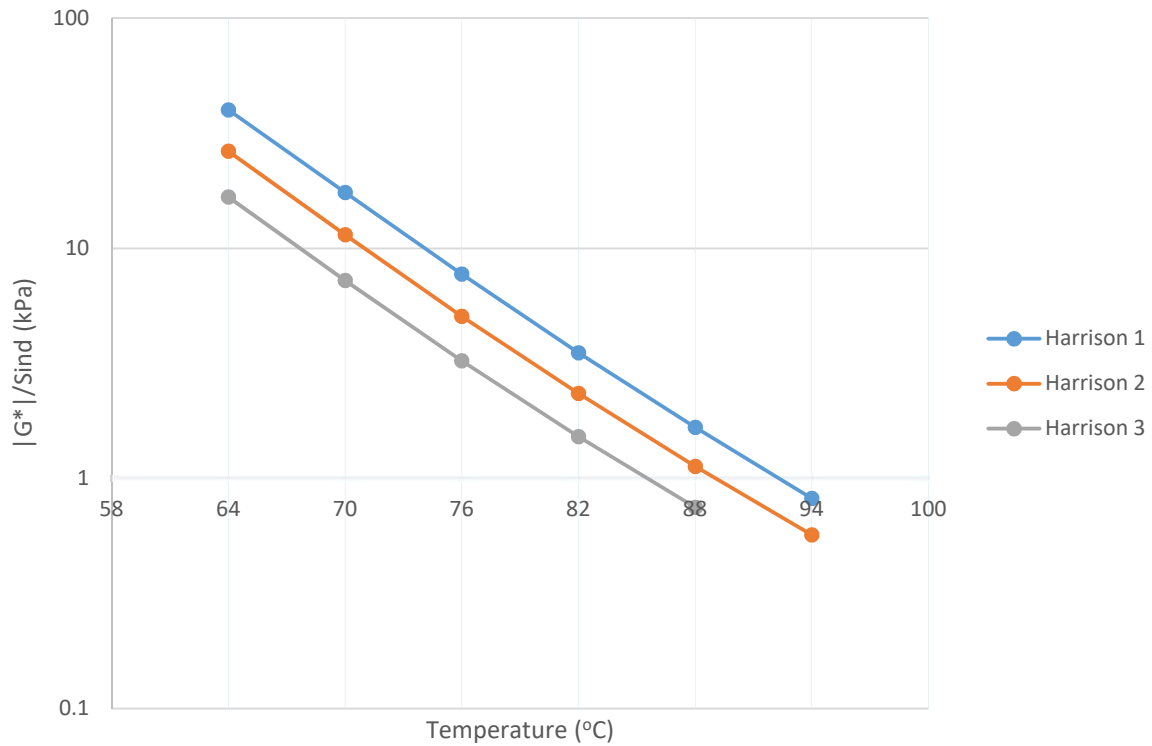
Figure 4-8: DSR Results for the Harrison RAP Binders (Unaged) at Various Temperatures
