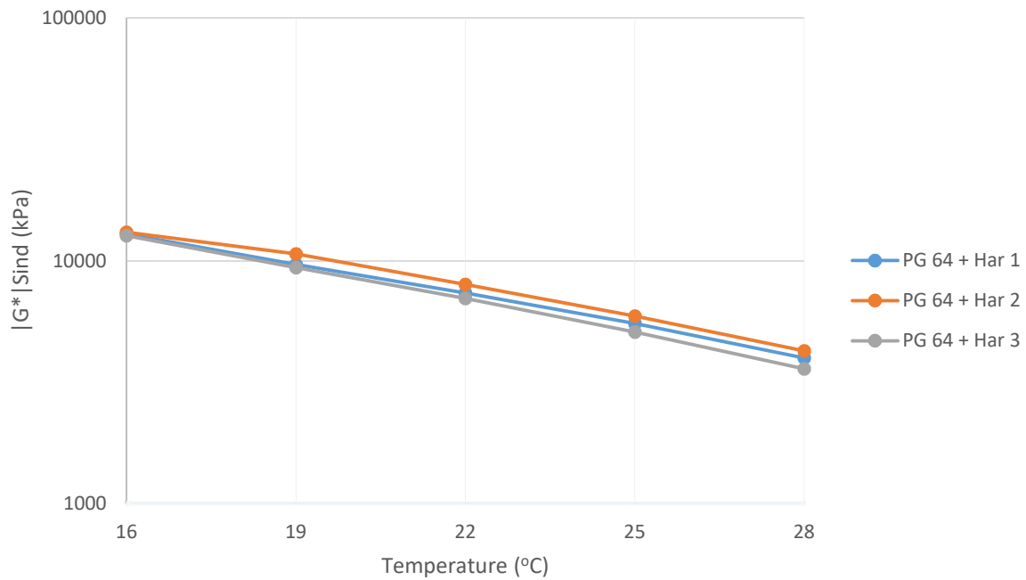
Figure 6-19: DSR Results of PG 64-22 and Harrison RAP Binder Blends (PAV Aged)
