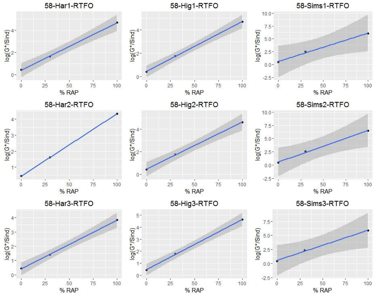
Figure 7-2: Blending Charts for PG 58-28 at 64°C (RTFO Aged)
