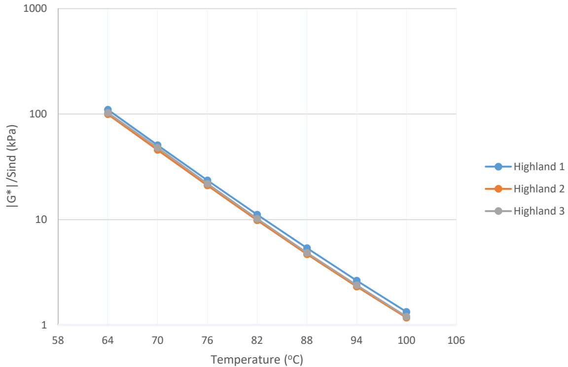
Figure 4-16: DSR Results for the Highland RAP Binders (RTFO Aged) at Various Temperatures
