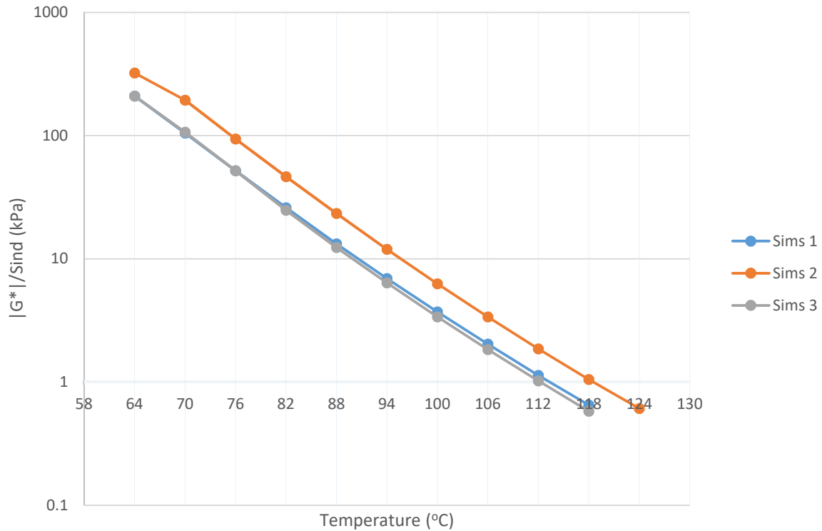
Figure 4-5: DSR Results for the Sims RAP Binders (Unaged) at Various Temperatures
