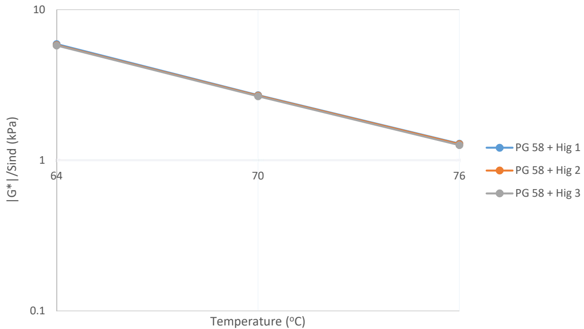
Figure 6-11: DSR Results of PG 58-28 and Highland RAP Binder Blends (RTFO Aged)
