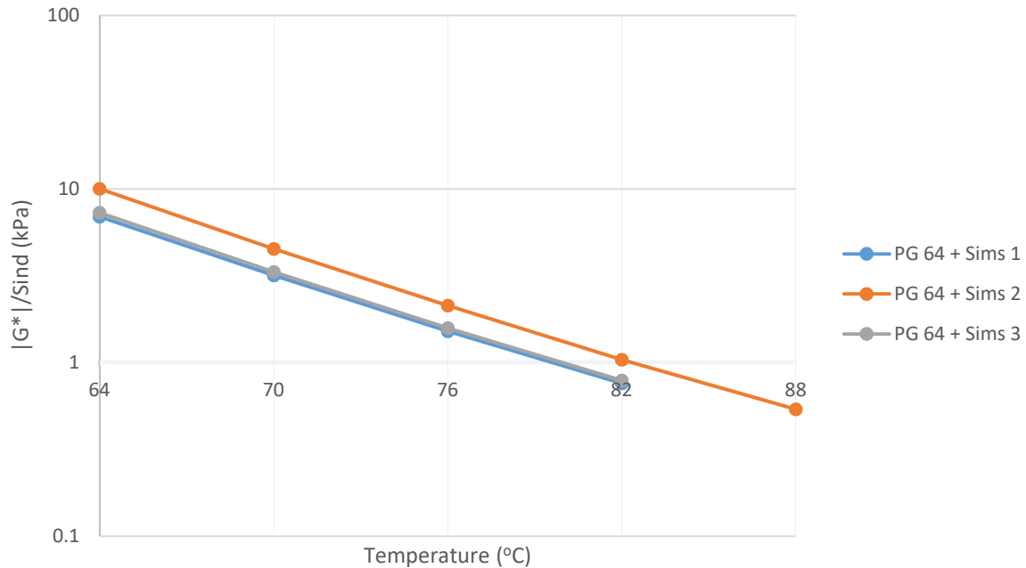
Figure 6-9: DSR Results of PG 64-22 and Sims RAP Binder Blends (Unaged)
