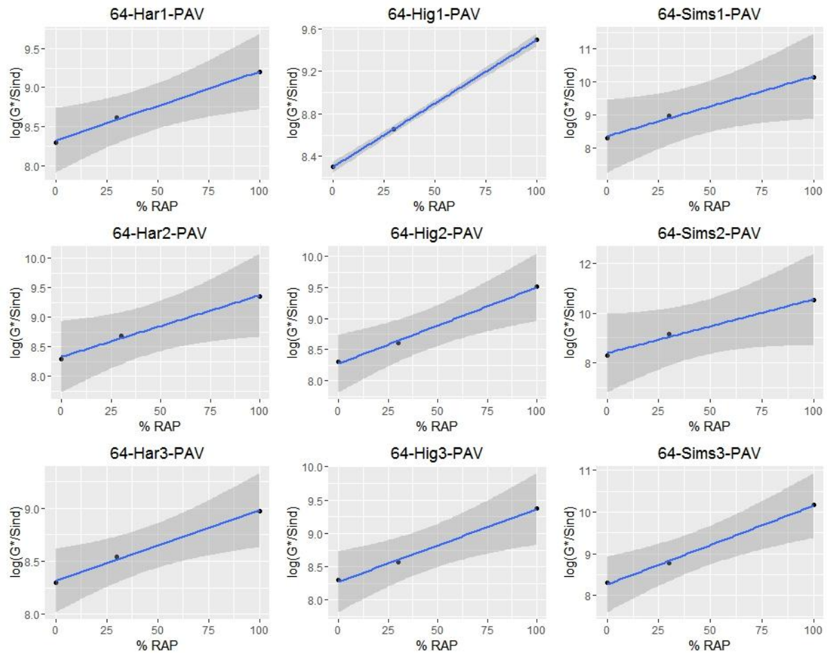
Figure 7-4: Blending Charts for PG 64-22 at 25°C (PAV Aged)
