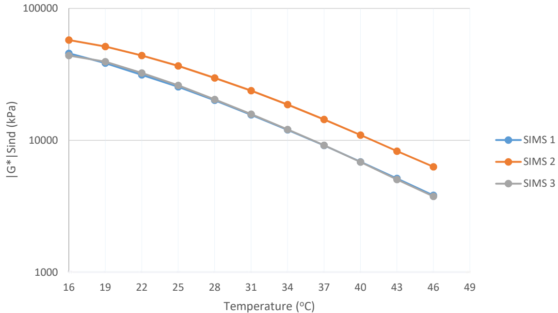
Figure 4-23: DSR Results for the Sims RAP Binders (PAV Aged) at Various Temperatures
