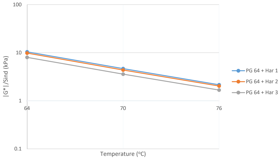
Figure 6-13: DSR Results of PG 64-22 and Harrison RAP Binder Blends (RTFO Aged)
