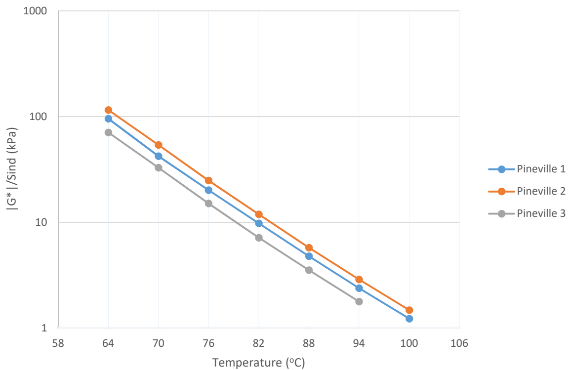
Figure 4-11: DSR Results for the Pineville RAP Binders (RTFO Aged) at Various Temperatures
