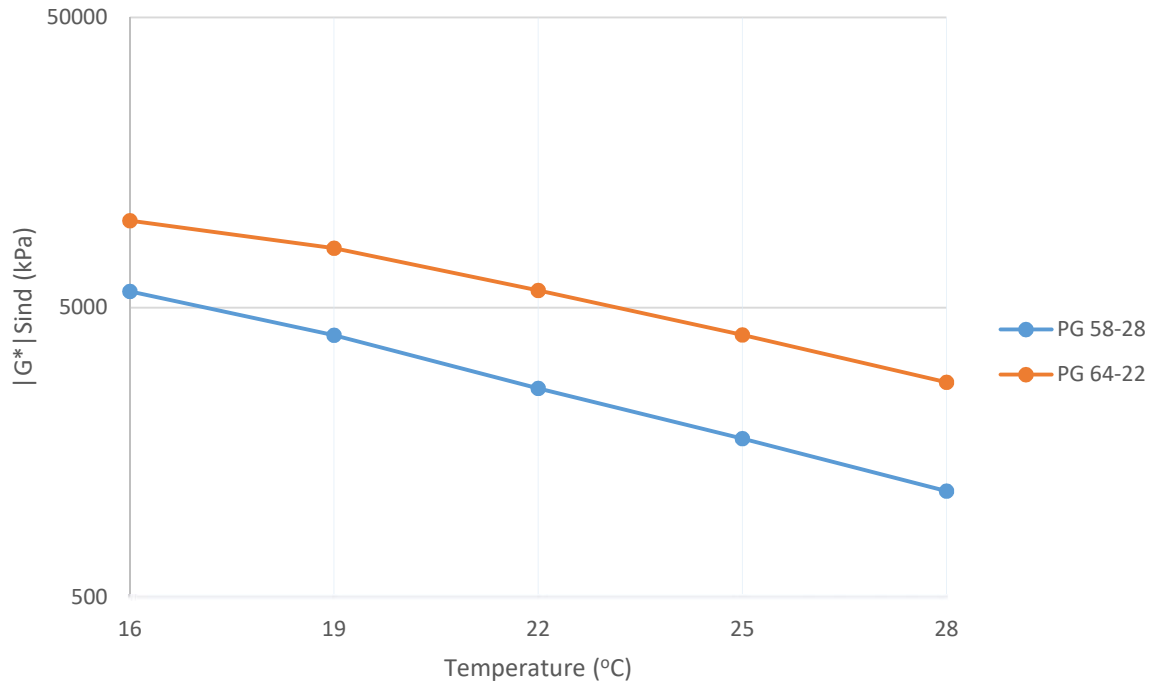
Figure 6-3: DSR Results of Virgin Binders (PAV Aged)
