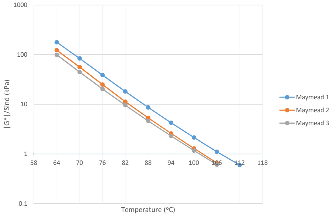
Figure 4-3: DSR Results for the Maymead RAP Binders (Unaged) at Various Temperatures
