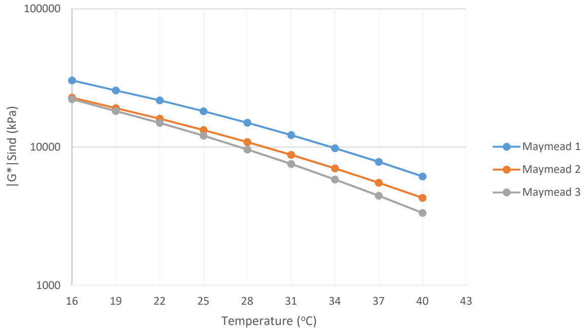
Figure 4-21: DSR Results for the Maymead RAP Binders (PAV Aged) at Various Temperatures
