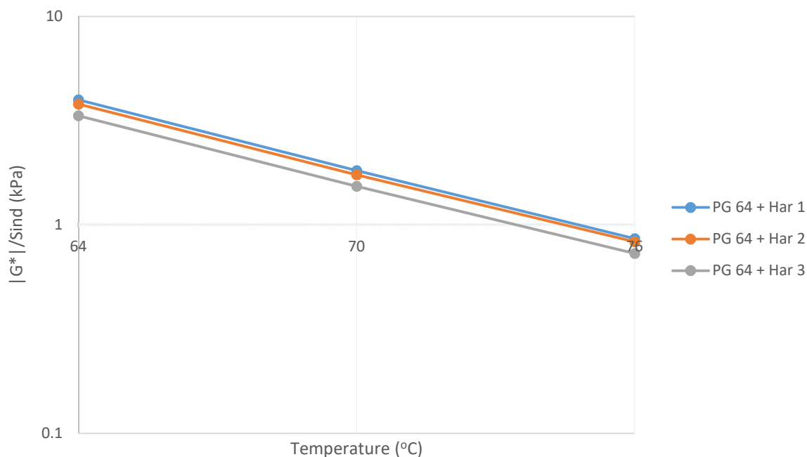
Figure 6-7: DSR Results of PG 64-22 and Harrison RAP Binder Blends (Unaged)
