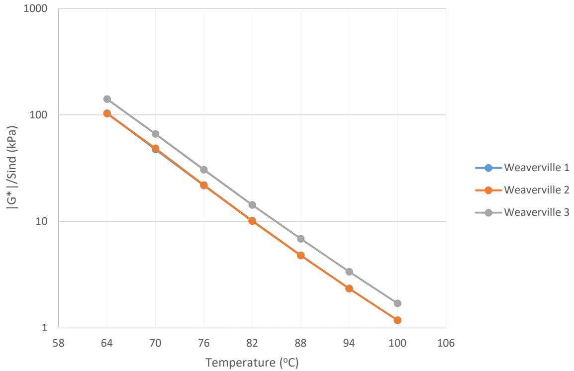
Figure 4-15: DSR Results for the Weaverville RAP Binders (RTFO Aged) at Various Temperatures
