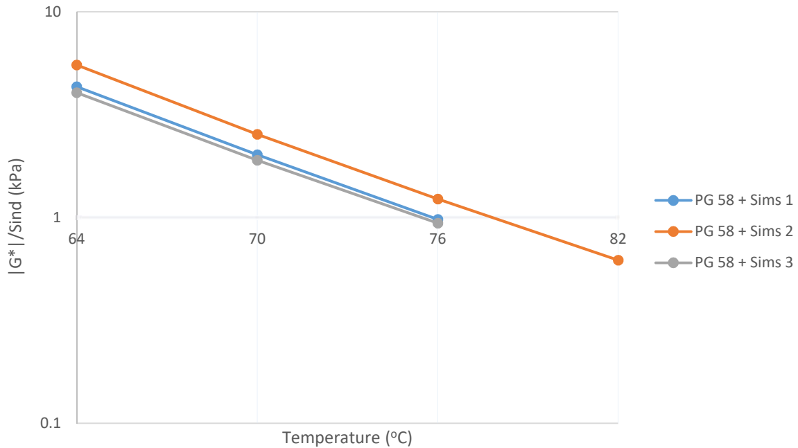
Figure 6-6: DSR Results of PG 58-28 and Sims RAP Binder Blends (Unaged)
