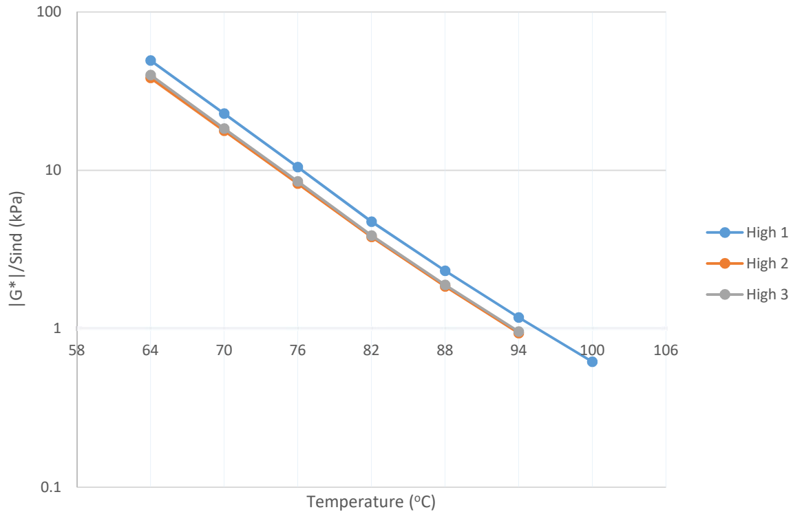
Figure 4-7: DSR Results for the Highland RAP Binders (Unaged) at Various Temperatures
