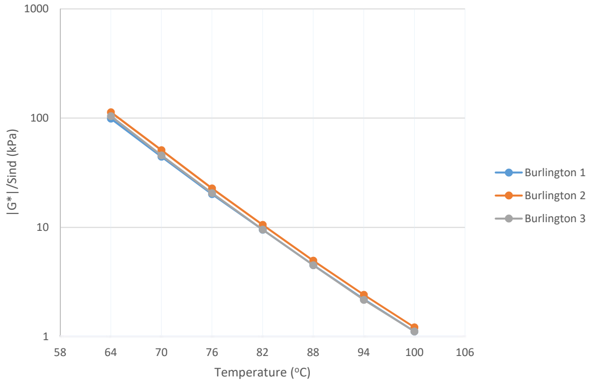
Figure 4-18: DSR Results for the Burlington RAP Binders (RTFO Aged) at Various Temperatures
