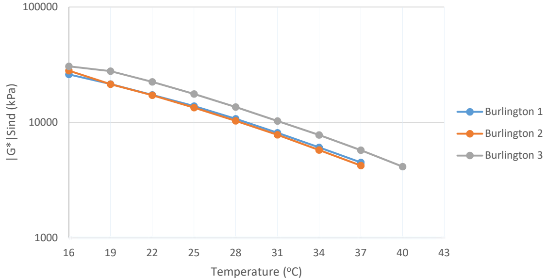
Figure 4-27: DSR Results for the Burlington RAP Binders (PAV Aged) at Various Temperatures
