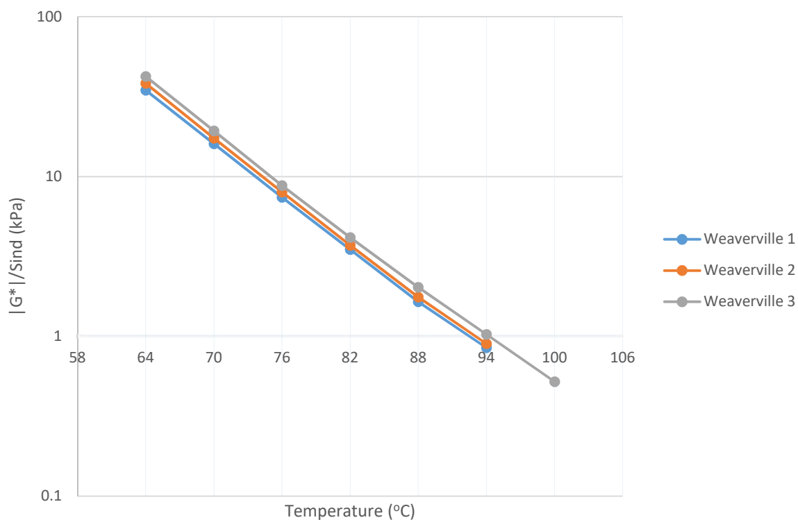
Figure 4-6: DSR Results for the Weaverville RAP Binders (Unaged) at Various Temperatures
