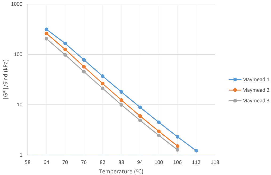
Figure 4-12: DSR Results for the Maymead RAP Binders (RTFO Aged) at Various Temperatures
