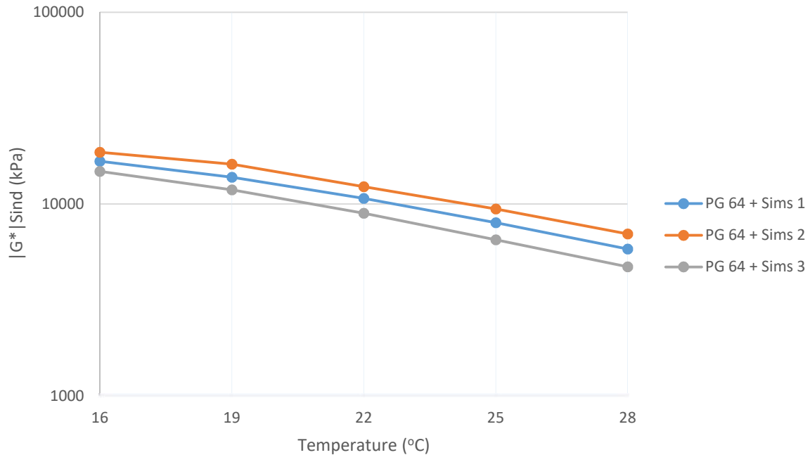
Figure 6-21: DSR Results of PG 64-22 and Sims RAP Binder Blends (PAV Aged)
