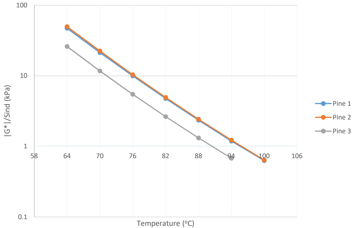
Figure 4-2: DSR Results for the Pineville RAP Binders (Unaged) at Various Temperatures
