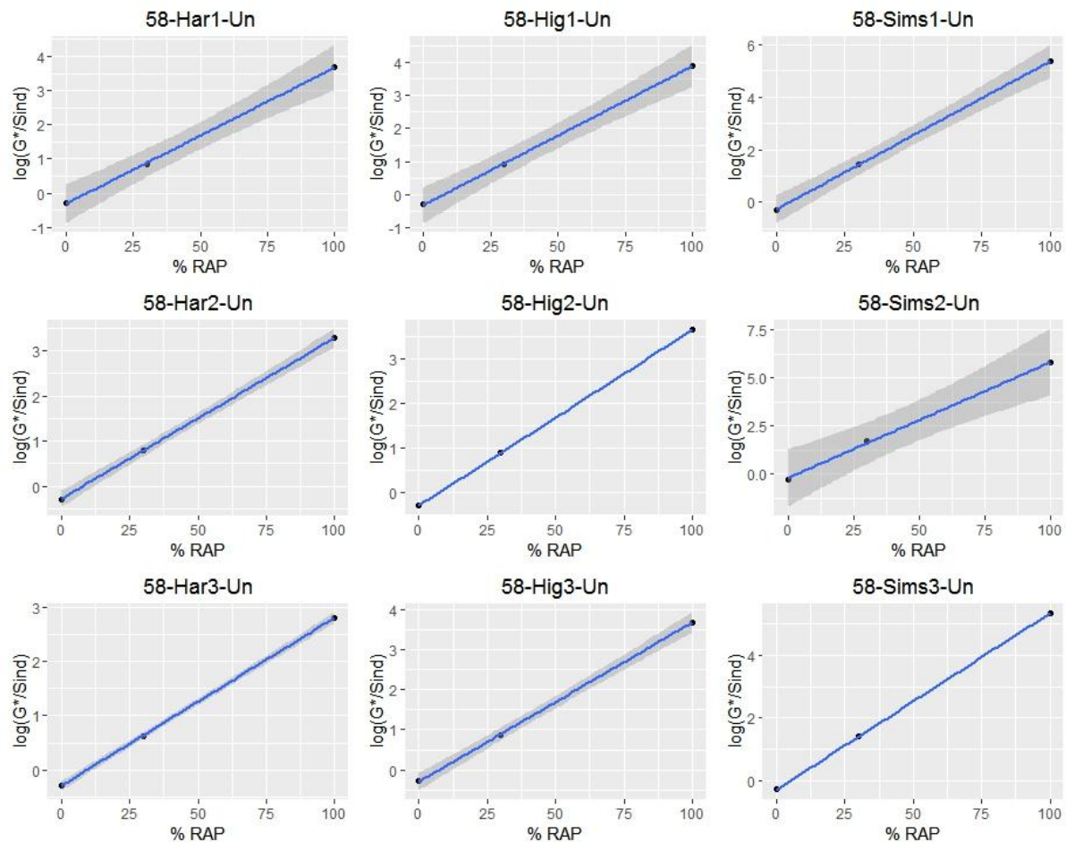
Figure 7-1: Blending Charts for PG 58-28 at 64°C (Unaged)
