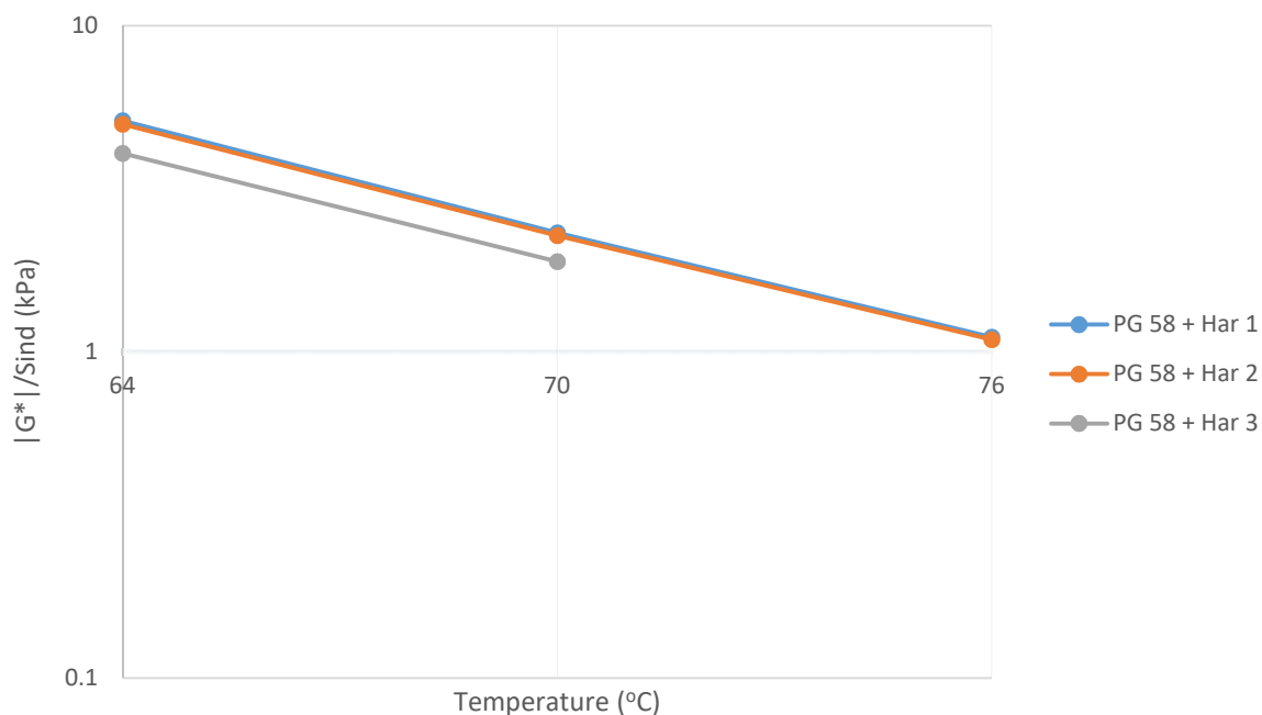
Figure 6-10: DSR Results of PG 58-28 and Harrison RAP Binder Blends (RTFO Aged)
