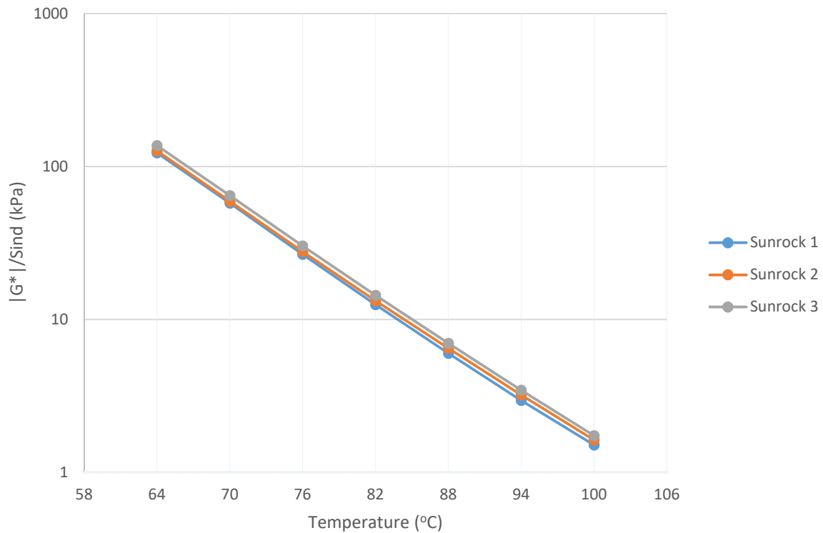
Figure 4-13: DSR Results for the Sunrock RAP Binders (RTFO Aged) at Various Temperatures
