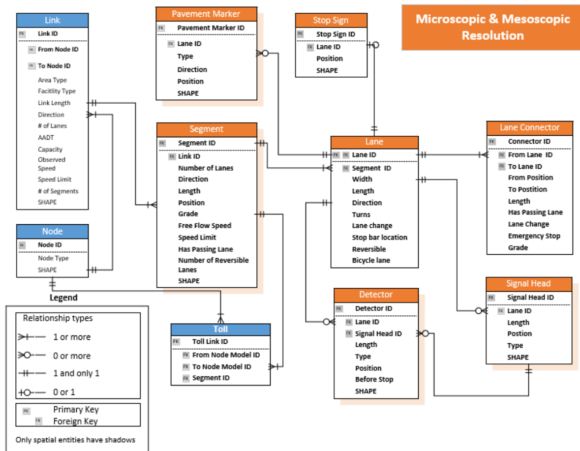
Figure 4-2 ER Diagram of the Microscopic/Mesoscopic Resolution Modeling
