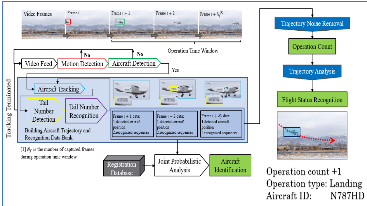
Figure 3.2 System flowchart
