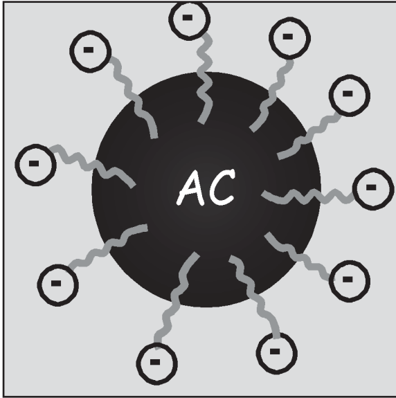
Figure 3.3.2. Anionic (-) Emulsion
