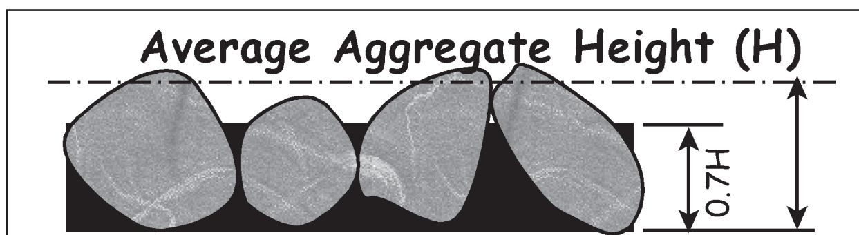
Figure 3.4.2. McLeod design: One-stone thick & proper embedment (70%).
