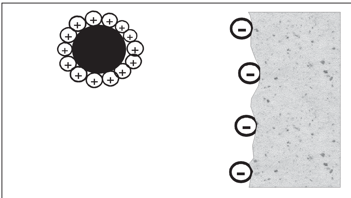
Figure 3.3.4. Cationic Emulsion before breaking
