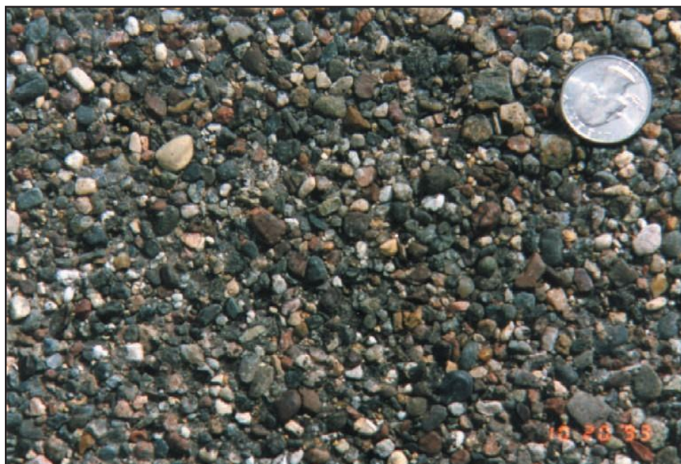
Figure 3.1.1 Example of an FA-2 Pea Rock (buckshot)
