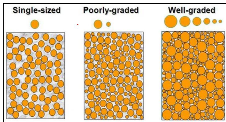
Figure 3.2.3 Aggregate grading
