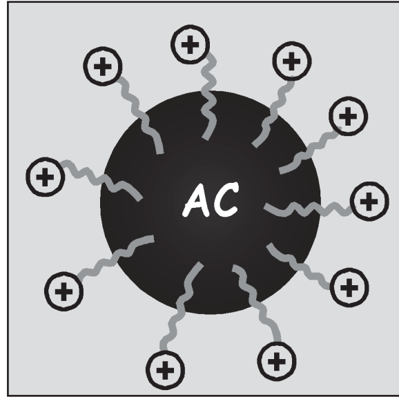
Figure 3.3.3. Cationic (+) Emulsion
