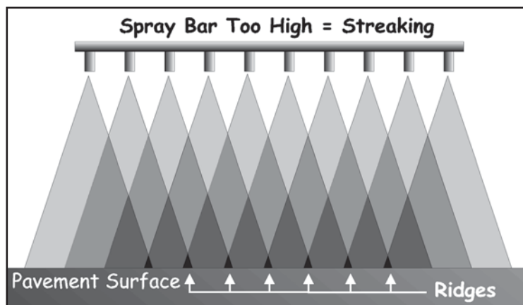
Figure 3.8.10. Spray bar is too high (ridges)
