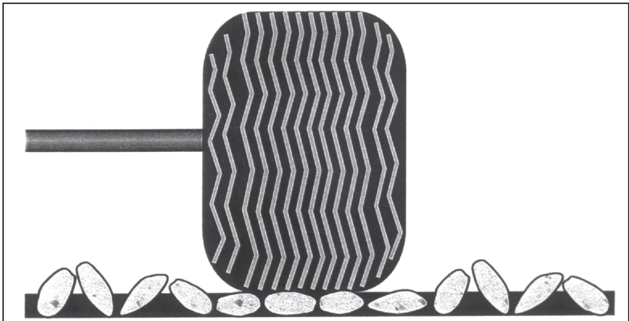
Figure 3.2.1. Traffic causes flat chips in the wheel path to lay down on their flattest side
