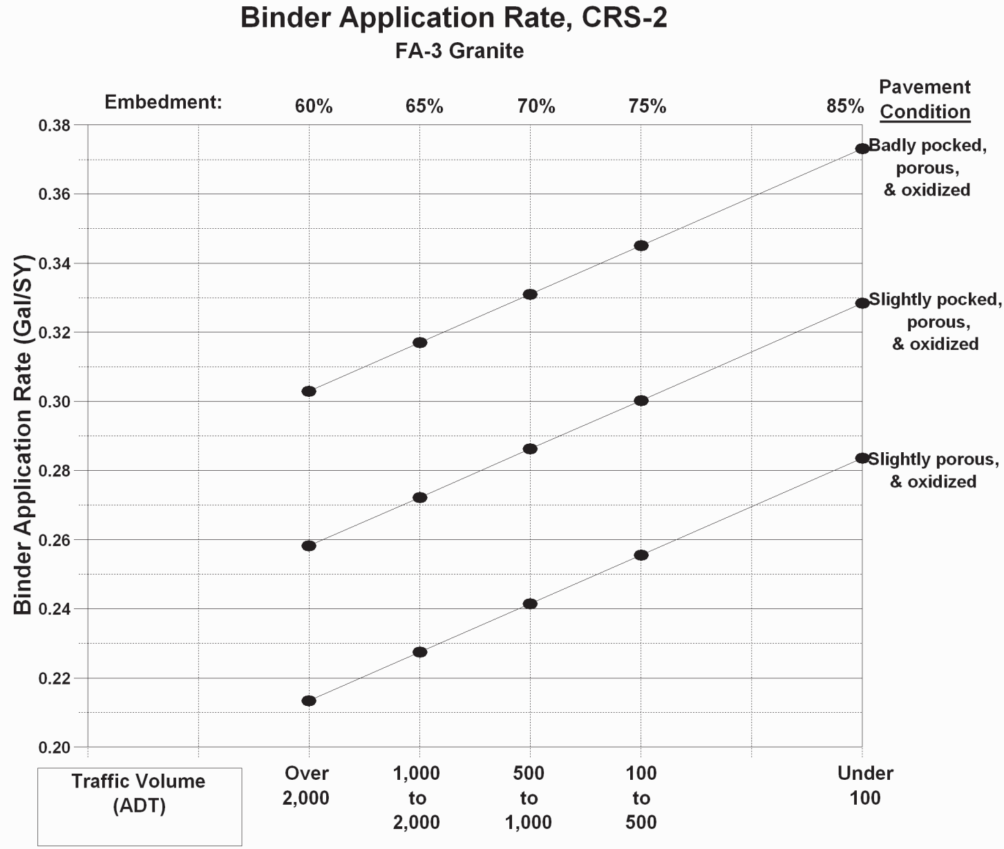
Figure 3.4.12. Example of a Binder Adjustment Chart
