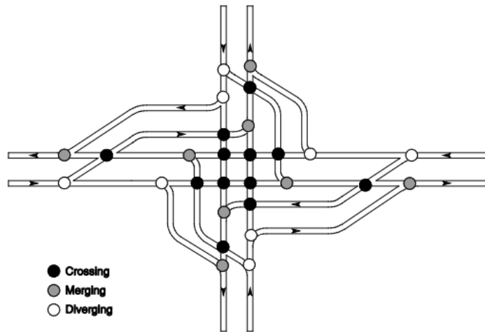
Figure 2-10: Conflict Point Diagram for a DLT Intersection with four DLT Crossovers Source: FHWA, Displaced Left Turn Intersection Informational Guide (2014)
