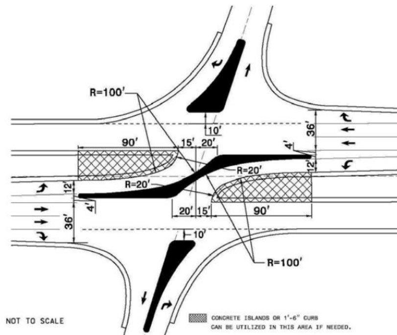
Figure 4-5: Left-turn Crossovers Design Layout Source: NCDOT Roadway Design Manual
