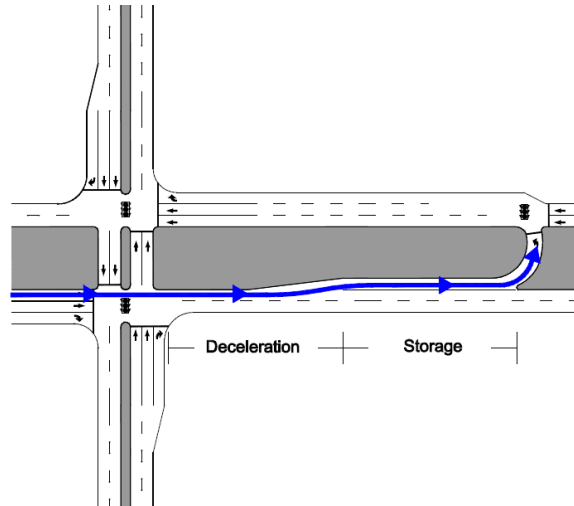
Figure 3-7: Spacing Consideration for A Major Street Left Turn Movement
