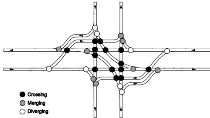
Figure 2-8: Conflict Point Diagram for a Conventional Intersection Source: FHWA, Displaced Left Turn Intersection Informational Guide (2014)
