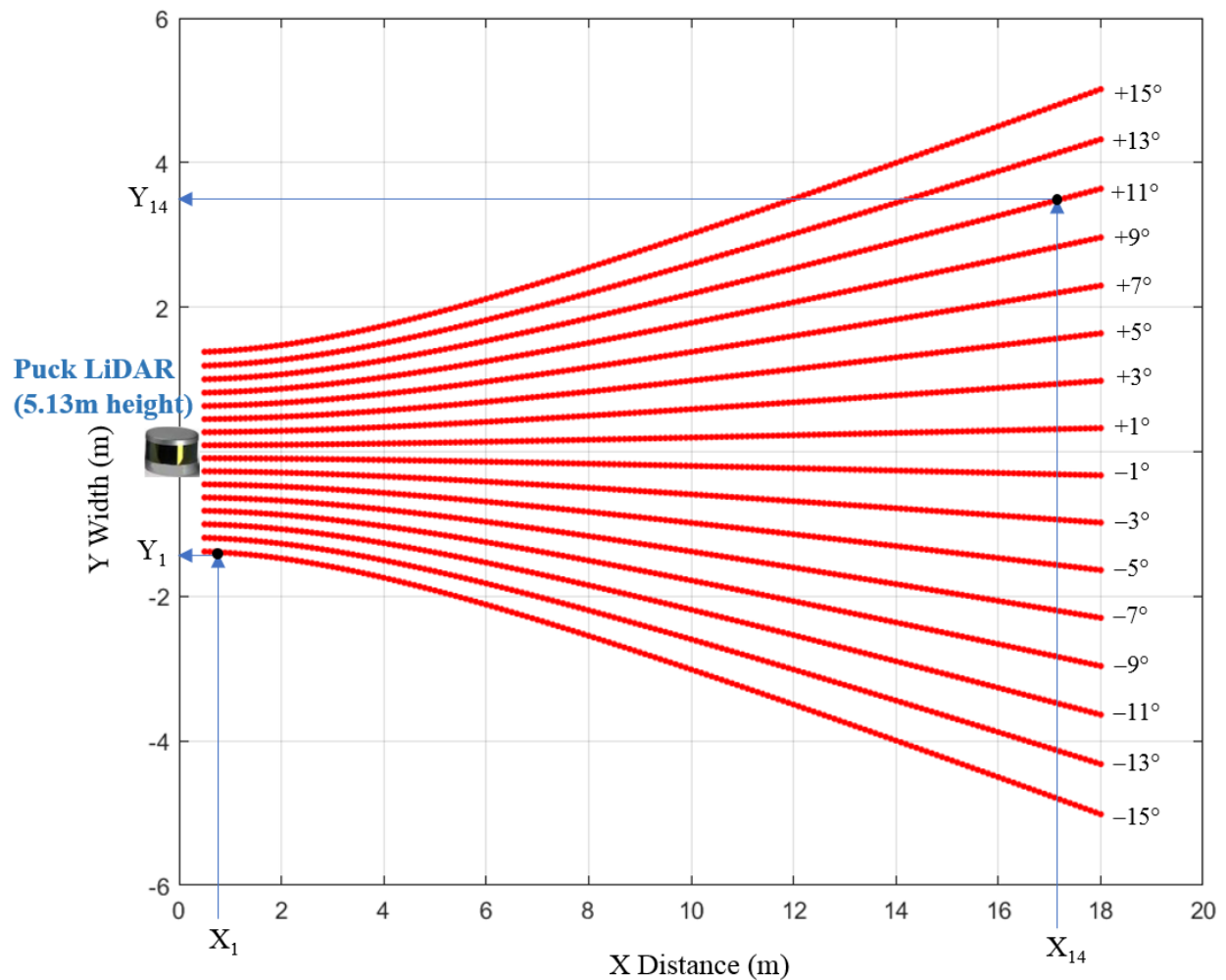
Figure 3-13. Calculated scan locations of the ceiling surface by a Puck LiDAR sensor (vertical installation)
