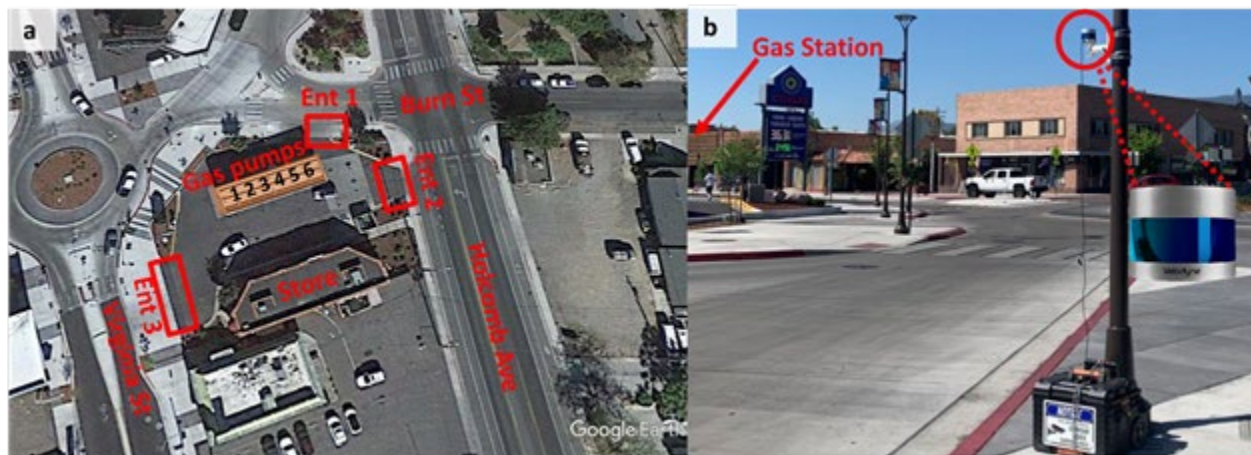
Figure 13-1. The location of the studied gas station/store (a), and the utilized LiDAR equipment installed in the northern part of the gas station/store (b)
