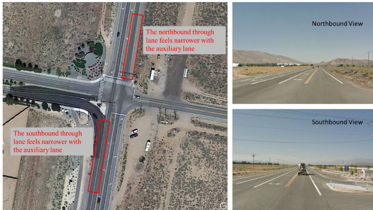
Figure 8-8 Comparison of northbound and southbound geometric elements that may have helped to reduce the southbound traffic speeds
