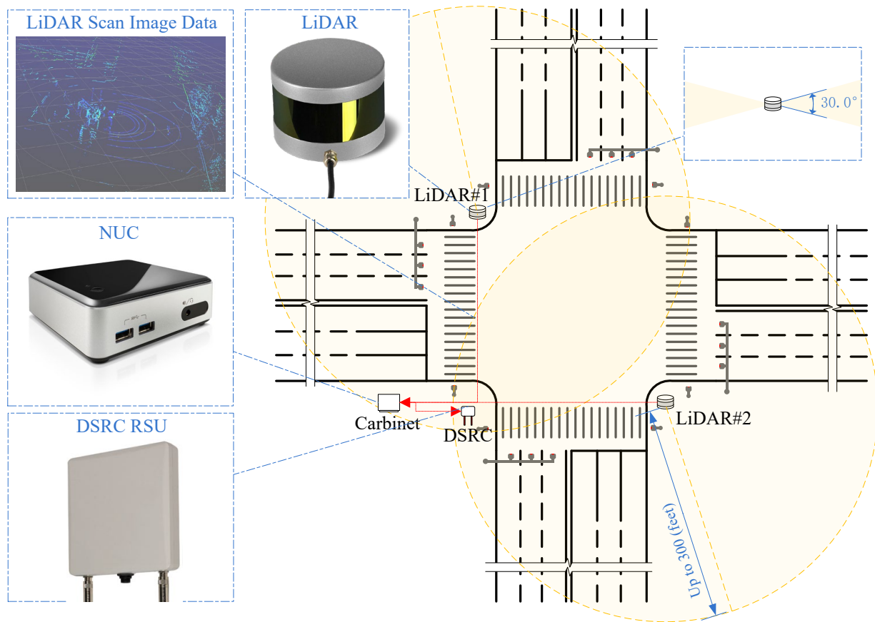
Figure 14-4. Implementation of the pilot DBCMA-LS RSU framework
