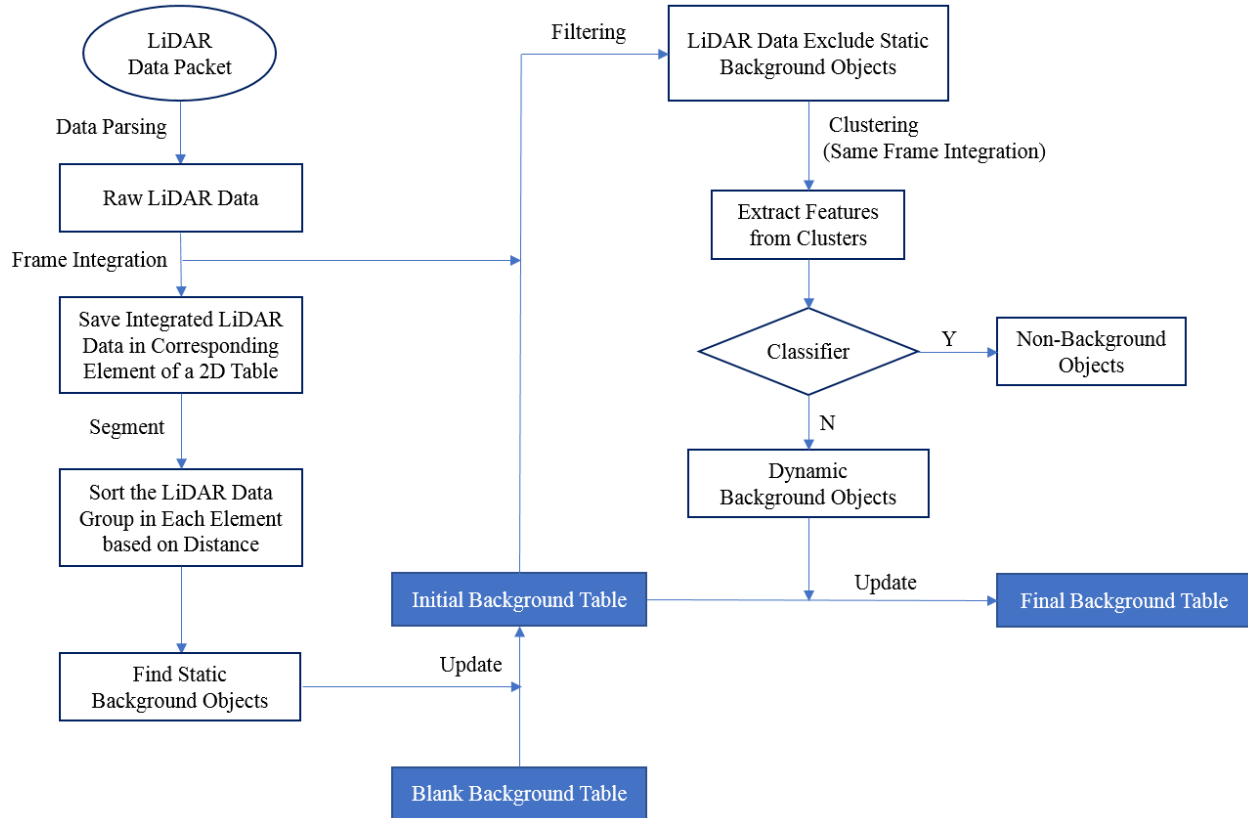
Figure 6-6 Flowchart of background table generation
