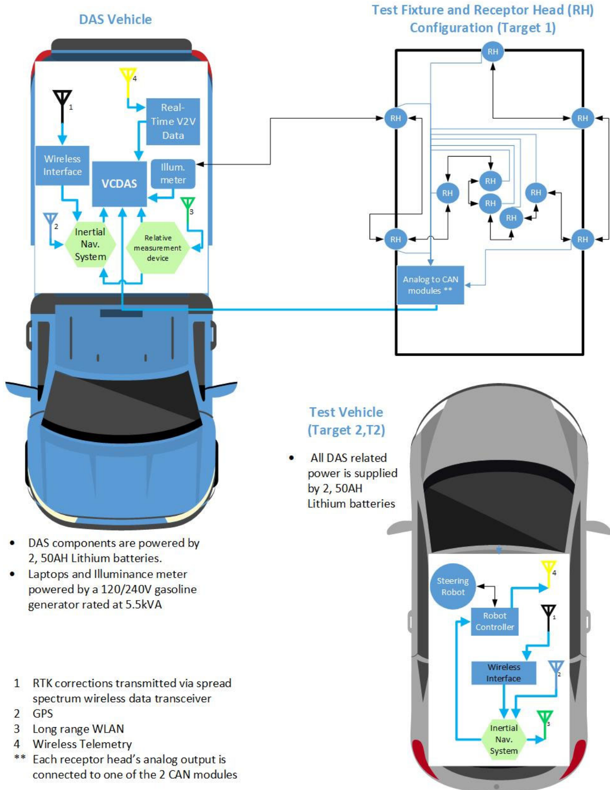
Figure 6. Data Acquisition System Diagram
