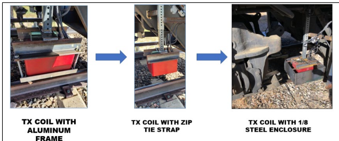
Figure 62. Evolution of Tx Coil Shielding
