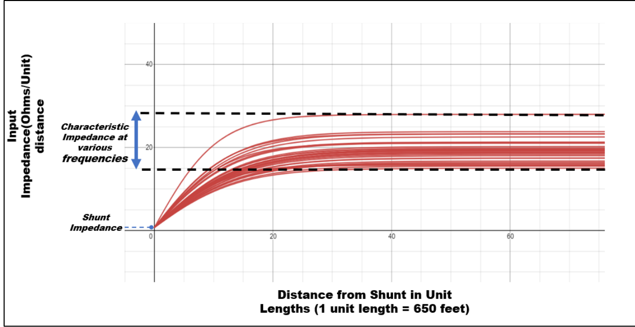
Figure 83. Sample Closed Loop Track Input Impedances at Different Frequencies and Distance to a Shunt
