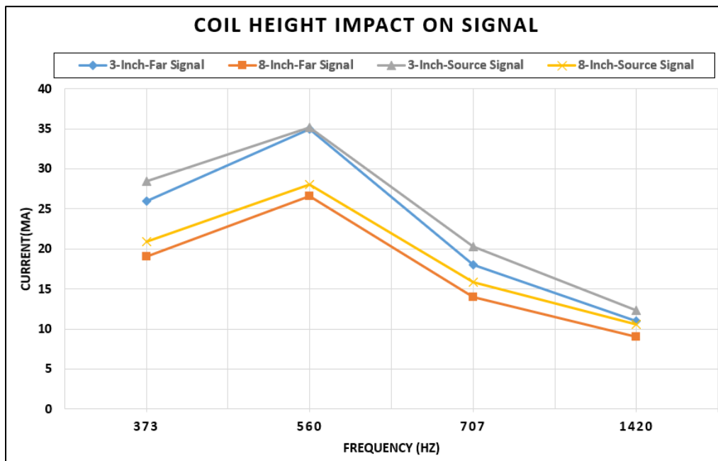
Figure 50. Comparison of Induced Current at Far and Source Ends at 12,000 feet vs. Tx Coil Height at Different Frequencies
