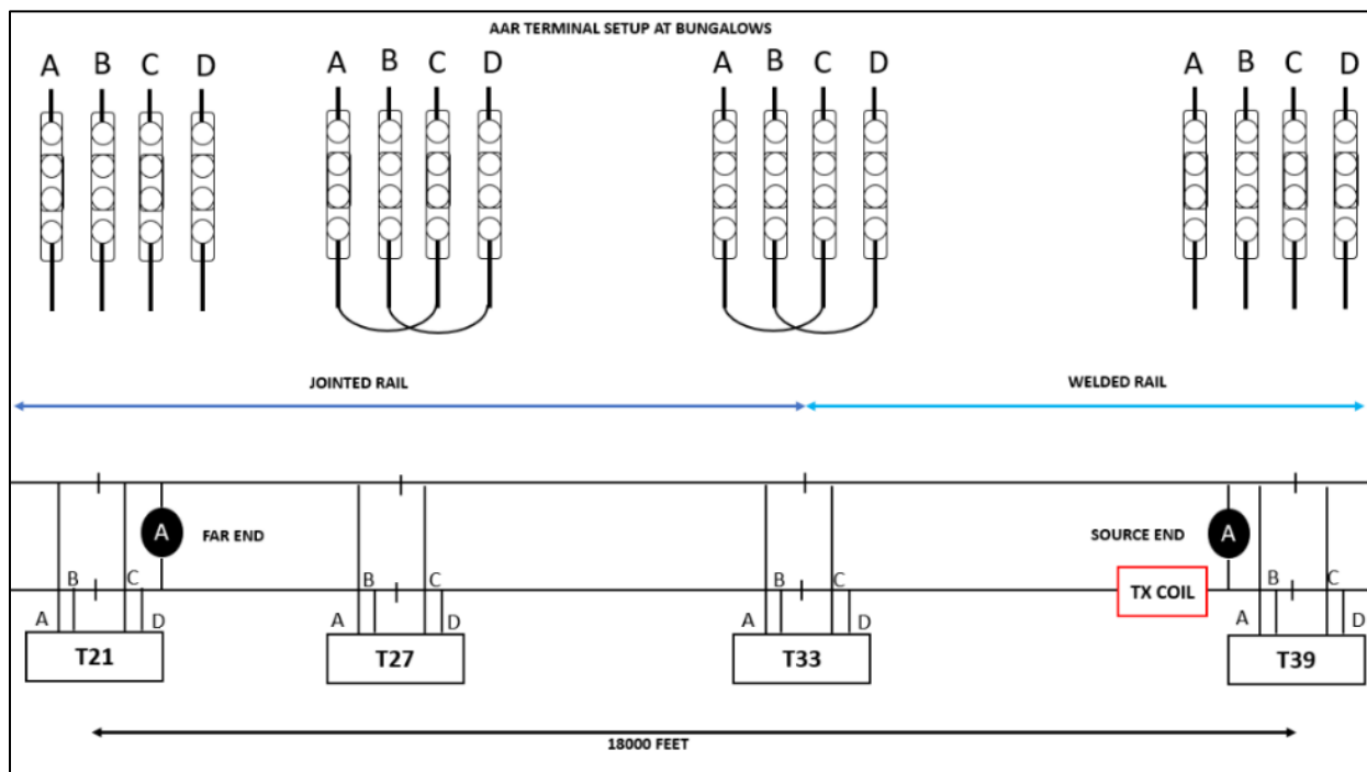
Figure 48. 18,000-foot Block Configuration for Static Testing
