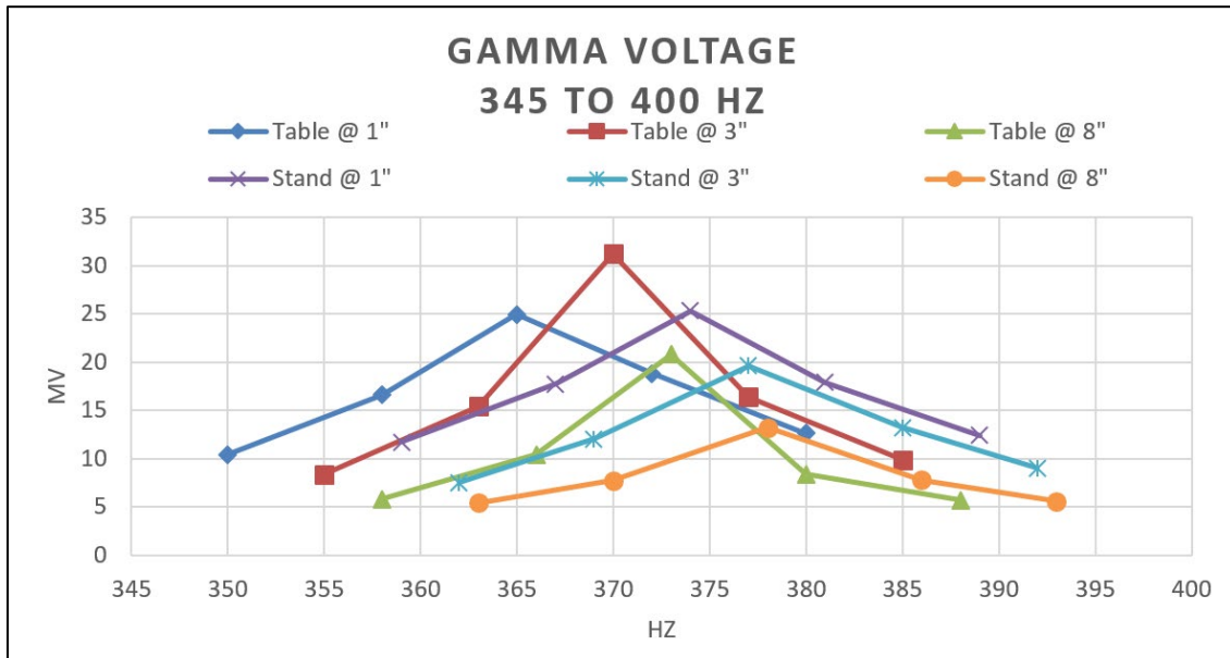
Figure 36. Gamma Voltage Measurements from 345–400 Hz
