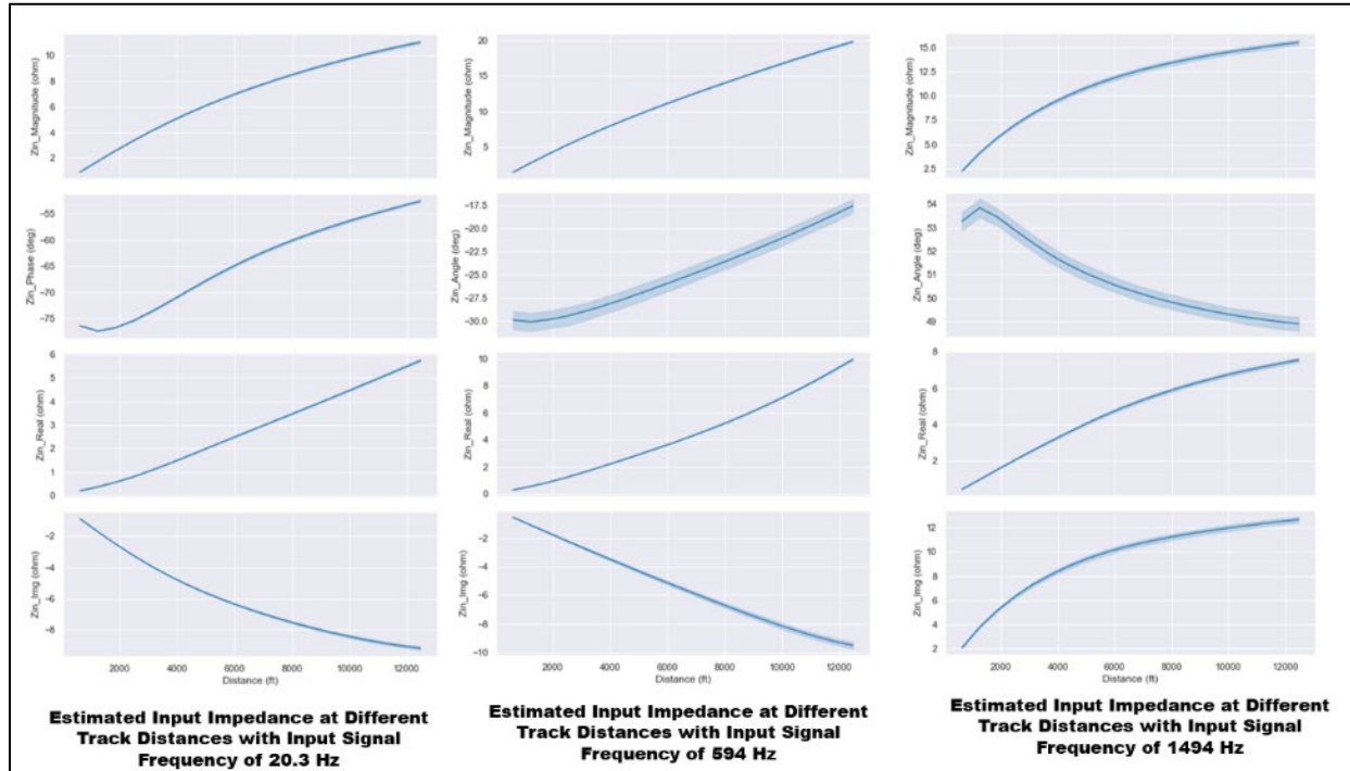
Figure 27. Estimated Input Impedance vs. Distances and for Different Frequencies
