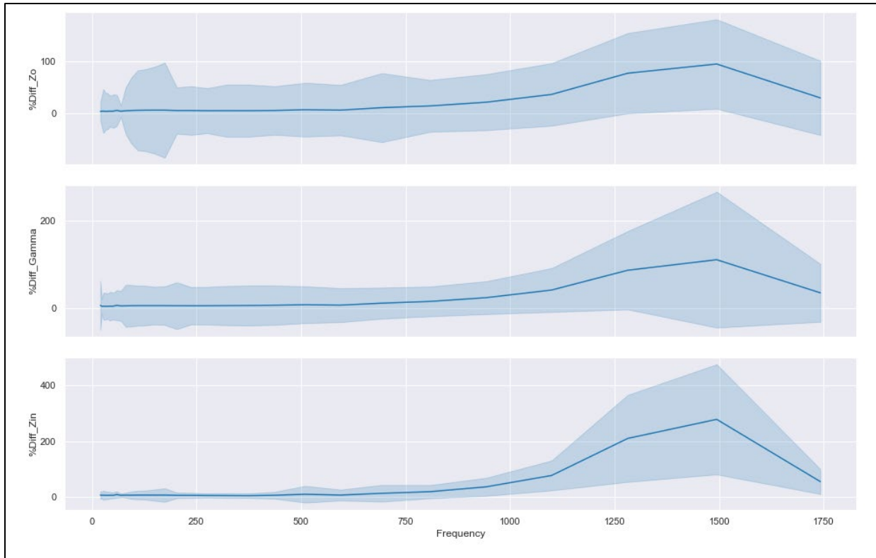
Figure G1. Percentage Difference and the Corresponding Standard Deviation Between the Results of the Two Methods of Calculating Z_o , \Gamma , and Z_{in} with the Transmission Line Equations
