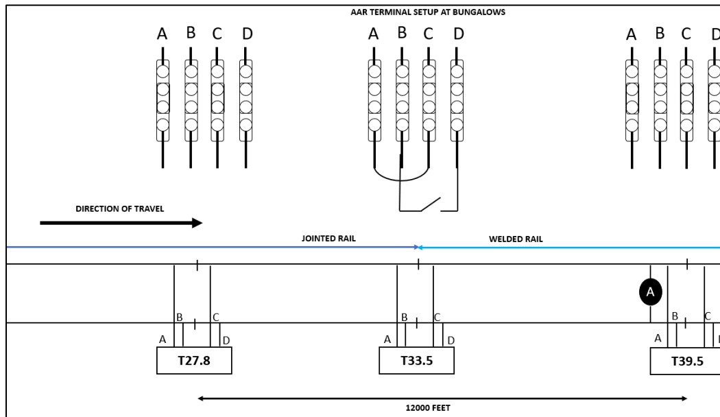
Figure 65. TTT Section and Track Connection Diagram for 12,000-foot Block Tests
