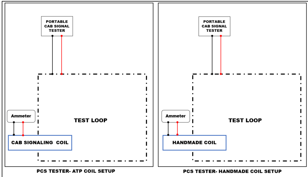
Figure 39. Portable Cab Signal Tester-Rx Coils Setup
