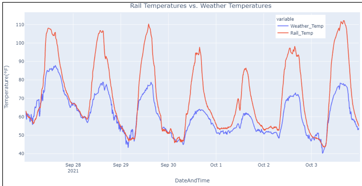
Figure 20. Weather and Rail Temperatures for a Sample of Fall Days
