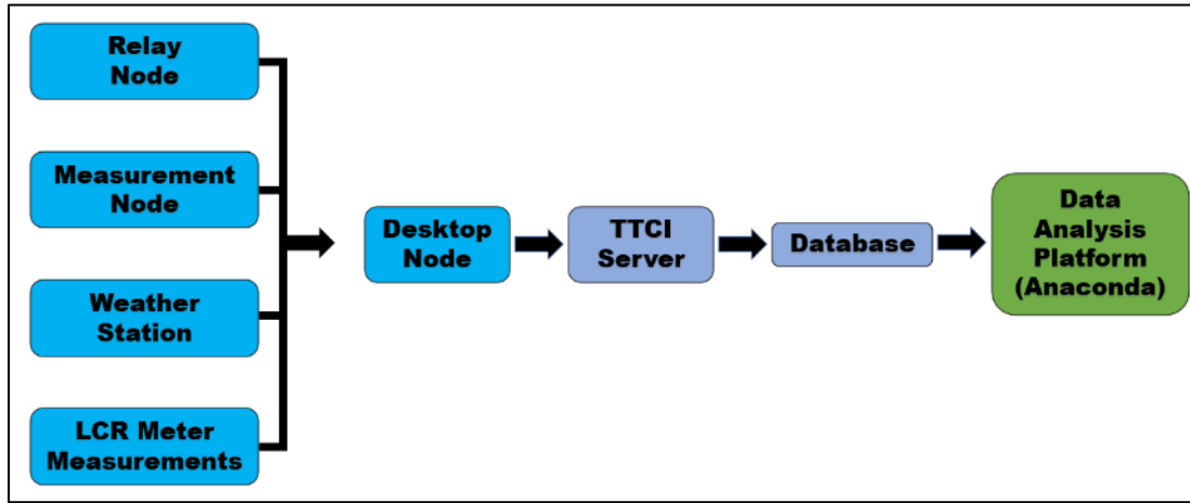
Figure 16. Flow Diagram of Measured Track Impedance Data of Data Analysis Process
