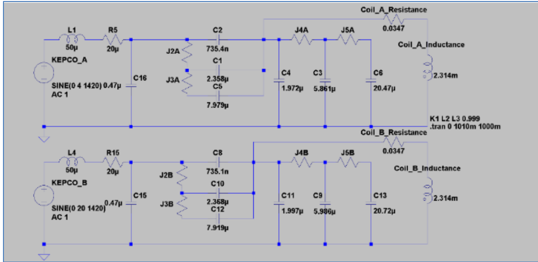
Figure A2. RNB Circuit Diagram
