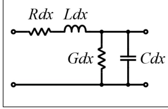
Figure 6. Transmission Line Distributed-Element Model
