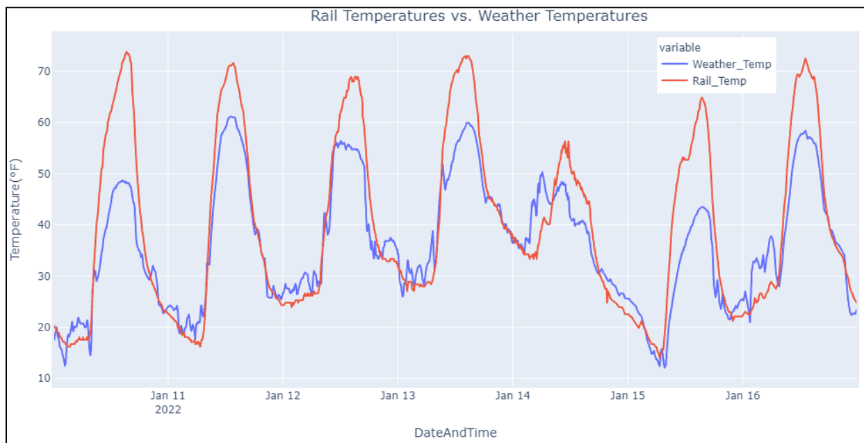
Figure 19. Weather and Rail Temperatures for a Sample of Winter Days
