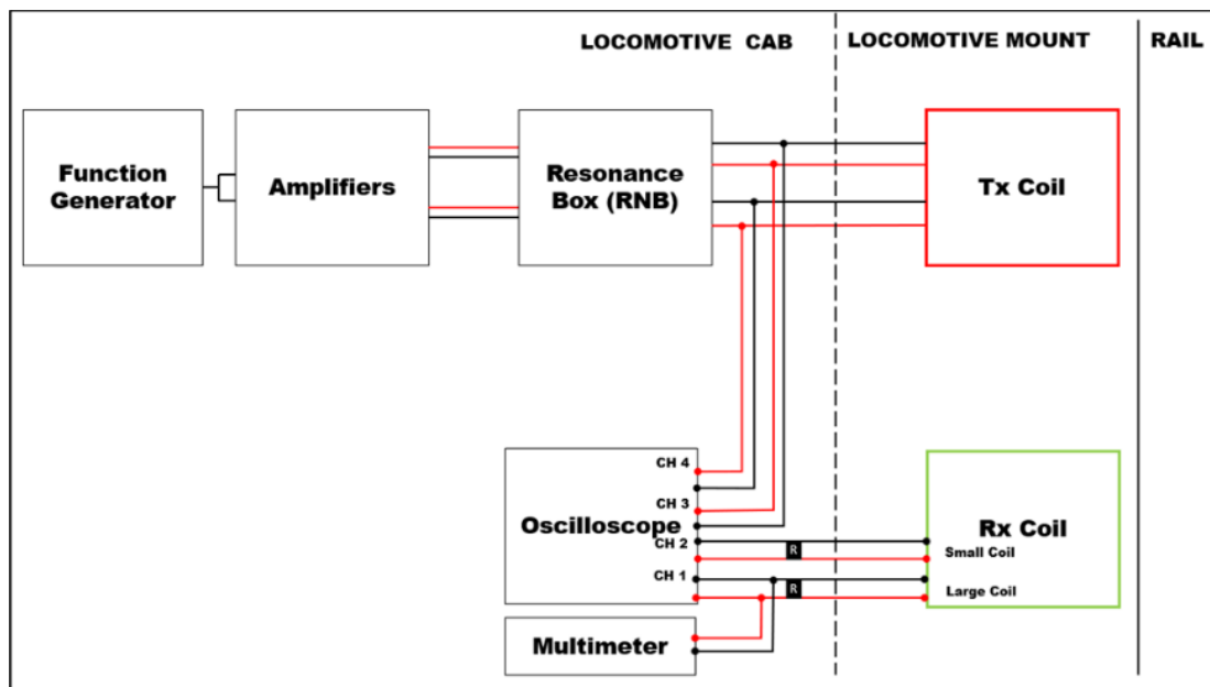
Figure 68. Electrical and Measurement Configuration of Tx and Rx Coil for Configuration A A second oscilloscope monitored the Rx coil when the system was set up in Configuration B.
