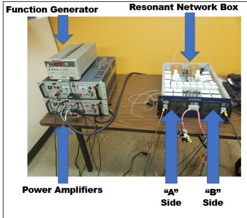
Figure 30. Resonance Signal Generation Equipment
