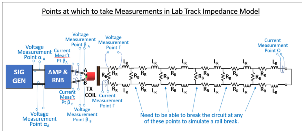
Figure 34. Lab Track Impedance Model Measurement Setup
