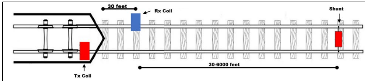
Figure 56. Test Case 2 Setup with Rx Coil Located 30 feet from Locomotive
