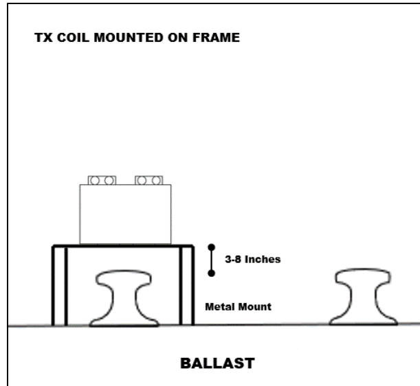
Figure 44. Tx Coil Setup for Static Testing
