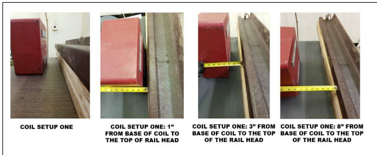
Figure 31. Tx Coil Setup One
