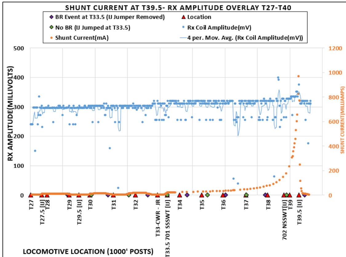
Figure 80. Dynamic Test Cases 7, 8, and 9 Tx and Rx Overlay vs. Locomotive Location from T27–T40
