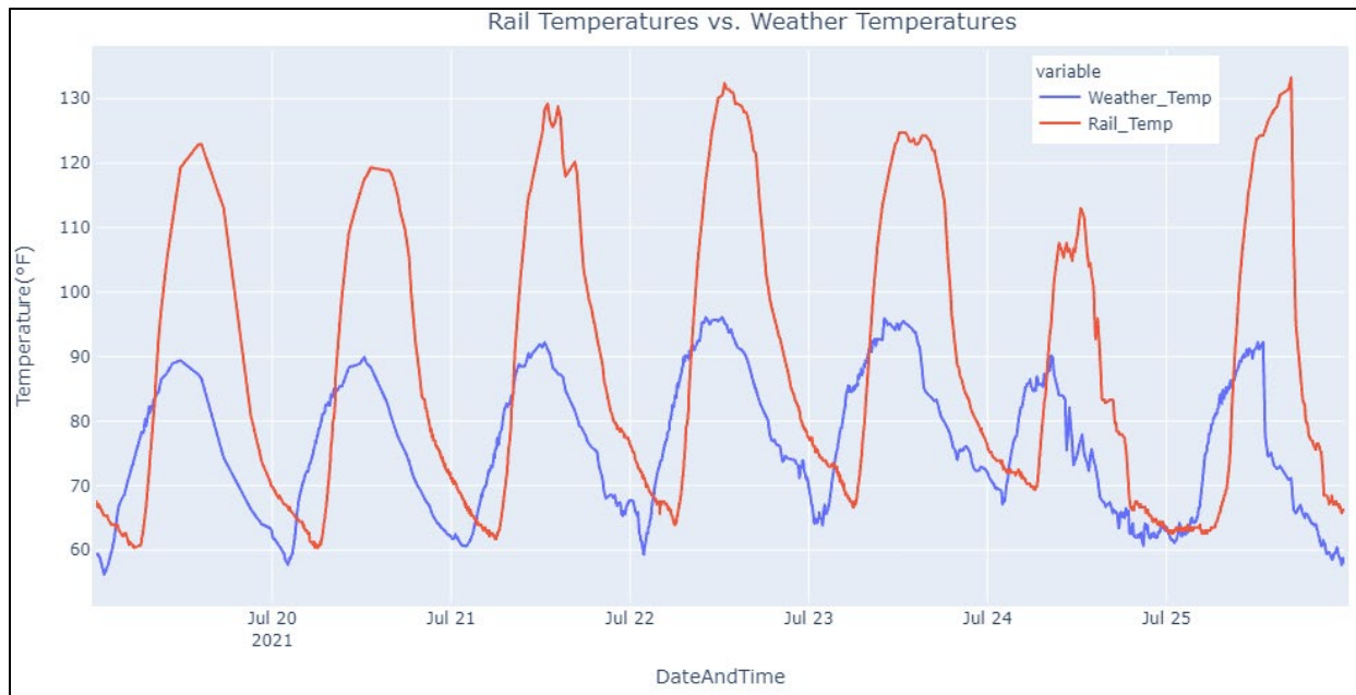
Figure 18. Weather and Rail Temperatures for a Sample of Summer Days
