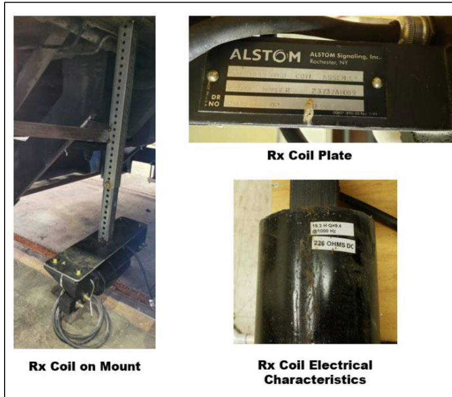
Figure C1. Rx Coil Assembly
