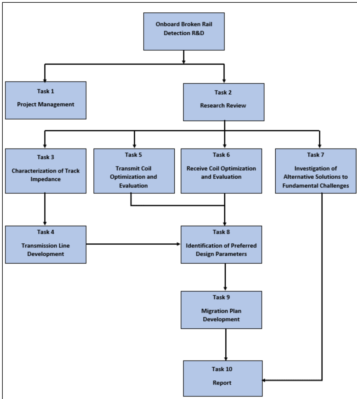
Figure 2. Project Work Breakdown Structure
