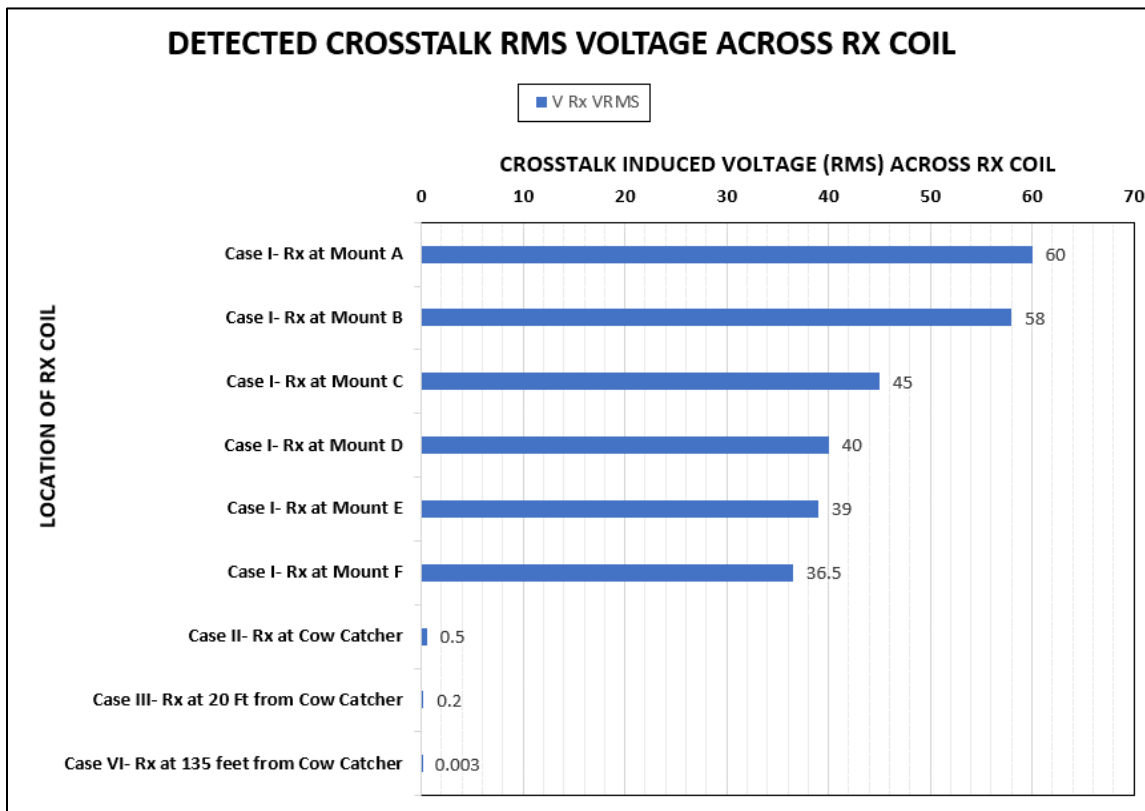
Figure 59. Detected Cross Talk RMS Voltage Across Rx Coil for Various Shields
