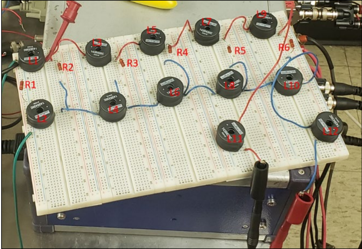
Figure 35. Image Simulated Track Circuit
