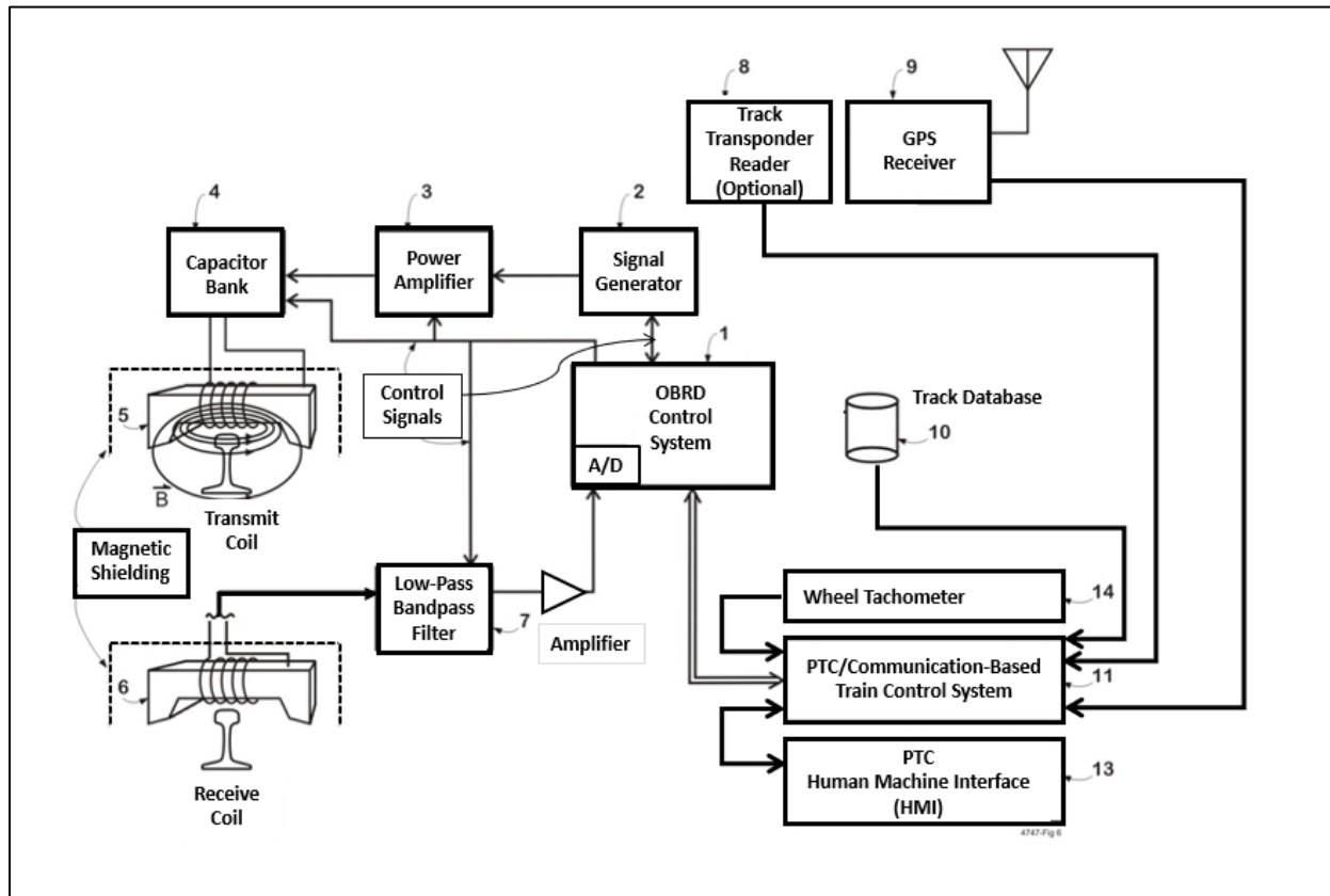
Figure 4. Functional Flow of OBRD System
