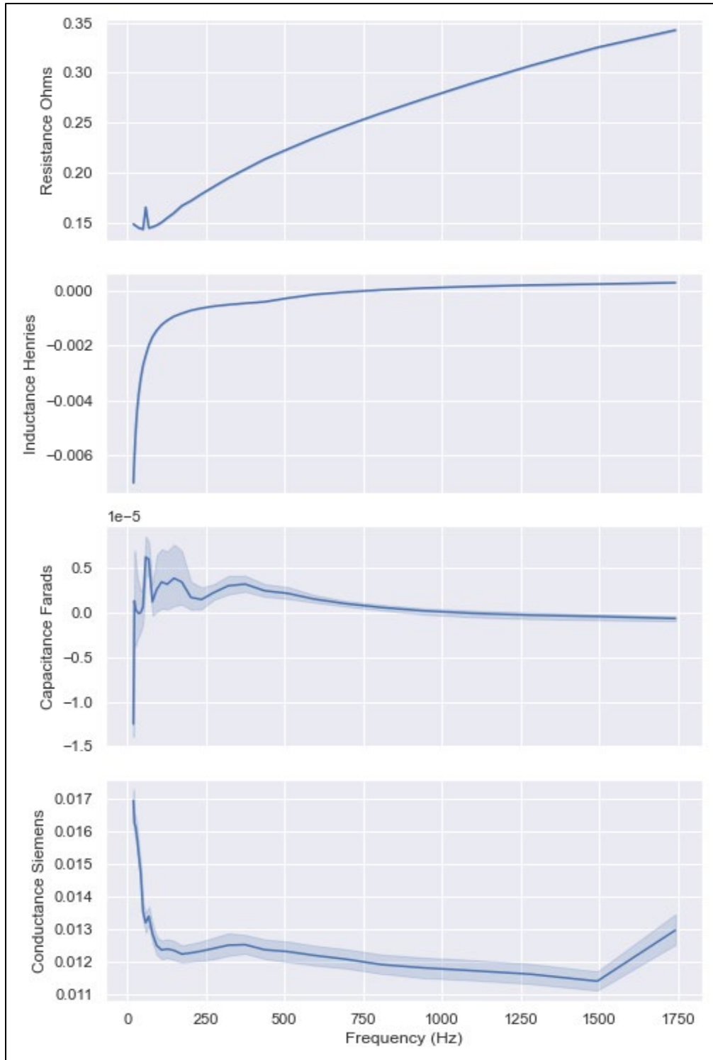
Figure 22. Track Impedance Variables (RLCG) vs. Frequency for 9 Months
