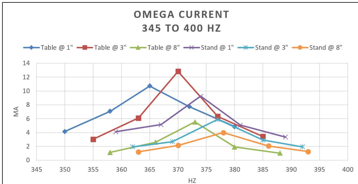
Figure 38. Omega Current Measurements from 345 Hz–400 Hz
