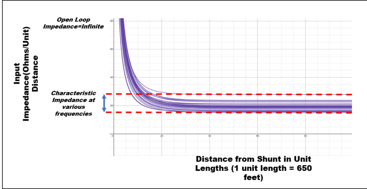
Figure 84. Sample Open Loop Track Input Impedances at Different Frequencies
