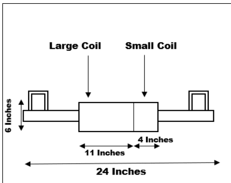
Figure C2. Illustration of Rx Coil Dimensions
