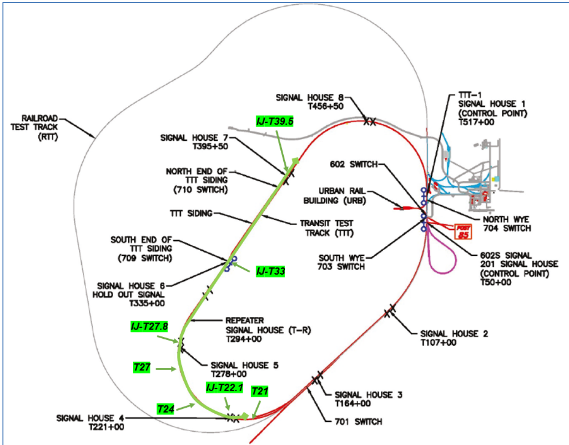
Figure 42. TTT Testing Zone
