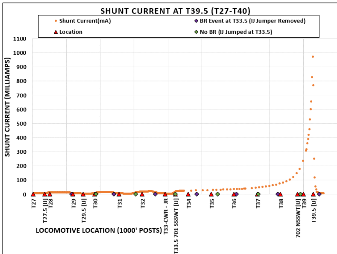
Figure 74. Shunt Current at T39.5 for Combined Dynamic Test Cases 7, 8, and 9 vs. Locomotive Location
