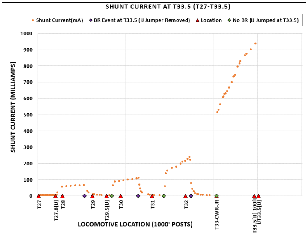
Figure 72. Shunt Current at T33.5 for Dynamic Test Case 6 vs. Locomotive Location
