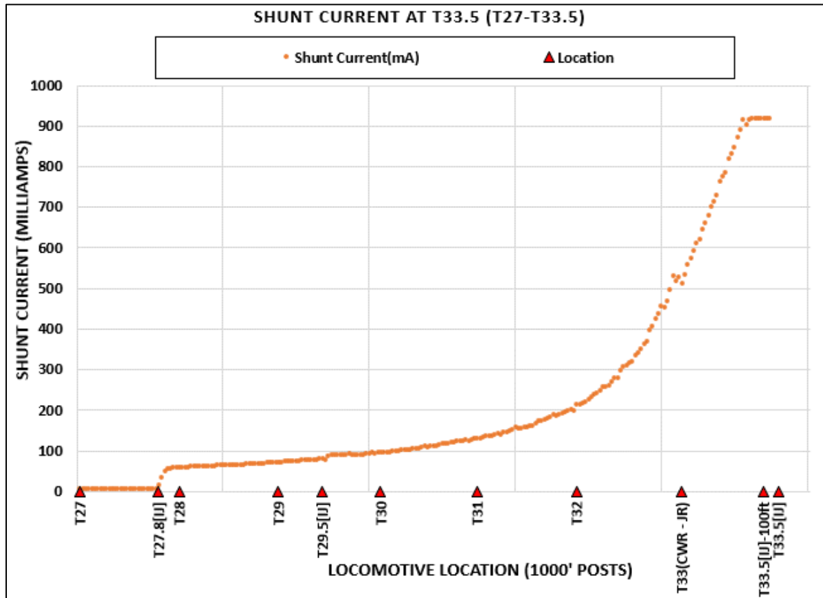
Figure 70. Shunt Current at T33.5 for Dynamic Test Cases 4 and 5 vs. Locomotive Location
