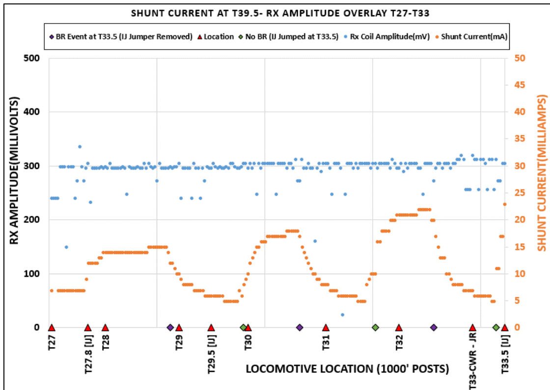
Figure 81. Dynamic Test Cases 7, 8, and 9 Tx and Rx Overlay vs. Locomotive Location from T27-T33.5
