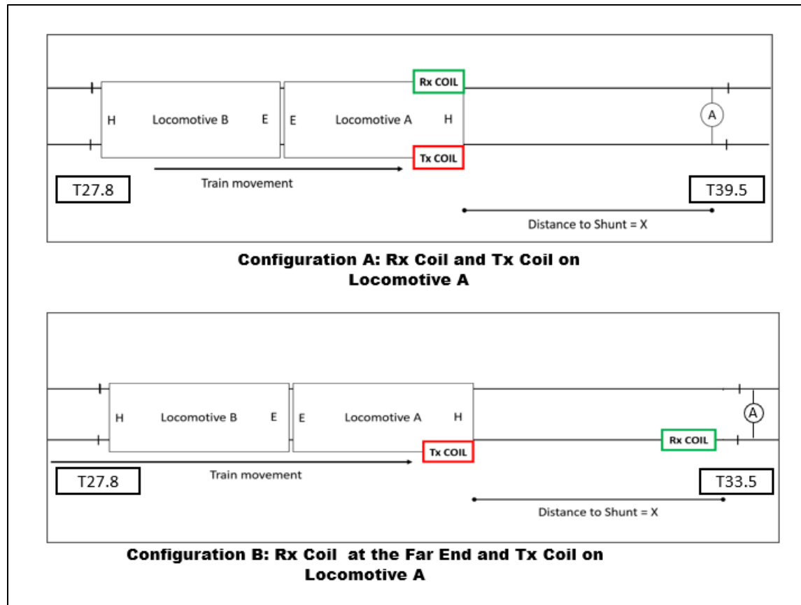
Figure 64. Locomotive, Tx and Rx Coil Configurations for Dynamic Test Cases 4, 5, 6, 7, 8, and 9
