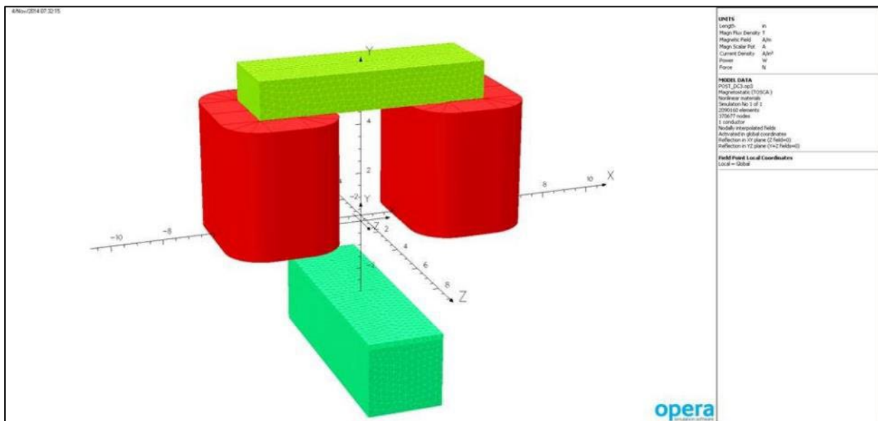
Figure B2. Simulation of Tx Electromagnetic Coils
