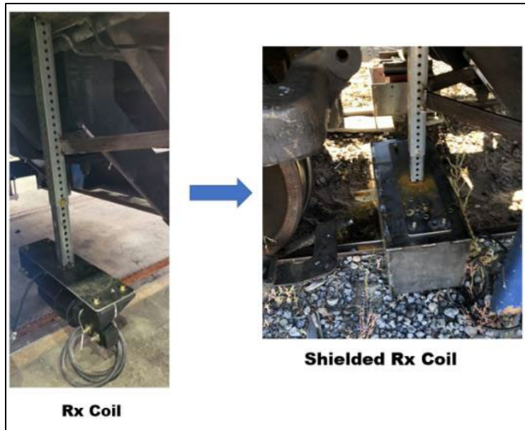
Figure 63. Evolution of Rx Coil Shielding
