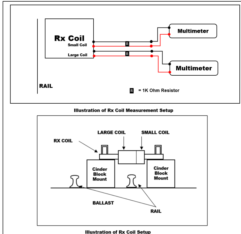
Figure 54. Rx Coil Setup
