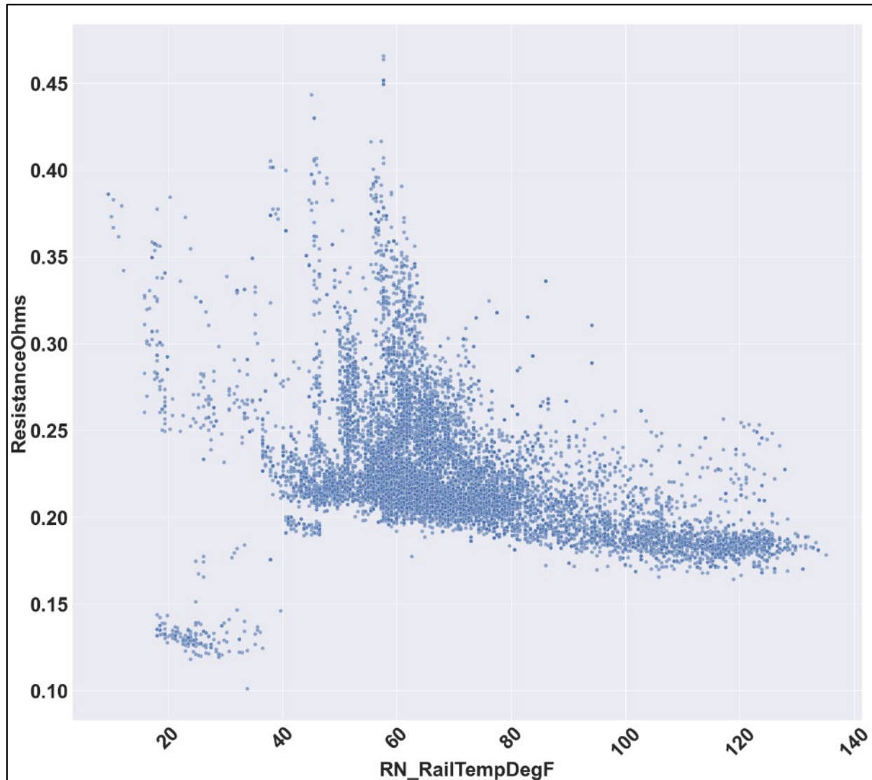
Figure 23. Track Resistance vs. Rail Temperature
