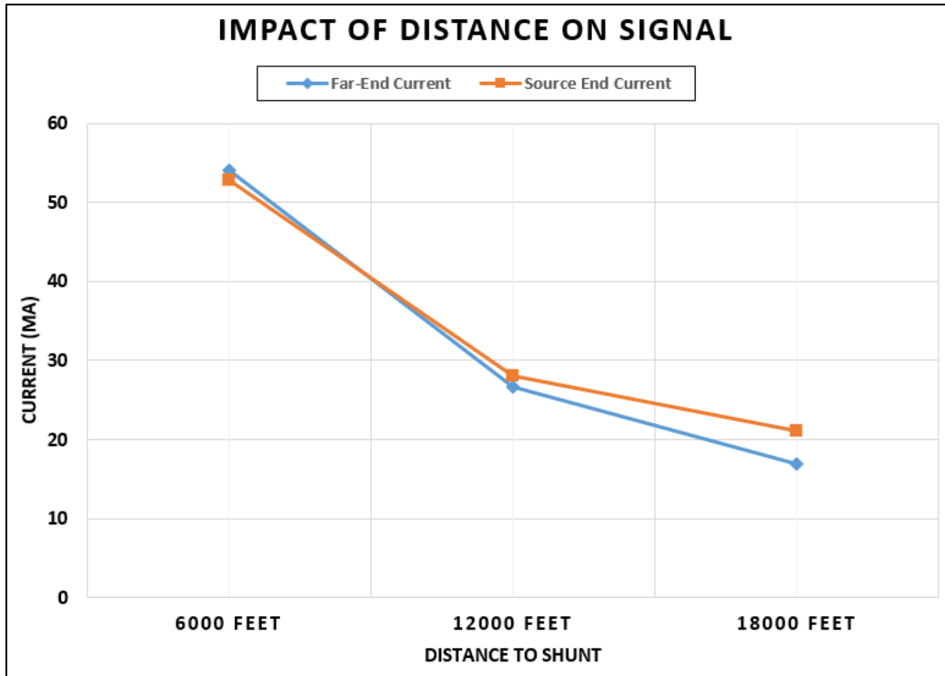
Figure 51. Comparison of Induced Current at 568 Hz to Distance from Source
