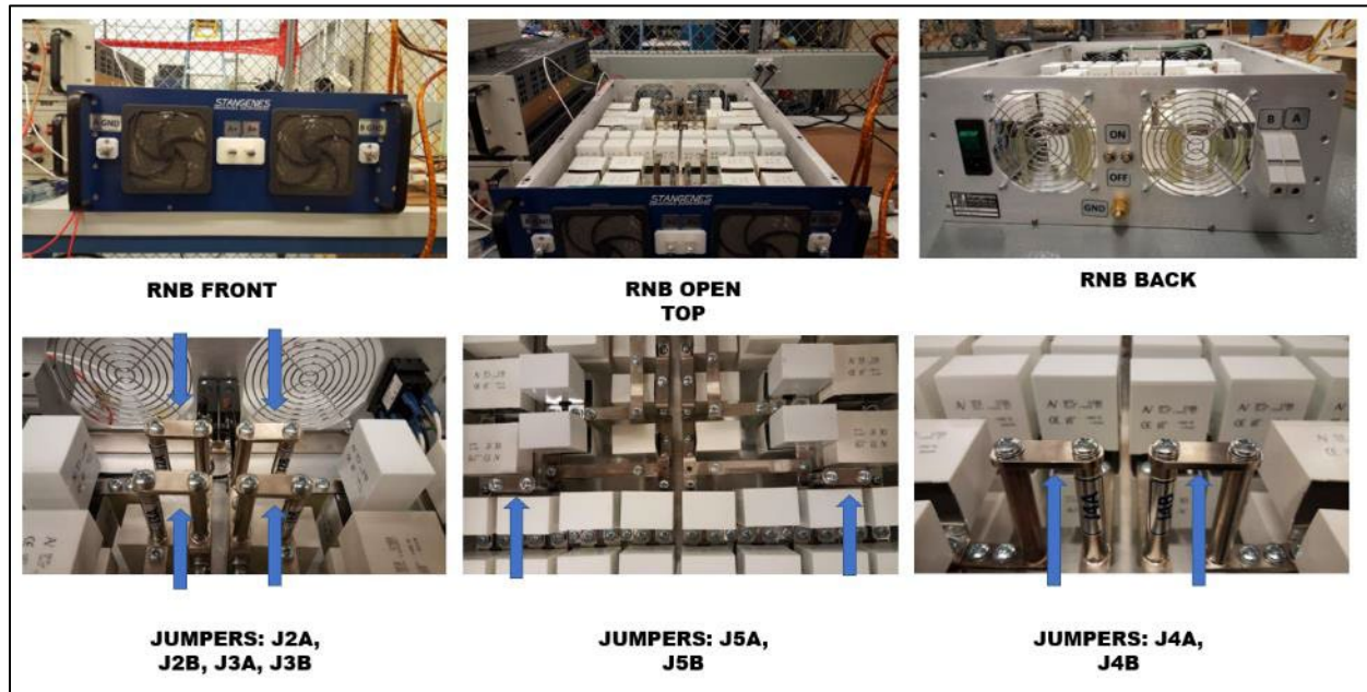
Figure A1. RNB Showing Jumper Locations
