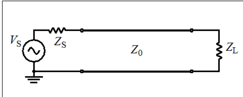
Figure 5. Transmission Line
