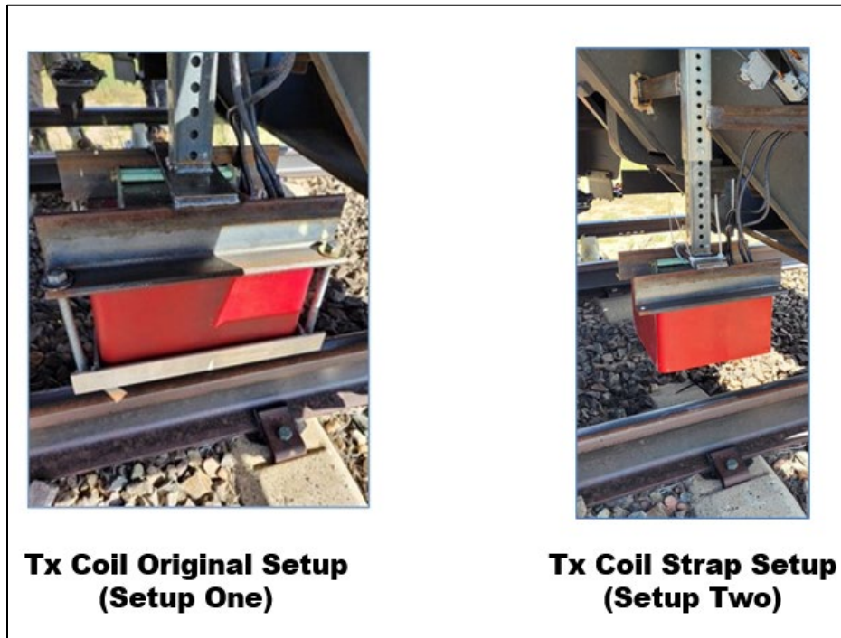
Figure 53. Tx Coil Setups
