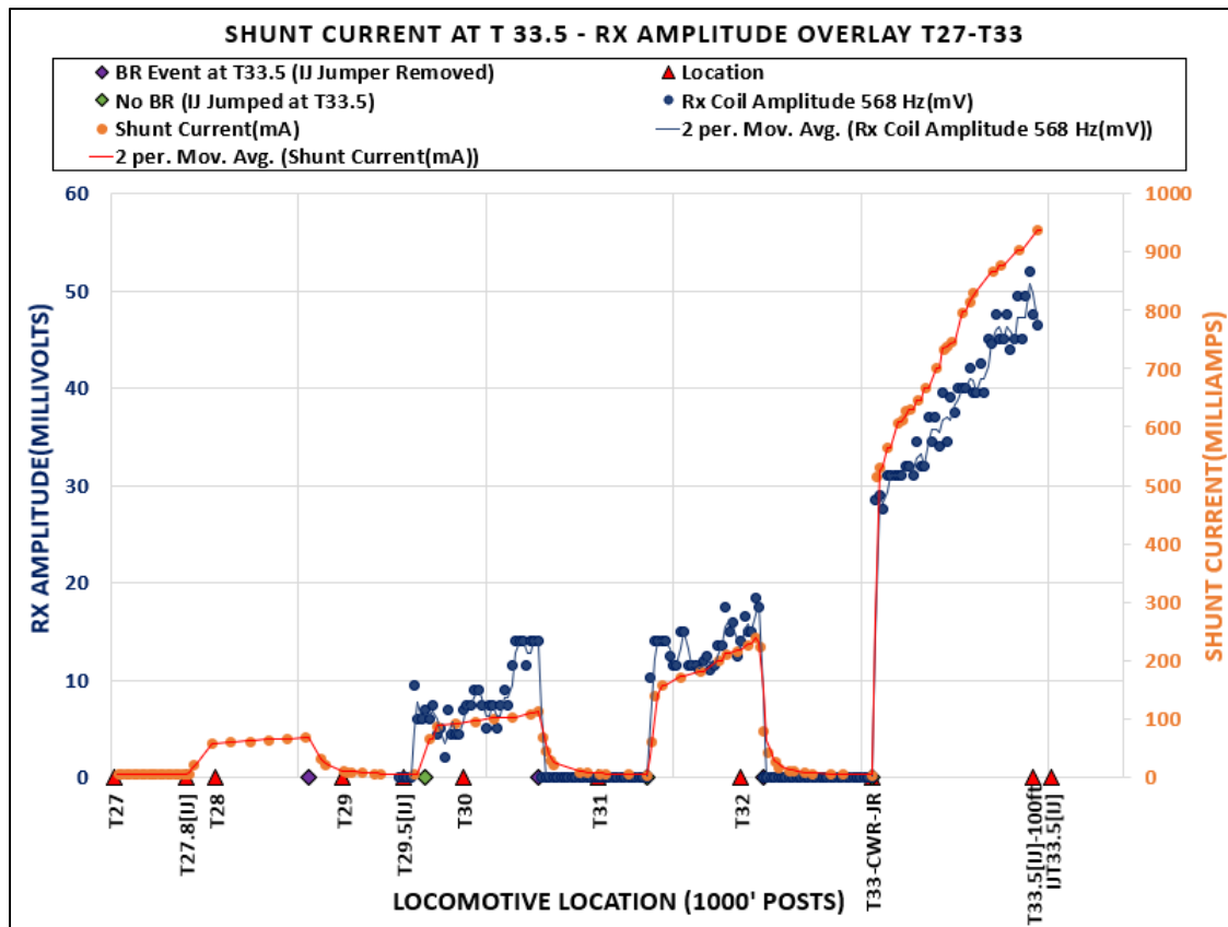
Figure 82. Dynamic Test Case 6 Tx and Rx Overlay vs. Locomotive Location
