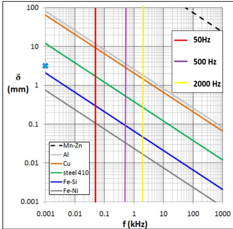
Figure 60. Skin Effect Depth Variance with Frequency for Various Materials
