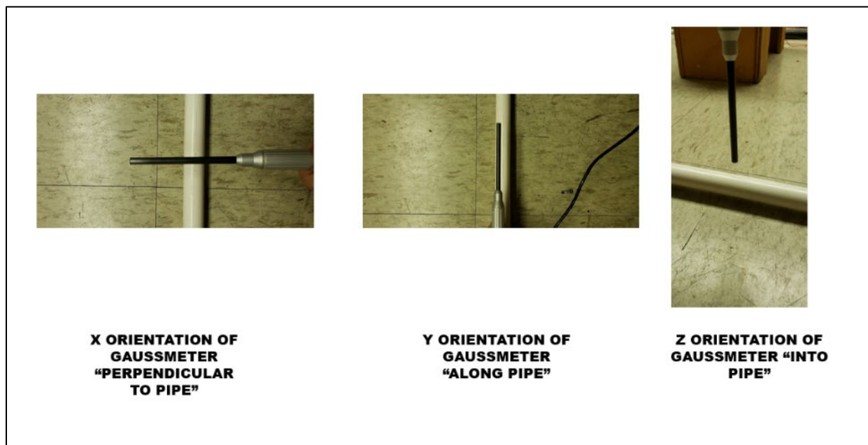
Figure 41. Gaussmeter Testing Orientation
