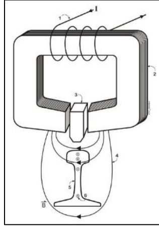
Figure 3. Functional Representation of a Tx or Rx Coil
