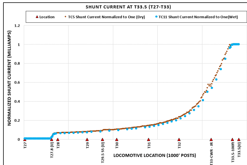
Figure 78. Dynamic Test Cases 11 and 5 Comparison Showing Effects of Wet Ballast on Induced Signal vs. Locomotive Location
