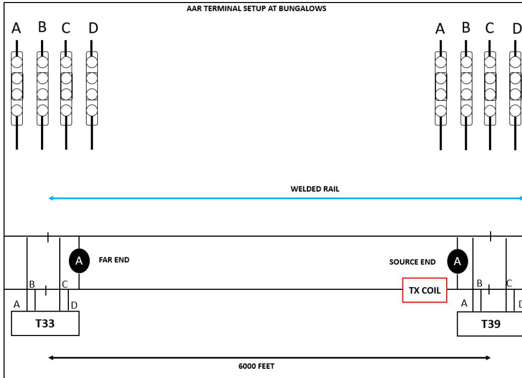
Figure 46. 6,000-foot Block Configuration for Static Testing
