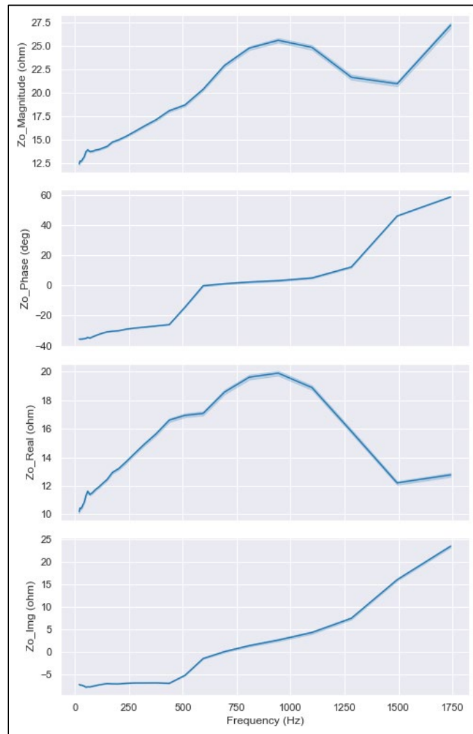
Figure 25. Characteristic Impedance vs. Frequency
