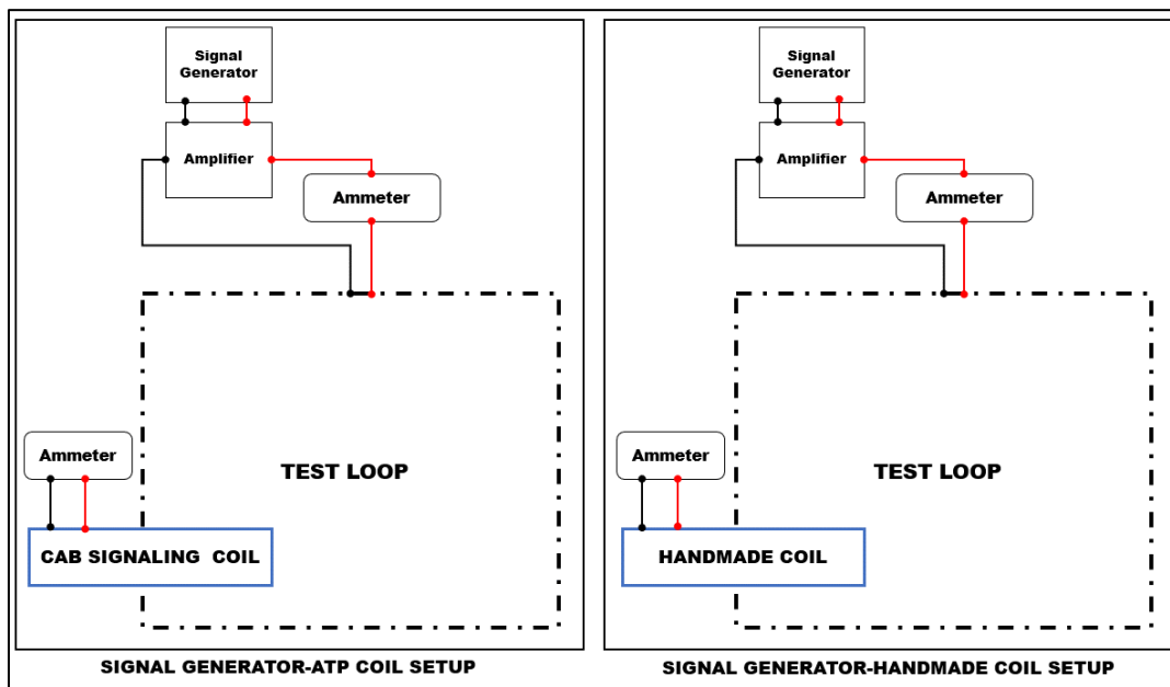
Figure 40. Signal Generator-Rx Coils Setup
