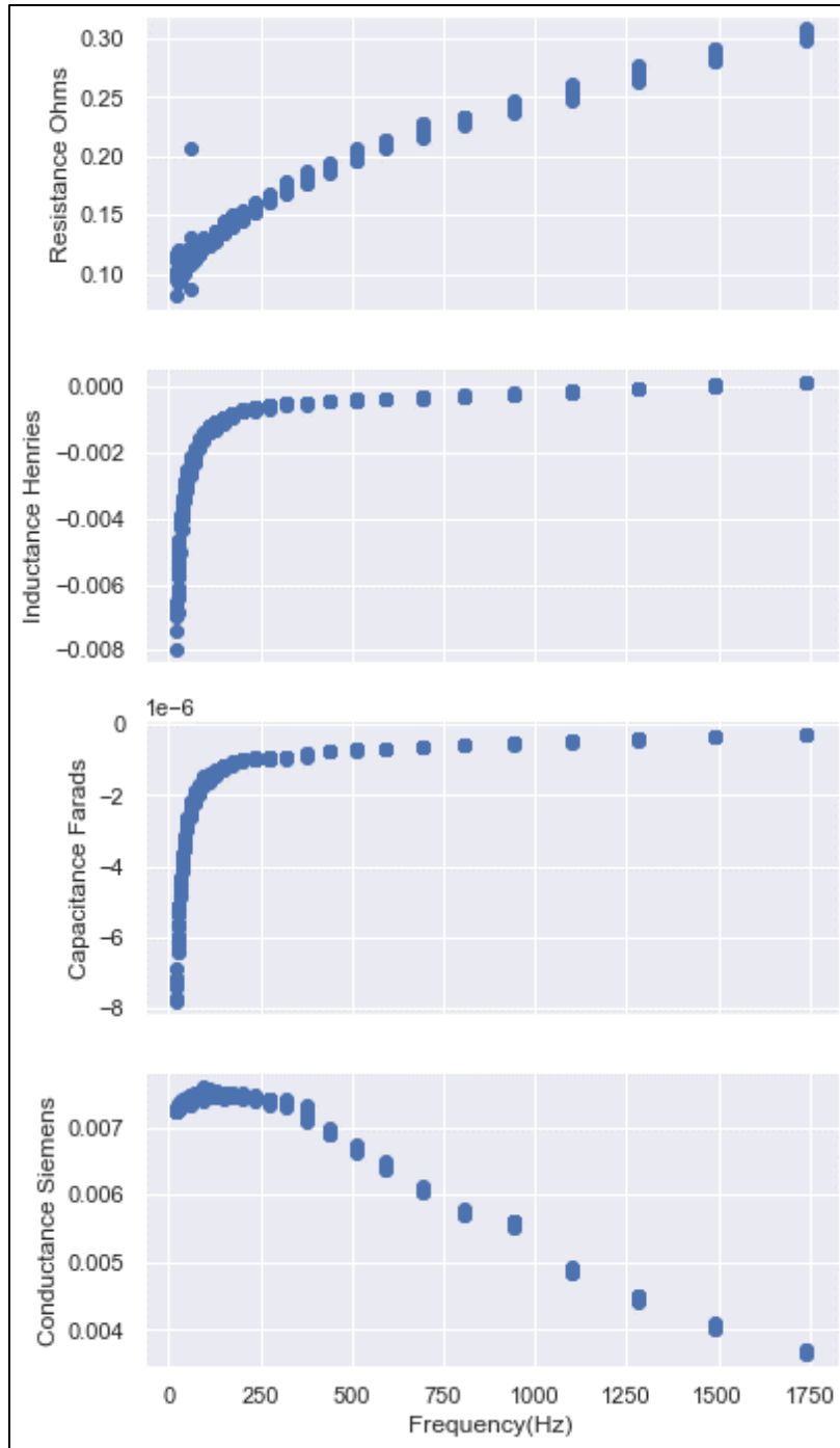
Figure 21. Track Impedance Variables (RLCG) vs. Frequency for 1 Day
