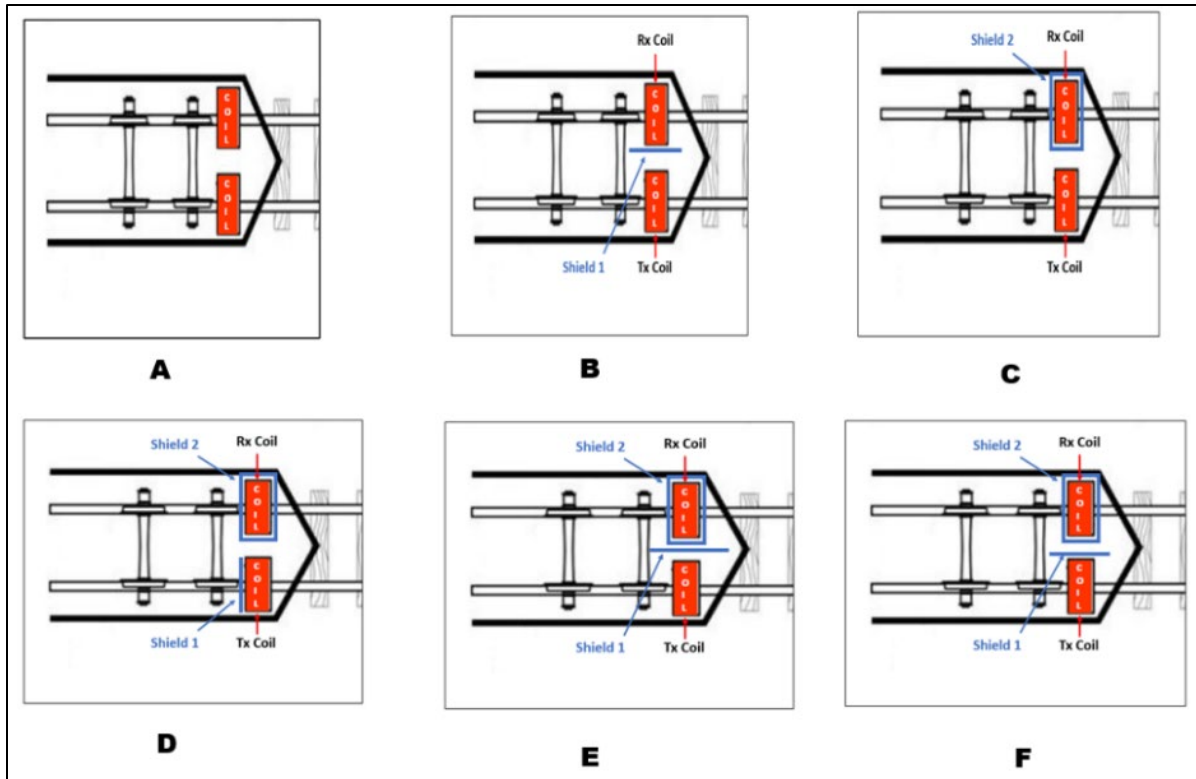
Figure 58. Case 1 Shielding Orientations
