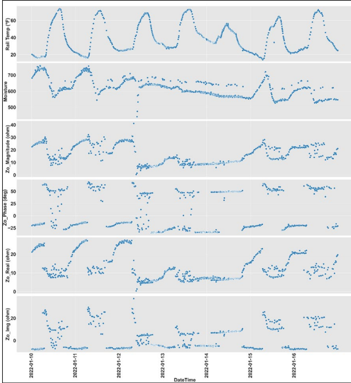
Figure 26. Time Series for Rail Temperature, Ballast Moisture, and Characteristic Impedance Magnitude, Phase Angle, Real and Imaginary Components
