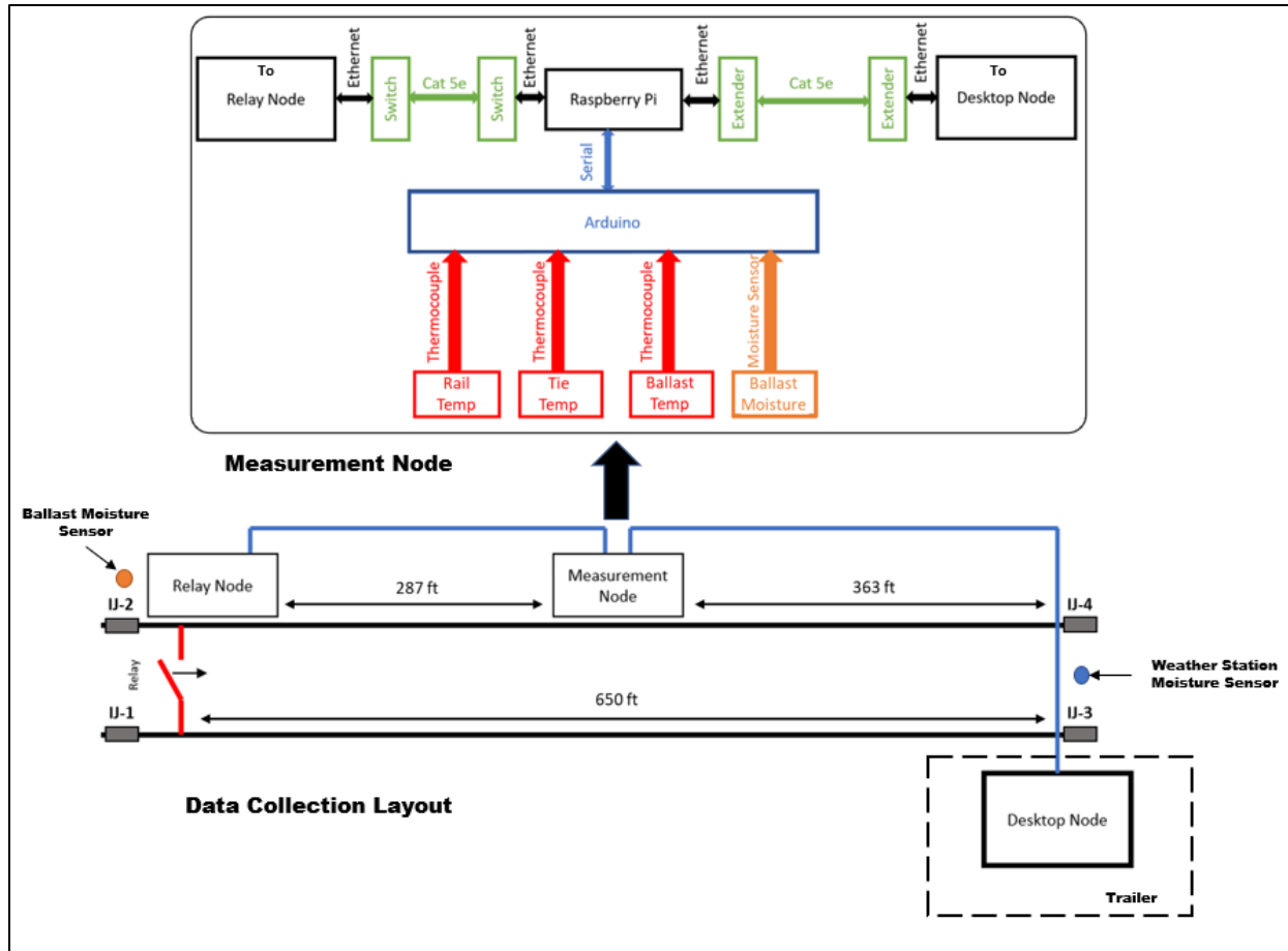
Figure 9. Track Impedance Data Collection and Measurement Setup
