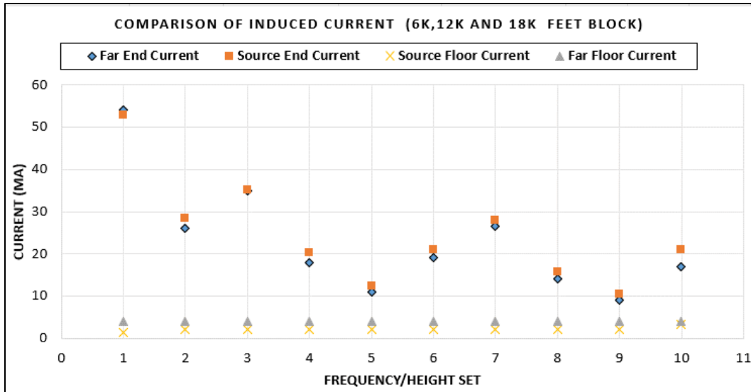
Figure 49. Comparison of Induced Currents at Far and Source Ends at Various Tx Coil Heights Above Rail and Distances from Far-End Shunt for Static Tests
