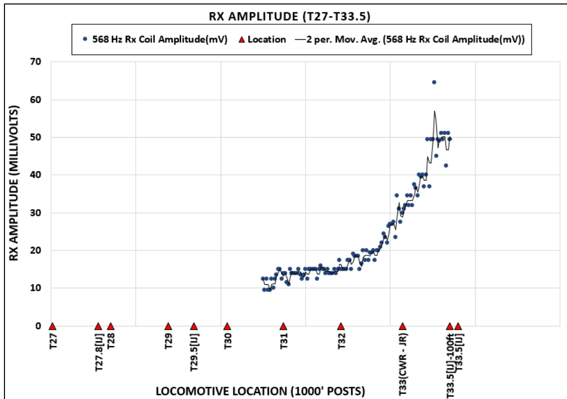
Figure 71. Rx Coil Signal Amplitude for Dynamic Test Cases 4 and 5 vs. Locomotive Location
