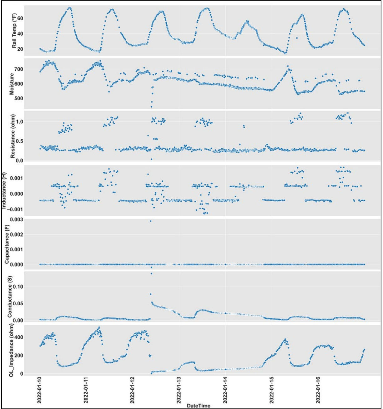
Figure 24. Time Series for Rail Temperature, Ballast Moisture, RLCG and Open Circuit Impedance
