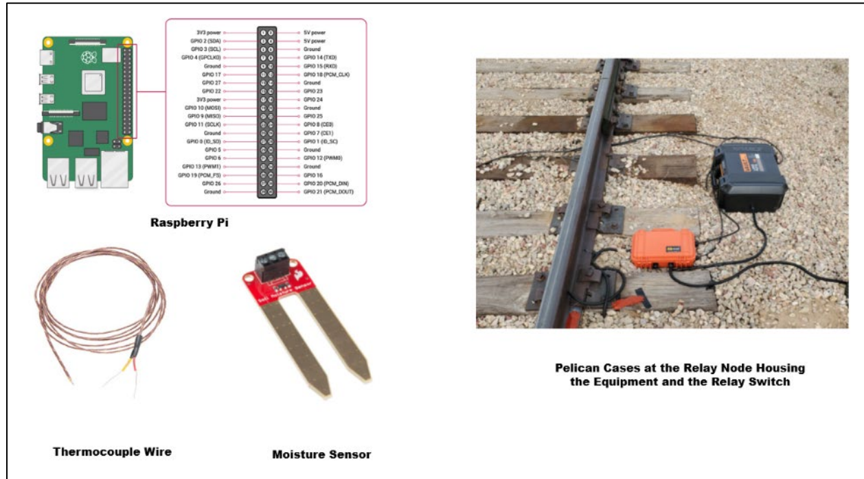
Figure 10. External Data Collection Hardware
