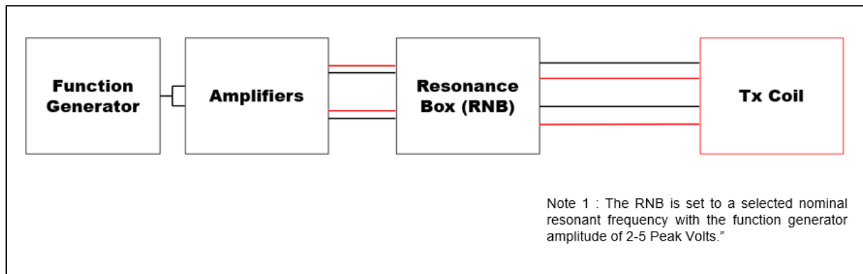
Figure A3. Flow Diagram of RNB Setup
