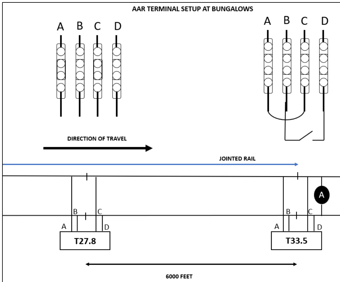
Figure 66. Test Track Section and Track Connection Diagram for 6,000-foot Block Tests
