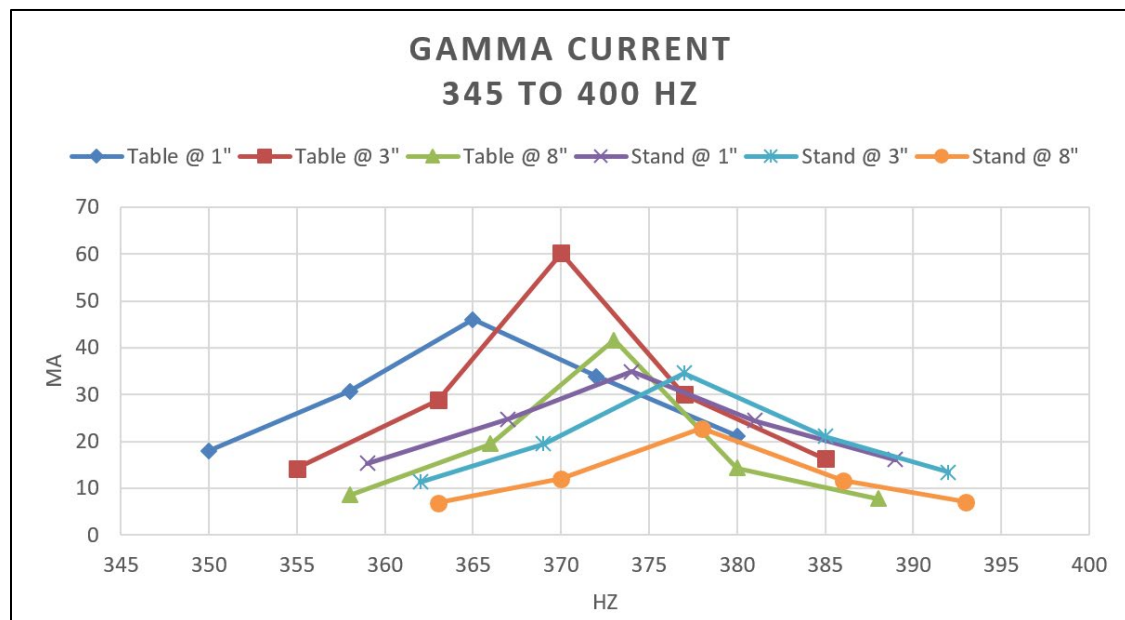
Figure 37. Gamma Current Measurements from 345–400 Hz
