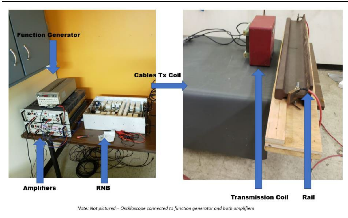
Figure 29. RNB Testing Setup
