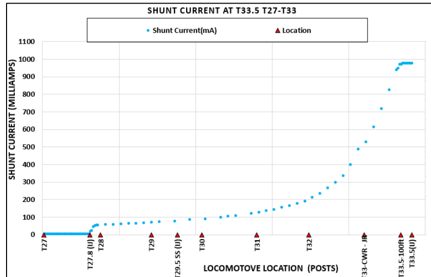
Figure 77. Dynamic Test Cases 11 Showing Effects of Wet Ballast on Induced Signal vs. Locomotive Location
