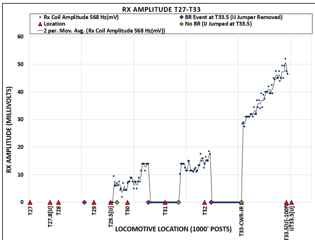
Figure 73. Rx Coil Amplitude for Dynamic Test Case 6 vs. Locomotive Location
