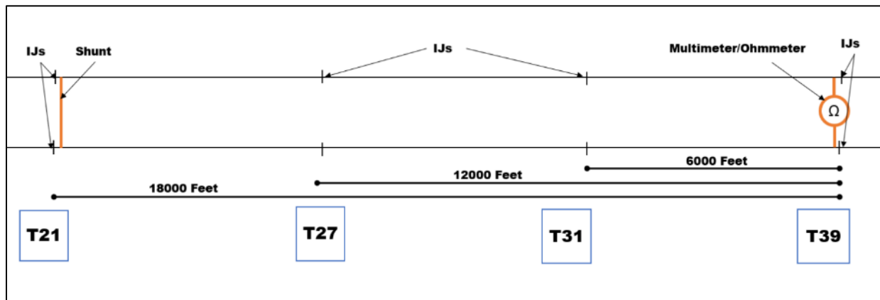
Figure 43. Track Resistance Measurement Setup
