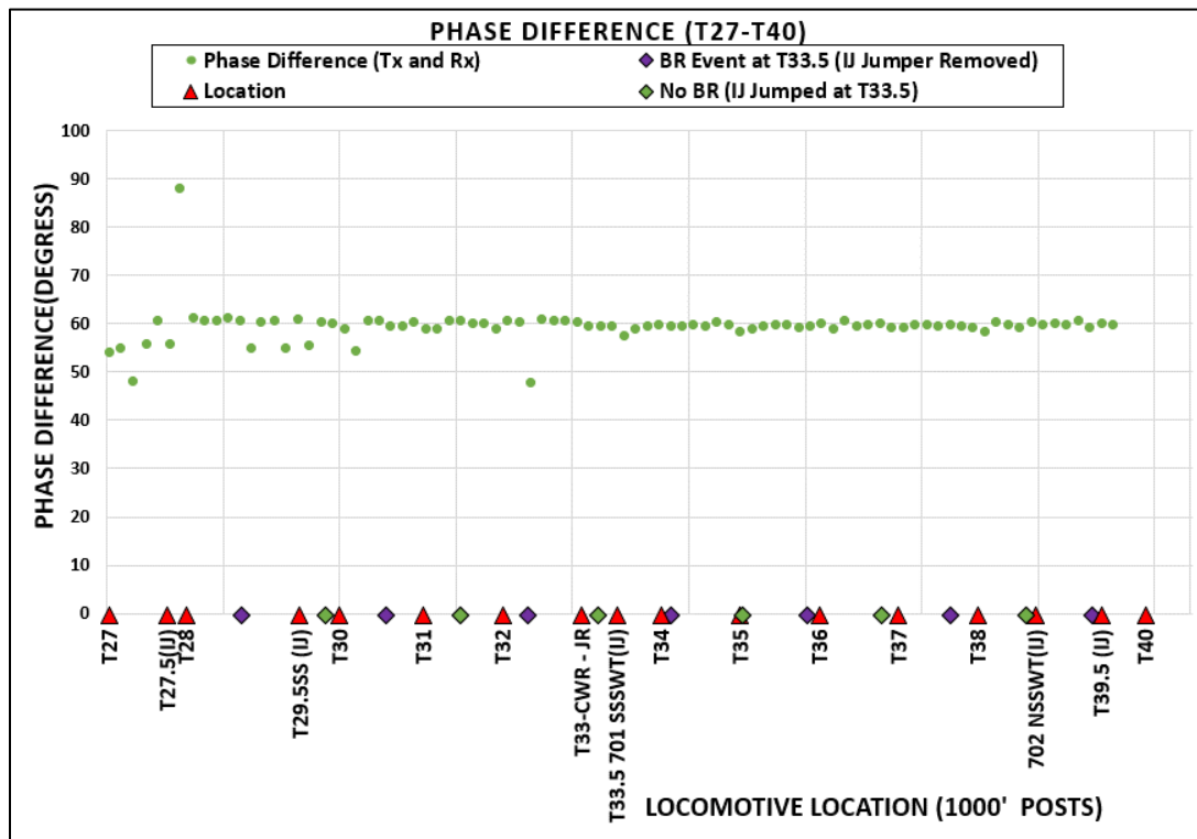
Figure 79. Dynamic Test Case 12: Phase Difference Between Signal Generator and Tx Coil vs. Locomotive Location
