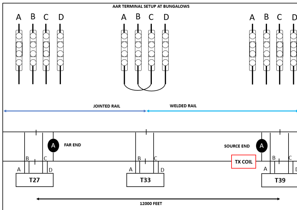
Figure 47. 12,000-foot Block Configuration for Static Testing
