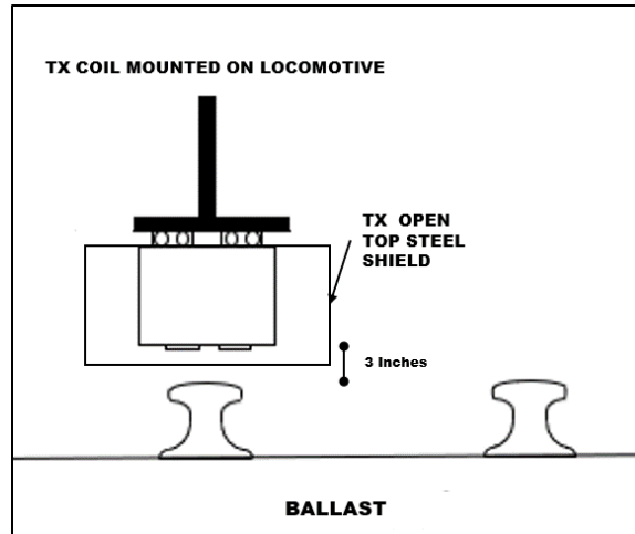
Figure 67. Illustration of Tx Coil Setup When Attached to Locomotive
