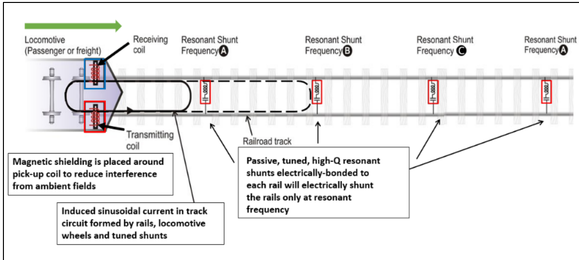
Figure 1. Illustration of the OBRD Concept
