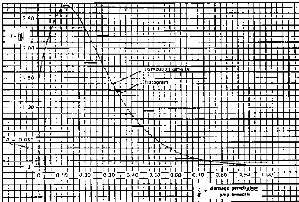
Figure 15 - Distribution density of nondimensional damage penetration
