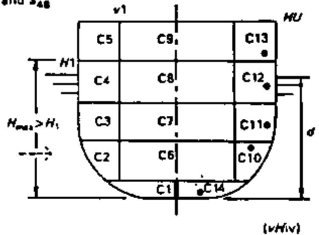
Figure A-12 – Interpretation of combined longitudinal and horizontal subdivision
