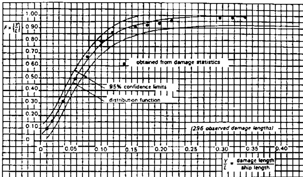
Figure 7 - Distribution function of nondimensional damage length
