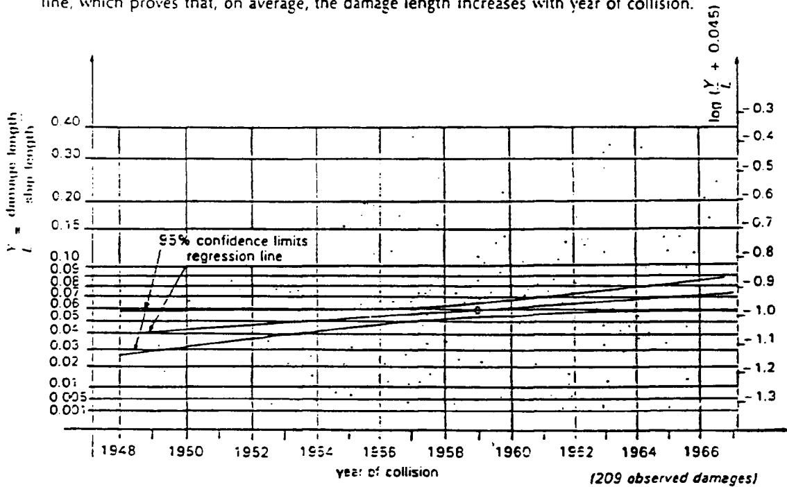
Figure 11 - Regression of nondimensional damage length depending on year of collision
