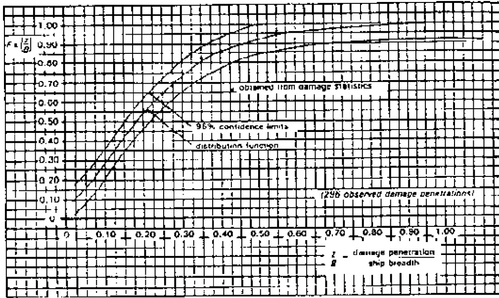
Figure 14 - Distribution function of nondimensional damage penetration
