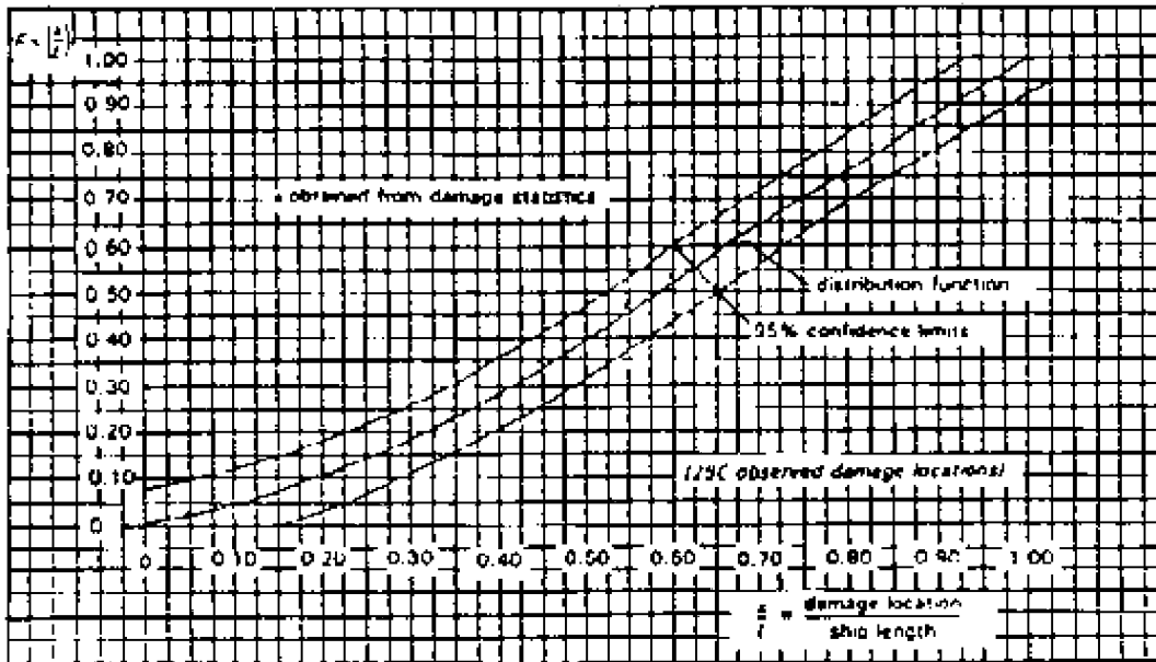
Figure 20 - Distribution function of nondimensional damage location
