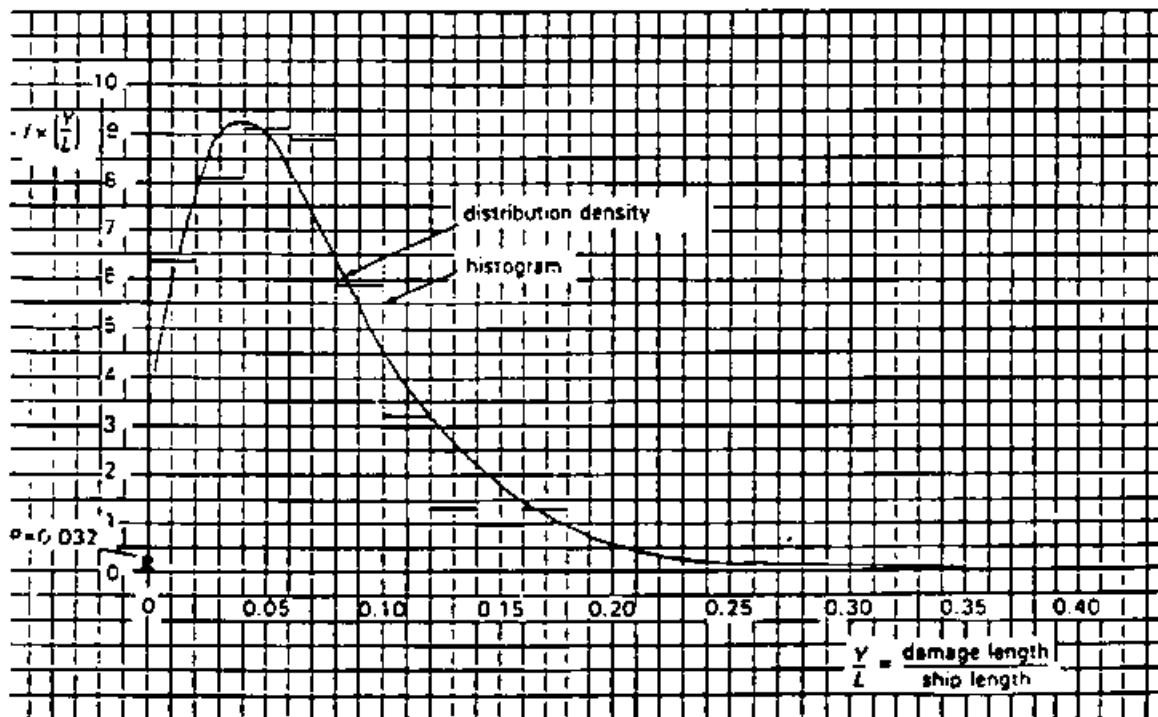
Figure 8 - Distribution density of nondimensional damage length
