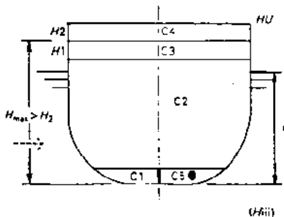
Figure A-10 – Interpretation of multiple horizontal subdivision (in all instances, r = 1 )
