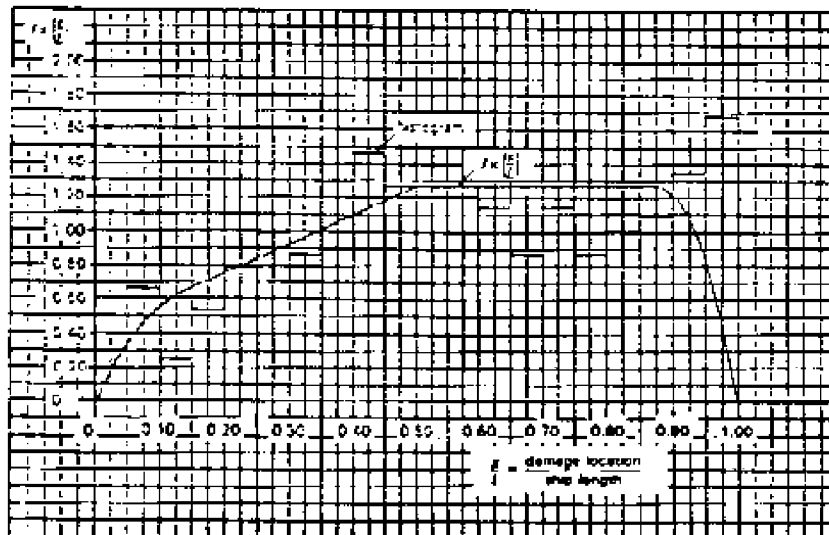
Figure 19 - Distribution density of nondimensional damage location
