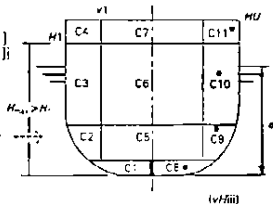
Figure A-11 - Interpretation of combined longitudinal and horizontal subdivision
