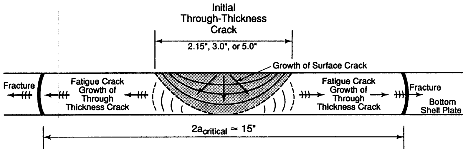
Figure 2. Through Thickness Crack Growth Model. Crack Grows from ~ to 2a_{cr} = 15" at 2a_{cr} – Rapid Fracture Occurs.
