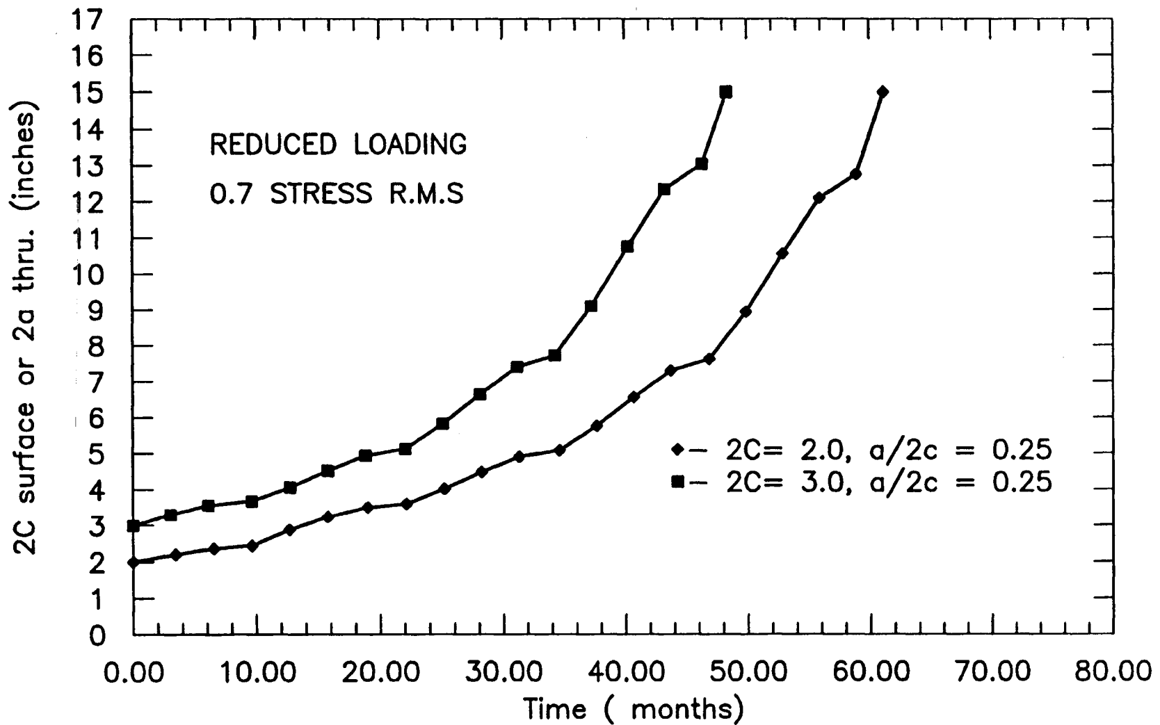
FIG (3)– The effect of 2C value on the crack growth time Using the reduced stress ( 0.7 stress R.M.S )
