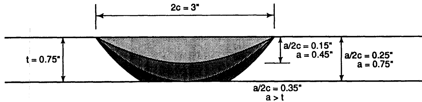
b) 3-Inch Long Surface Crack
