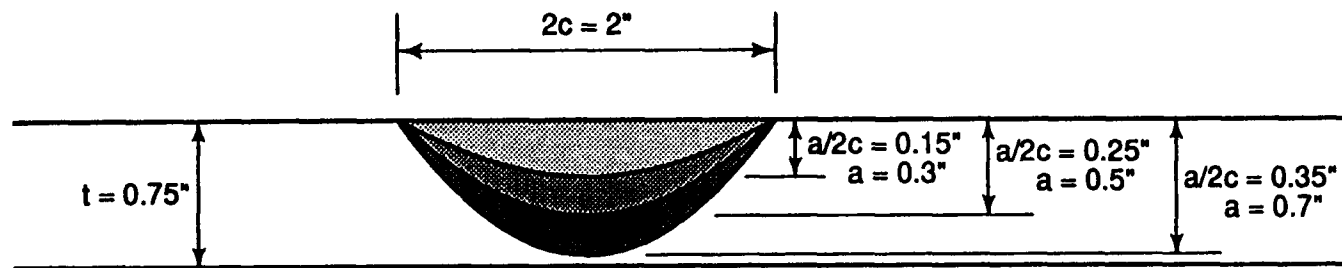
a) 2-Inch Long Surface Crack.
