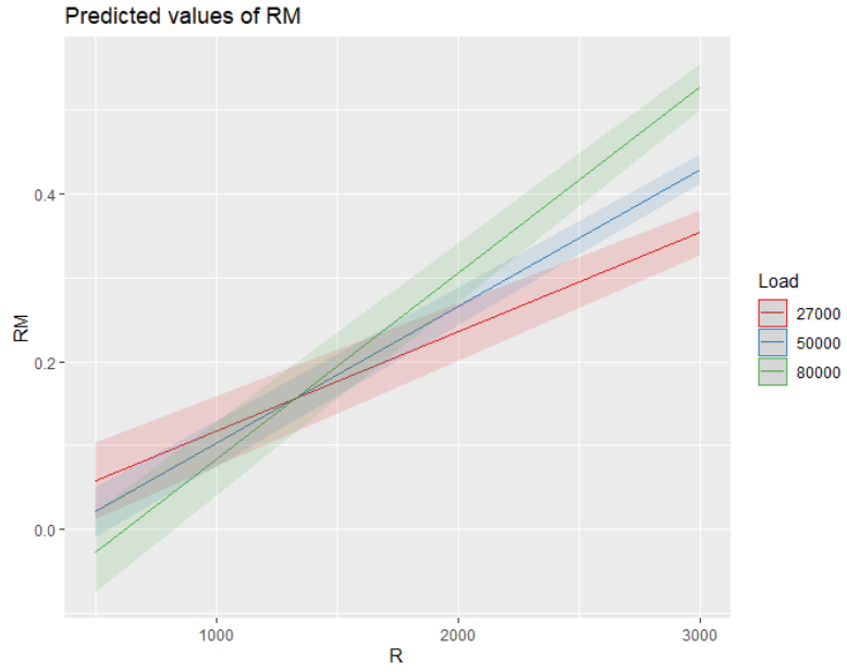
Figure 5.10 The interaction impact of the curve radius and truck gross weight on the rollover margin
