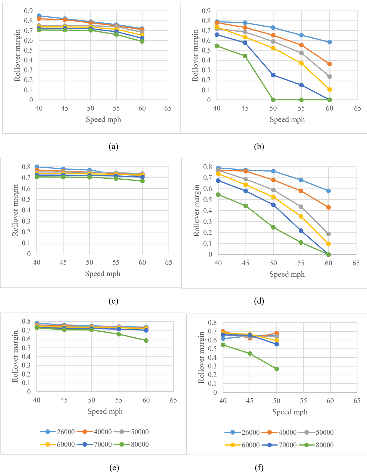
Figure 6.3 The impact of truck speeds with different gross weights on rollover safety margins for moderate-sharpness and sharp curves on dry (a, b), wet (c, d), and snowy roads (e, f)
