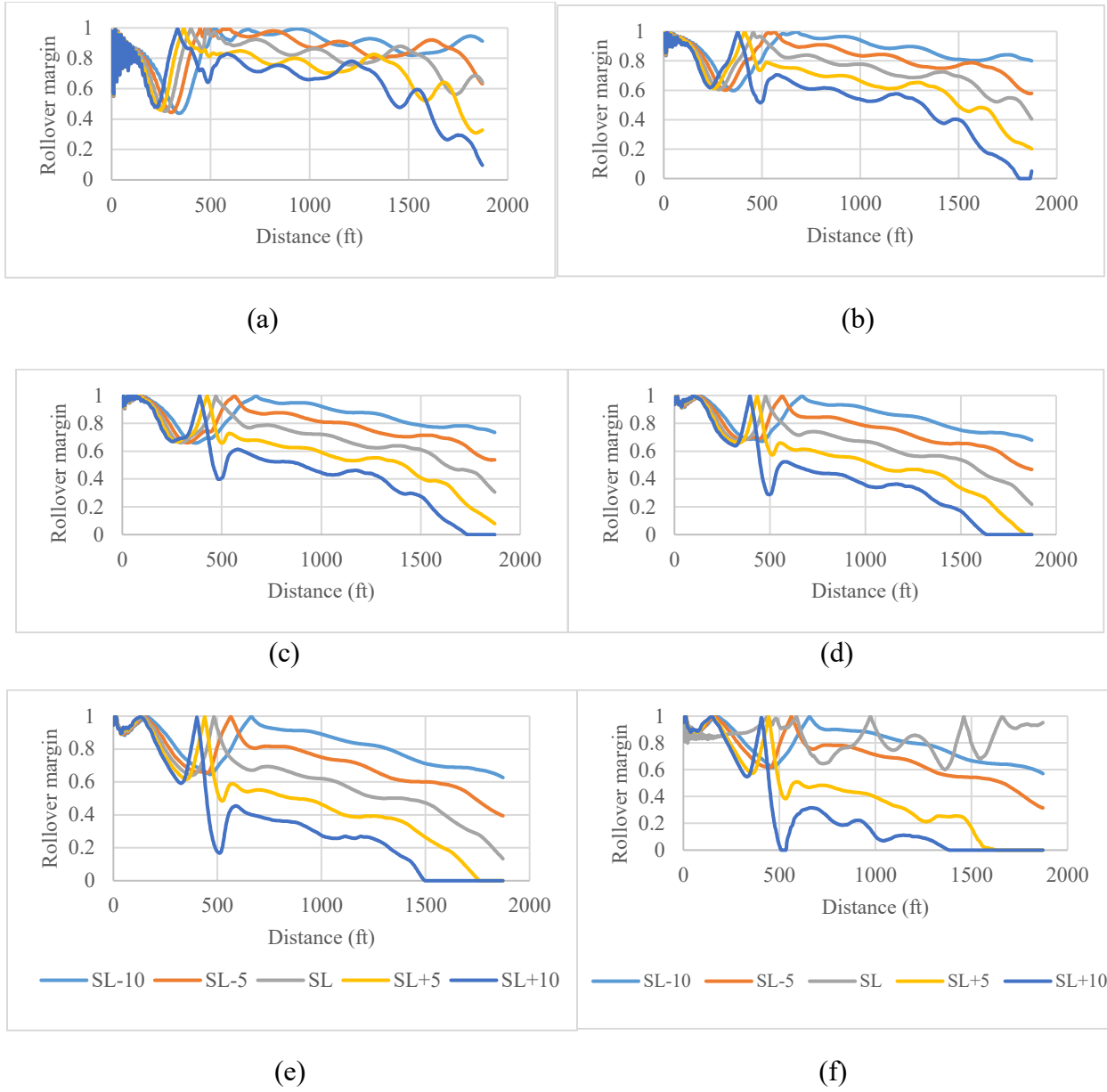
Figure 4.2 Rollover margins for different operating speeds (SL= speed limit) and different truck gross weights on a moderate curve (a–unloaded weight, b–40,000 lb, c–50,000 lb, d–60,000 lb, e–70,000 lb, f–80,000 lb)
