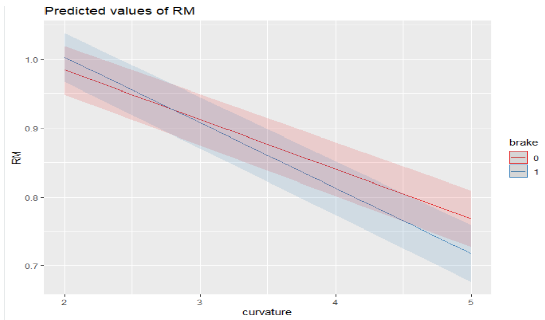
Figure 3.10 The impact of brake application on rollover margin for different degrees of curvature for SUV (RM: rollover margin)
