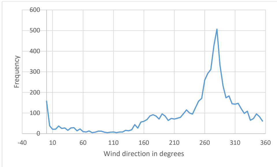
Figure 5.2 Frequency periods of the wind directions on I-80 for the last three years in the winter season
