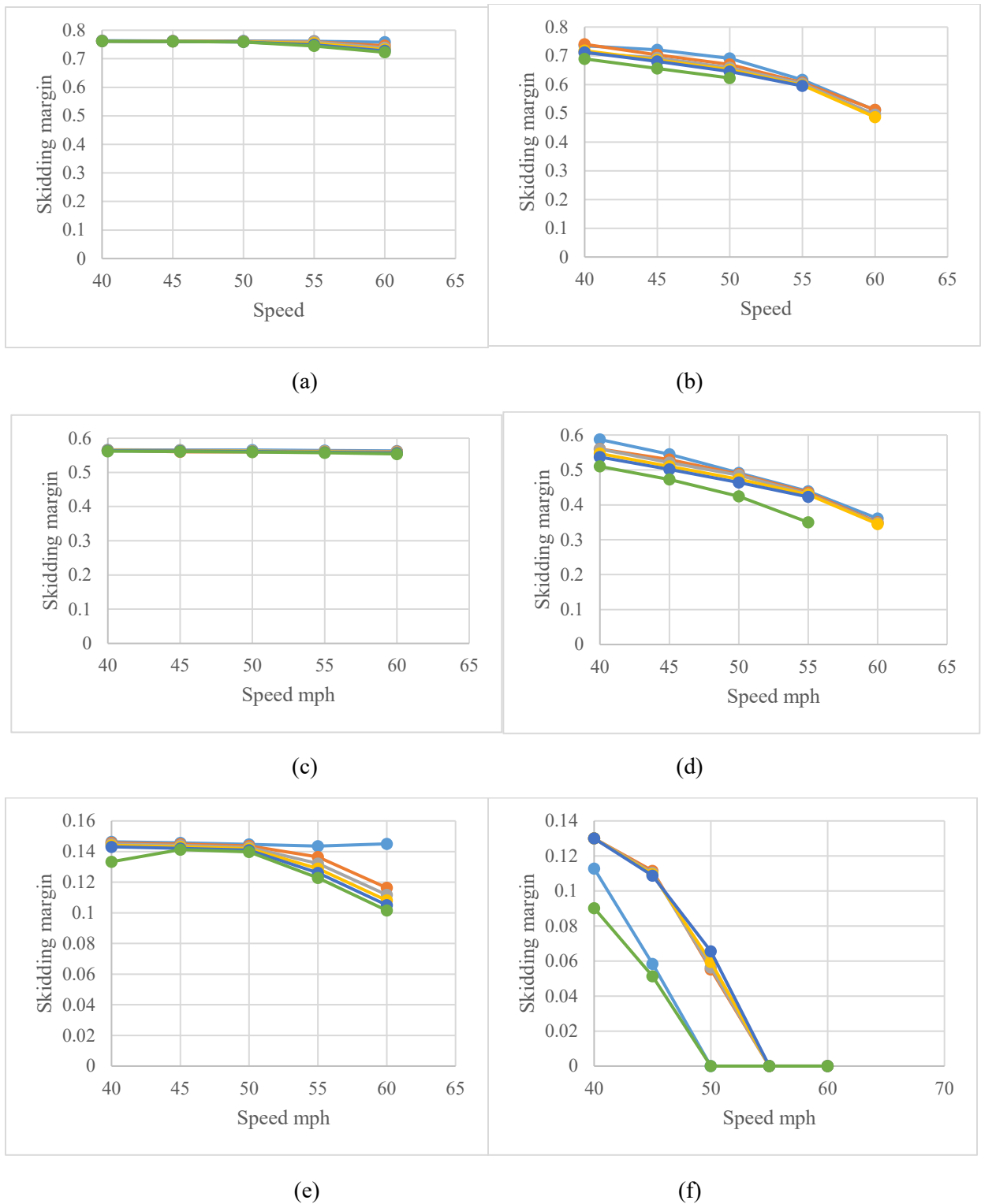
Figure 6.2 The impact of truck speeds with different gross weights on skidding safety margins for moderate-sharpness and sharp curves on dry (a, b), wet (c, d), and snowy roads (e, f)
