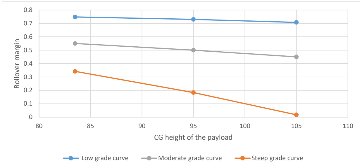
Figure 4.4 Rollover margin for different downgrades along with CG height values of payload
