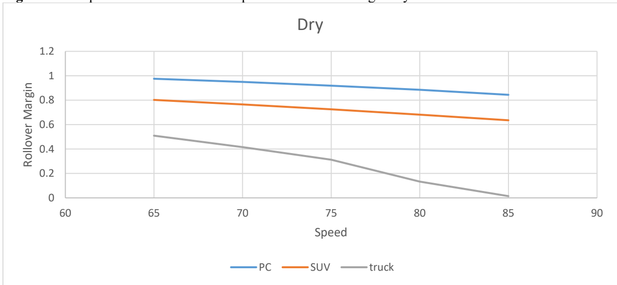
Figure 3.7 Impact of vehicle type on rollover margins
