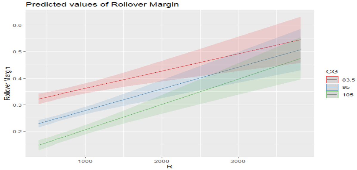
Figure 4.5 Rollover margin for different CG heights of payload with curve radius values
