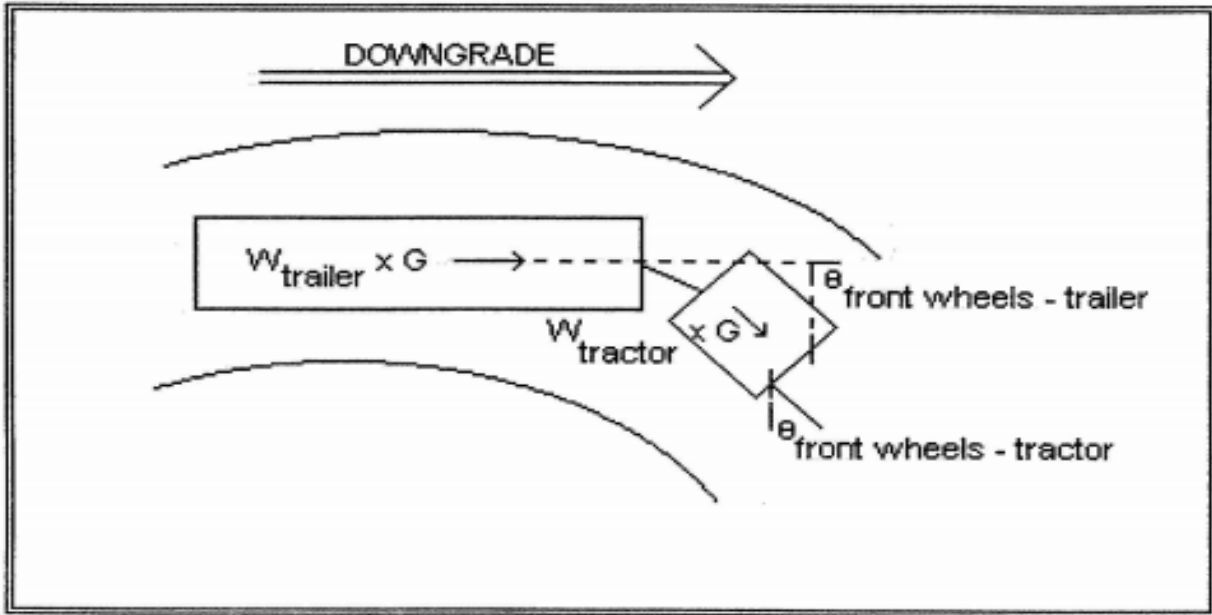
Figure 1.1 The condition of the center of gravity in tractor and trailer of an articulated vehicle on combined horizontal curves with vertical alignments (Eck and French 2003)
