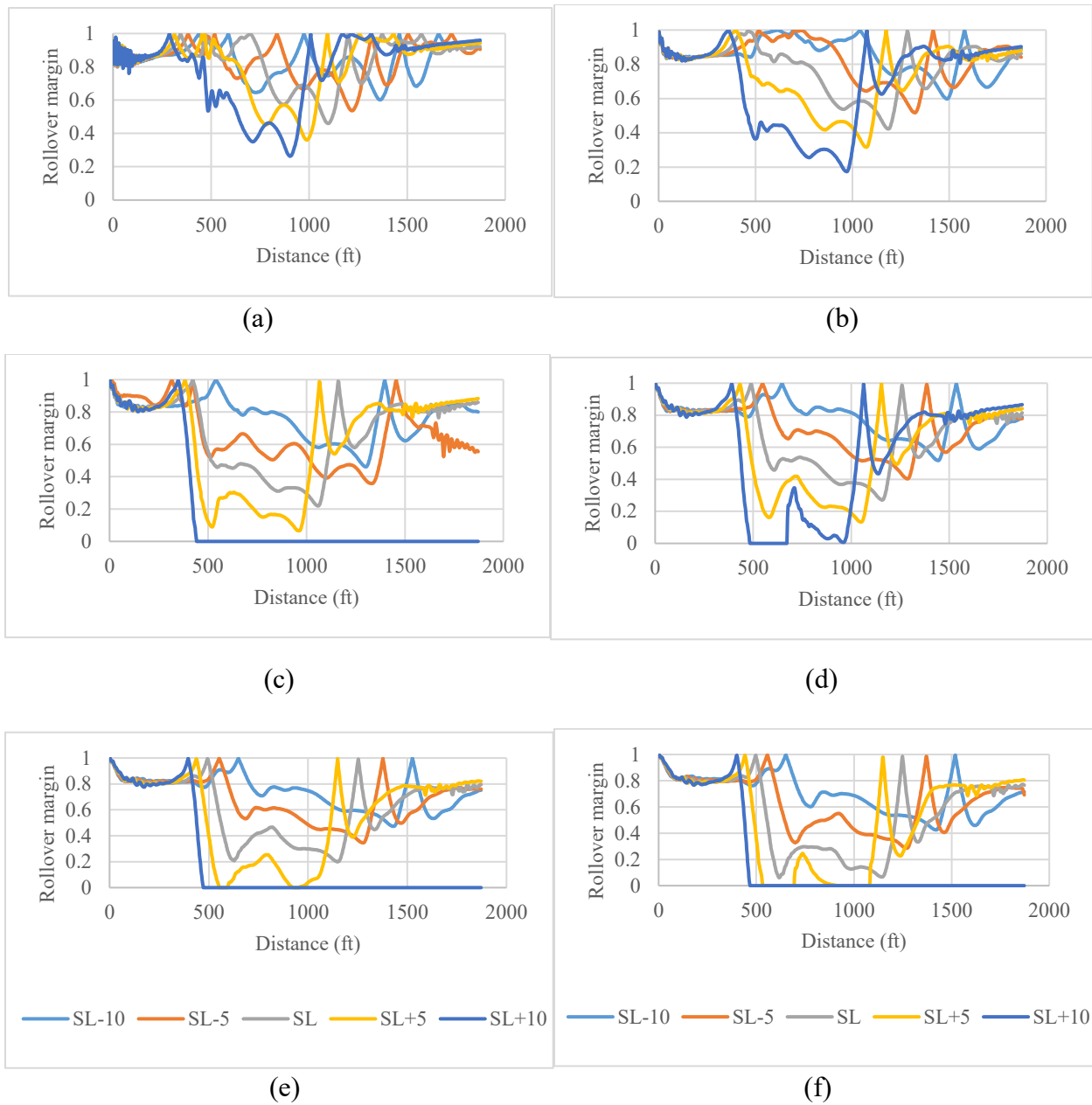
Figure 4.3 Rollover margins for different operating speeds (SL=speed limit) and different truck gross weights on a sharp curve (a–unloaded weight, b–40,000 lb, c–50,000 lb, d–60,000 lb, e–70,000 lb, f–80,000 lb)
