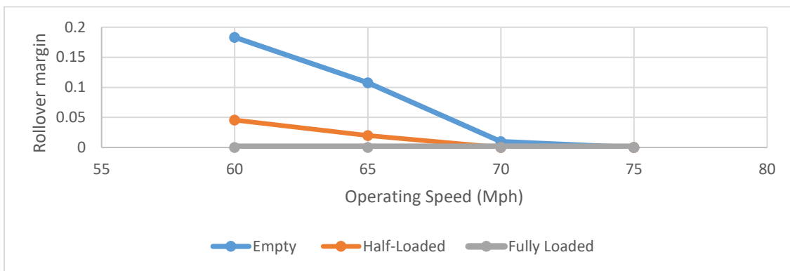
(c) Sharp and steep curve case
