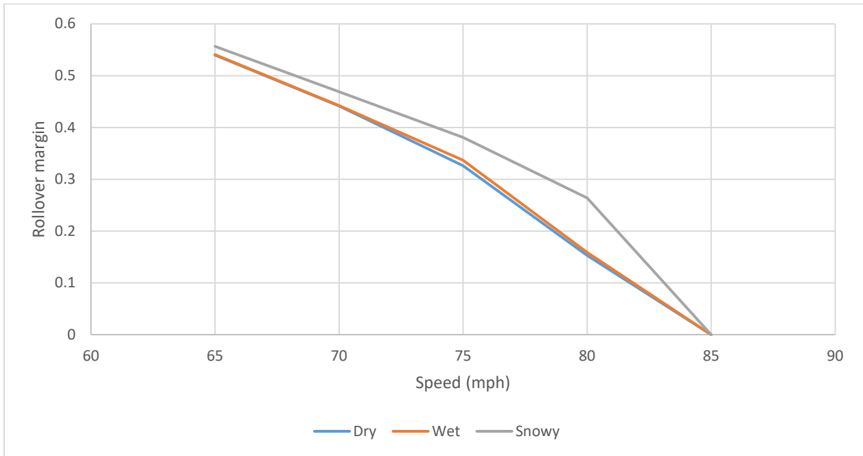
Figure 3.6 Impact of semi-trailer truck speeds on rollover margins by road surface condition
