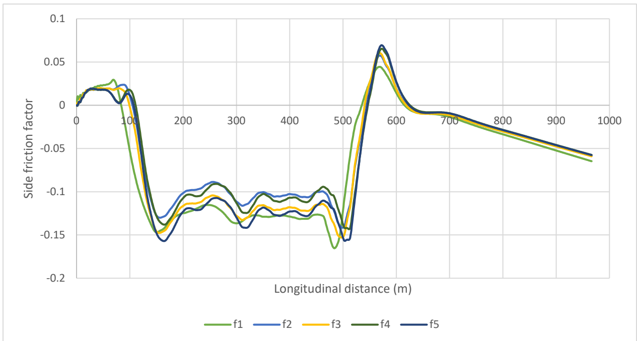
b) Side friction factor for each truck axle on a right-turn curve (moderate downgrade)
