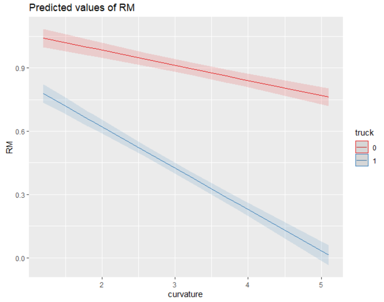
Figure 3.11 The interaction impact between the truck vehicle and different curvature degrees on rollover margin (RM: rollover margin)
