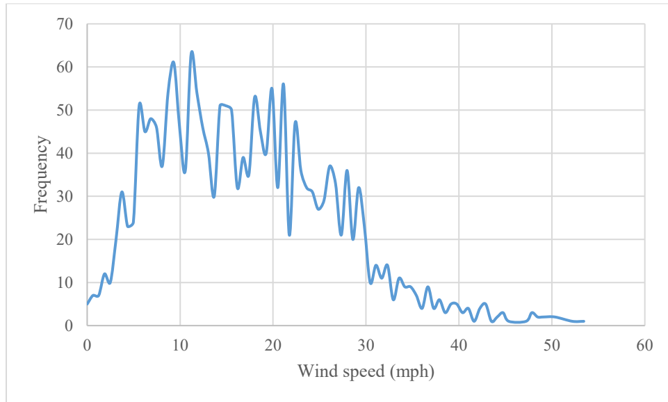
Figure 5.1 Frequency periods of the wind speeds on I-80 for the last three years in the winter season
