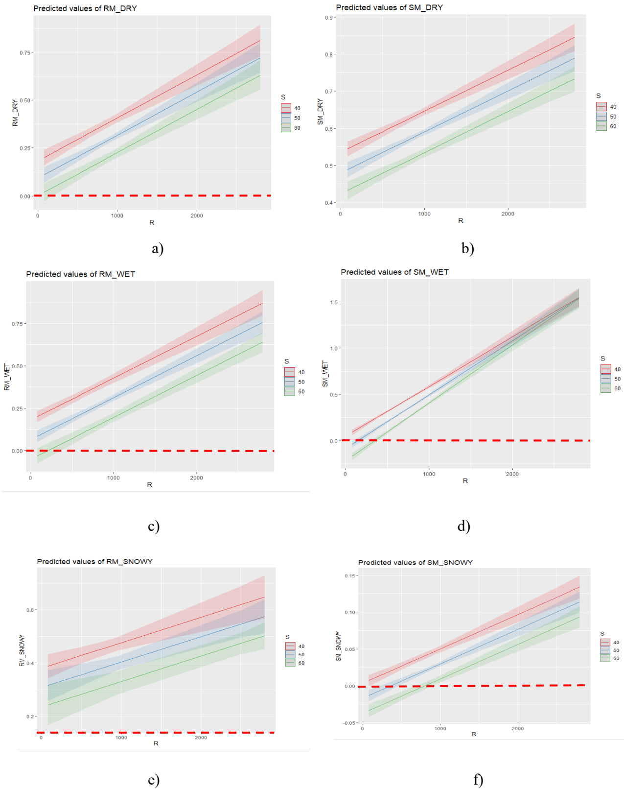
Figure 6.4 The impact of truck speeds (S) with different curve radii (R) on SM and RM on dry (a, b), wet (c, d), and snowy roads (e, f) (The red dashed line represents the skidding and rollover point, safety margin = 0)
