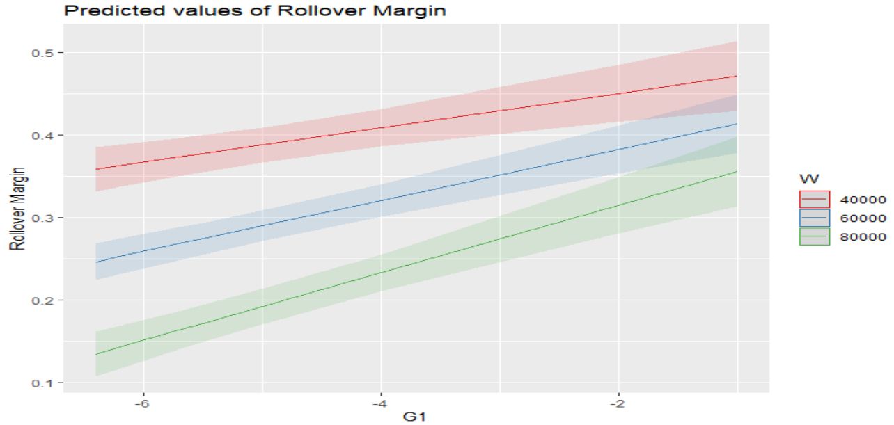
Figure 4.7 Rollover margin for different truck gross weights along with grade values
