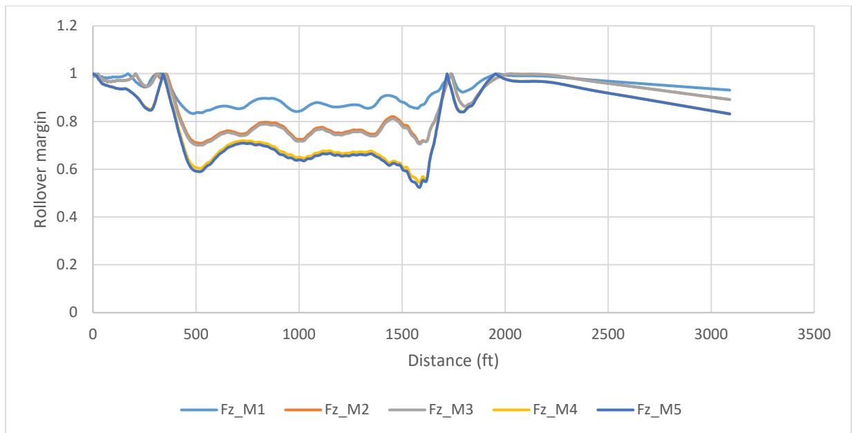
a) Rollover margin for each truck axle on a right-direction moderate curve
