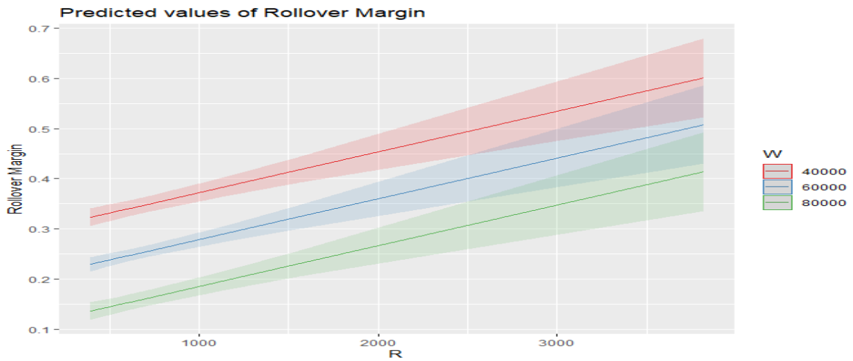
Figure 4.6 Rollover margin for different truck gross weights along with curve radius values
