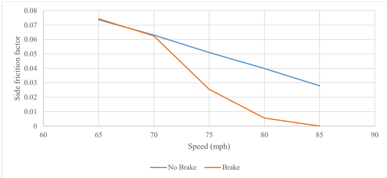
a) The impact of brake application on snowy road surfaces for the passenger car
