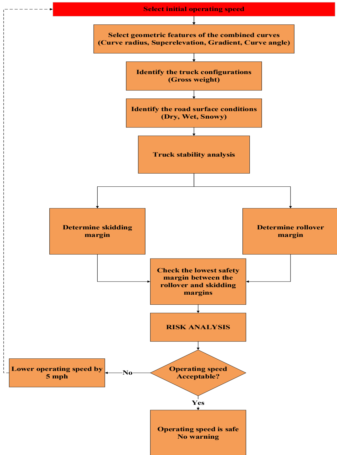
Figure 6.6 Speed limit assessment framework
