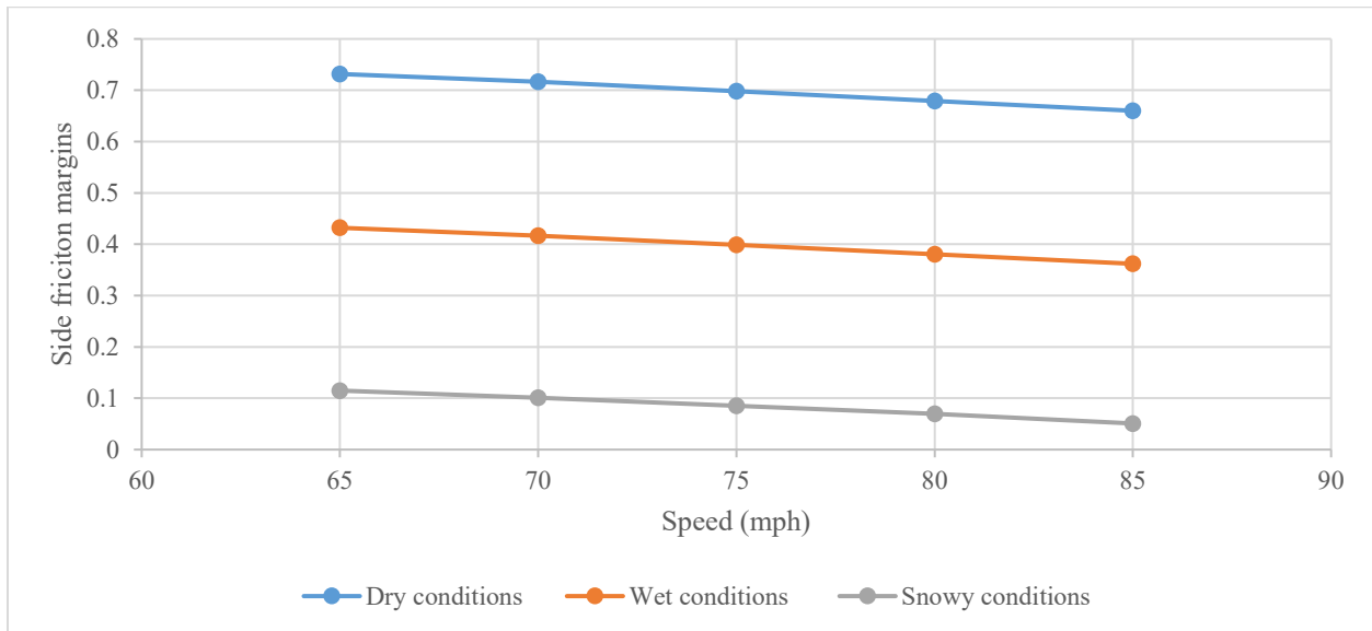
Figure 3.2 The impact of passenger car's speed on the side friction margin for different road surface conditions (moderately sharp curve)
