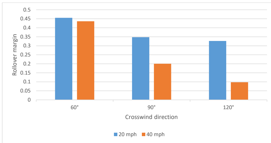
Figure 5.9 The relationship between the wind speed and direction with respect to the rollover margin
