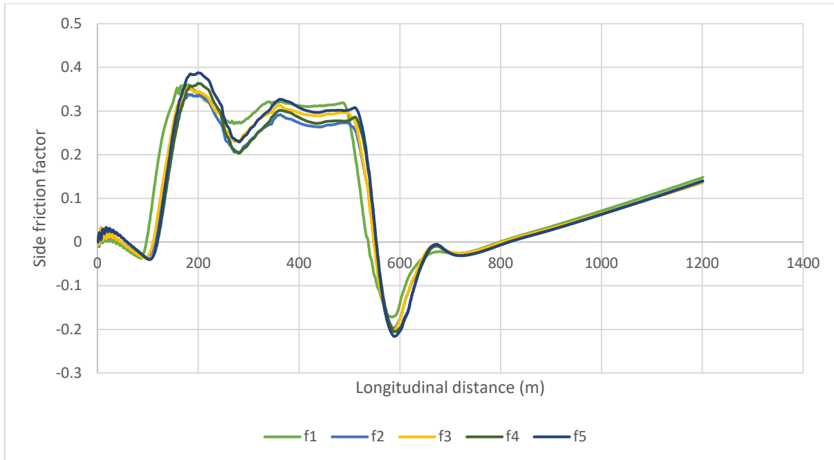
c) Side friction factor for each truck axle on a left-turn curve (steep downgrade)
