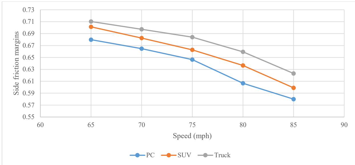
Figure 3.3 The impact of different types of vehicles on the side friction margin
