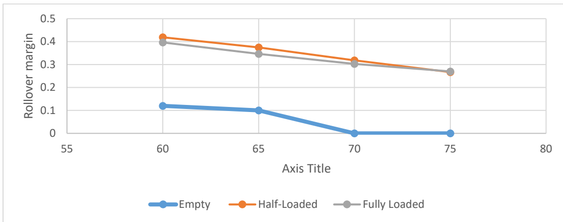
(b) Moderate sharpness and steepness curve case
