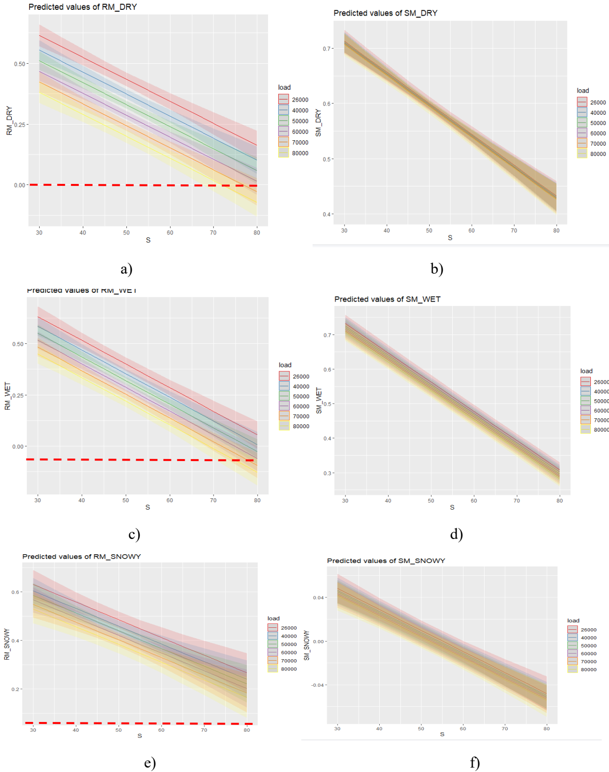
Figure 6.5 The impact of truck gross weights in lbs with different speeds (S) on SM and RM on dry (a, b), wet (c, d), and snowy roads (e, f) (The red dashed line represents the skidding and rollover point, safety margin = 0)
