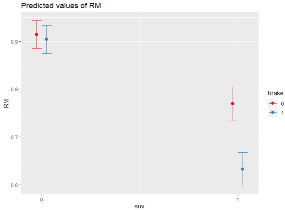
Figure 3.9 The interaction impact between SUV vehicle and brake application on rollover margin (RM: rollover margin)
