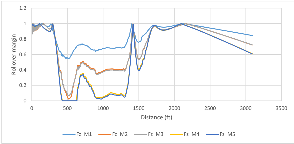
b) Rollover margin for each truck axle on a left-direction tight curve
