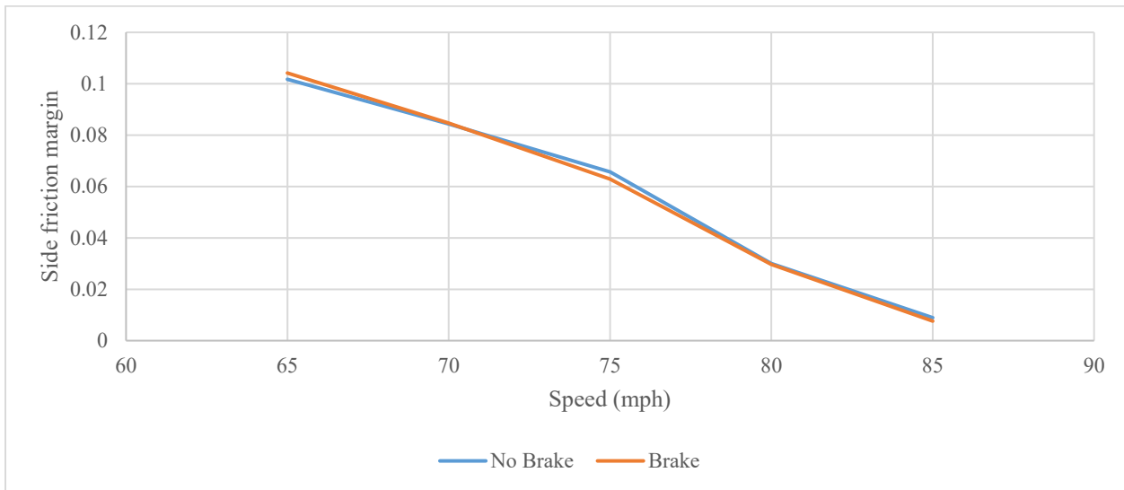
b) The impact of brake application on snowy road surfaces for the SUV
