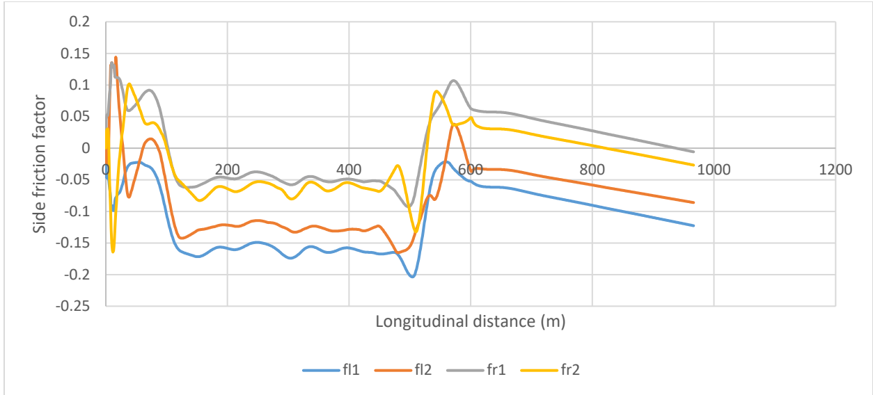
a) Side friction factor for each passenger car tire on a right-turn curve (moderate downgrade)
