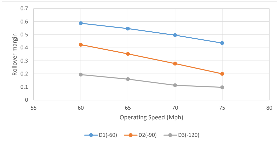
Figure 5.8 Rollover margins for different crosswind directions
