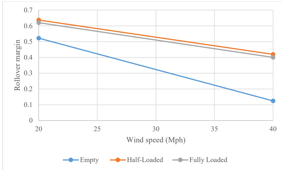
Figure 5.5 Rollover margins for different truckload conditions under various wind speeds
