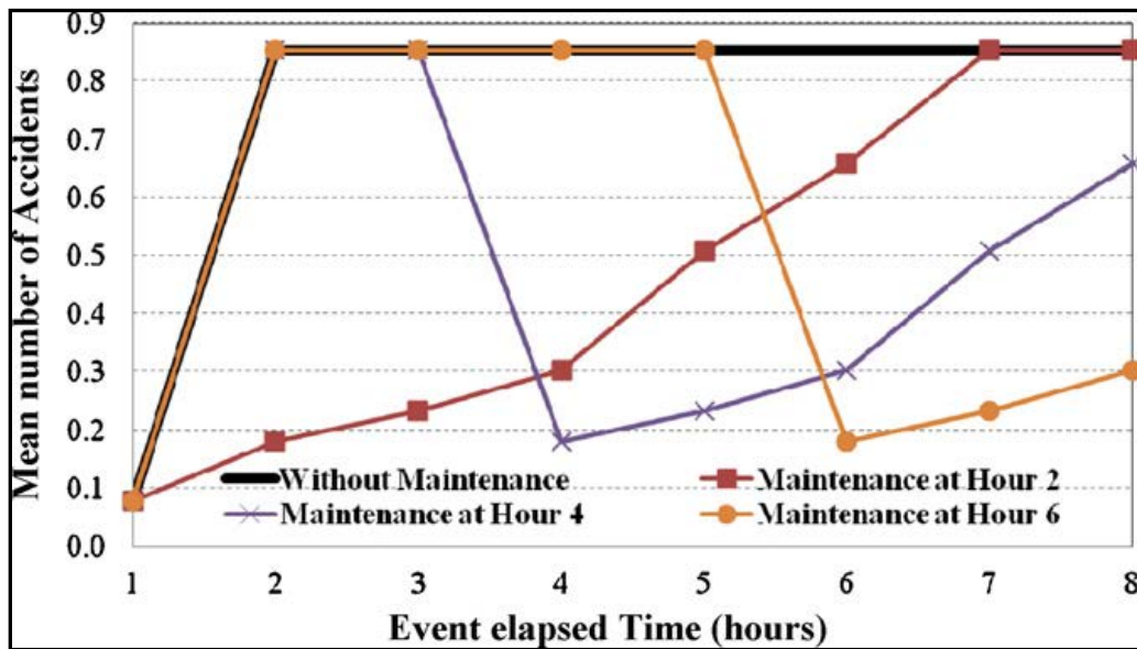
Figure 2. Safety Benefits of Plowing and Salting Operations Versus No Maintenance (88)
