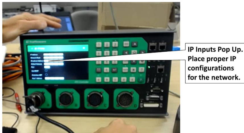
Figure 9. Trafficware Commander Initializing Controller-IP Setup
