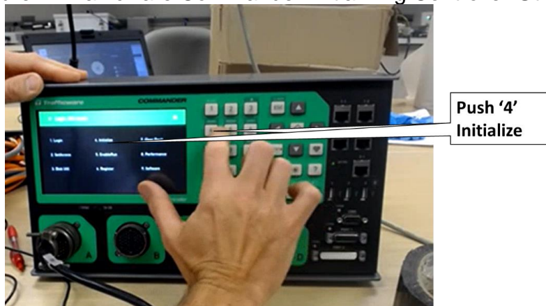
Figure 5. Trafficware Commander Initializing Controller-Initialize
