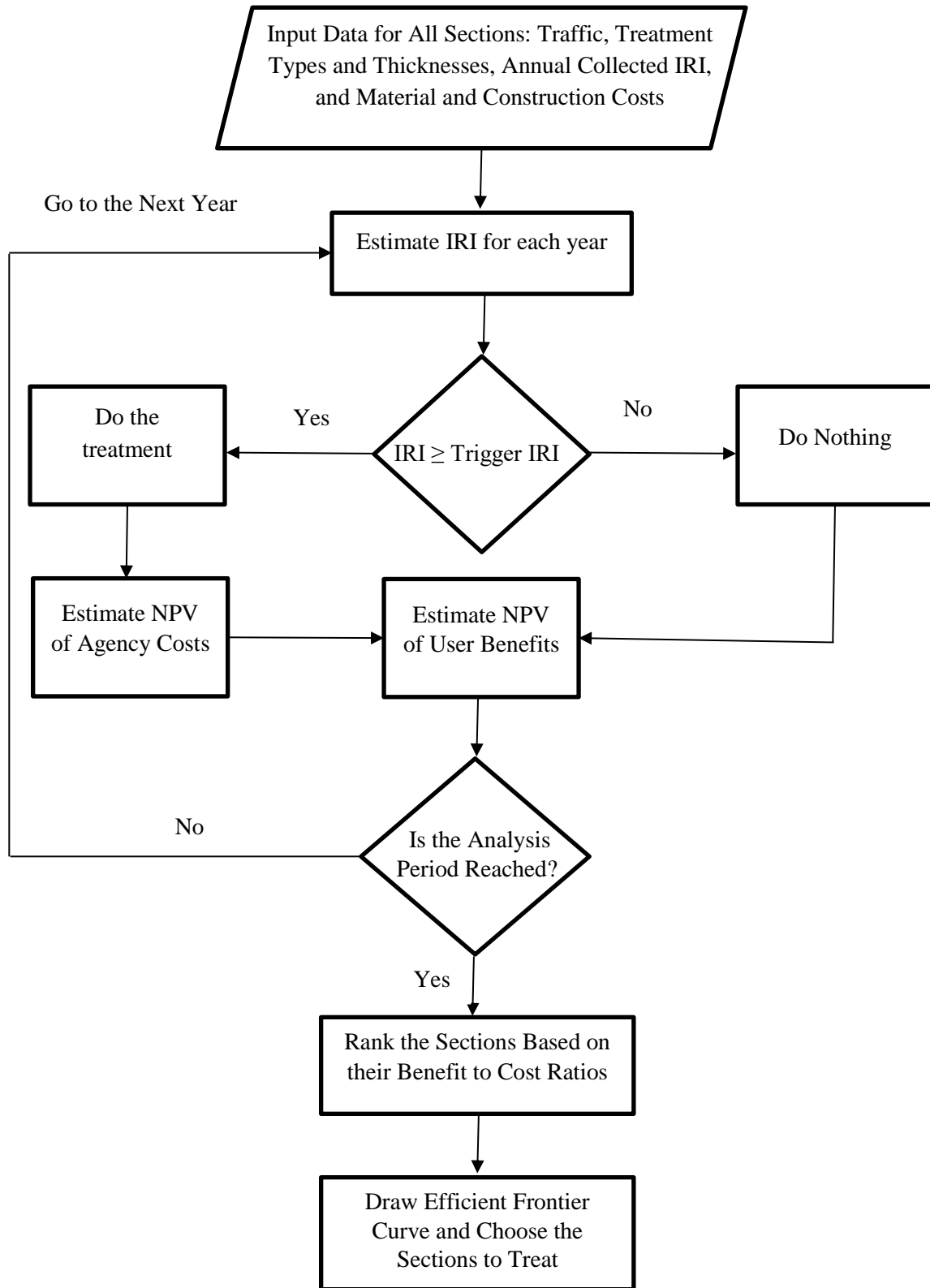
Figure 3.1. Flowchart of procedure to develop the decision-making tool (MATLAB code)
